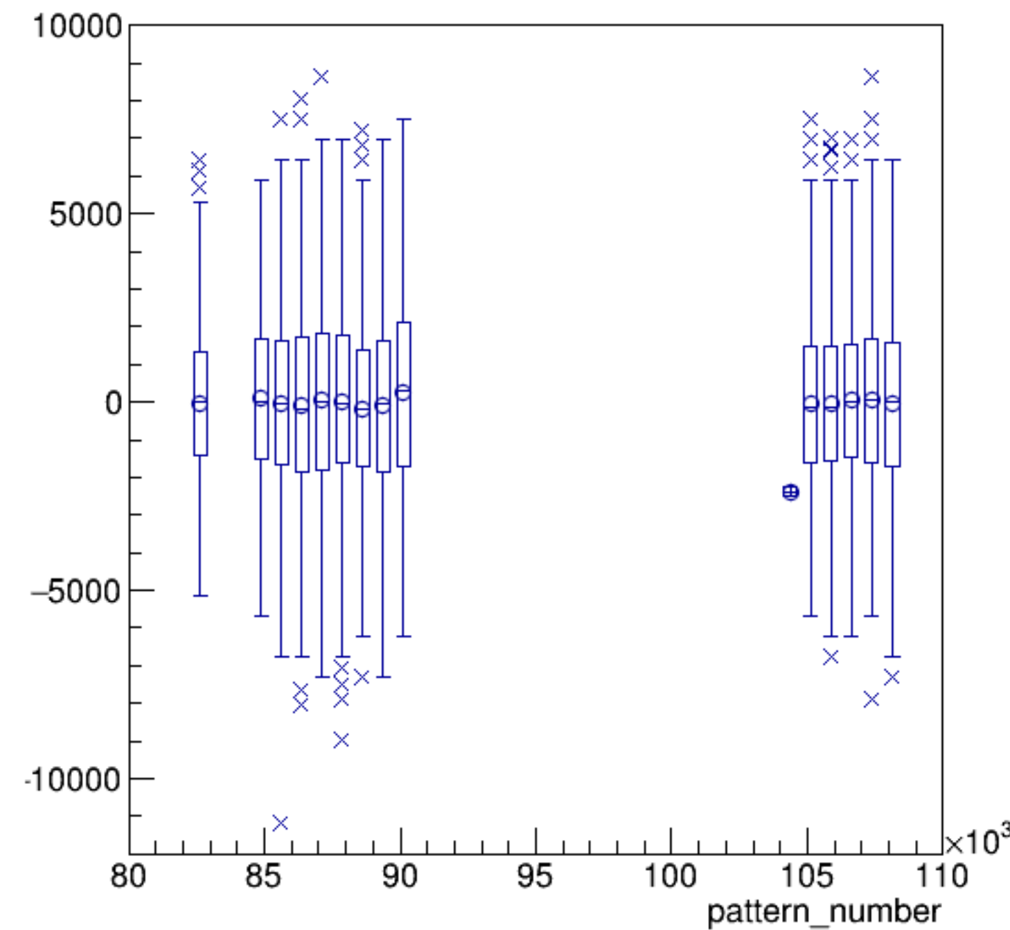
asym_sam4/ppm:pattern_number {ErrorFlag==0}
