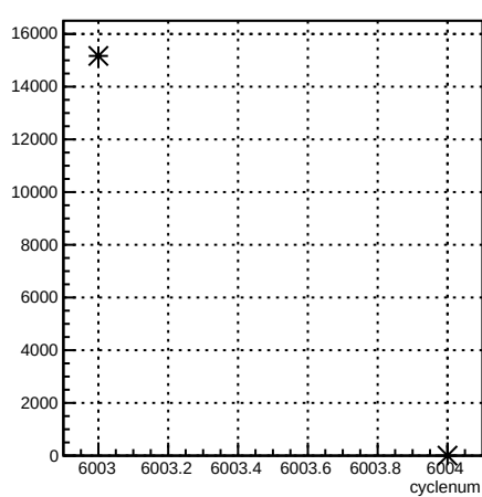
usl_coil7:cyclenum {run == 6334}
