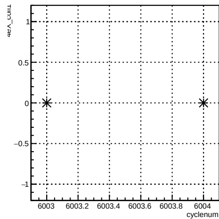
4eX_coil1:cyclenum {run == 6334}
