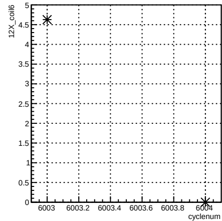
12X_coil6:cyclenum {run == 6334}
