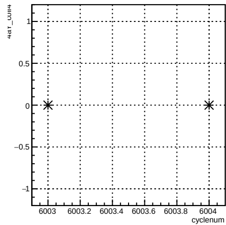
4eY_coil4:cyclenum {run == 6334}
