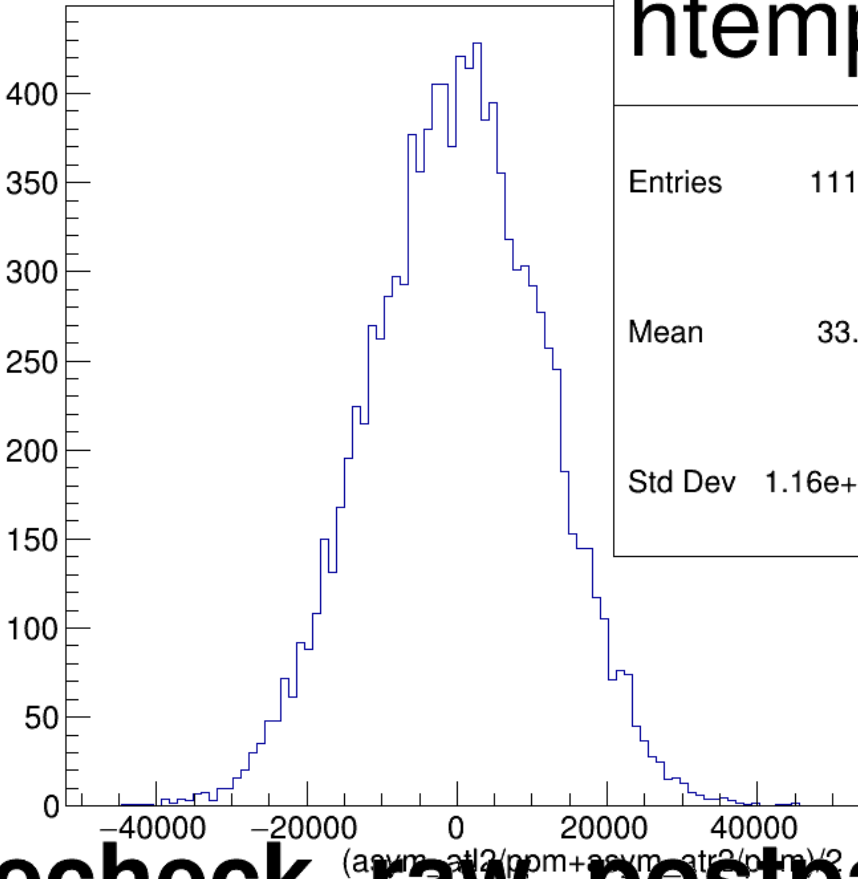
(asym_atl2/ppm+asym_atr2/ppm)/2 {ok_cut}
