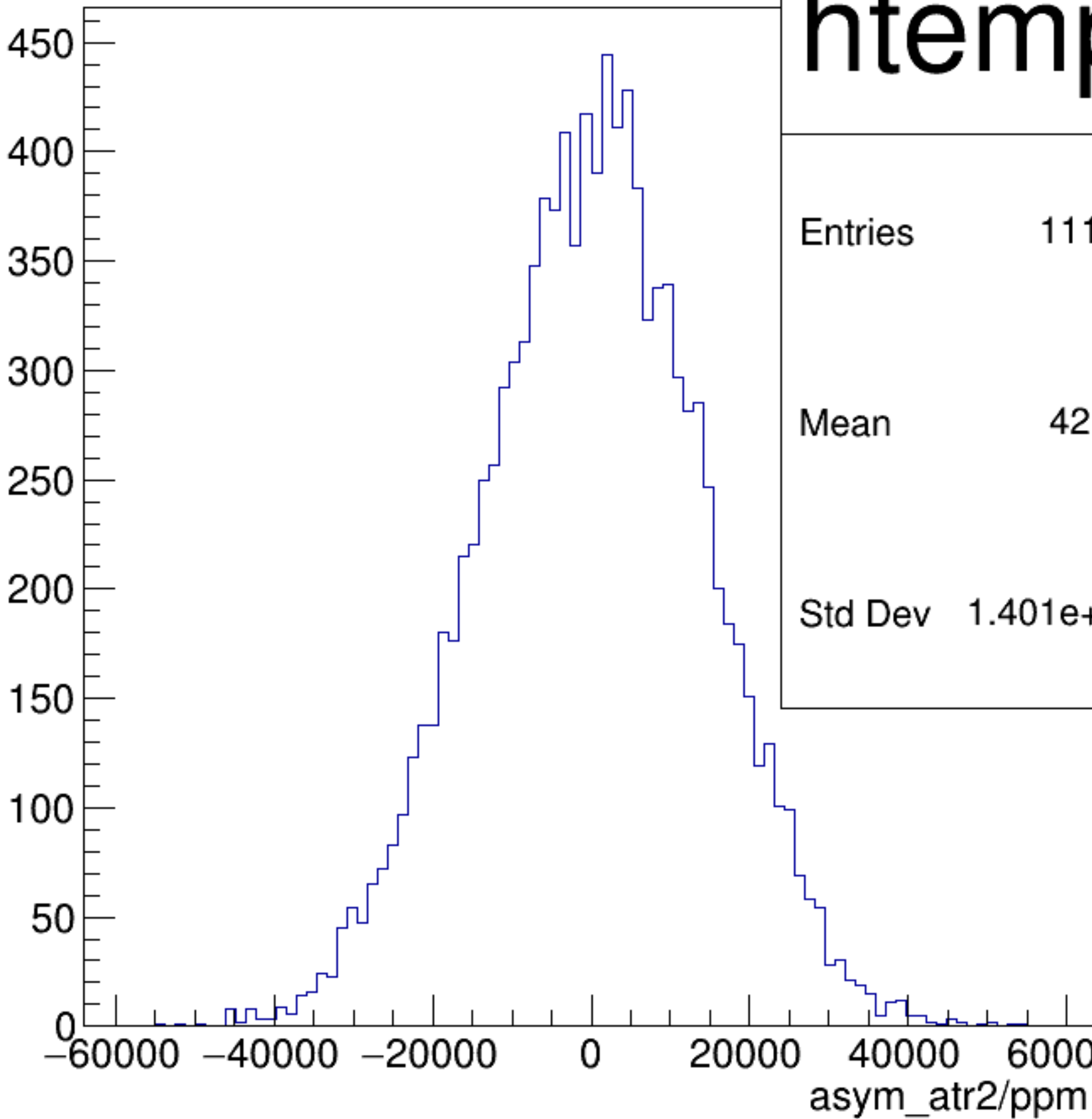
asym_atr2/ppm {ok_cut}
