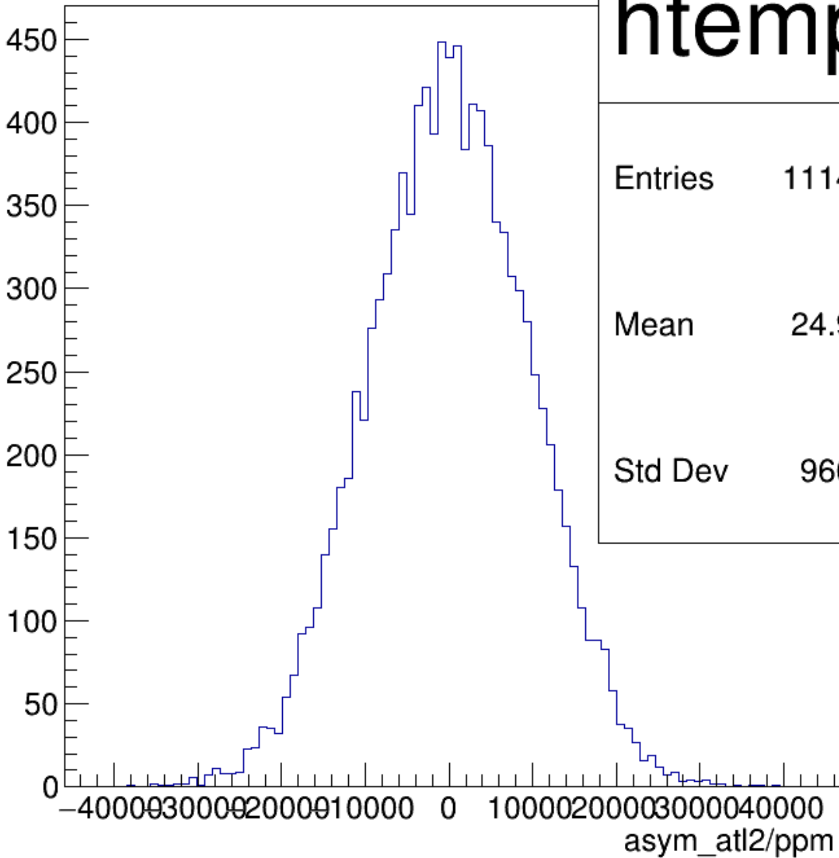
asym_atl2/ppm {ok_cut}
