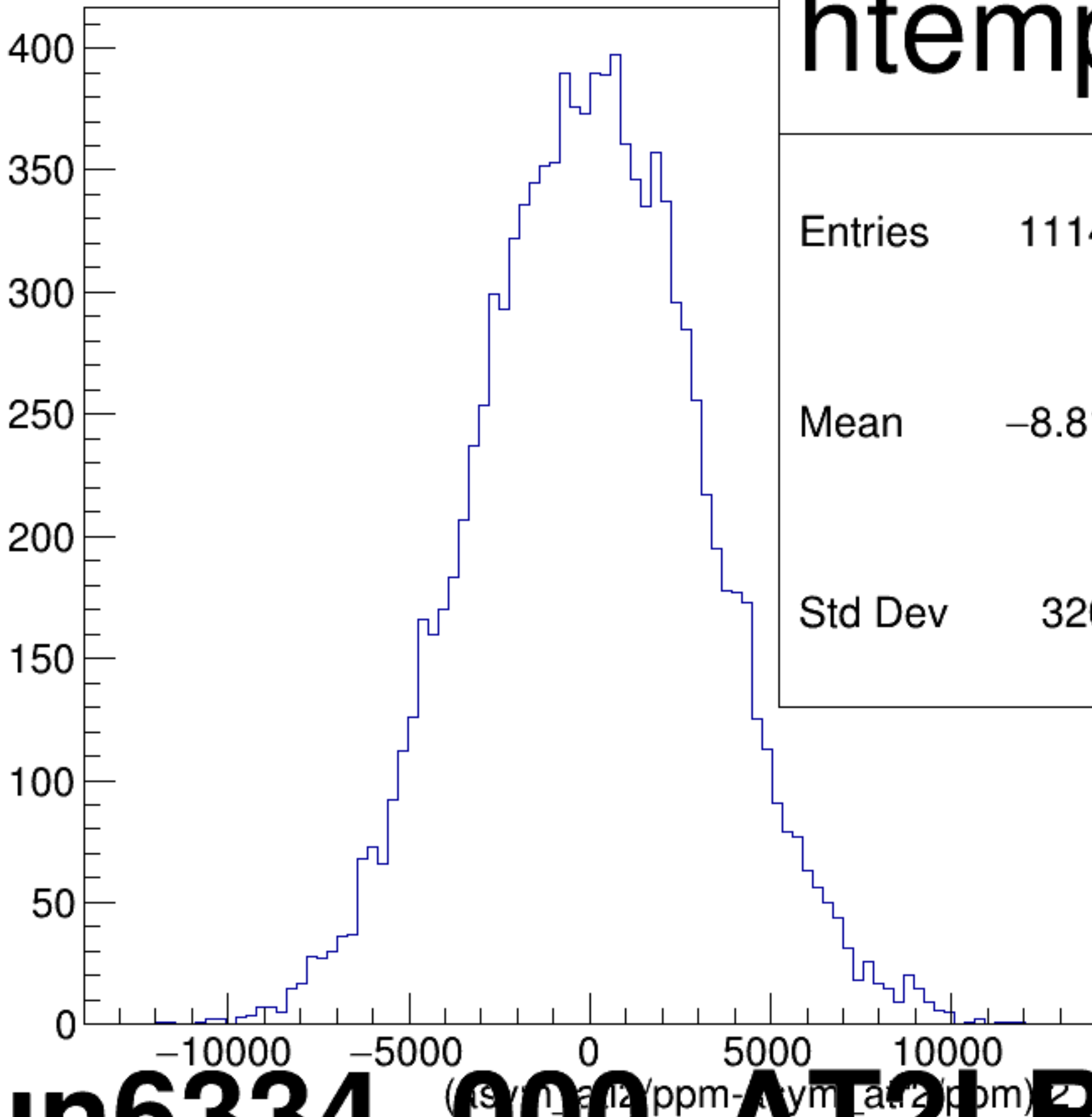
(asym_atl2/ppm-asym_atr2/ppm)/2 {ok_cut}
