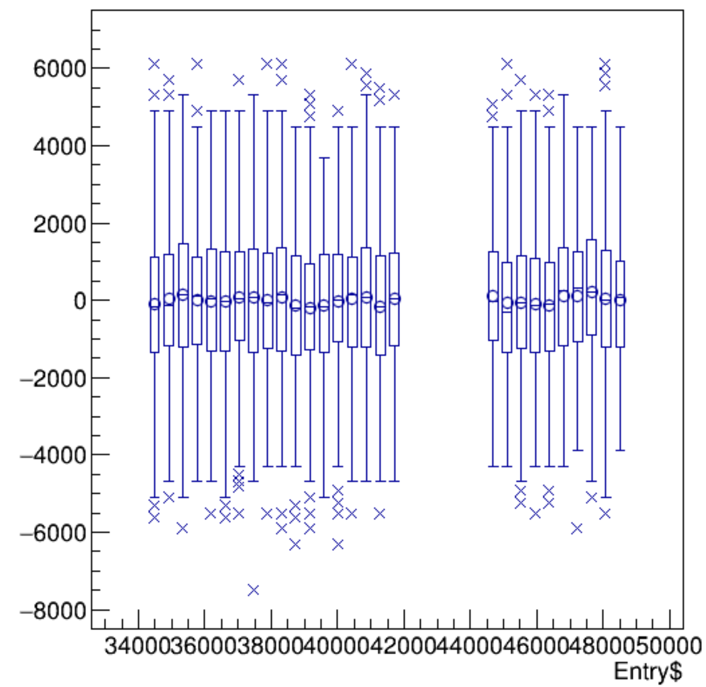
(reg_asym_atl2/ppm-reg_asym_atr2/ppm)/2:Entry$ {ok_cut}
