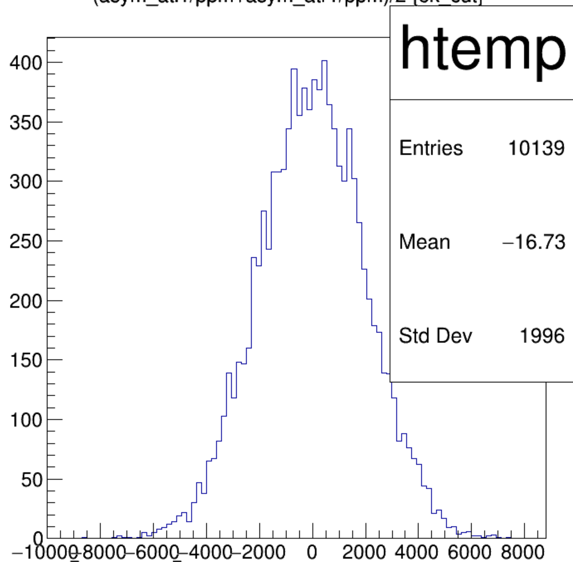
(asym_atl1/ppm+asym_atr1/ppm)/2 {ok_cut}
