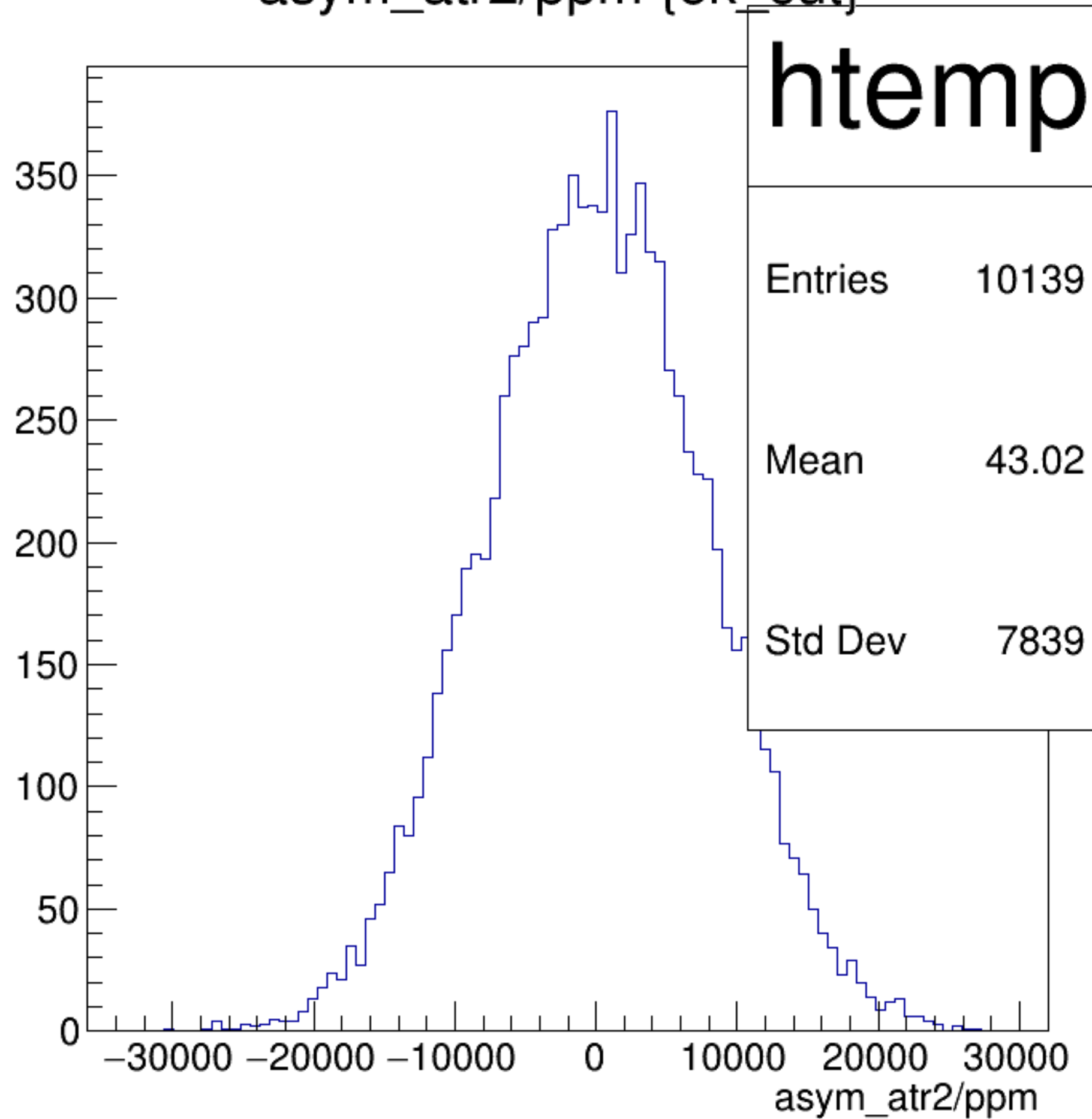
asym_atr2/ppm {ok_cut}
