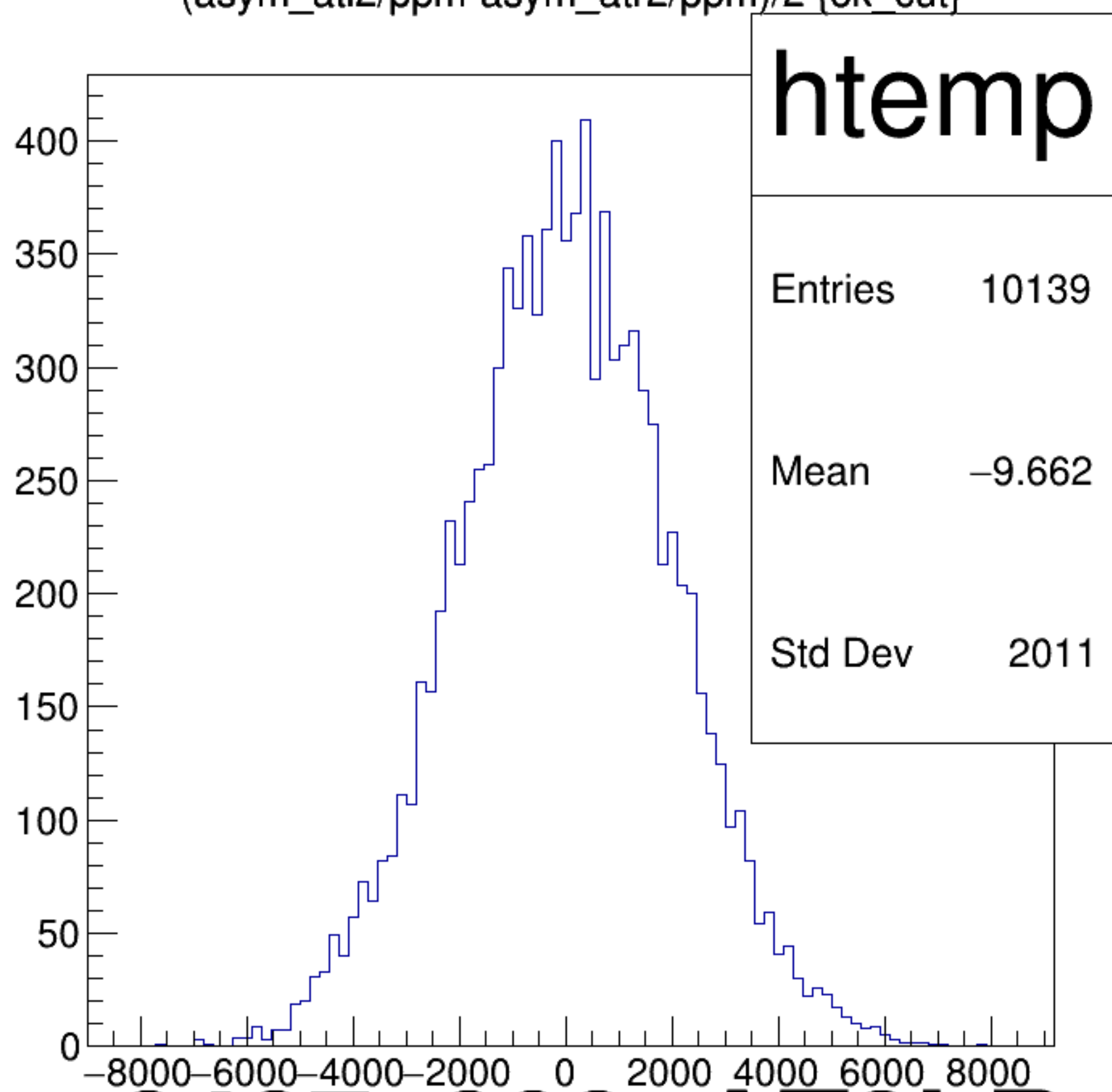
(asym_atl2/ppm-asym_atr2/ppm)/2 {ok_cut}
