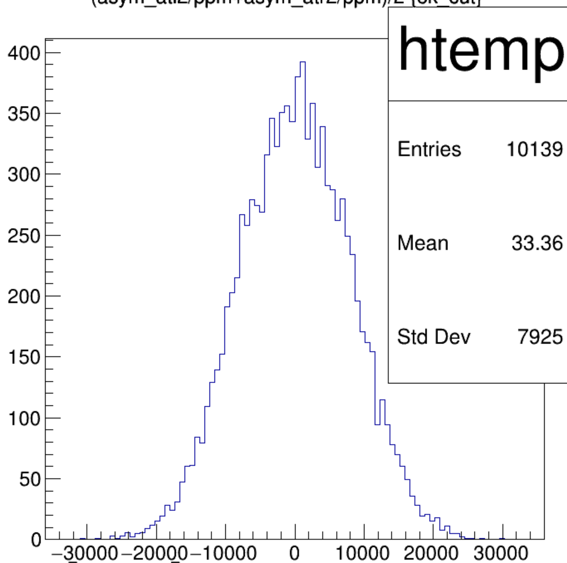
(asym_atl2/ppm+asym_atr2/ppm)/2 {ok_cut}
