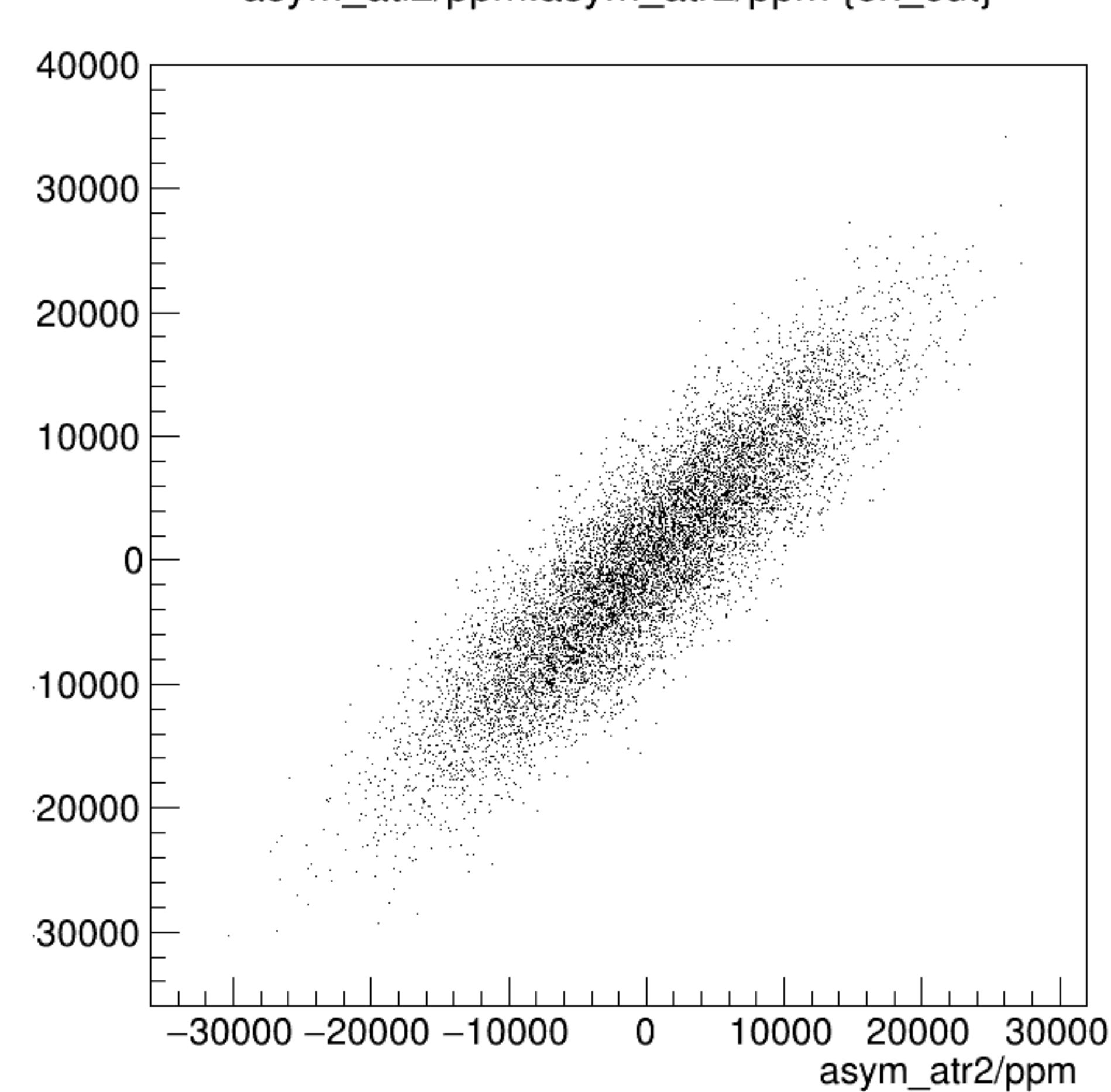
asym_atl2/ppm:asym_atr2/ppm {ok_cut}
