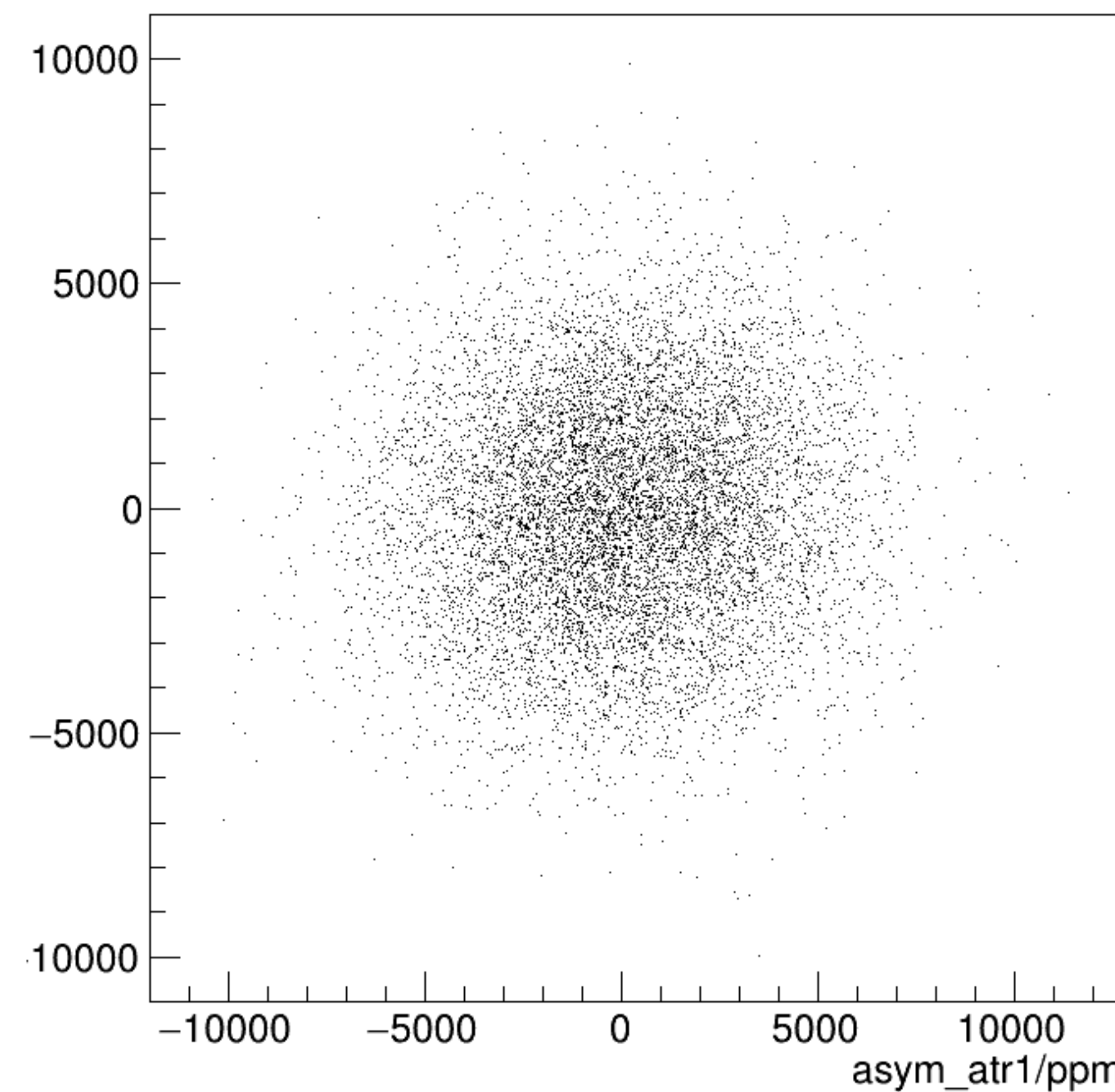
asym_atl1/ppm:asym_atr1/ppm {ok_cut}
