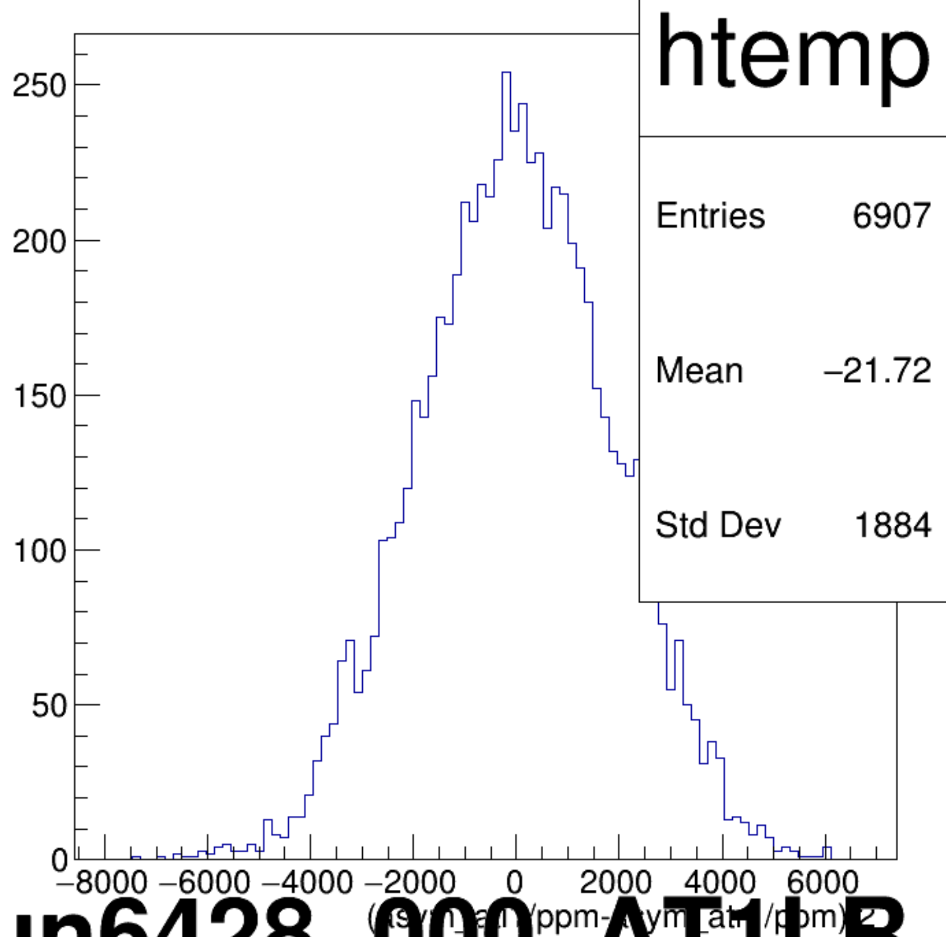
(asym_atl1/ppm-asym_atr1/ppm)/2 {ok_cut}
