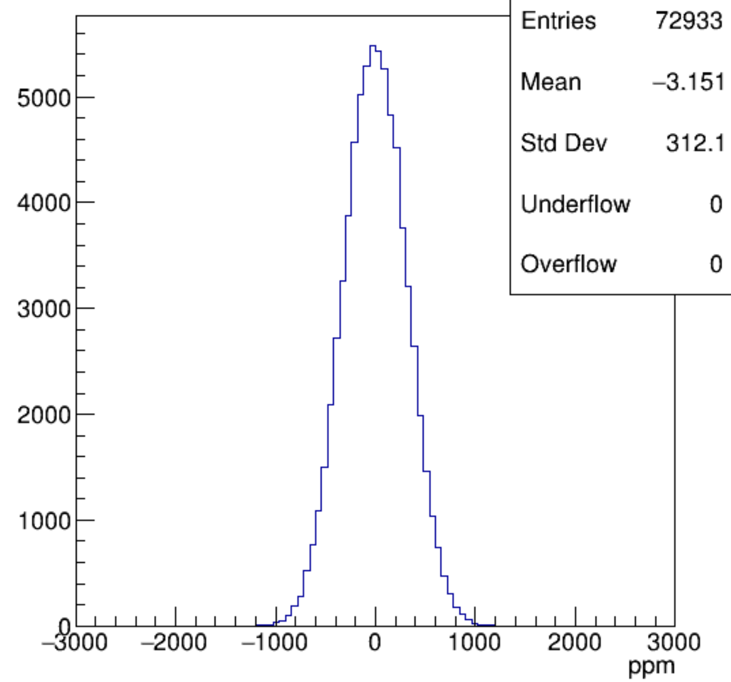
asym_sam8
