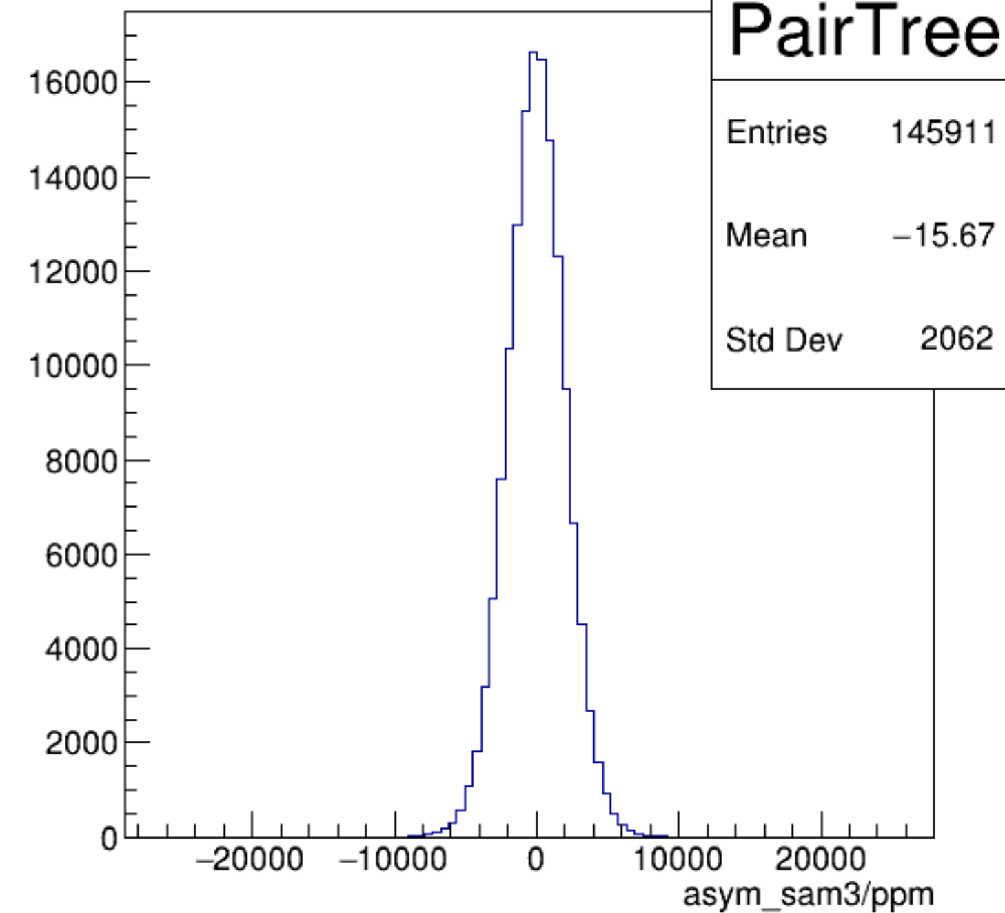
asym_sam3/ppm {ErrorFlag==0}
