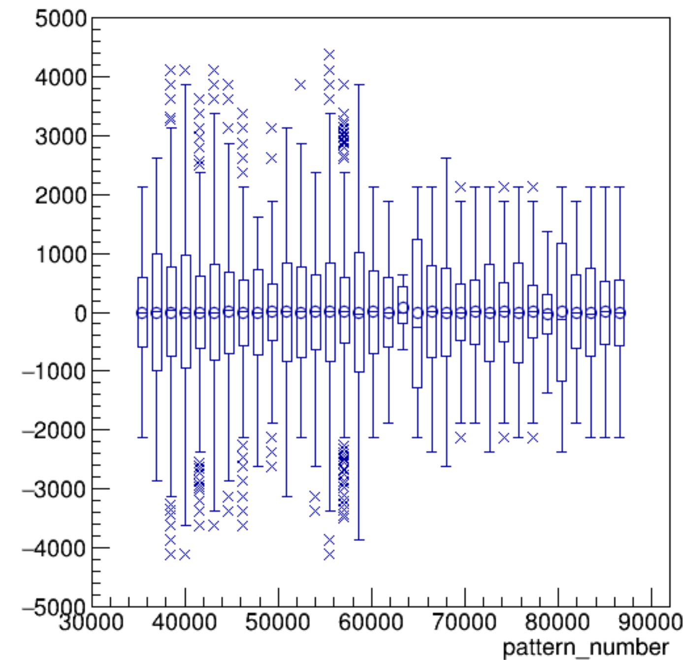
asym_bcm_an_ds/ppm:pattern_number {ErrorFlag==0}
