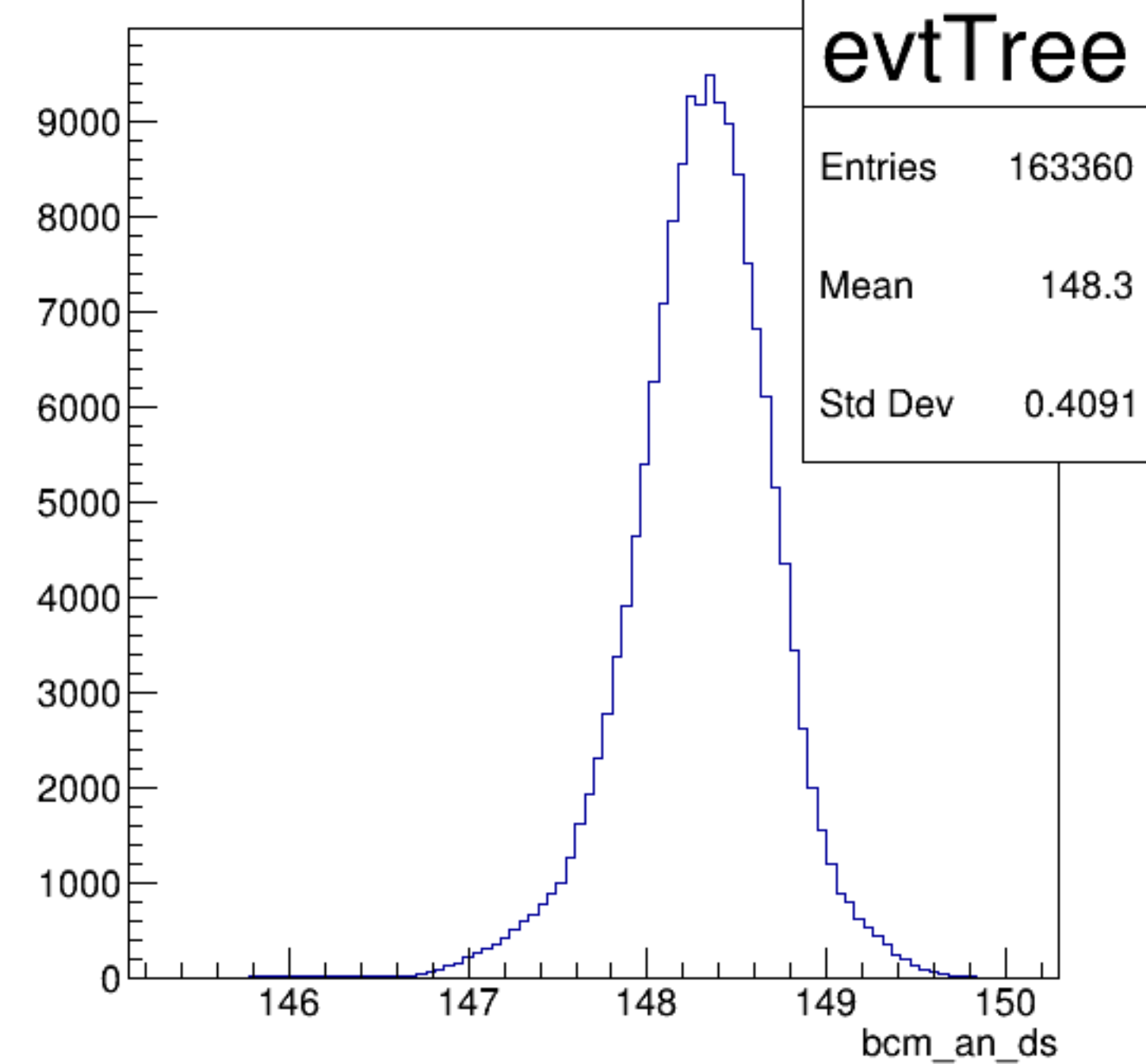
bcm_an_ds {ErrorFlag==0}
