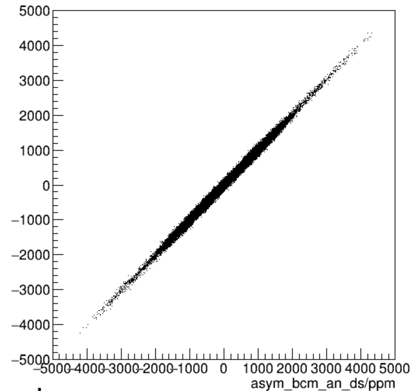
run6440_000_asym_bcm_dg_us_vs_asym_bcm_an_ds_pr.png
