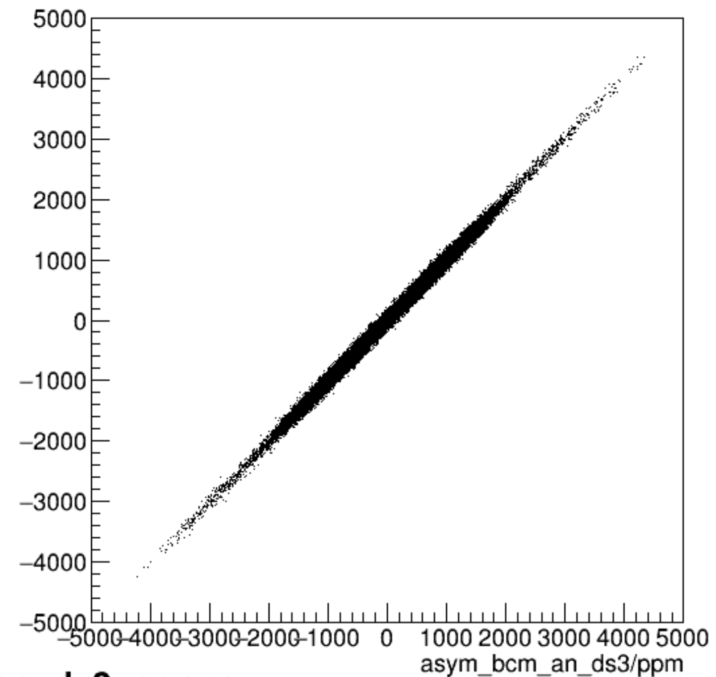
run6440_000_asym_bcm_dg_us_vs_asym_bcm_an_ds3_pr.png
