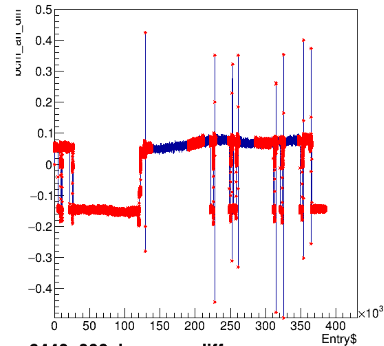
bcm_an_diff:Entry$
