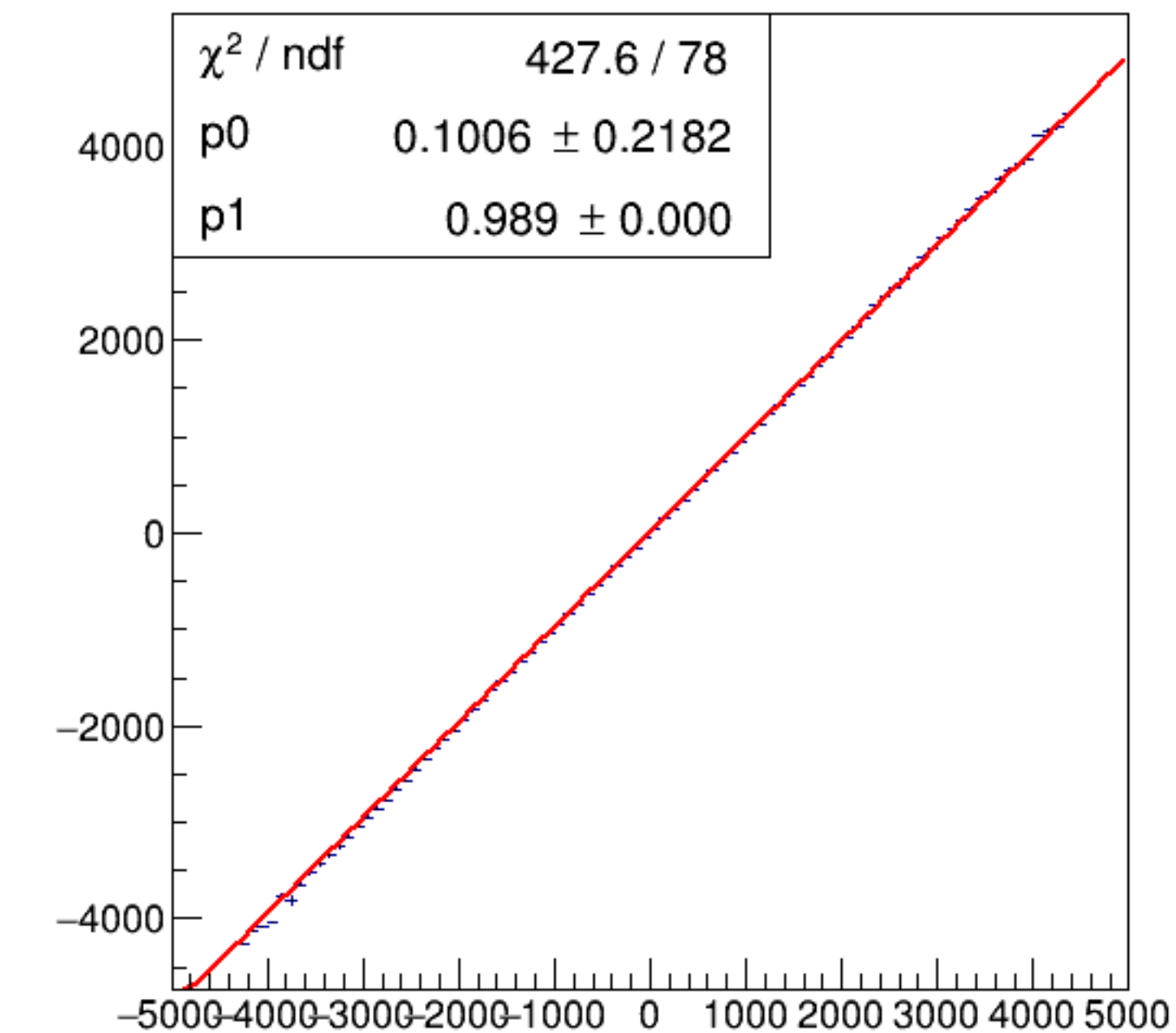
run6440_000_asym_bcm_dg_ds_vs_asym_bcm_an_us_pr.png
