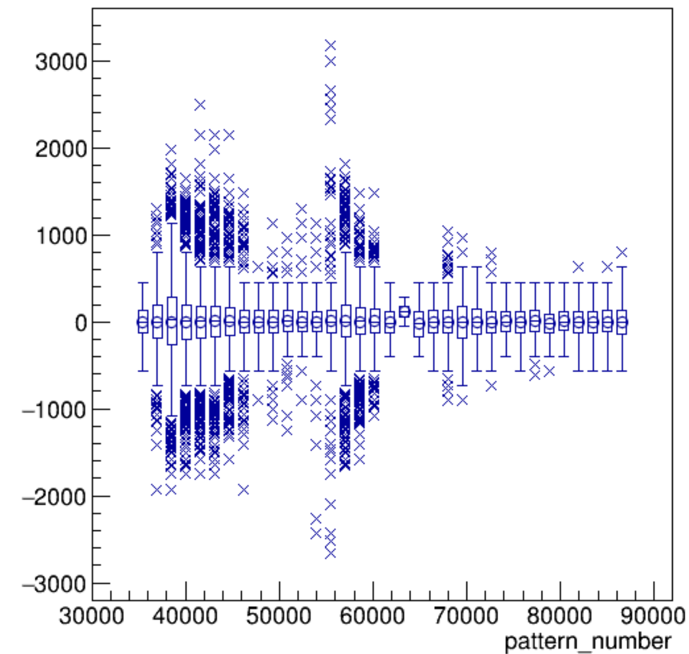
asym_bcm_an_ds3/ppm:pattern_number {ErrorFlag==0}
