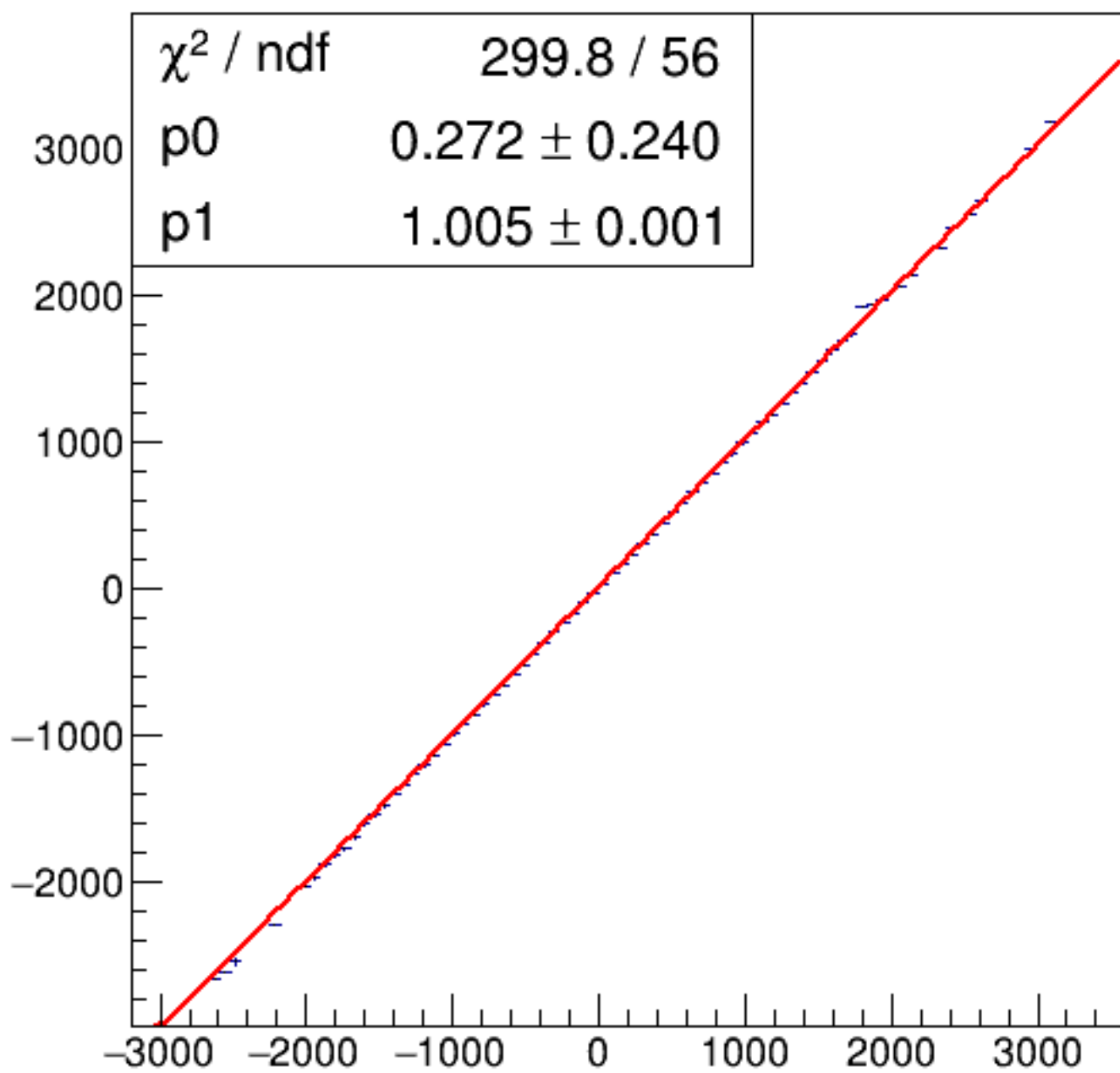
run6440_000_asym_bcm_dg_us_vs_asym_bcm_an_ds_mul.png
