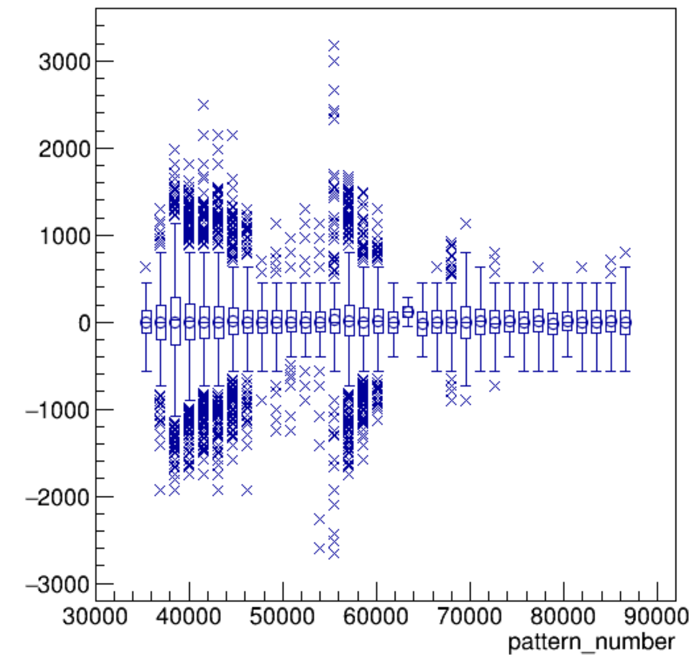
asym_bcm_dg_us/ppm:pattern_number {ErrorFlag==0}
