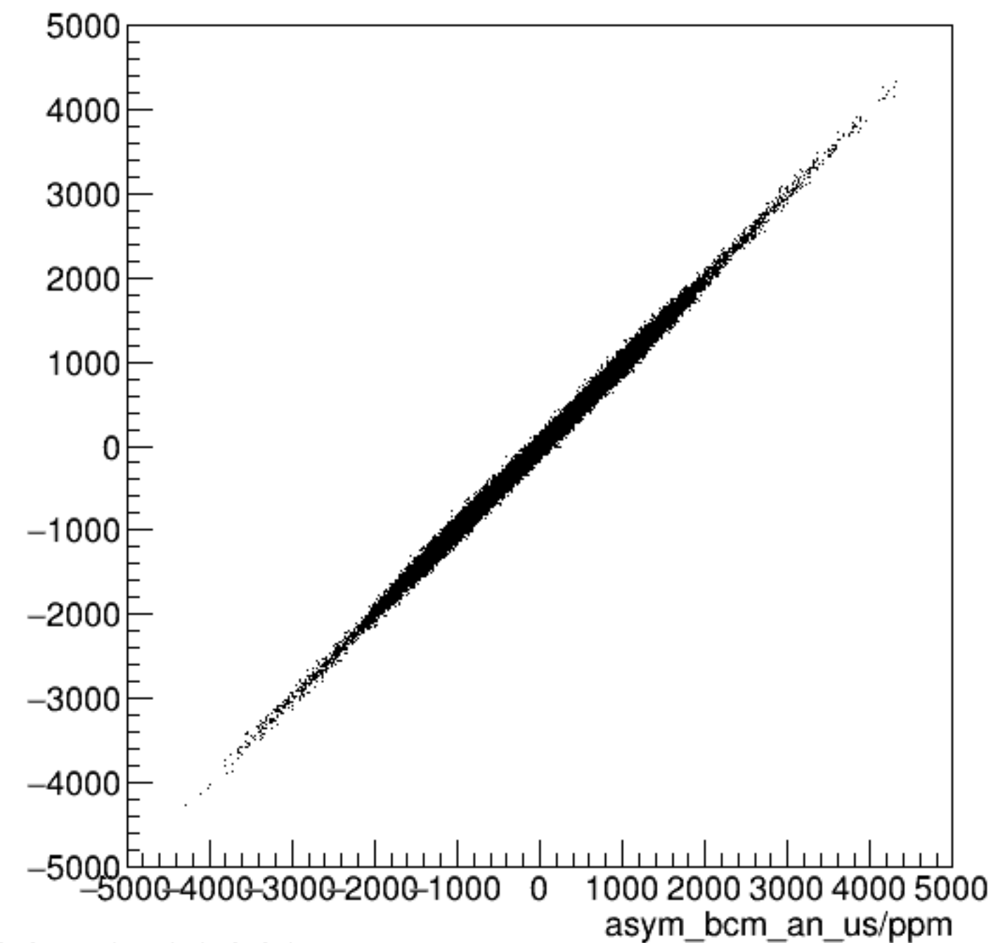
run6440_000_asym_bcm_dg_ds_vs_asym_bcm_an_us_pr.png
