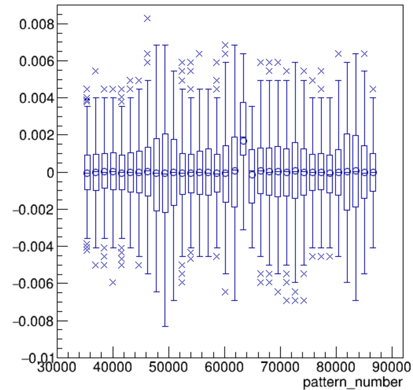
asym_bcm_an_diff*yield_bcm_an_diff:pattern_number {ErrorFlag==0}
