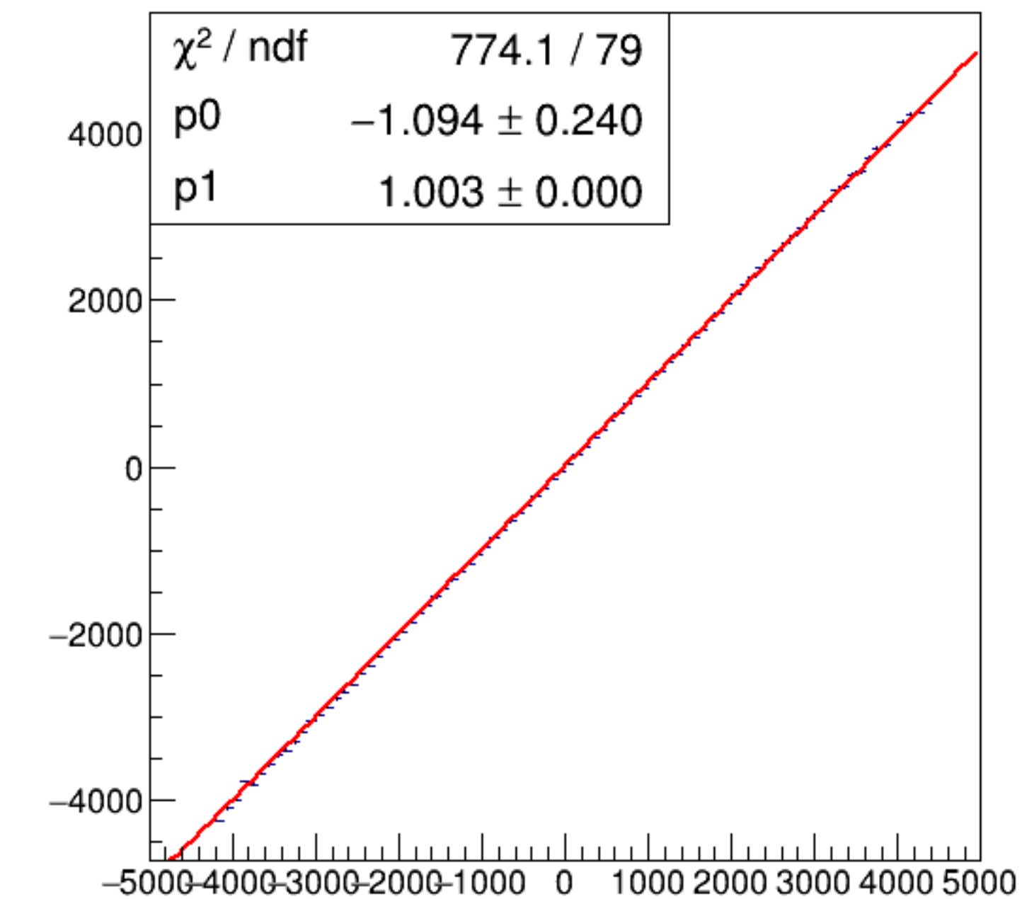
run6440_000_asym_bcm_dg_us_vs_asym_bcm_an_ds_pr.png
