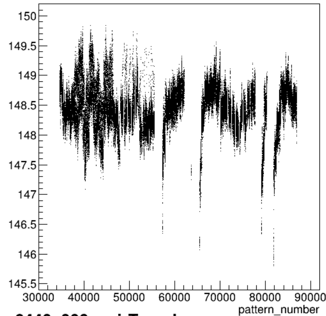
yield_bcm_an_us:pattern_number {ErrorFlag==0}
