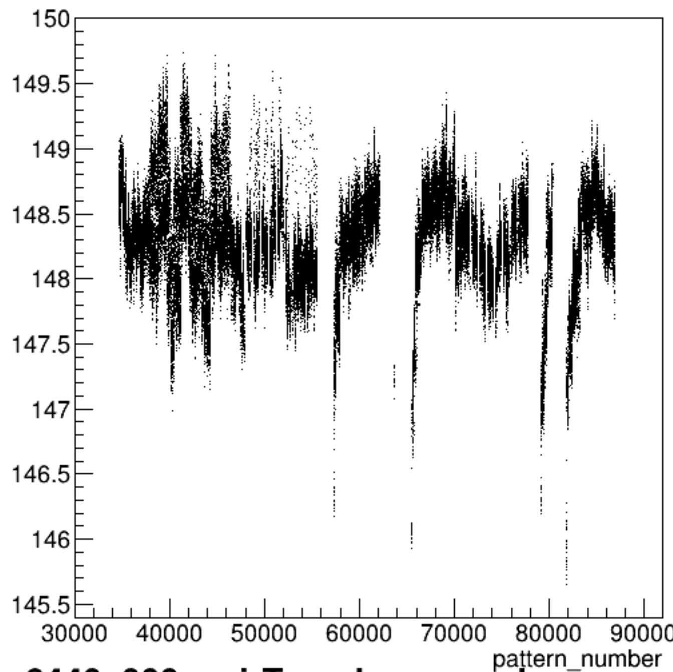
yield_bcm_an_ds:pattern_number {ErrorFlag==0}
