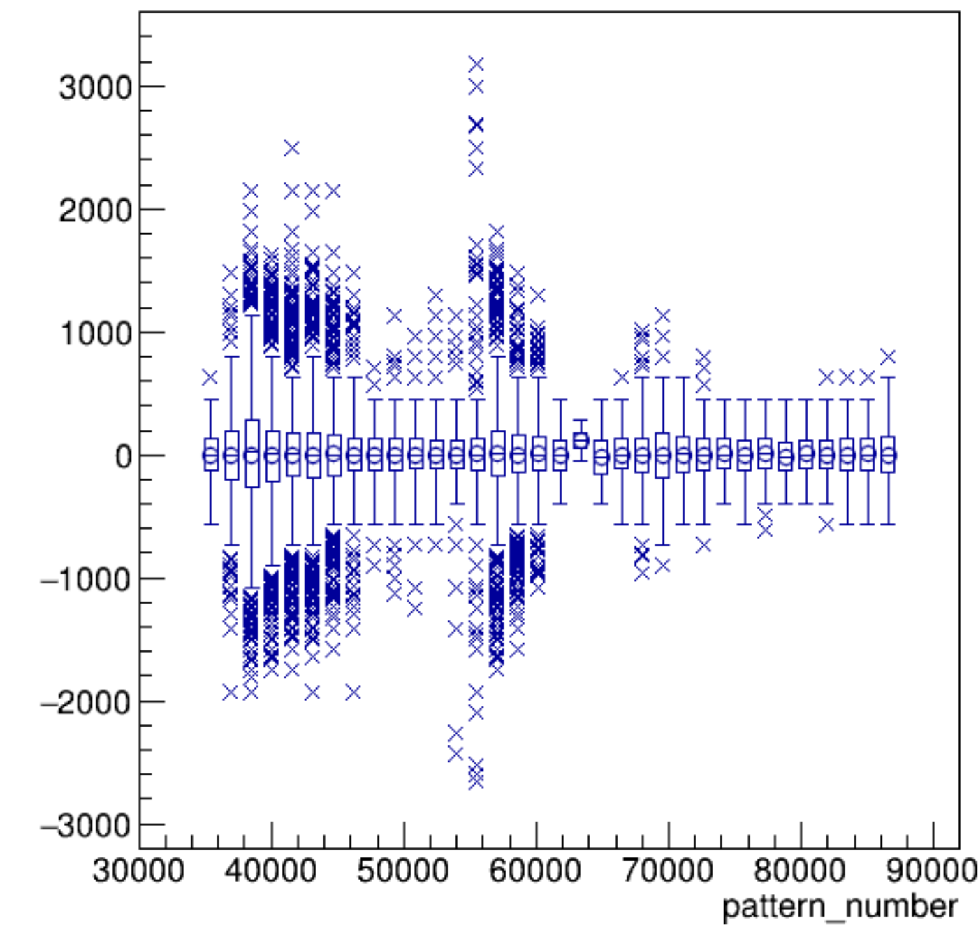
asym_bcm_dg_ds/ppm:pattern_number {ErrorFlag==0}
