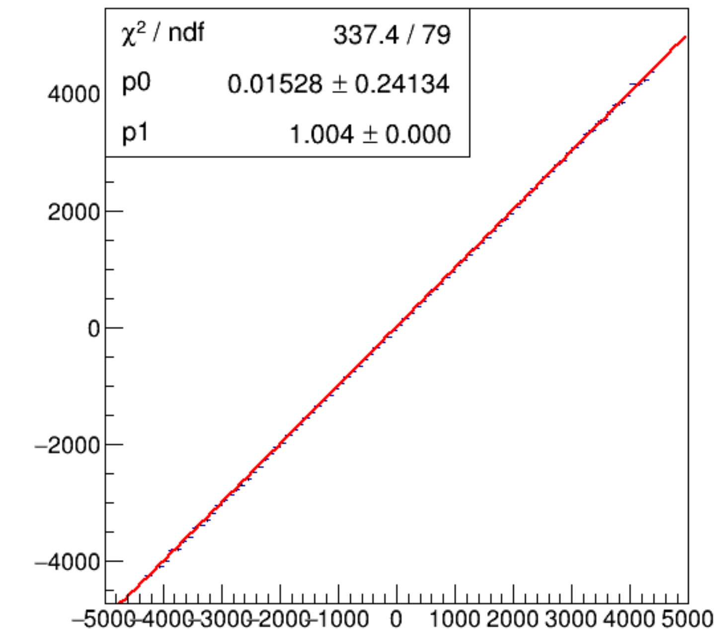
run6440_000_asym_bcm_dg_us_vs_asym_bcm_an_ds3_pr.png
