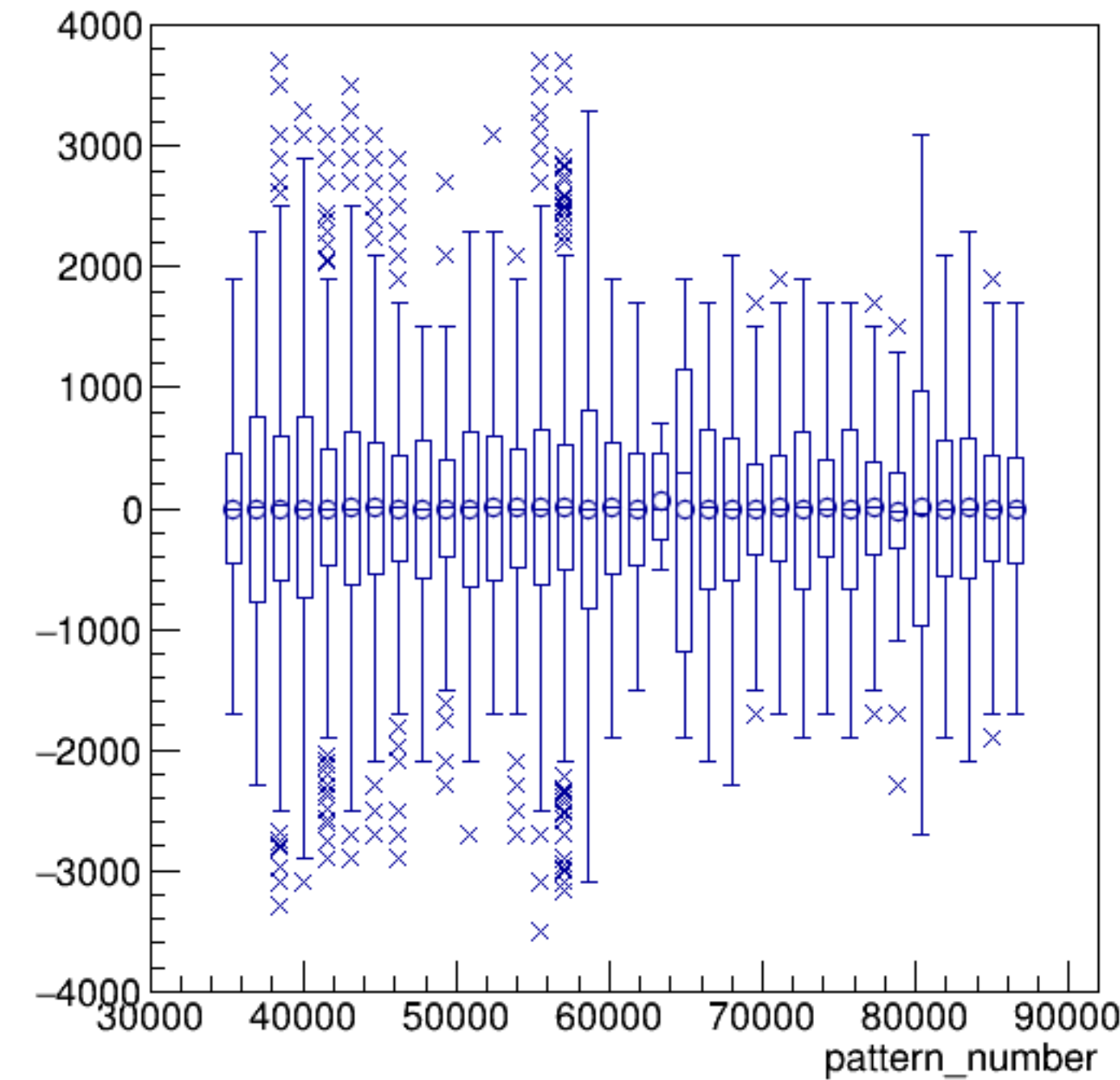
asym_bcm0l02/ppm:pattern_number {ErrorFlag==0}
