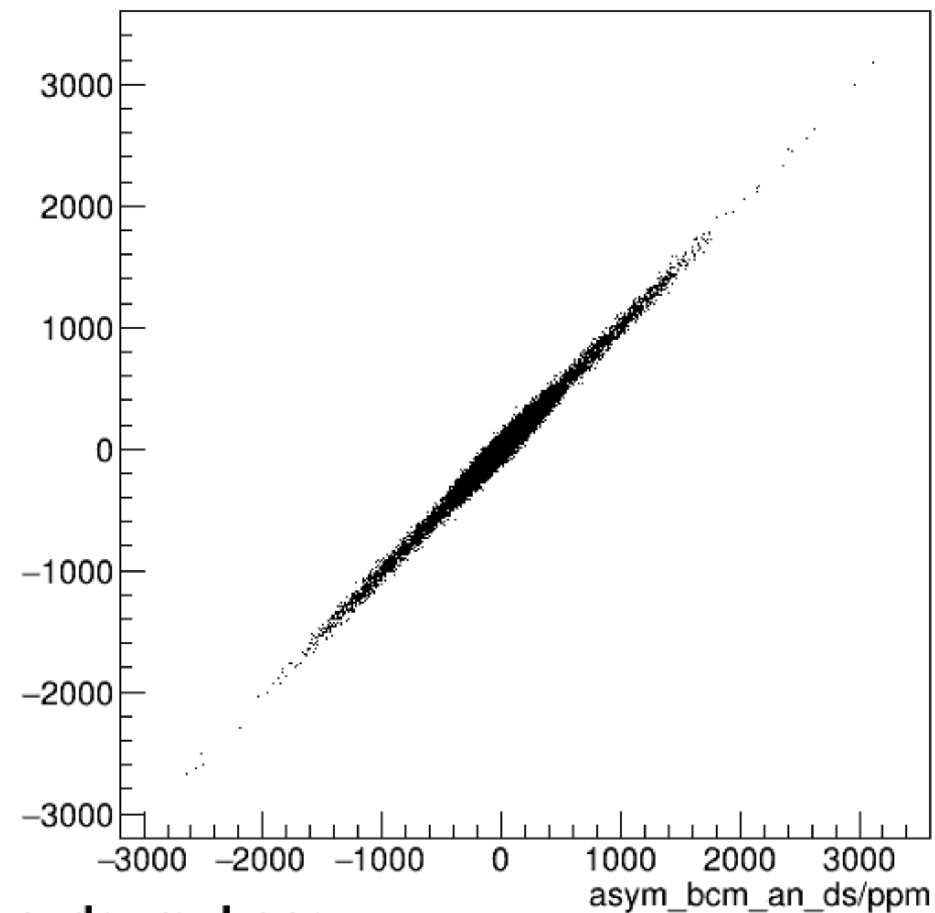
run6440_000_asym_bcm_dg_us_vs_asym_bcm_an_ds_mul.png
