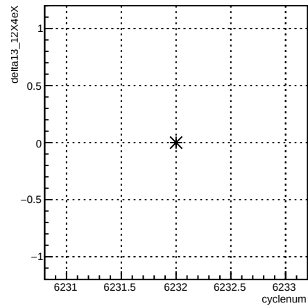
segment:cyclenum {run == 6441}
