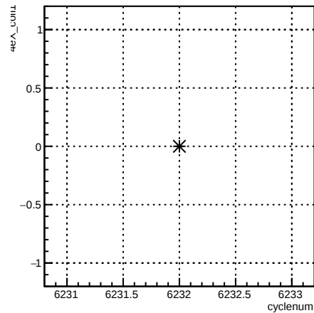
4eX_coil1:cyclenum {run == 6441}
