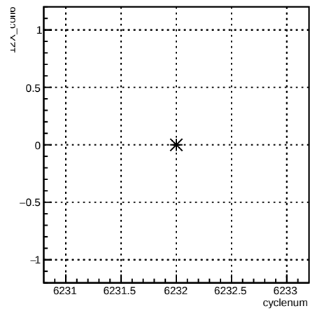
12X_coil6:cyclenum {run == 6441}
