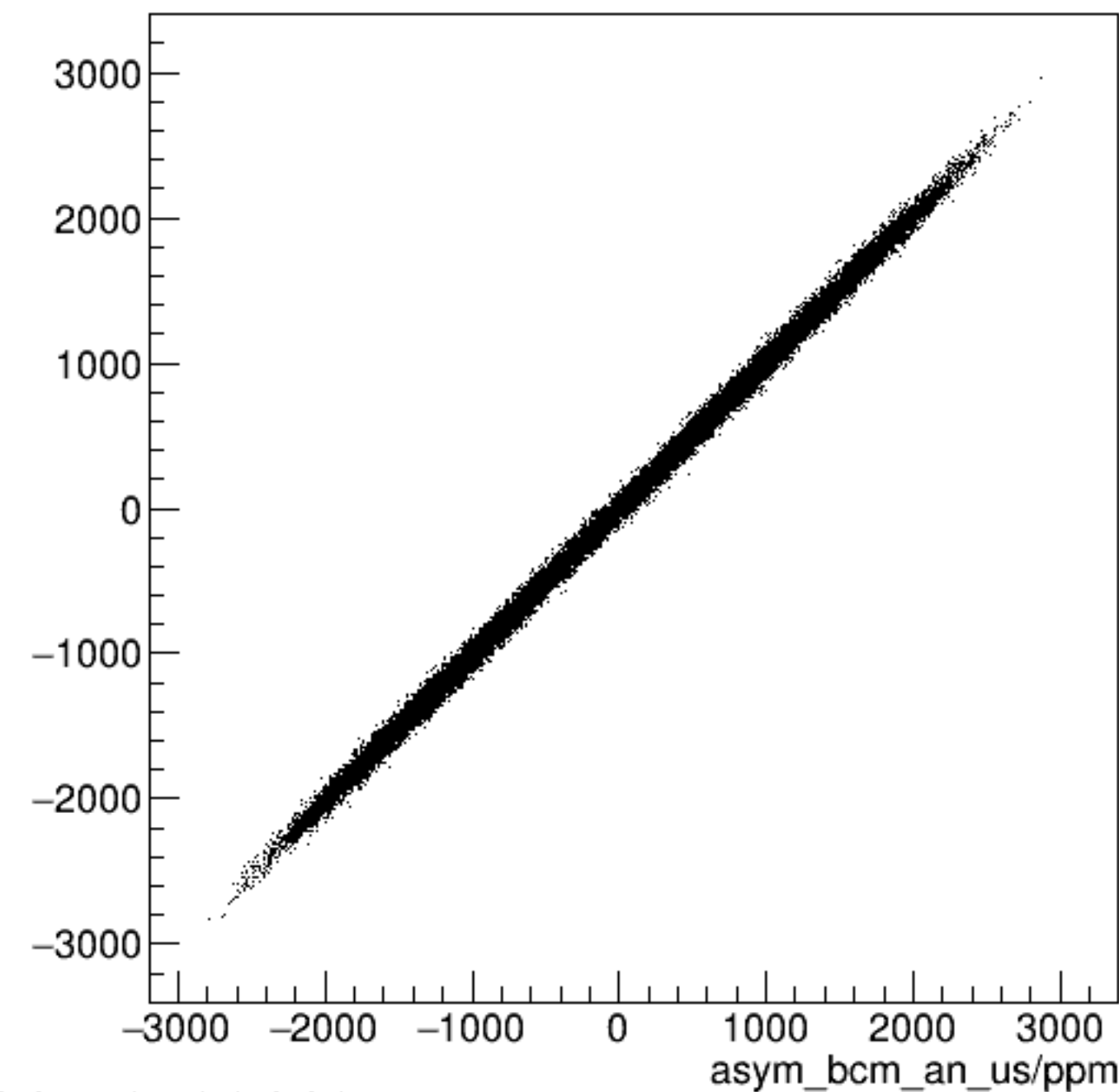
run6444_000_asym_bcm_dg_ds_vs_asym_bcm_an_us_pr.png
