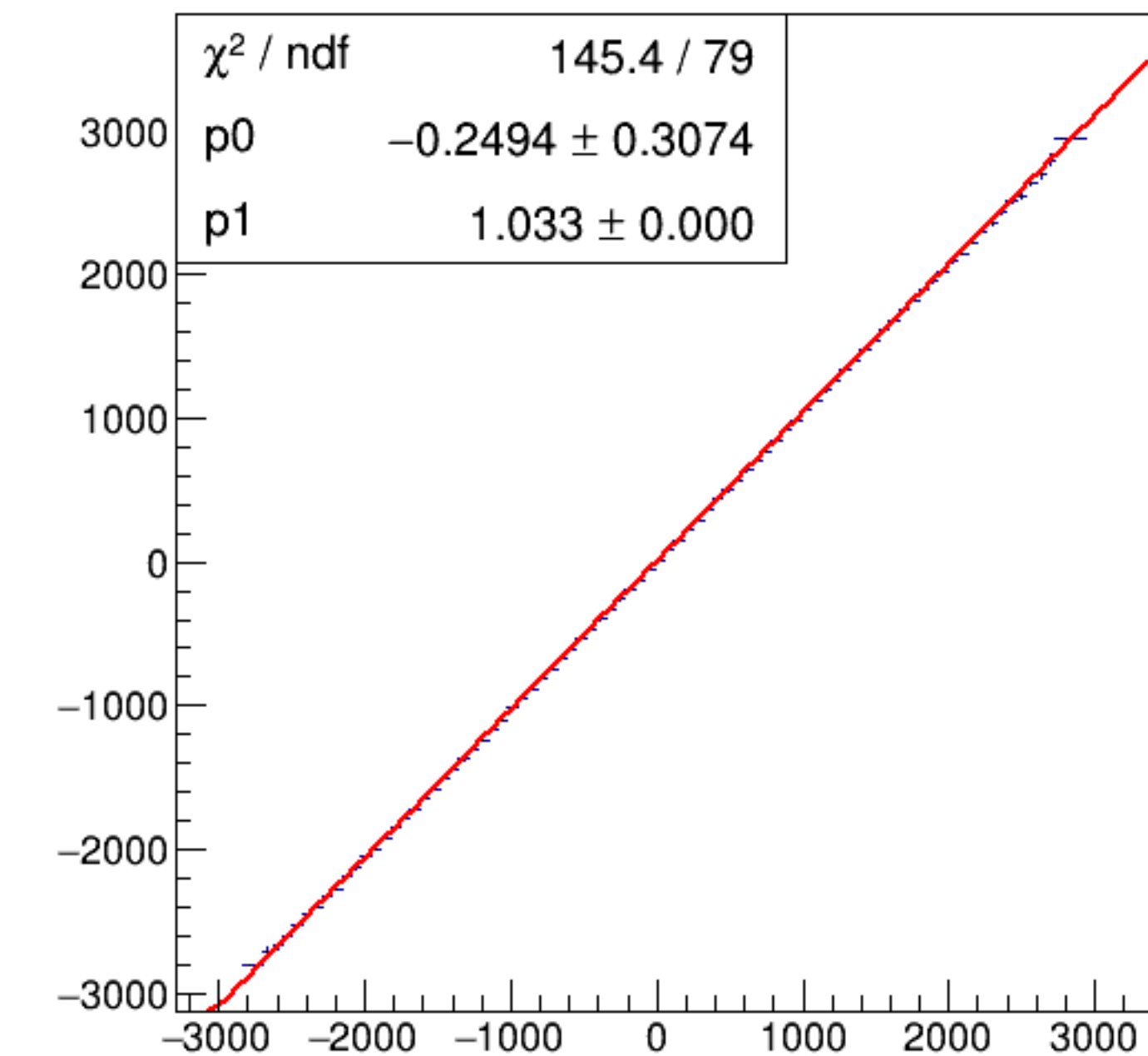
run6444_000_asym_bcm_dg_us_vs_asym_bcm_an_ds_pr.png
