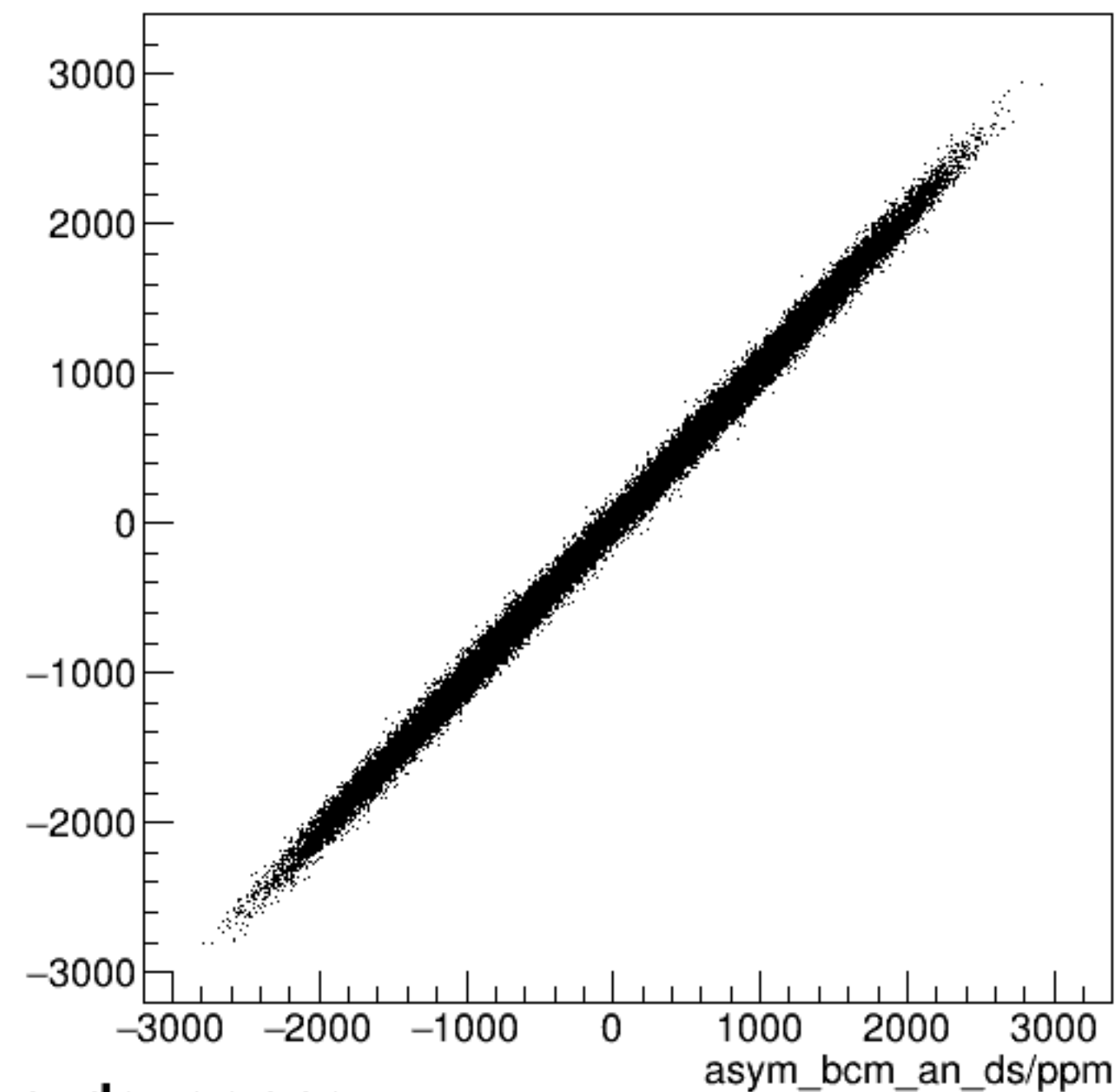
run6444_000_asym_bcm_dg_us_vs_asym_bcm_an_ds_pr.png
