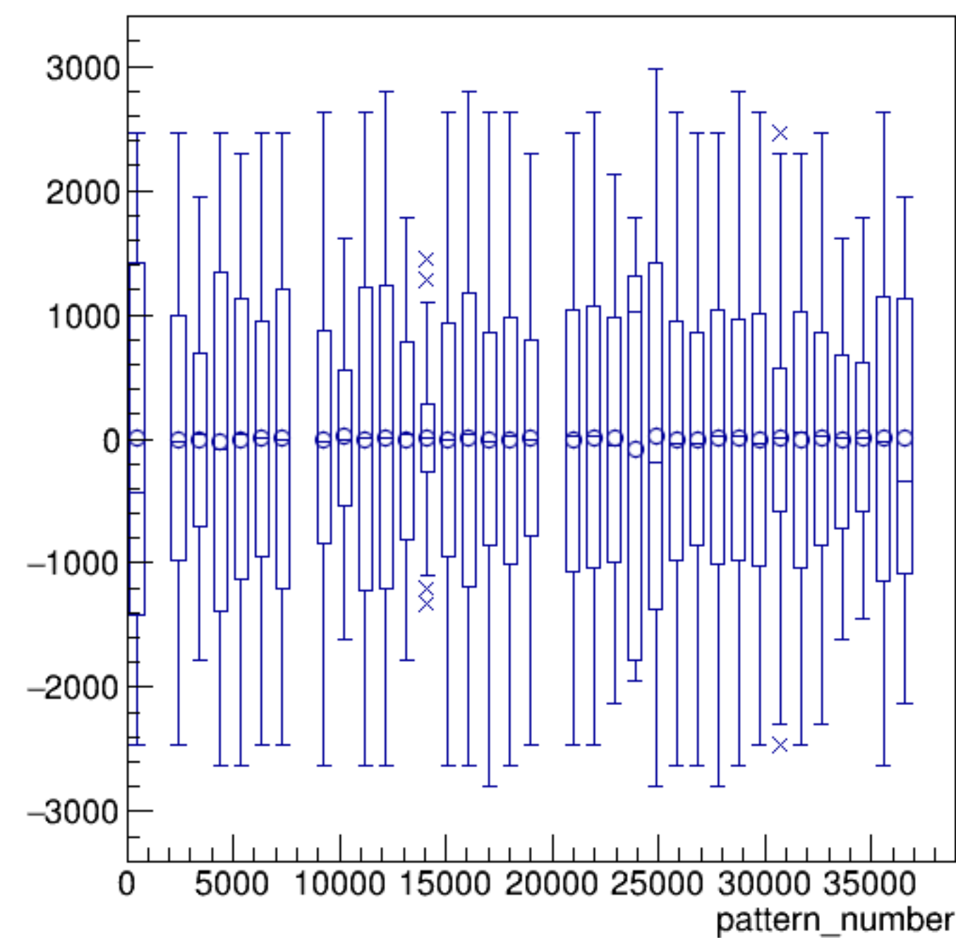
asym_bcm_dg_ds/ppm:pattern_number {ErrorFlag==0}
