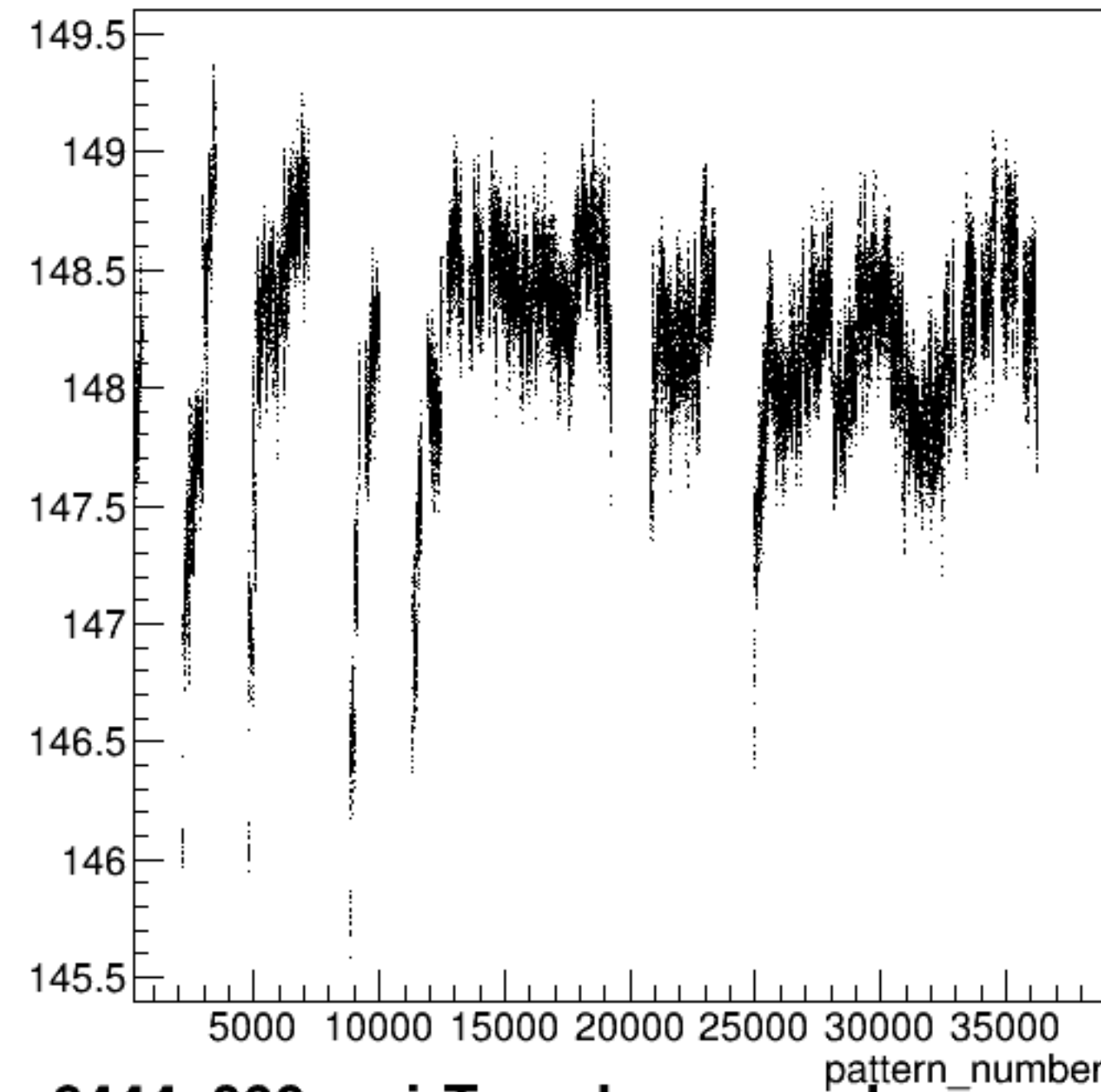
yield_bcm_an_ds:pattern_number {ErrorFlag==0}
