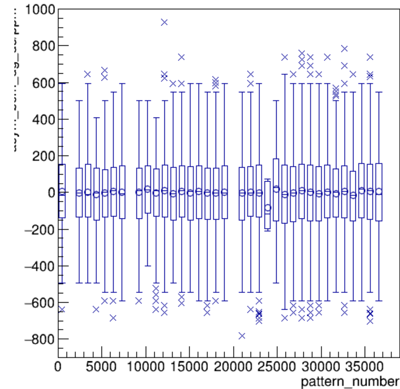
asym_bcm_dg_ds/ppm:pattern_number {ErrorFlag==0}
