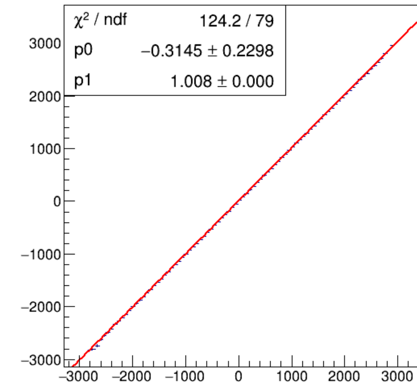
run6444_000_asym_bcm_dg_ds_vs_asym_bcm_an_us_pr.png
