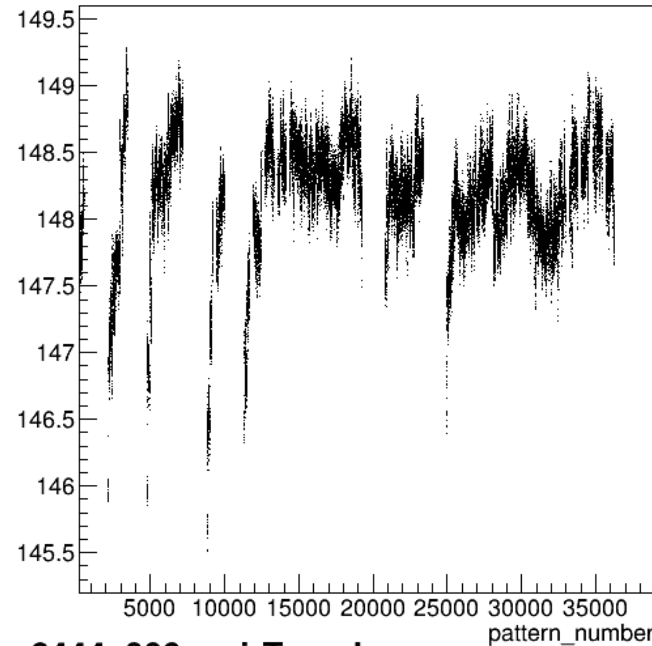
yield_bcm_an_us:pattern_number {ErrorFlag==0}
