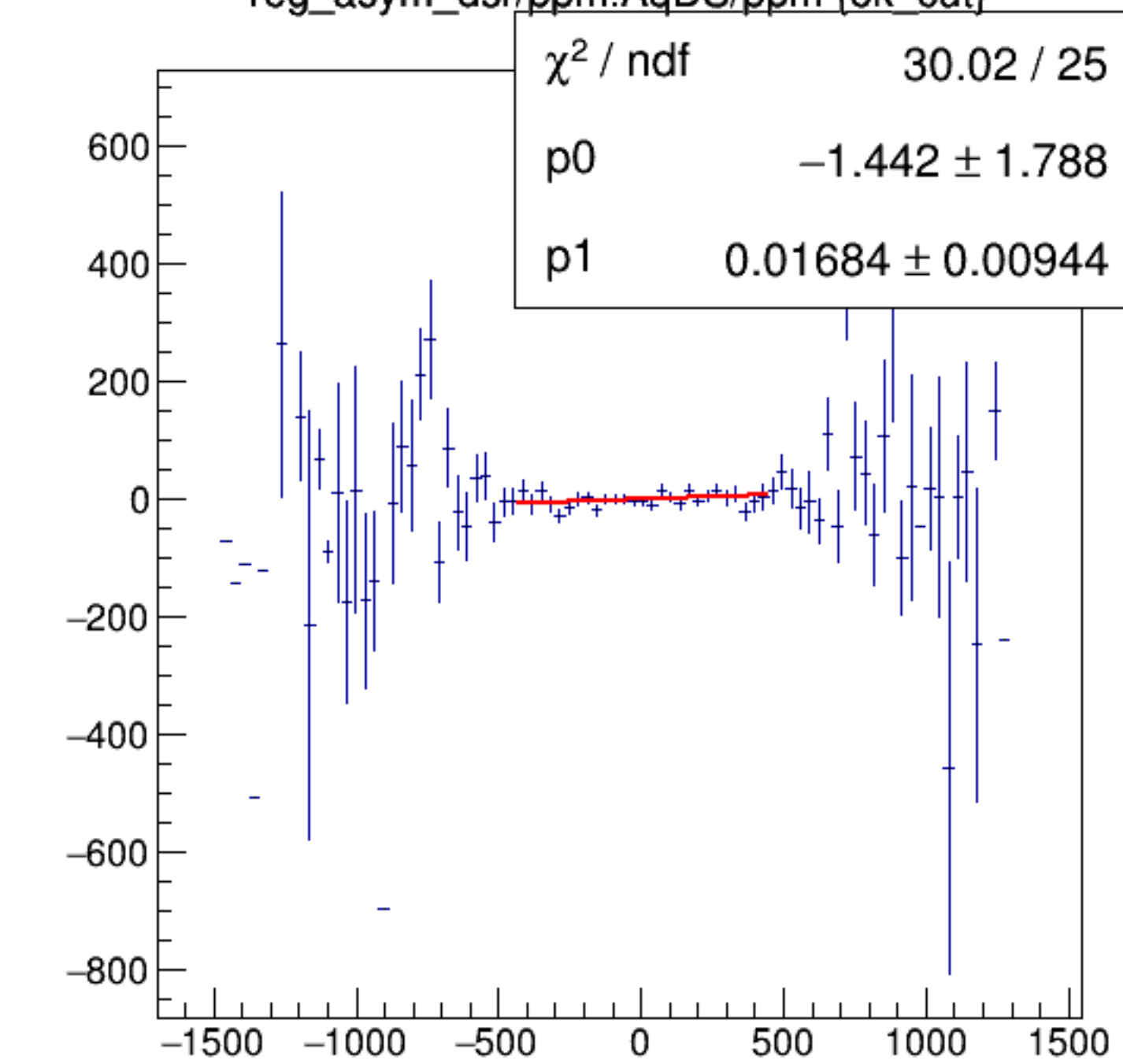
reg_asym_dsr/ppm:AqDS/ppm {ok_cut}
