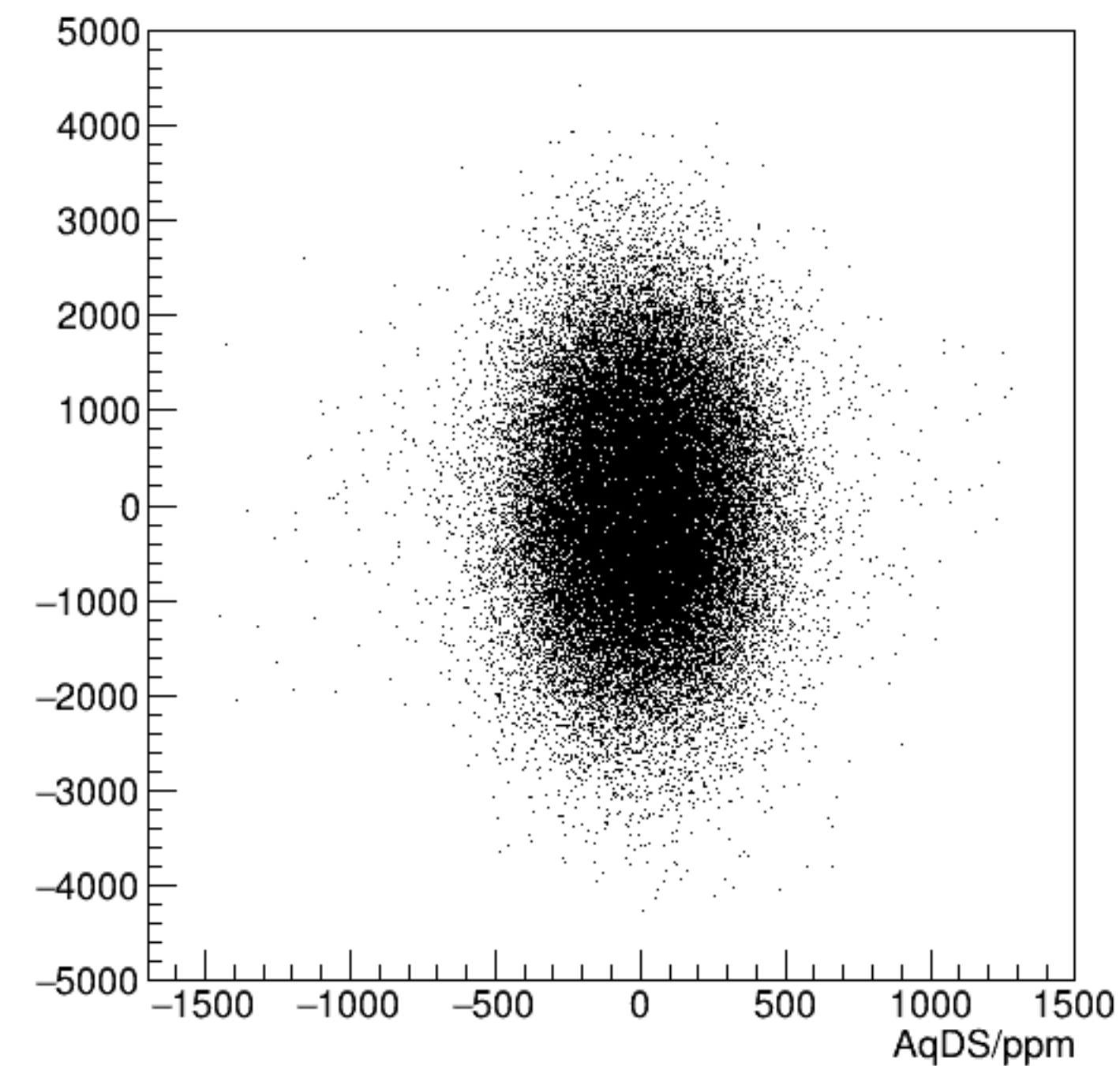
reg_asym_usr/ppm:AqDS/ppm {ok_cut}
