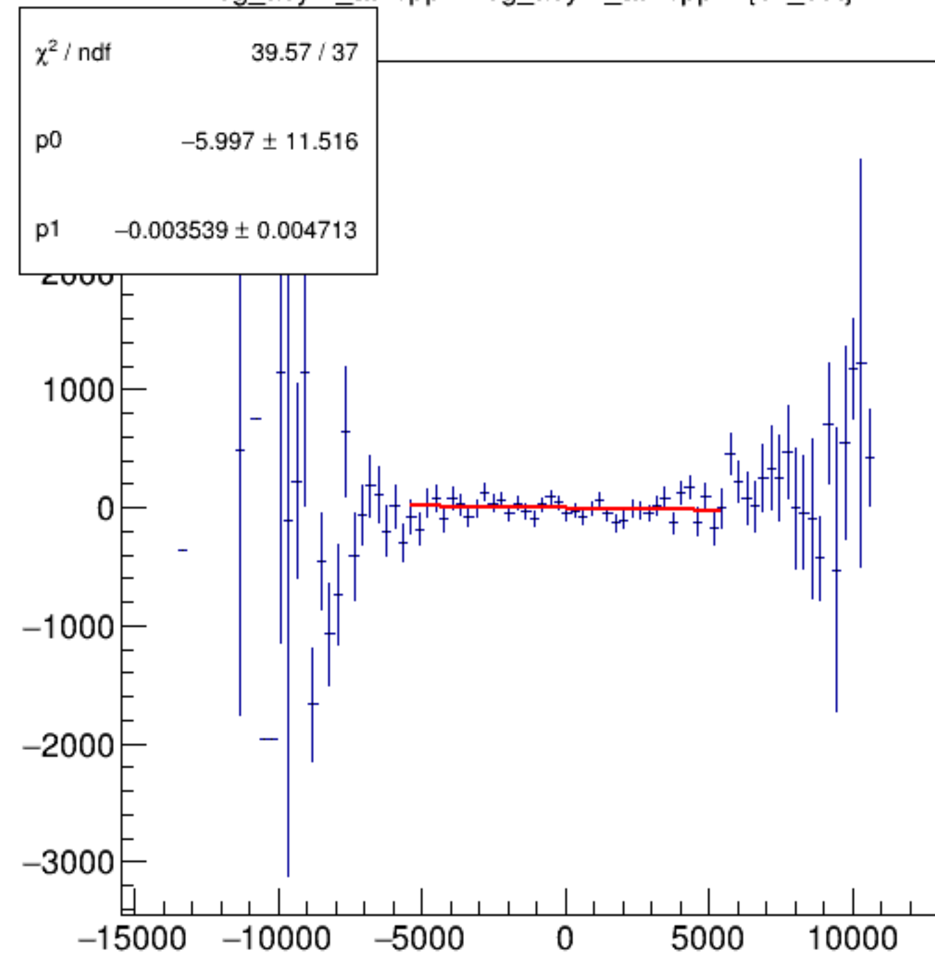
reg_asym_atl1/ppm:reg_asym_atr1/ppm {ok_cut}
