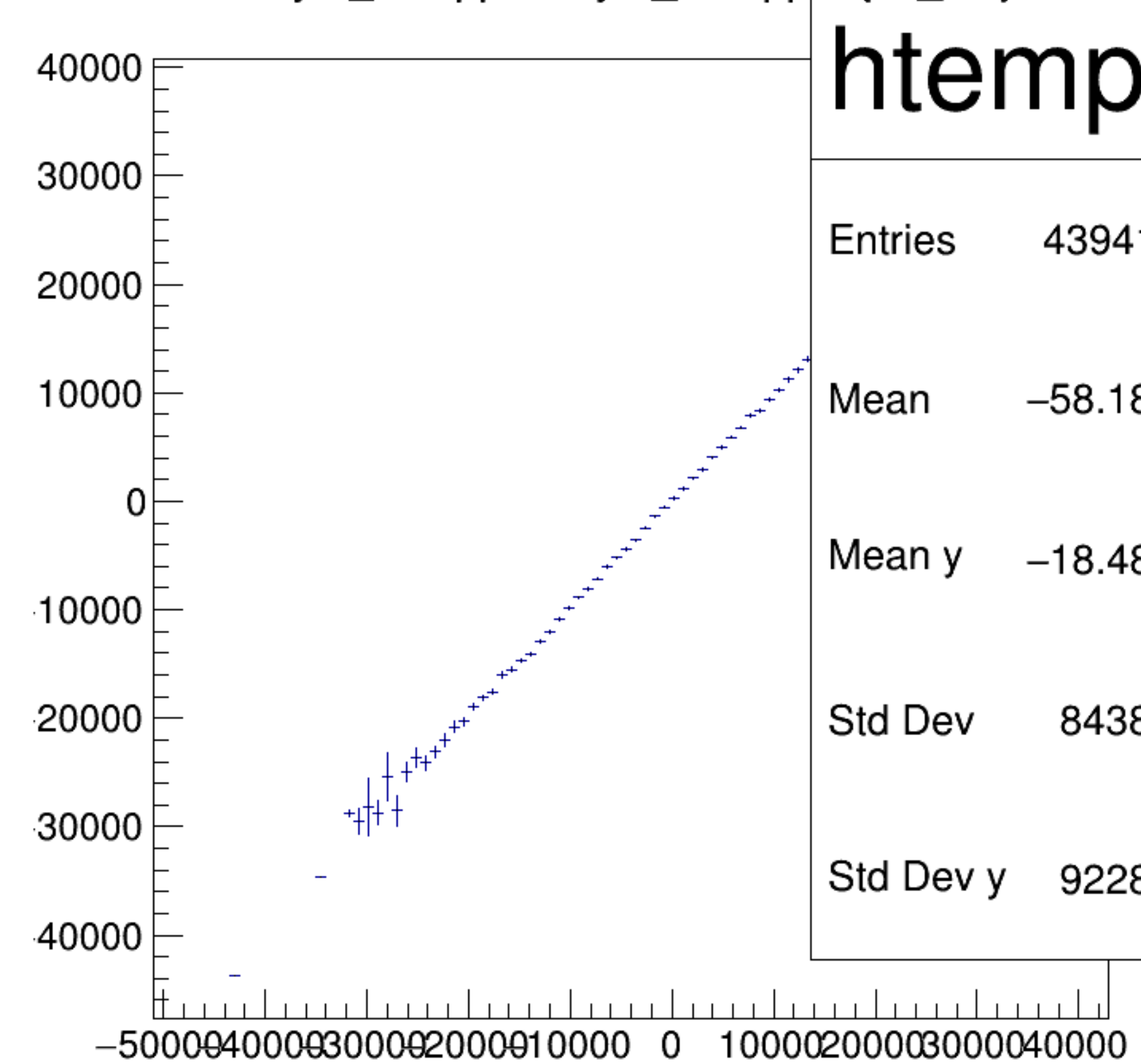
asym_atl2/ppm:asym_atr2/ppm {ok_cut}
