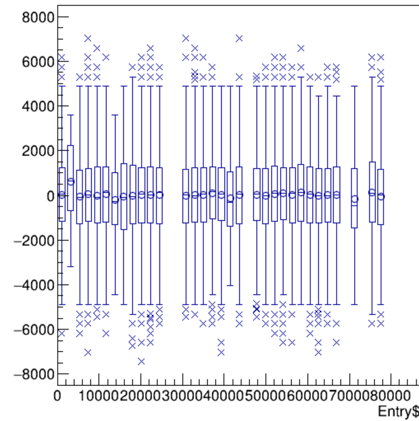
(reg_asym_atl2/ppm-reg_asym_atr2/ppm)/2:Entry$ {ok_cut}
