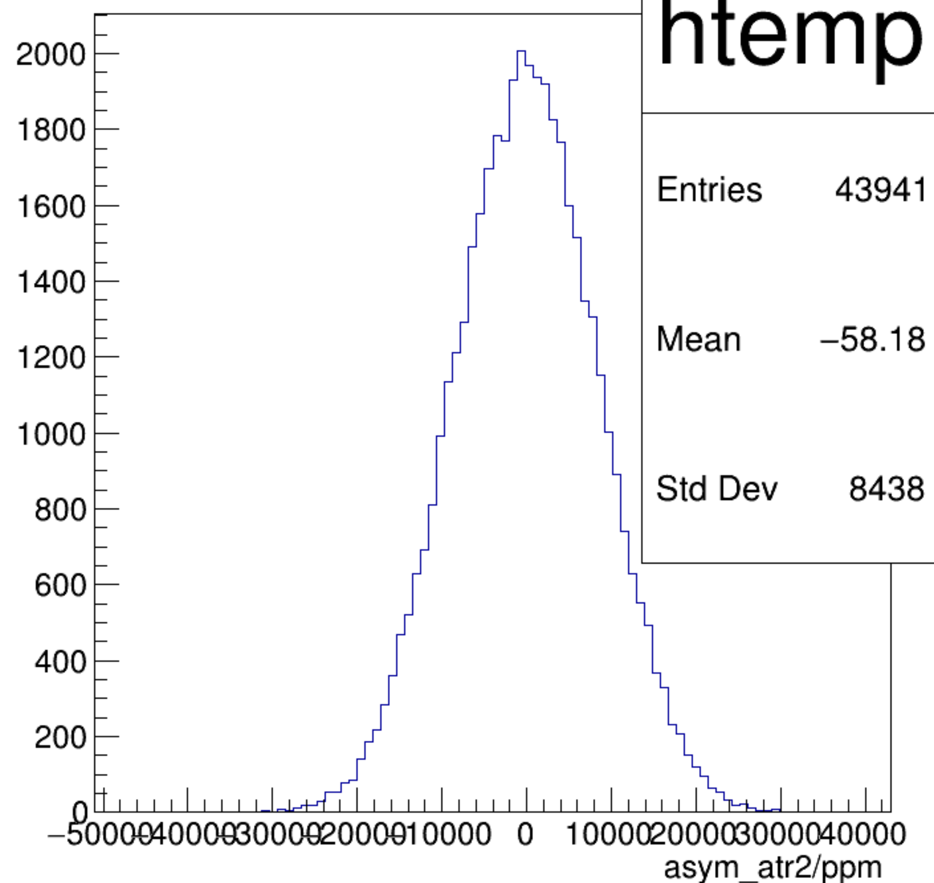
asym_atr2/ppm {ok_cut}
