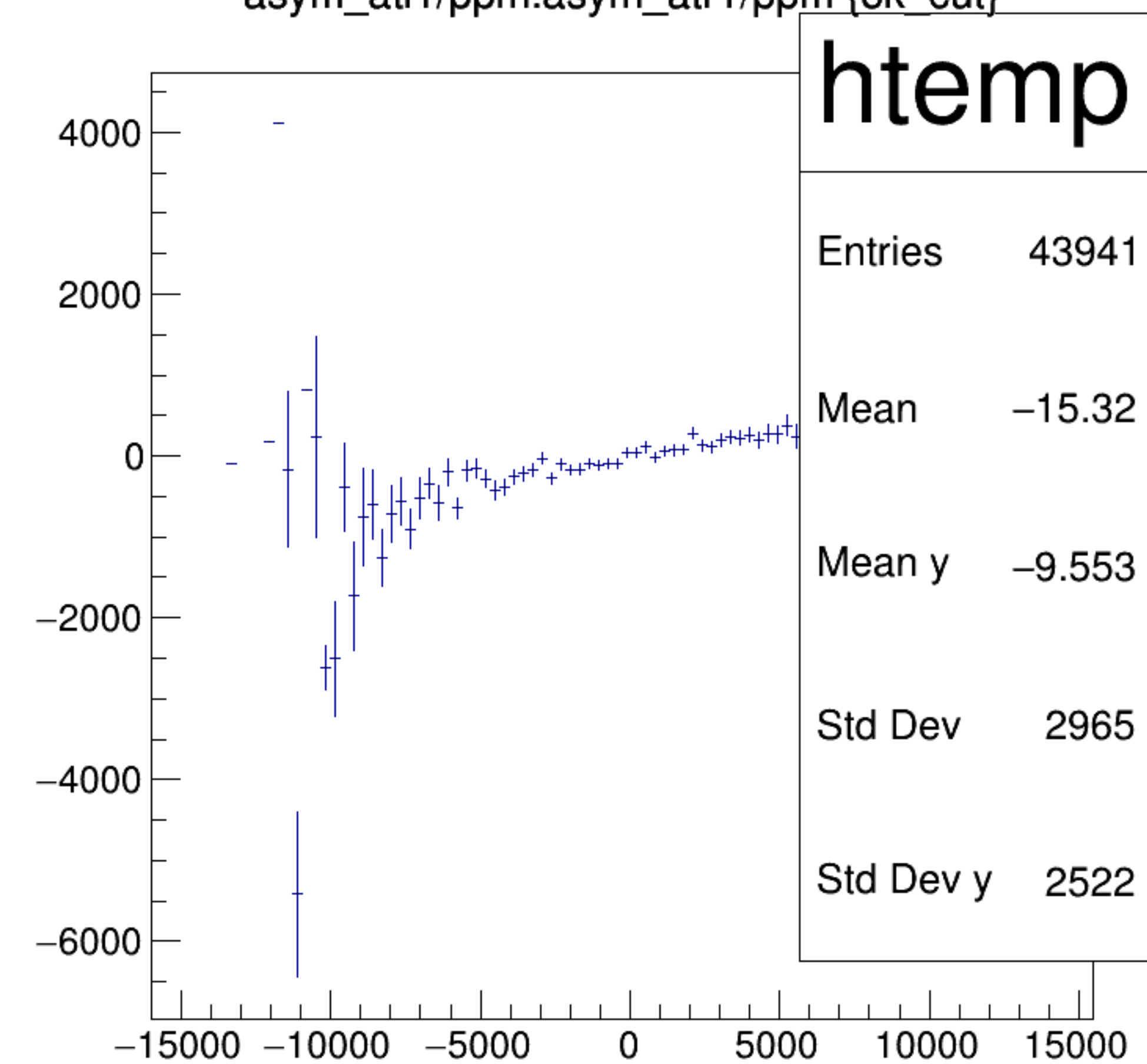
asym_atl1/ppm:asym_atr1/ppm {ok_cut}
