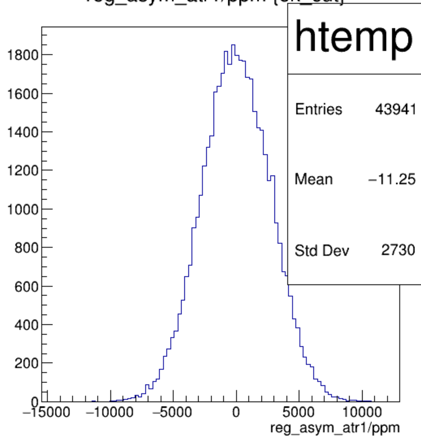
reg_asym_atr1/ppm {ok_cut}
