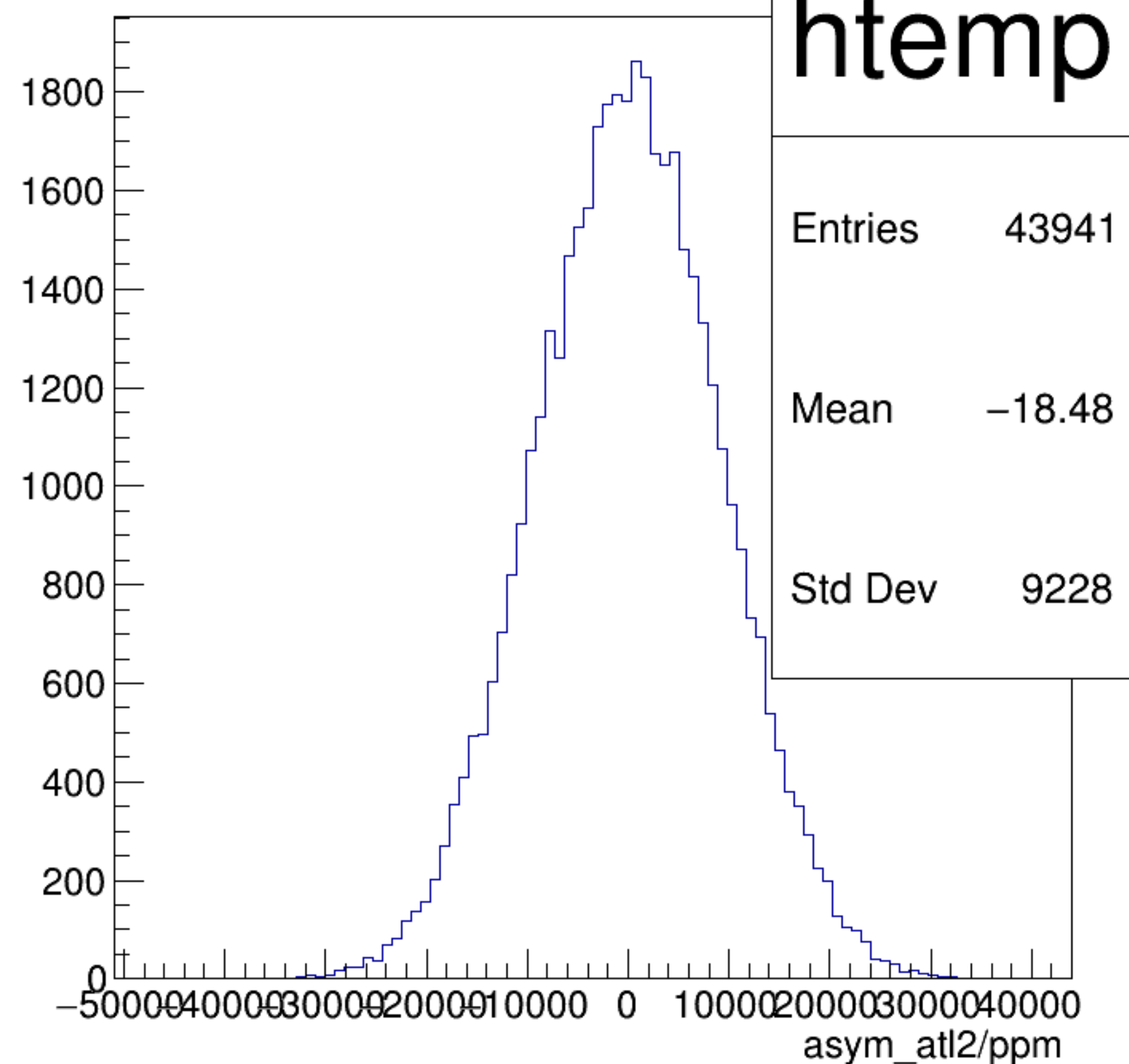
asym_atl2/ppm {ok_cut}
