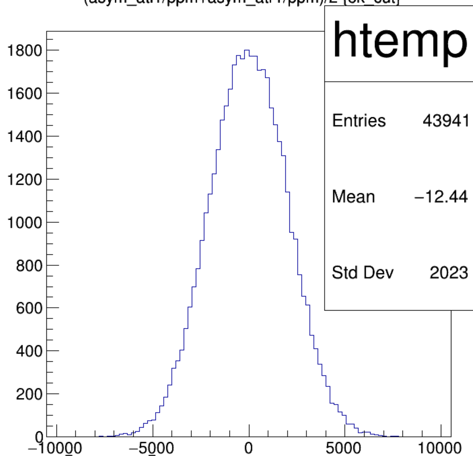
(asym_atl1/ppm+asym_atr1/ppm)/2 {ok_cut}
