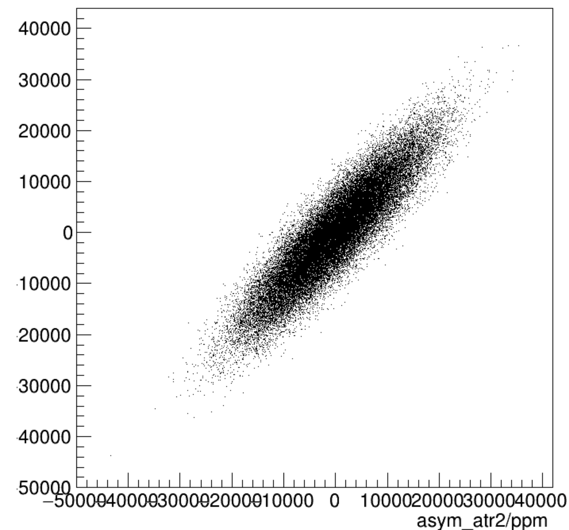
asym_atl2/ppm:asym_atr2/ppm {ok_cut}
