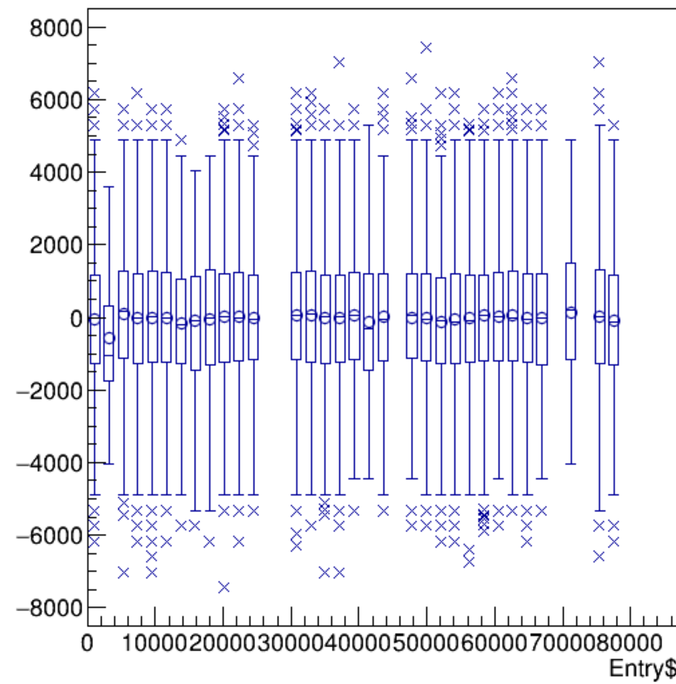
(reg_asym_atl1/ppm+reg_asym_atr1/ppm)/2:Entry$ {ok_cut}
