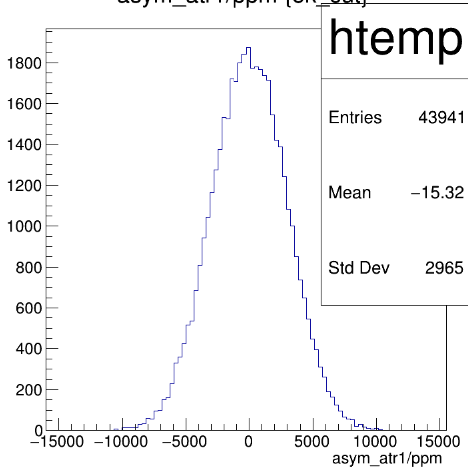
asym_atr1/ppm {ok_cut}
