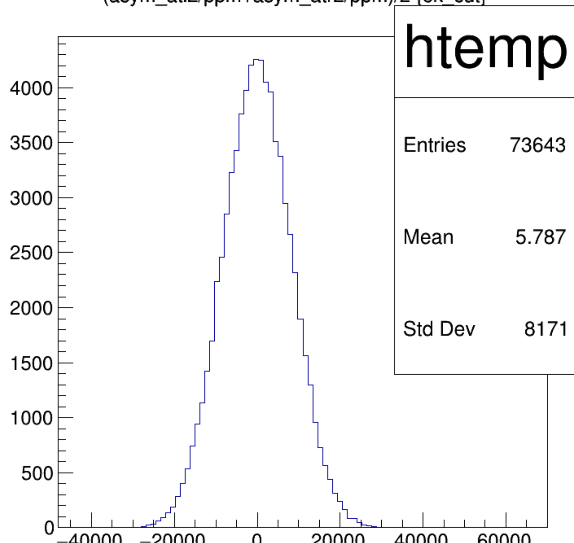
(asym_atl2/ppm+asym_atr2/ppm)/2 {ok_cut}
