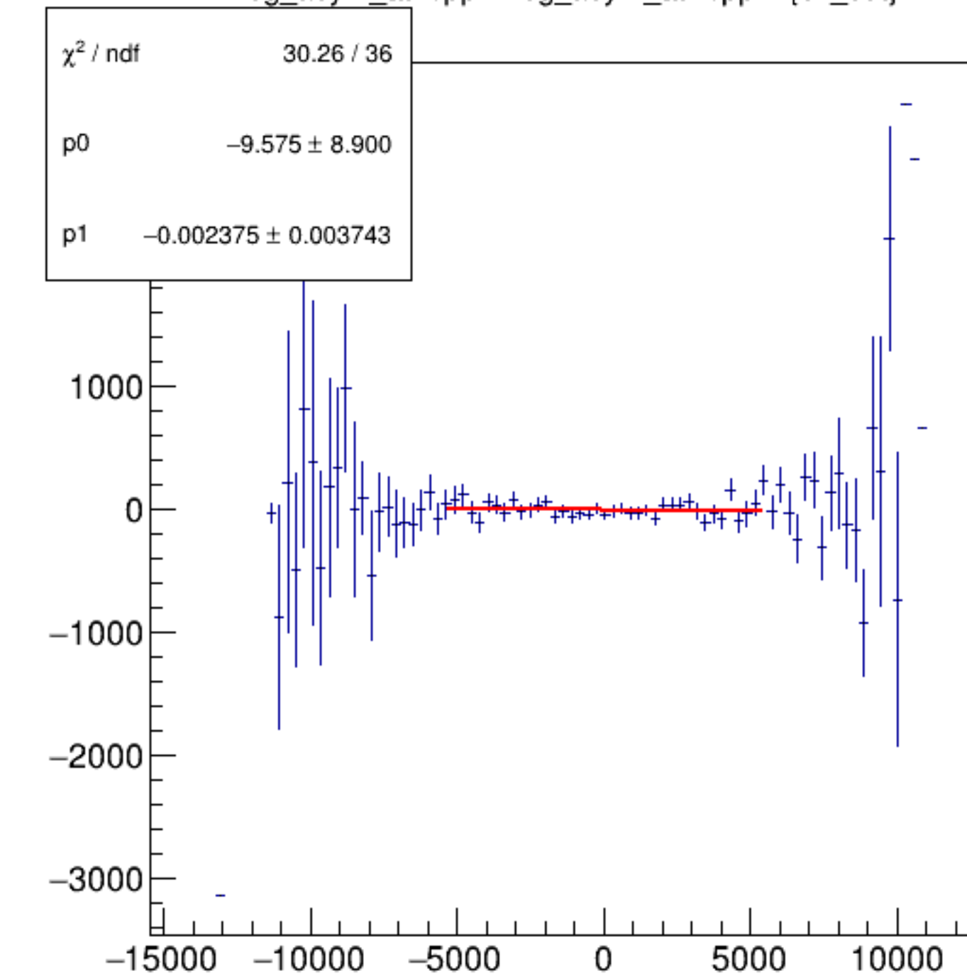
reg_asym_atl1/ppm:reg_asym_atr1/ppm {ok_cut}
