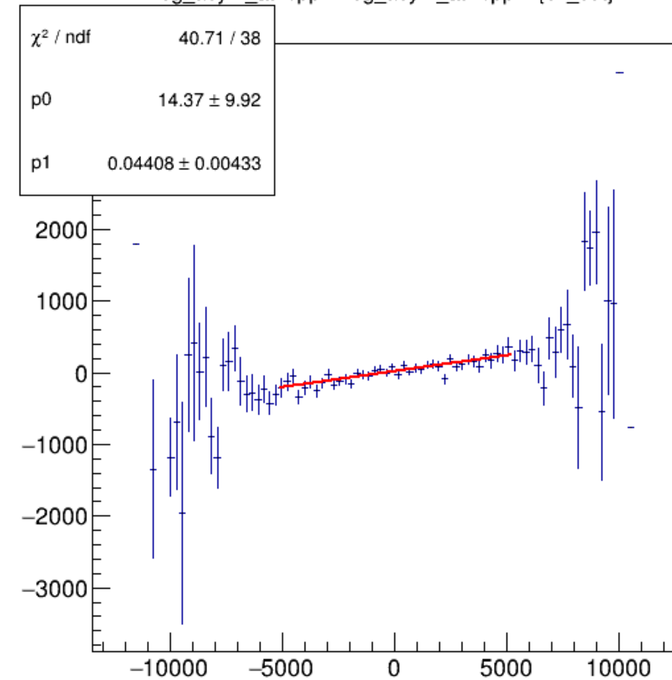
reg_asym_atl2/ppm:reg_asym_atr2/ppm {ok_cut}
