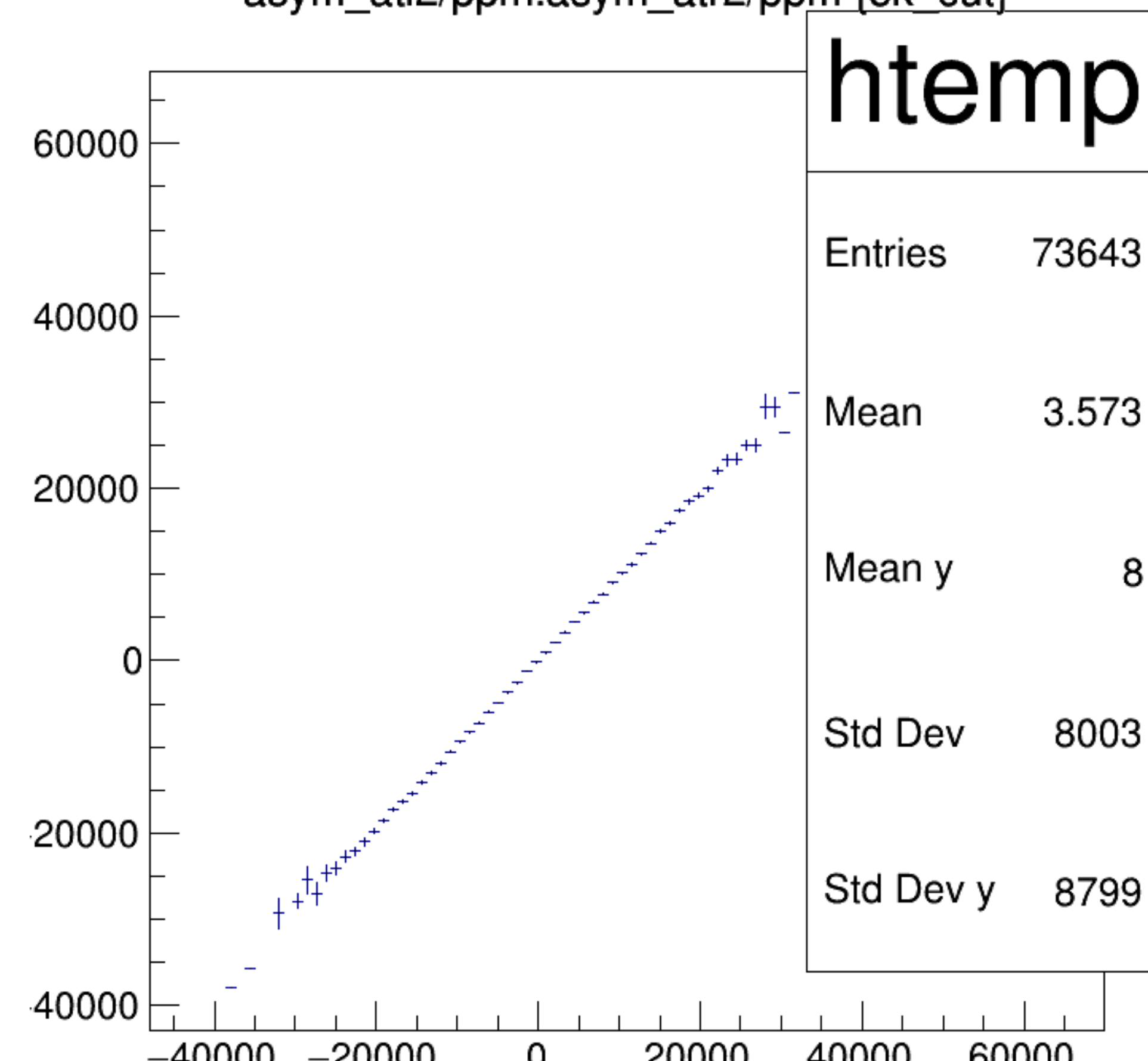
asym_atl2/ppm:asym_atr2/ppm {ok_cut}
