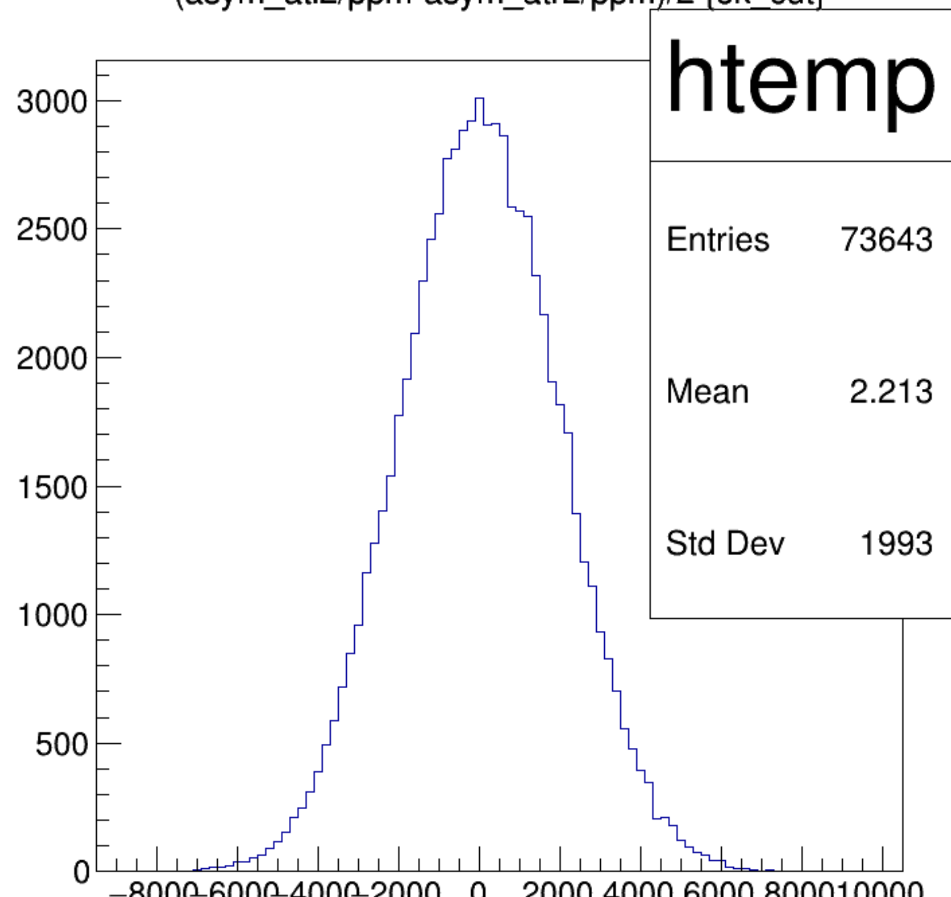
(asym_atl2/ppm-asym_atr2/ppm)/2 {ok_cut}
