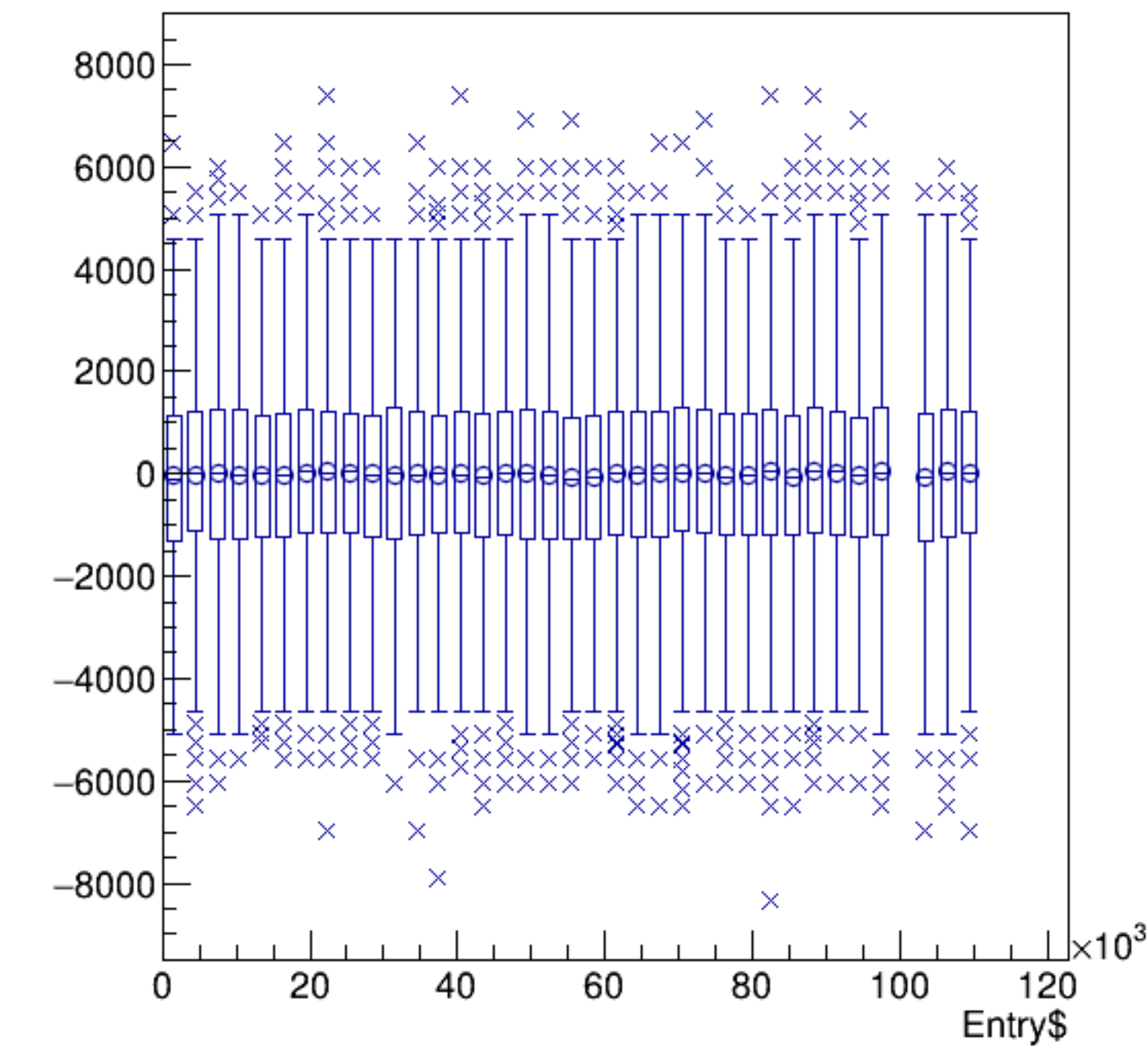
(reg_asym_atl1/ppm+reg_asym_atr1/ppm)/2:Entry$ {ok_cut}
