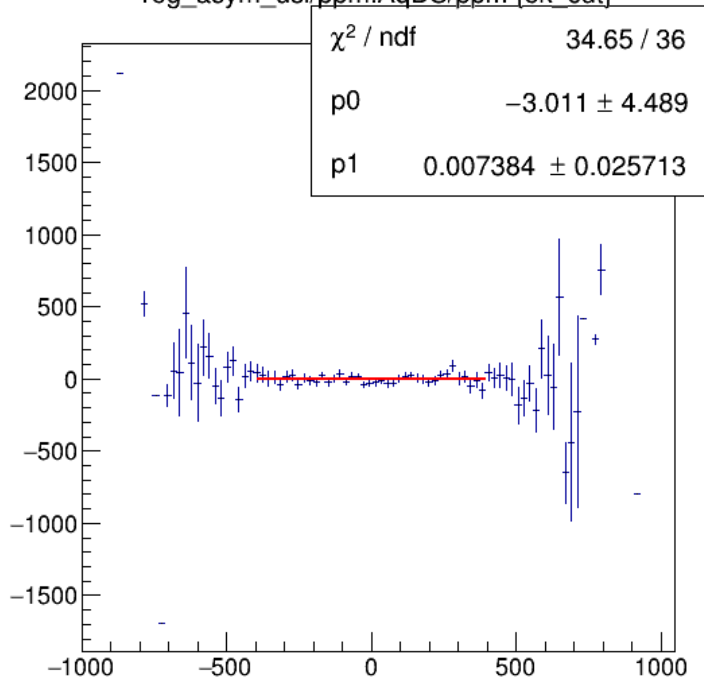
reg_asym_usl/ppm:AqDS/ppm {ok_cut}
