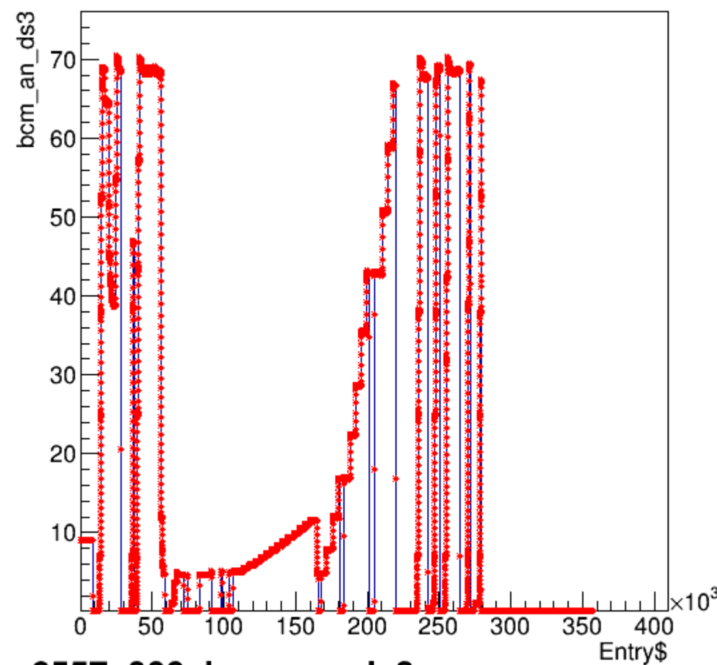
bcm_an_ds3:Entry$
