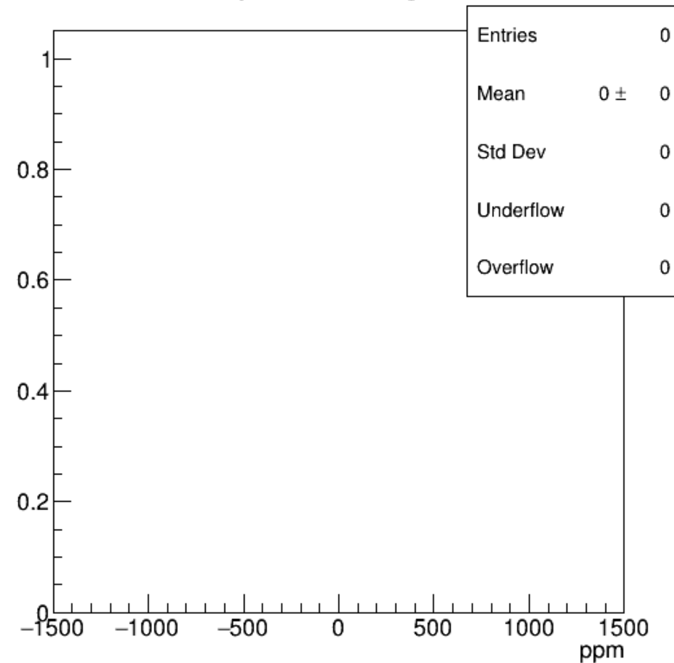
asym_bcm_dg_us
