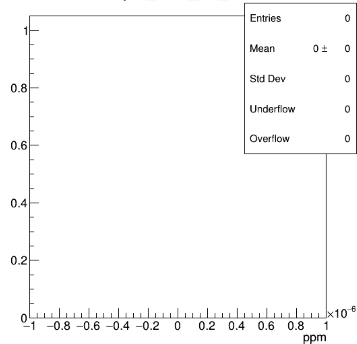
asym_bcm_an_diff
