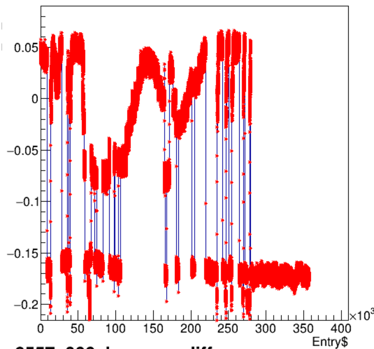
bcm_an_diff:Entry$
