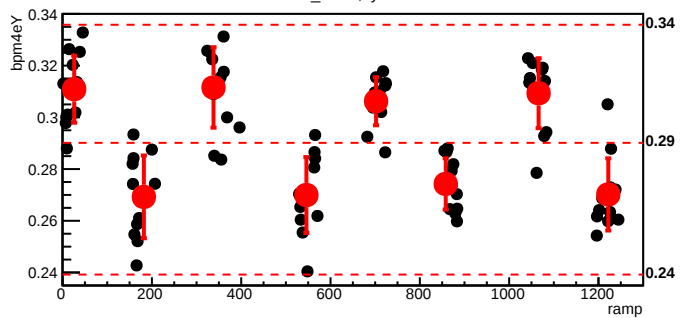
bmod_trim1,cyc=6476
