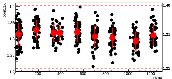
bmod_trim6,cyc=6476
