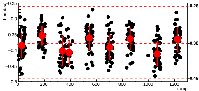
bmod_trim6,cyc=6476
