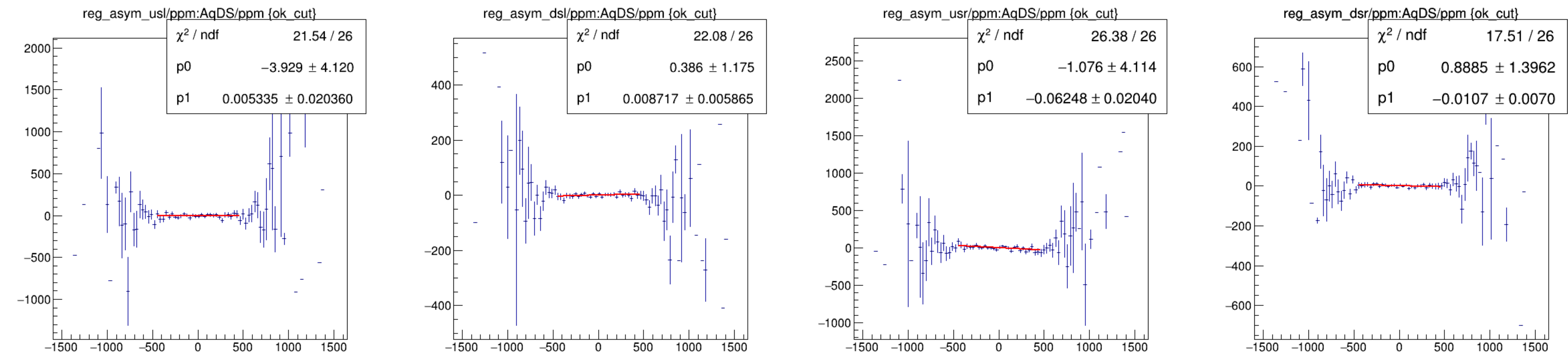
run6574_000_main_vs_AqDS_ratecheck_reg_postpan.png
