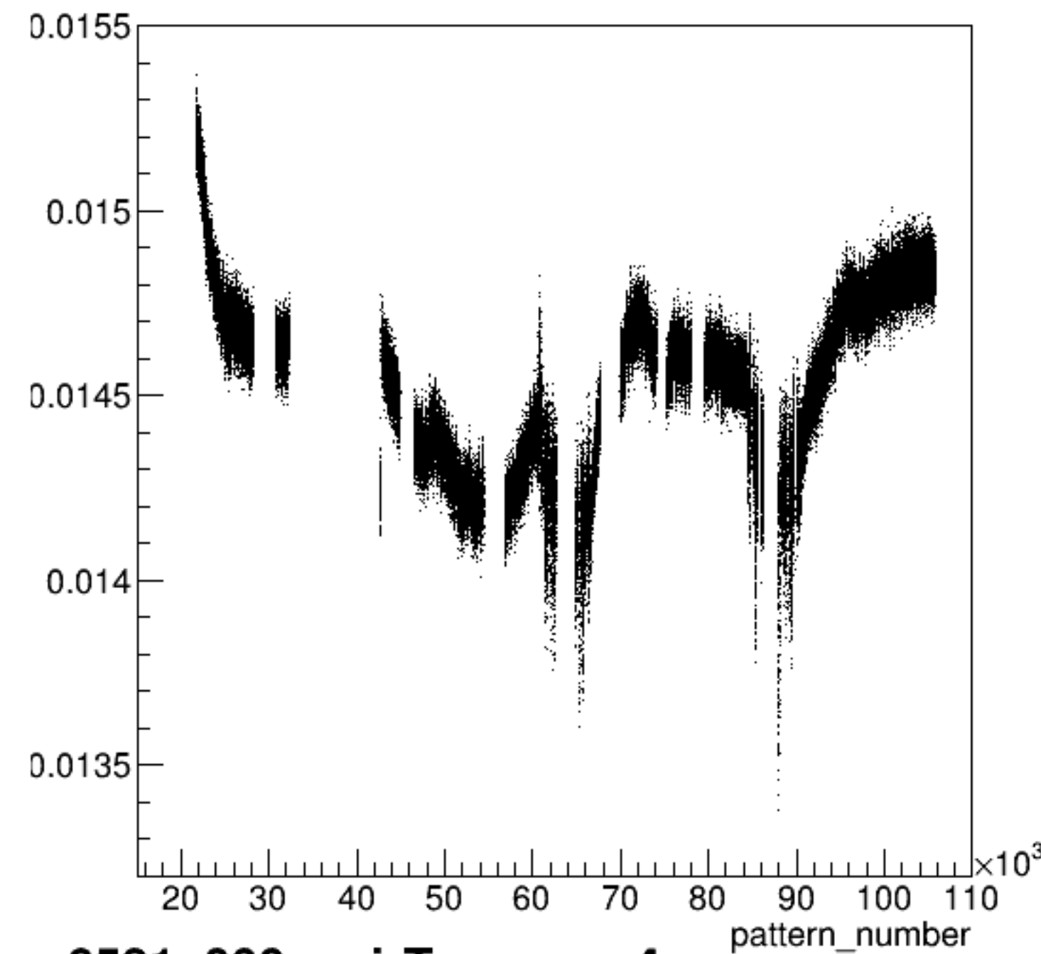
yield_sam4:pattern_number {ErrorFlag==0}
