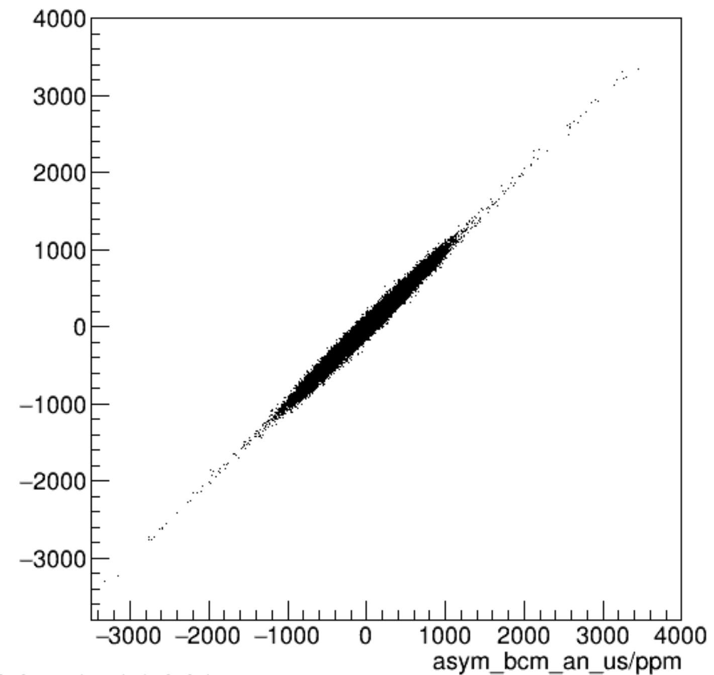
run6584_000_asym_bcm_dg_ds_vs_asym_bcm_an_us_pr.png
