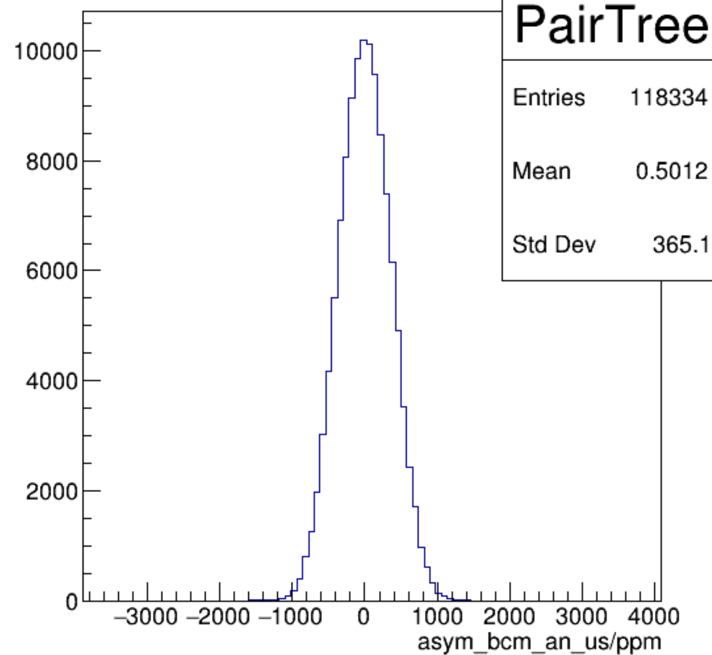
asym_bcm_an_us/ppm {ErrorFlag==0}
