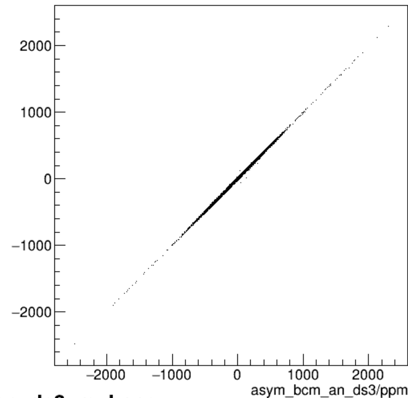
run6584_000_asym_bcm_an_ds_vs_asym_bcm_an_ds3_mul.png
