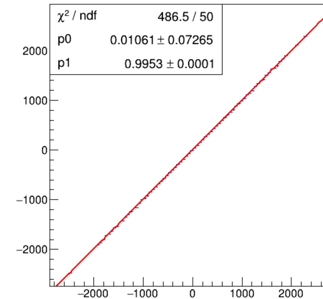
run6584_000_asym_bcm_an_ds_vs_asym_bcm_an_ds3_mul.png
