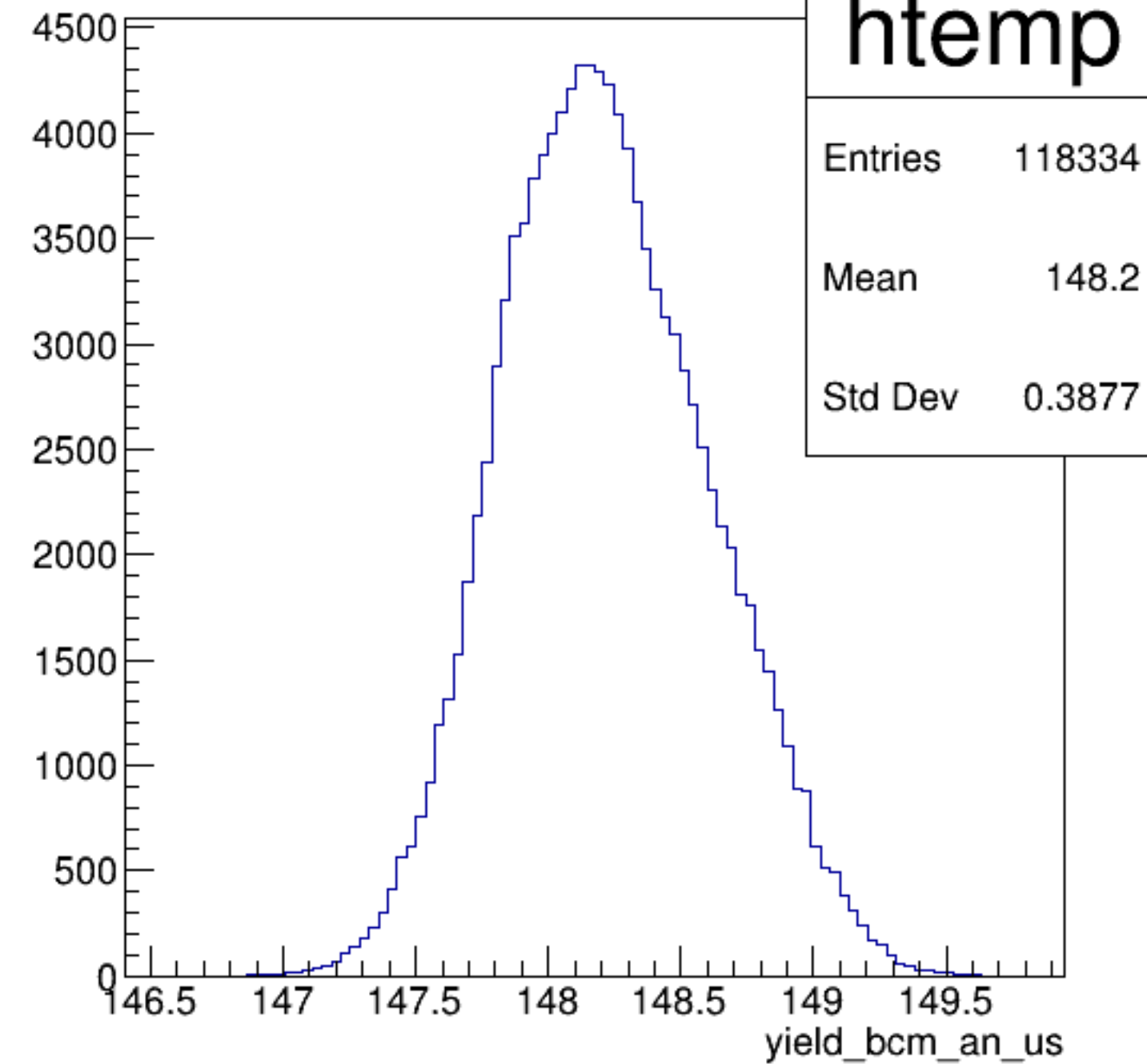
yield_bcm_an_us {ErrorFlag==0}
