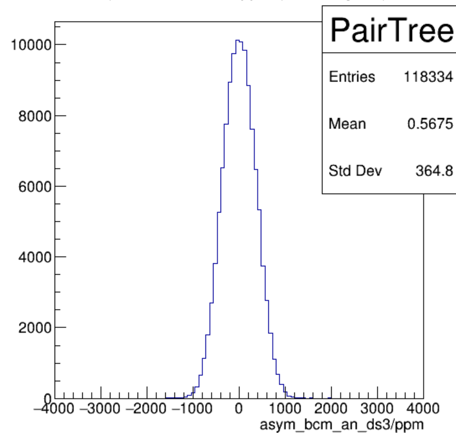
asym_bcm_an_ds3/ppm {ErrorFlag==0}
