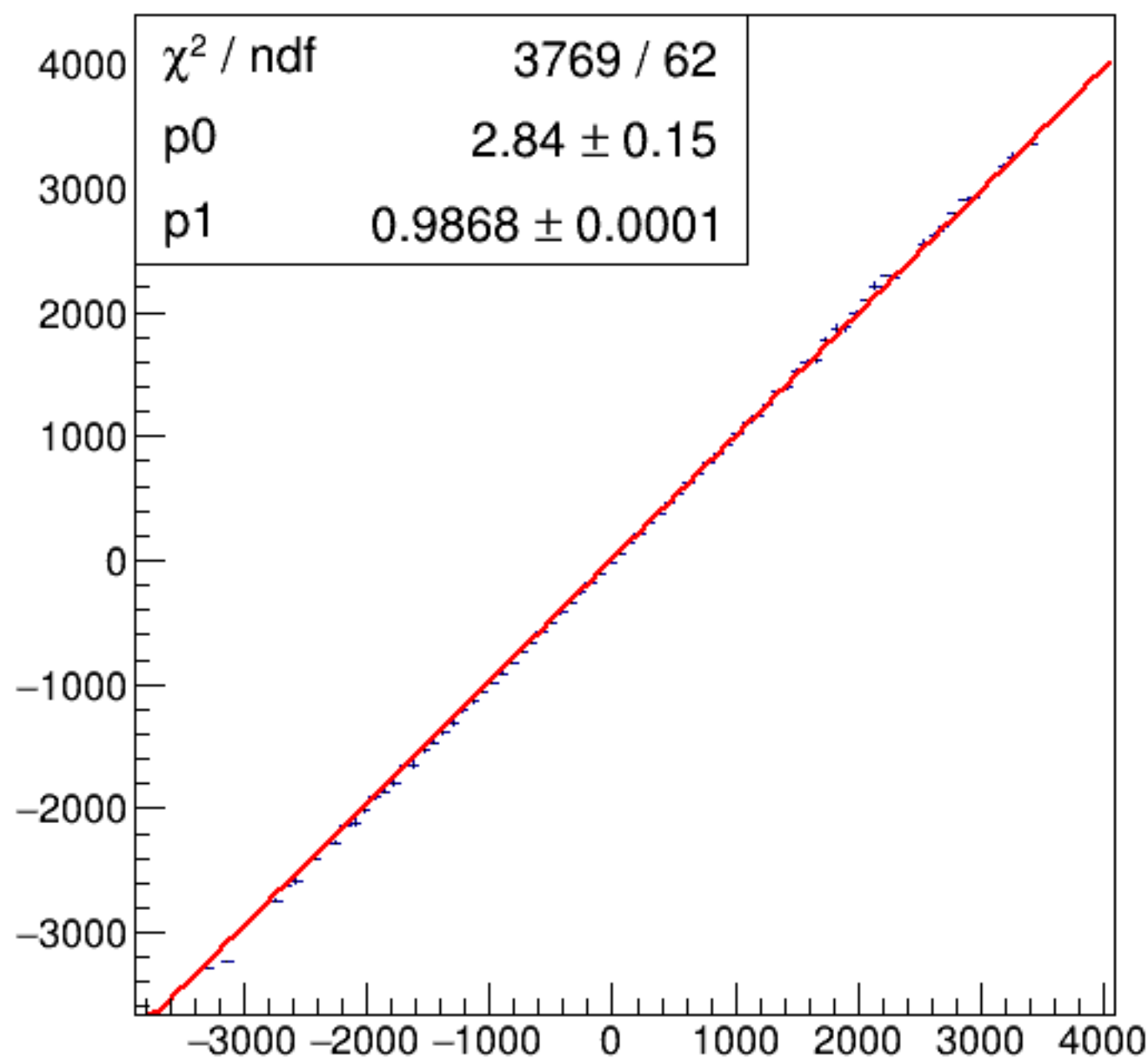
run6584_000_asym_bcm_dg_ds_vs_asym_bcm_an_us_pr.png
