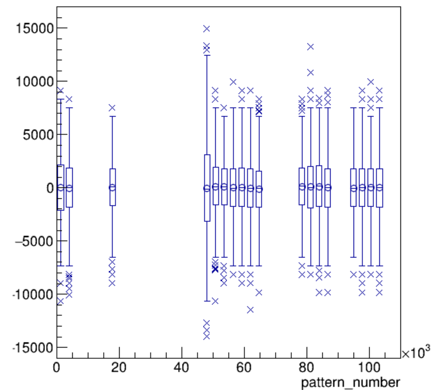
asym_atl1/ppm:pattern_number {ErrorFlag==0}
