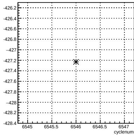
4eX_coil1:cyclenum {run == 6586}
