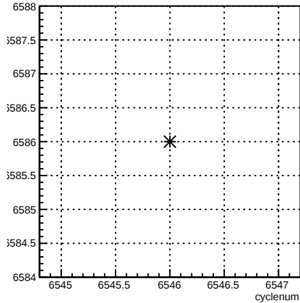
run:cyclenum {run == 6586}
