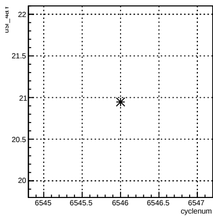
usr_4aY:cyclenum {run == 6586}
