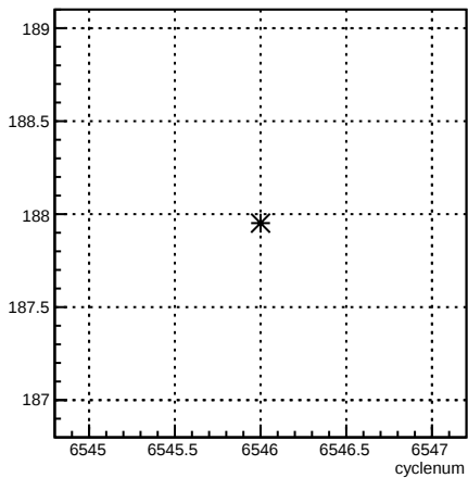
4eY_coil4:cyclenum {run == 6586}
