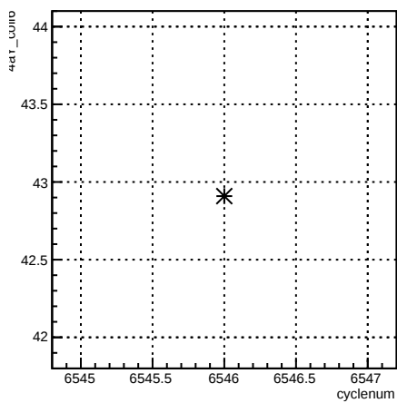
4aY_coil6:cyclenum {run == 6586}
