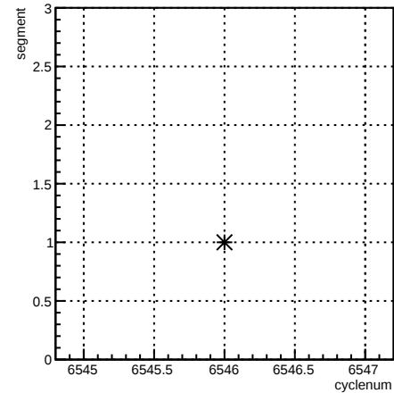
segment:cyclenum {run == 6586}
