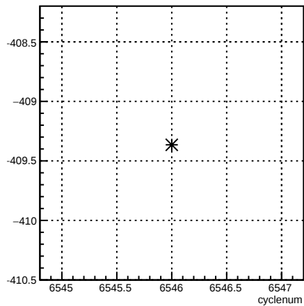
12X_coil7:cyclenum {run == 6586}
