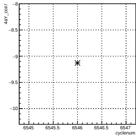
4aY_coil7:cyclenum {run == 6586}
