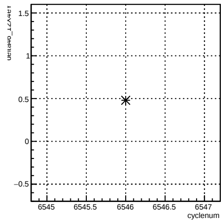
delta46_12X4eY:cyclenum {run == 6586}
