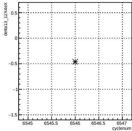
delta13_12X4eX:cyclenum {run == 6586}
