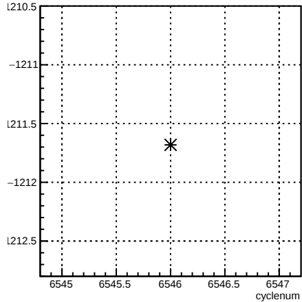
usl_coil6:cyclenum {run == 6586}
