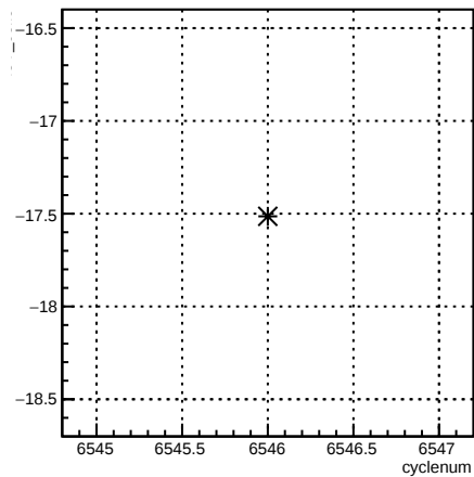
4eY_coil6:cyclenum {run == 6586}
