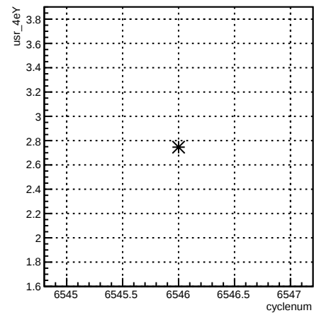
usr_4eY:cyclenum {run == 6586}
