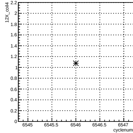
run:cyclenum {run == 6586}
