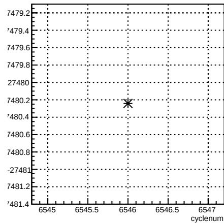
usr_coil6:cyclenum {run == 6586}
