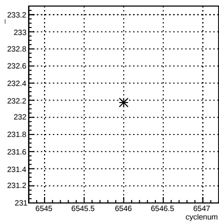
usr_4eX:cyclenum {run == 6586}
