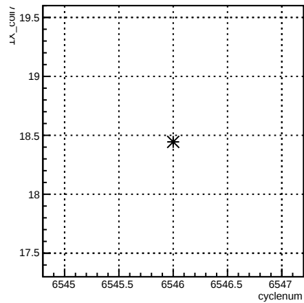
4eX_coil7:cyclenum {run == 6586}
