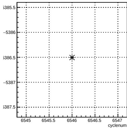
usr_coil7:cyclenum {run == 6586}
