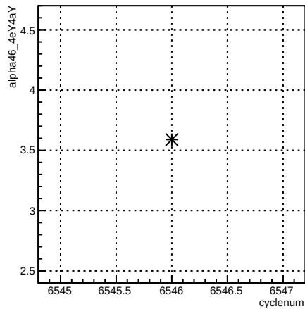
alpha46_4eY4aY:cyclenum {run == 6586}
