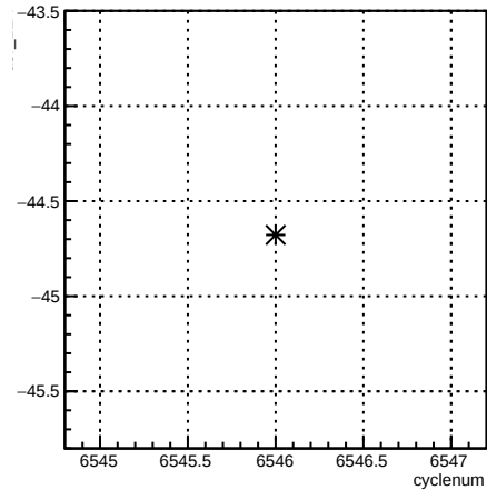
usr_12X:cyclenum {run == 6586}
