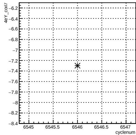
4eY_coil7:cyclenum {run == 6586}
