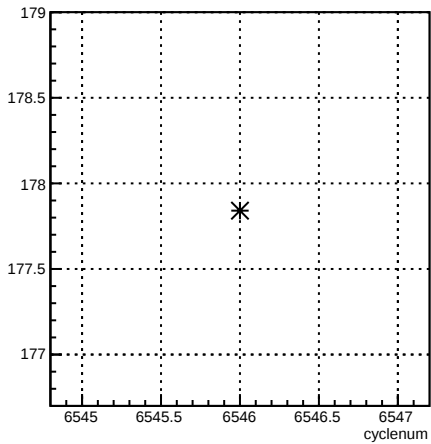
4aY_coil4:cyclenum {run == 6586}
