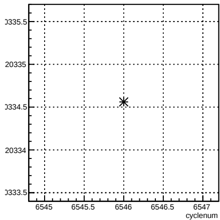
usl_coil7:cyclenum {run == 6586}
