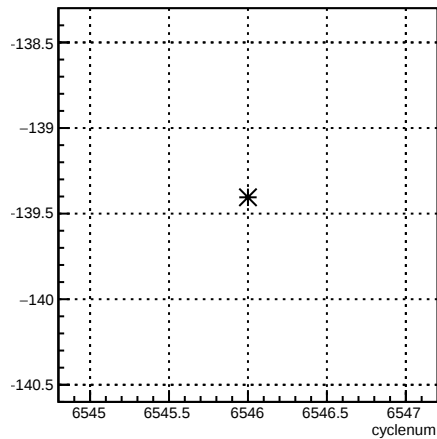
usl_4eY:cyclenum {run == 6586}
