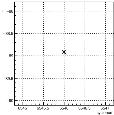
4eX_coil3:cyclenum {run == 6586}
