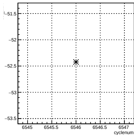
usl_12X:cyclenum {run == 6586}
