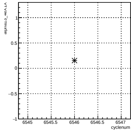
alpha13_4eX1X:cyclenum {run == 6586}
