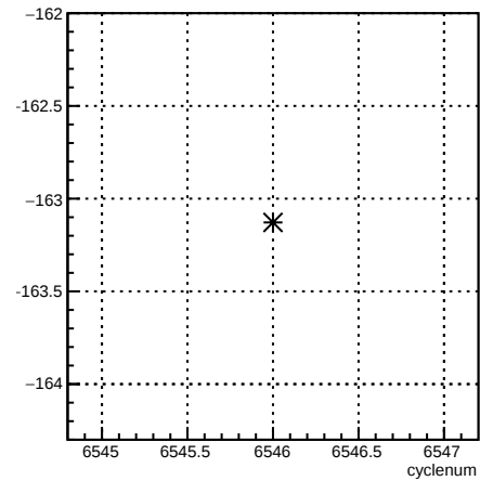
usr_1X:cyclenum {run == 6586}
