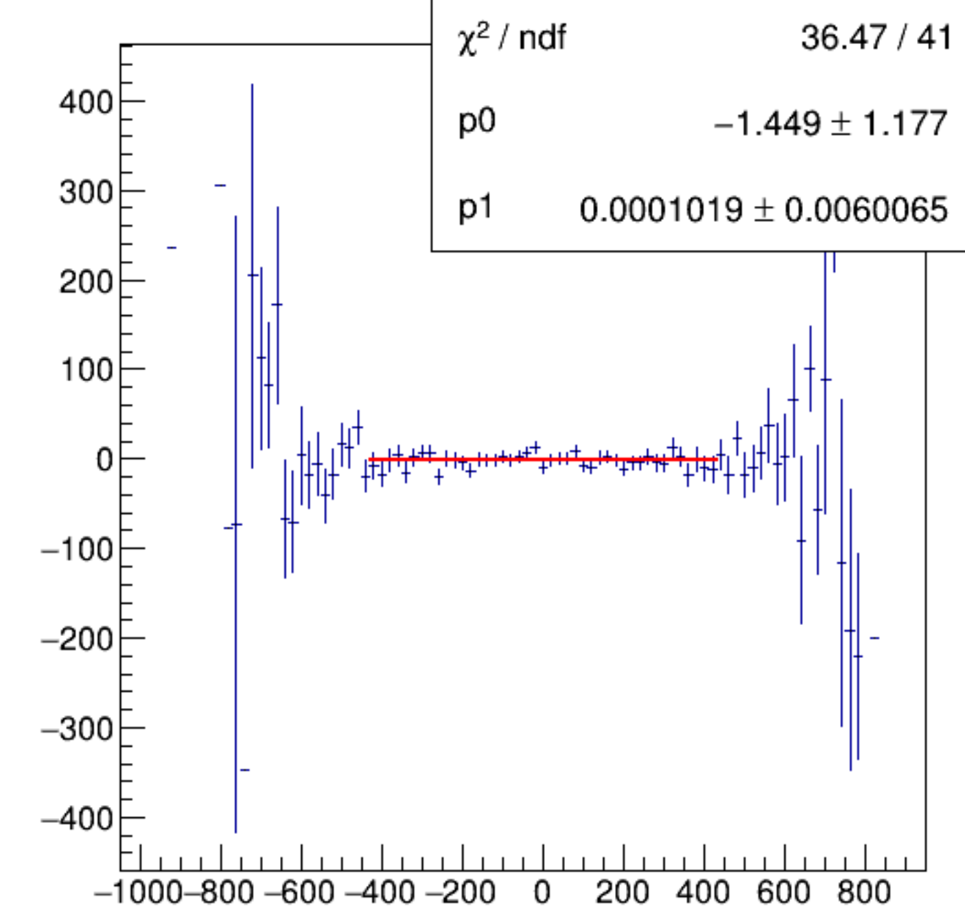
reg_asym_dsl/ppm:AqUS/ppm {ok_cut}
