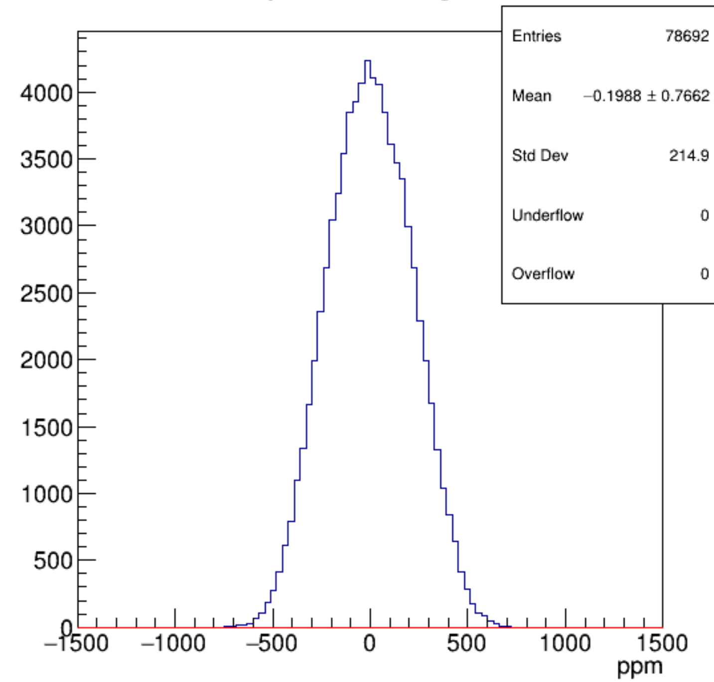
asym_bcm_dg_ds
