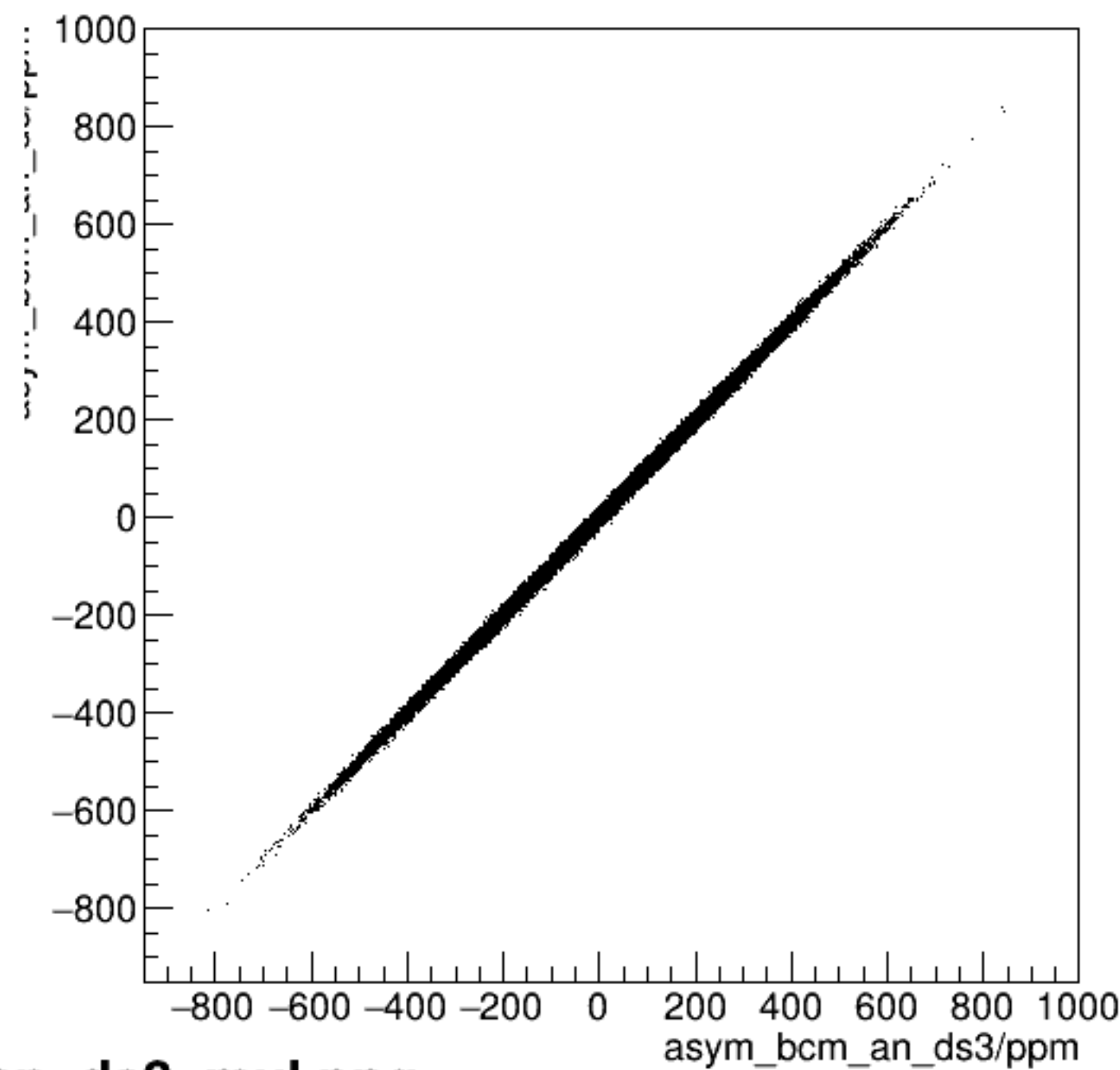
run6587_000_asym_bcm_an_ds_vs_asym_bcm_an_ds3_mul.png
