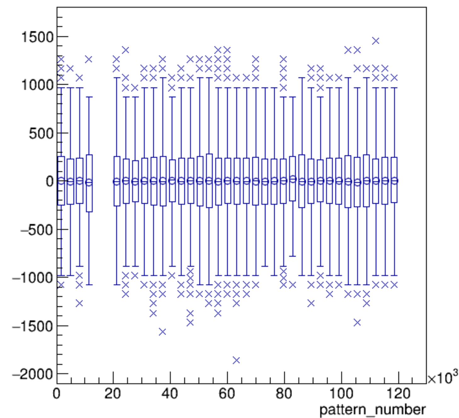
asym_bcm_an_ds/ppm:pattern_number {ErrorFlag==0}
