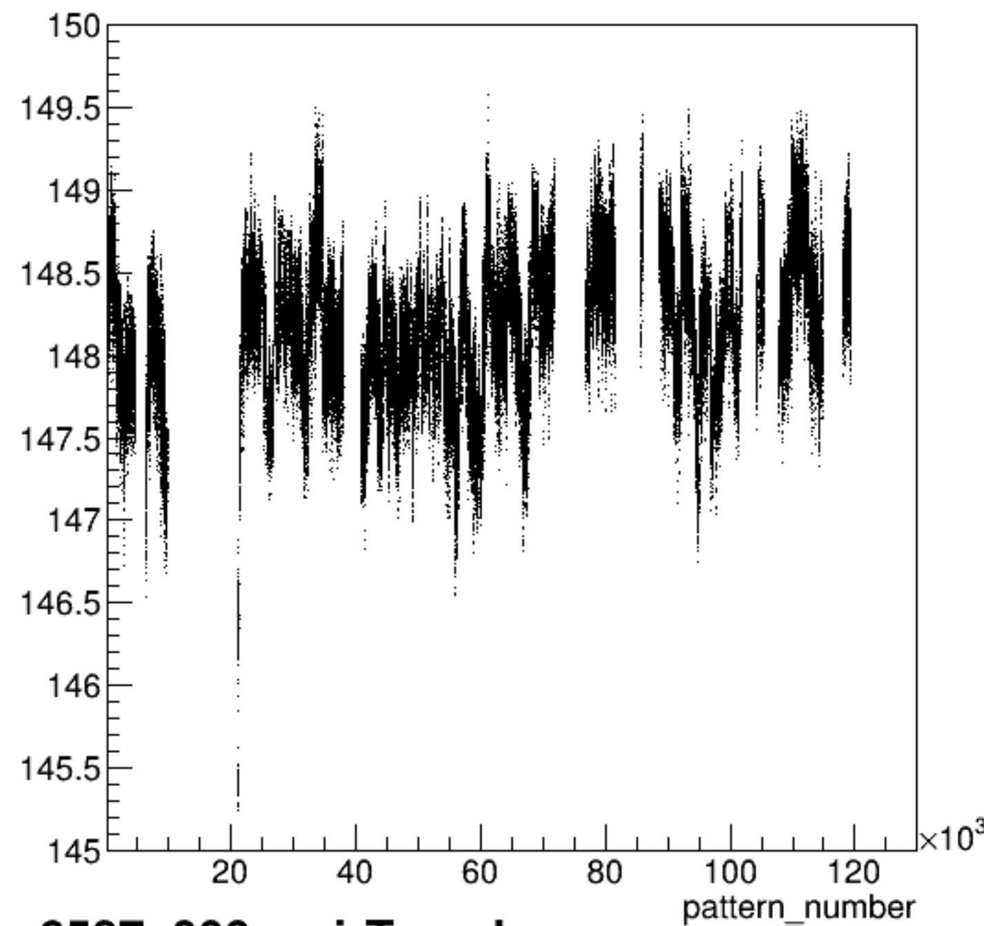
yield_bcm_an_us:pattern_number {ErrorFlag==0}
