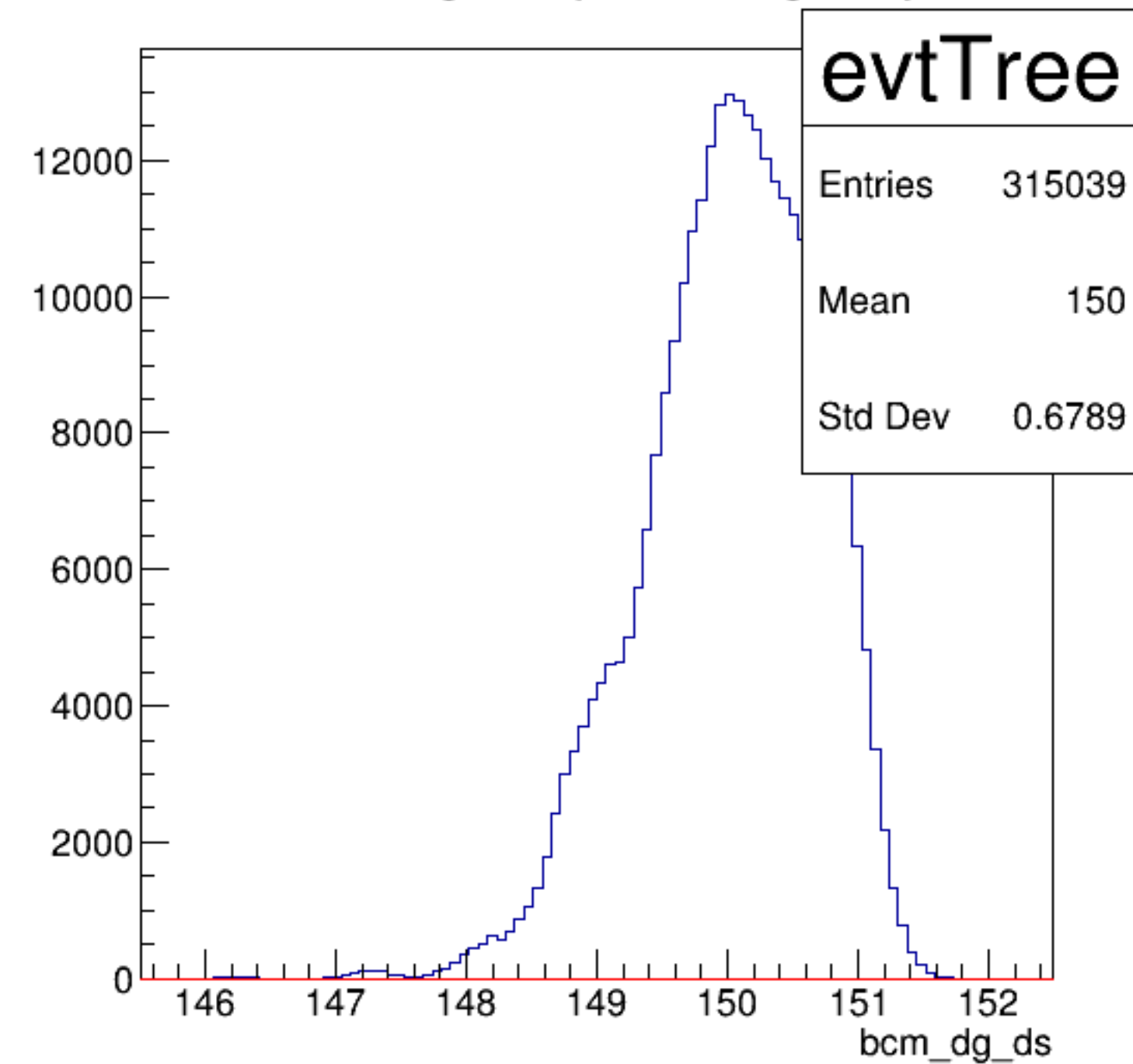
bcm_dg_ds {ErrorFlag==0}
