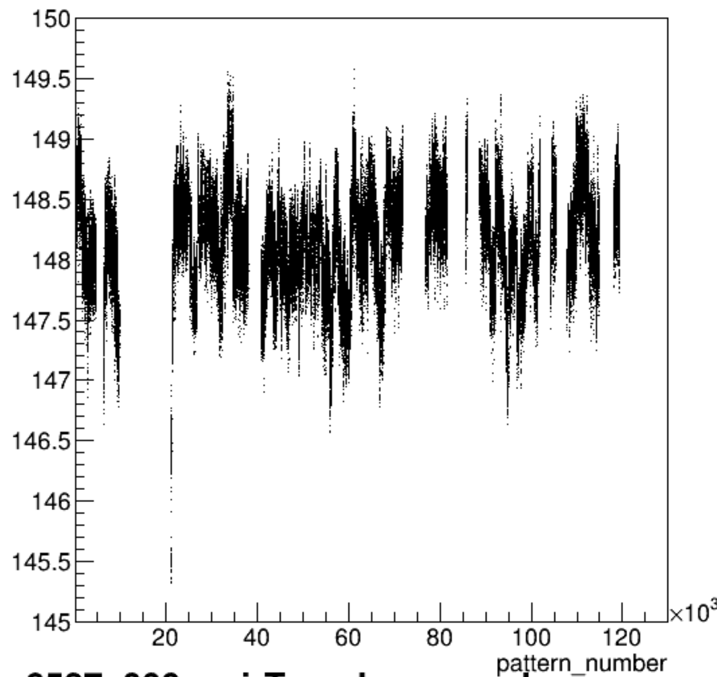
yield_bcm_an_ds:pattern_number {ErrorFlag==0}
