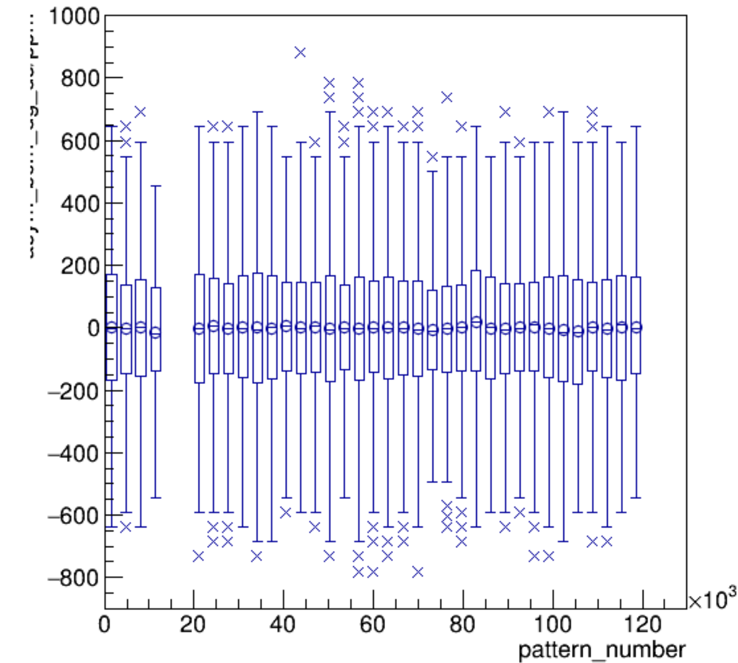
asym_bcm_dg_ds/ppm:pattern_number {ErrorFlag==0}
