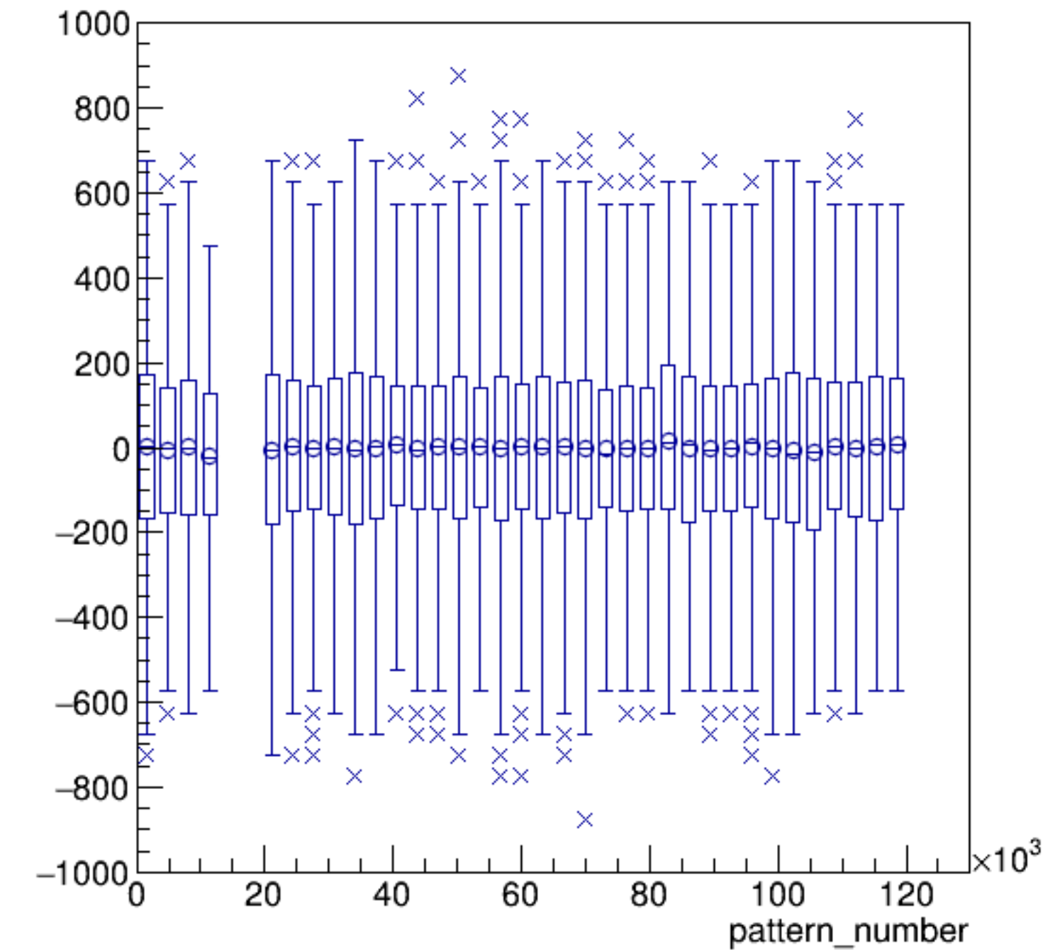
asym_bcm_dg_us/ppm:pattern_number {ErrorFlag==0}
