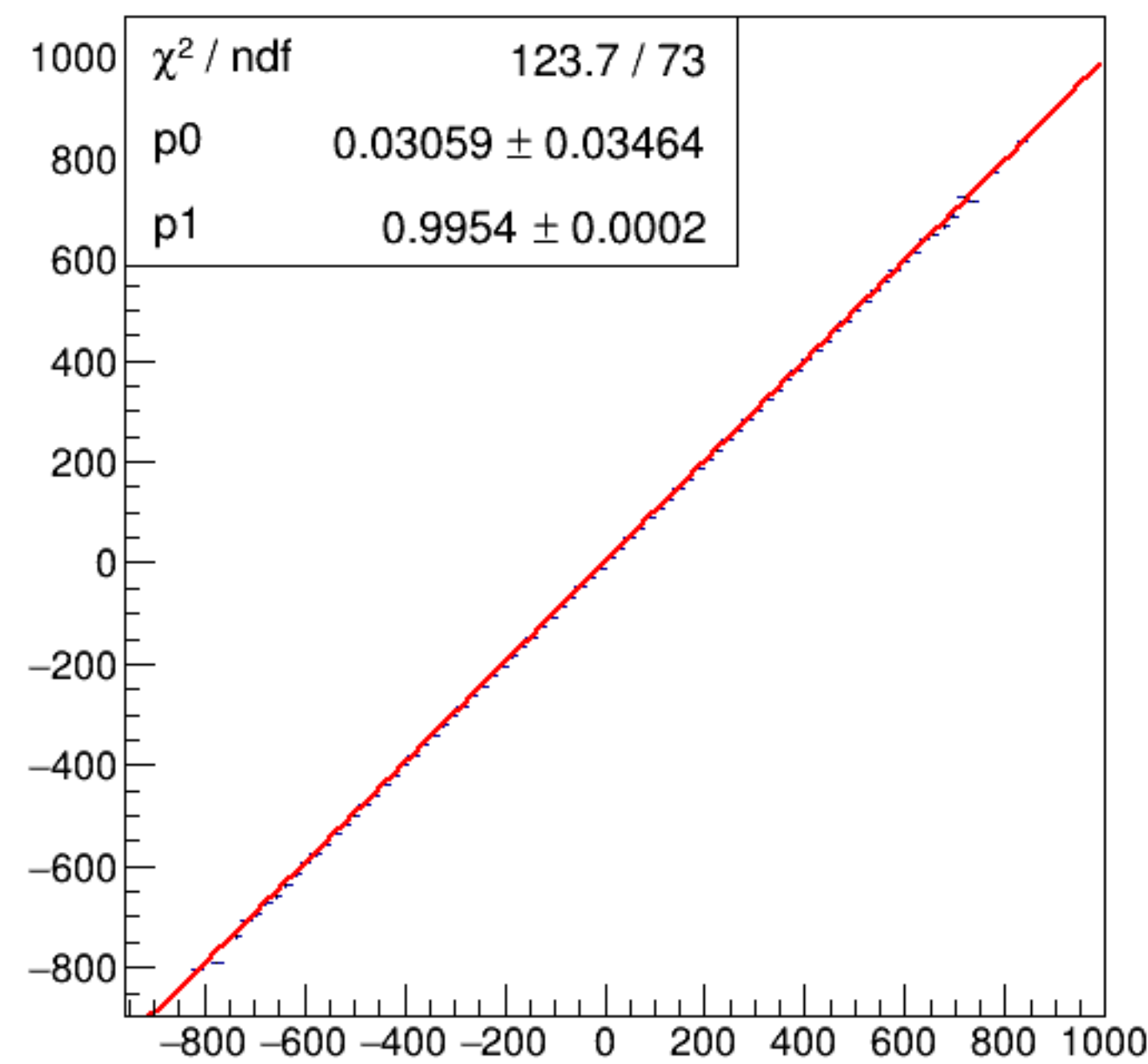
run6587_000_asym_bcm_an_ds_vs_asym_bcm_an_ds3_mul.png
