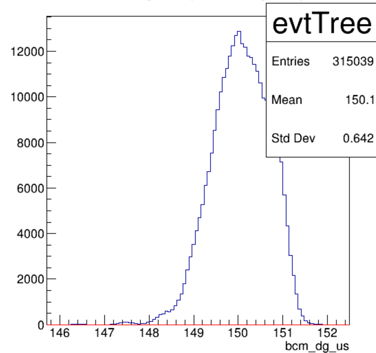
bcm_dg_us {ErrorFlag==0}
