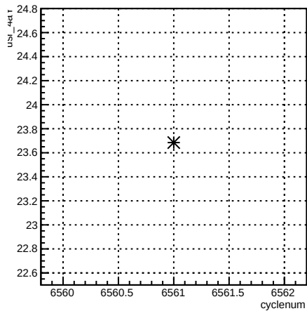
usr_4aY:cyclenum {run == 6589}
