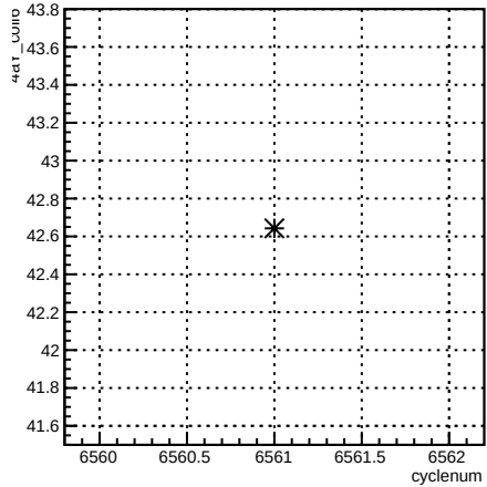
4eY_coil6:cyclenum {run == 6589}
