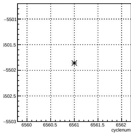
usr_coil3:cyclenum {run == 6589}
