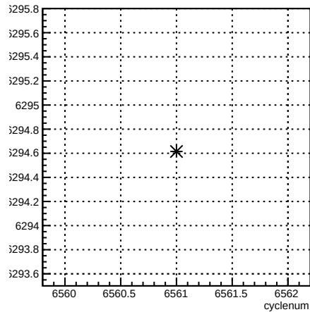
usl_coil3:cyclenum {run == 6589}
