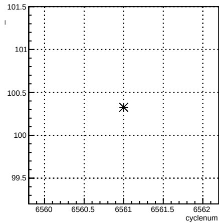
usl_4eX:cyclenum {run == 6589}
