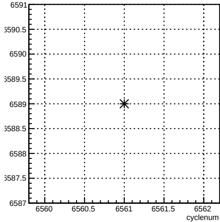
run:cyclenum {run == 6589}
