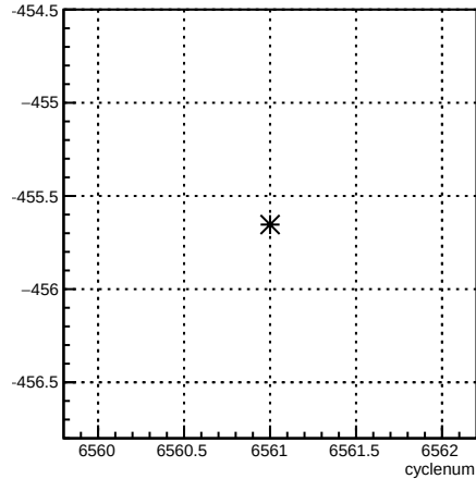
4eX_coil1:cyclenum {run == 6589}
