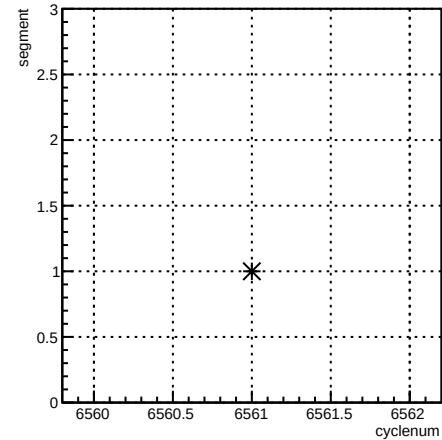
segment:cyclenum {run == 6589}
