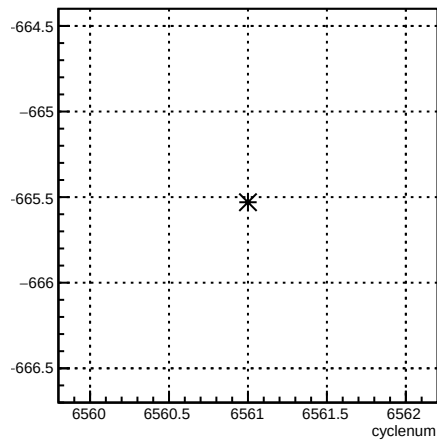
usr_coil6:cyclenum {run == 6589}
