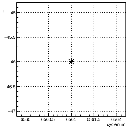
usr_12X:cyclenum {run == 6589}
