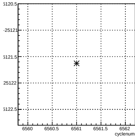
usr_coil1:cyclenum {run == 6589}
