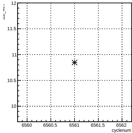
usl_4eY:cyclenum {run == 6589}
