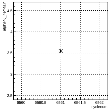
alpha46_4eY4aY:cyclenum {run == 6589}
