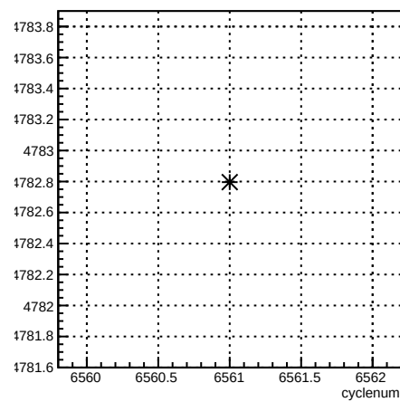
usr_coil4:cyclenum {run == 6589}
