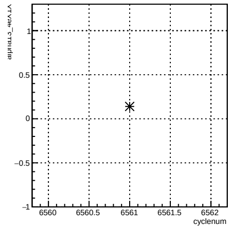
alpha13_4eX1X:cyclenum {run == 6589}
