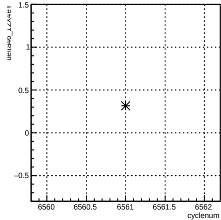
delta46_12X4eY:cyclenum {run == 6589}
