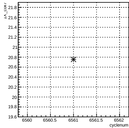
4eX_coil7:cyclenum {run == 6589}
