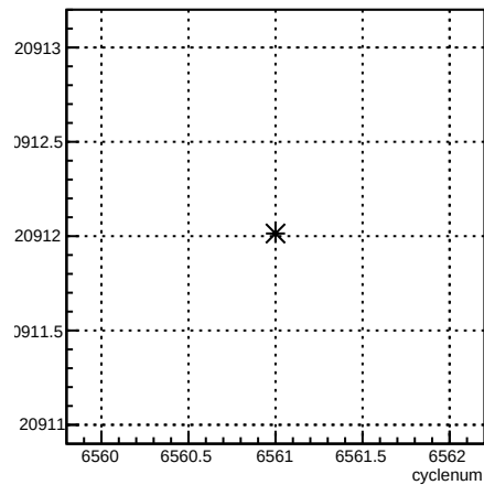
usl_coil7:cyclenum {run == 6589}
