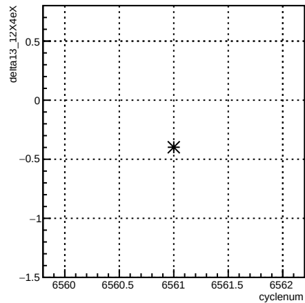
delta13_12X4eX:cyclenum {run == 6589}
