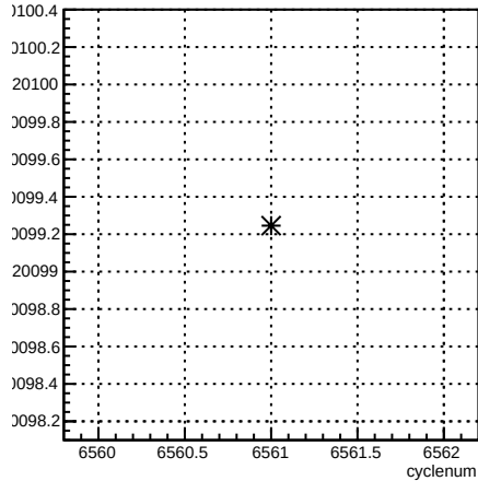
usr_coil7:cyclenum {run == 6589}
