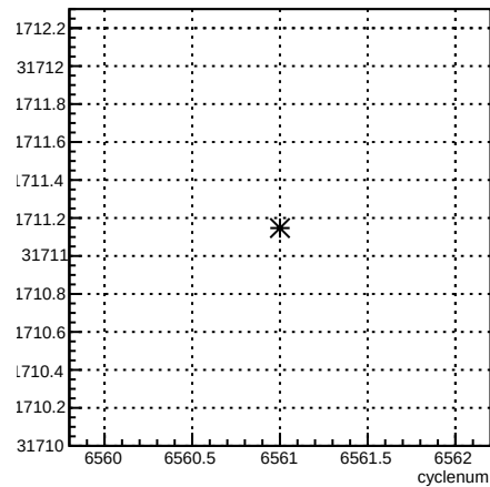
usl_coil6:cyclenum {run == 6589}
