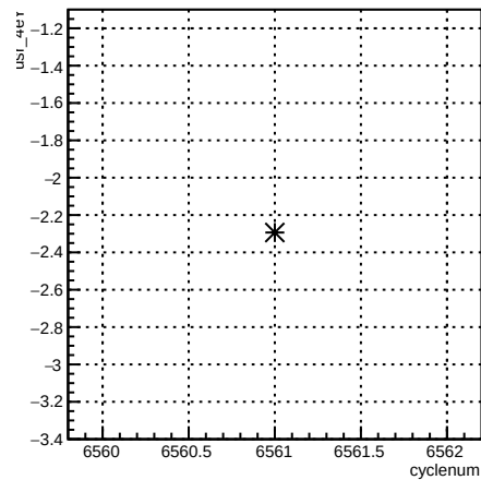
usr_4eY:cyclenum {run == 6589}
