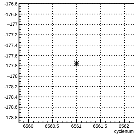
usr_1X:cyclenum {run == 6589}
