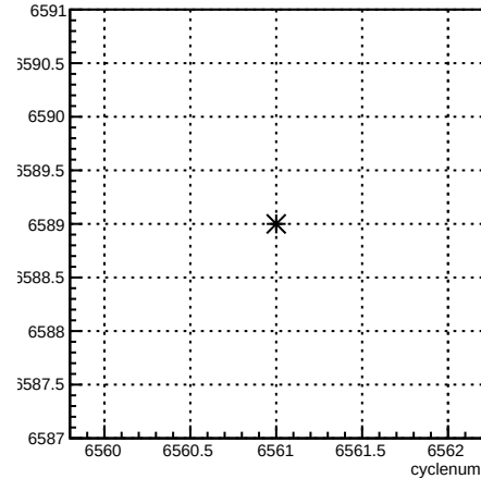
run:cyclenum {run == 6589}
