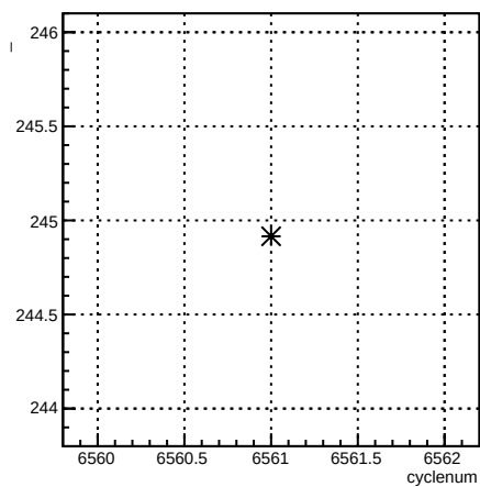
usr_4eX:cyclenum {run == 6589}
