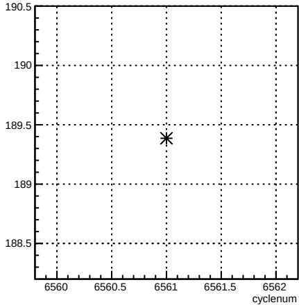
4eY_coil4:cyclenum {run == 6589}
