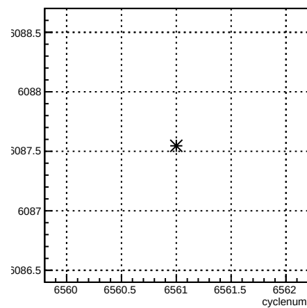
usl_coil4:cyclenum {run == 6589}
