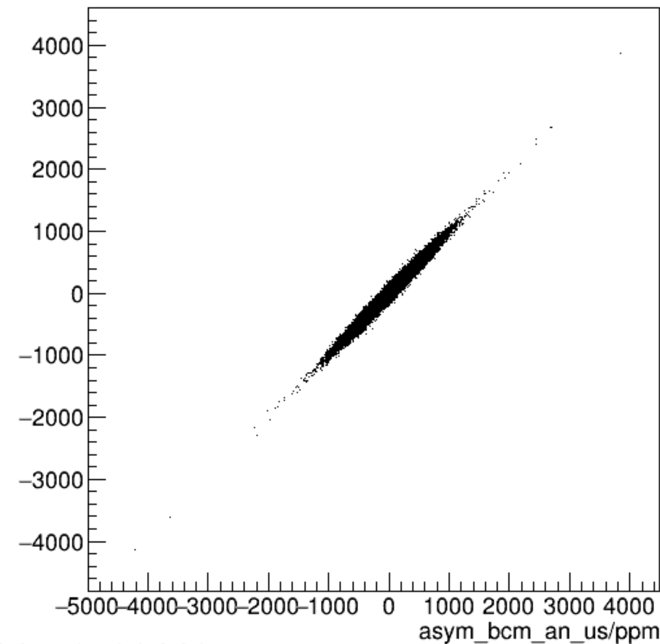
run6590_000_asym_bcm_dg_ds_vs_asym_bcm_an_us_pr.png
