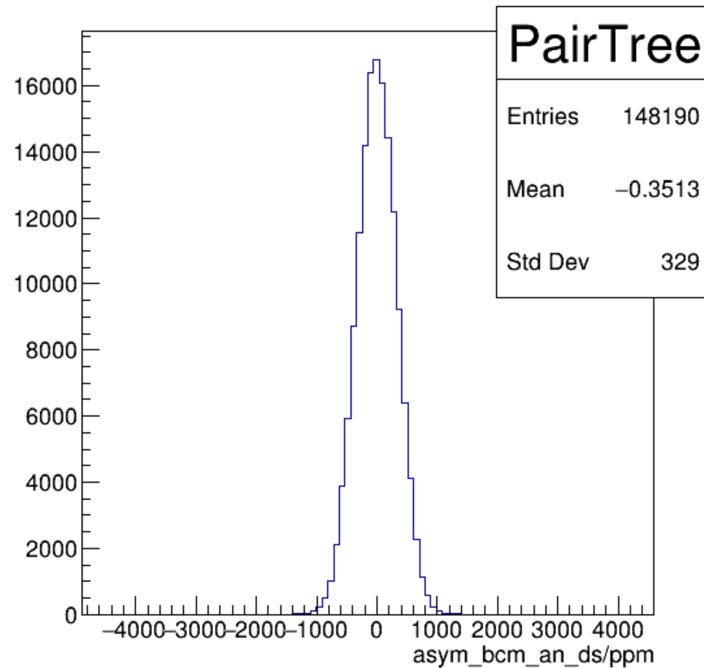
asym_bcm_an_ds/ppm {ErrorFlag==0}
