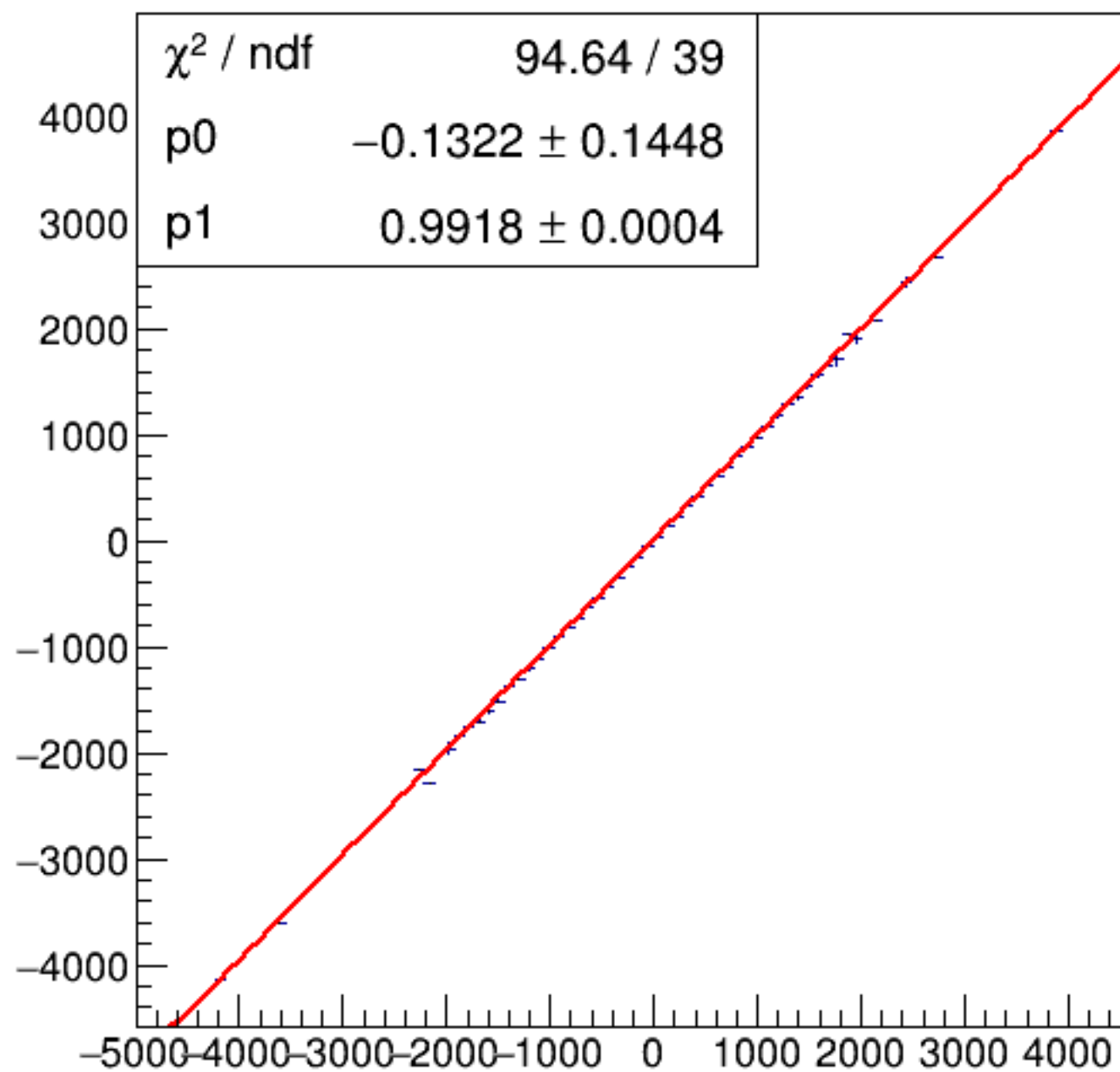
run6590_000_asym_bcm_dg_ds_vs_asym_bcm_an_us_pr.png
