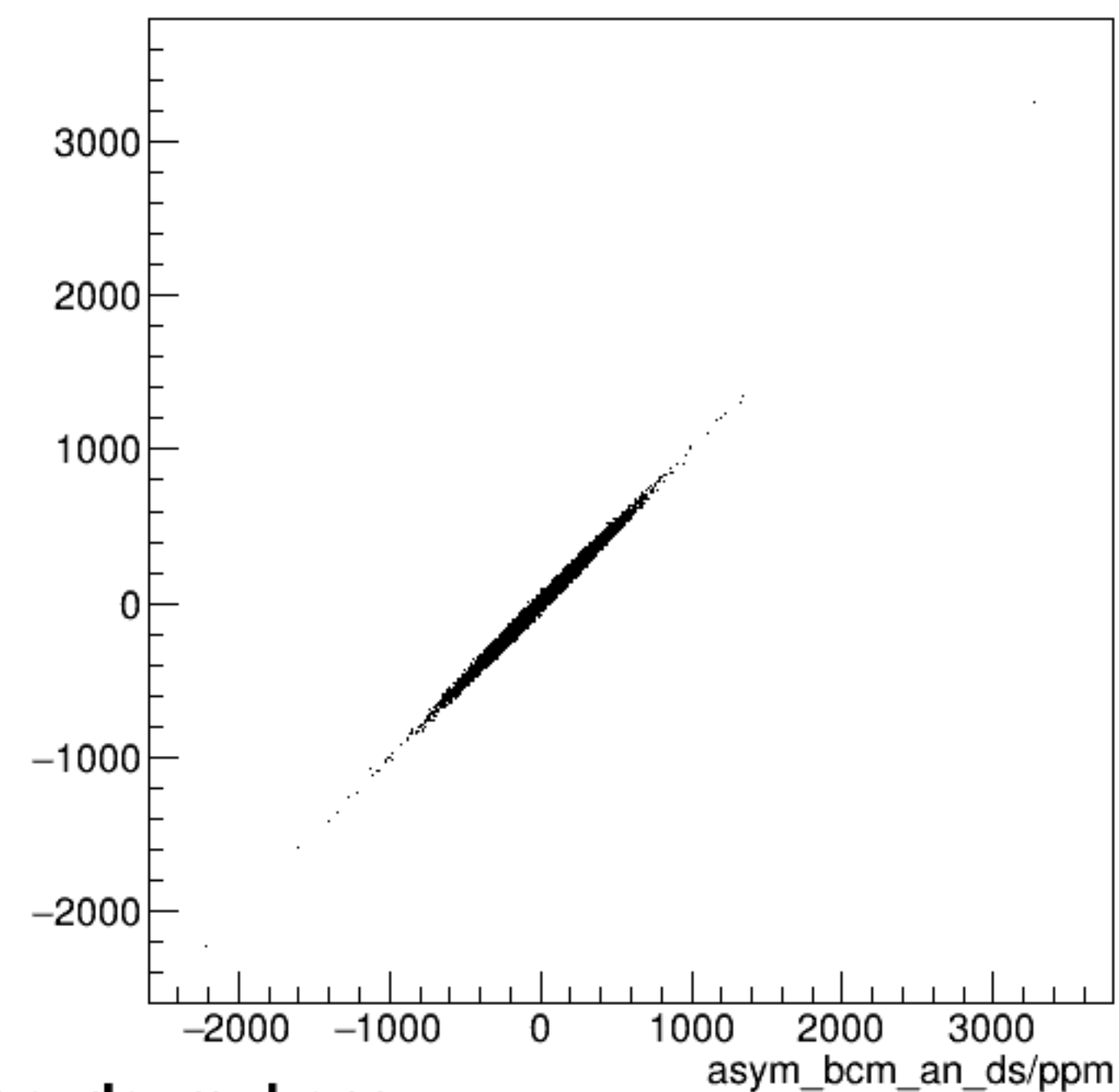
run6590_000_asym_bcm_an_us_vs_asym_bcm_an_ds_mul.png
