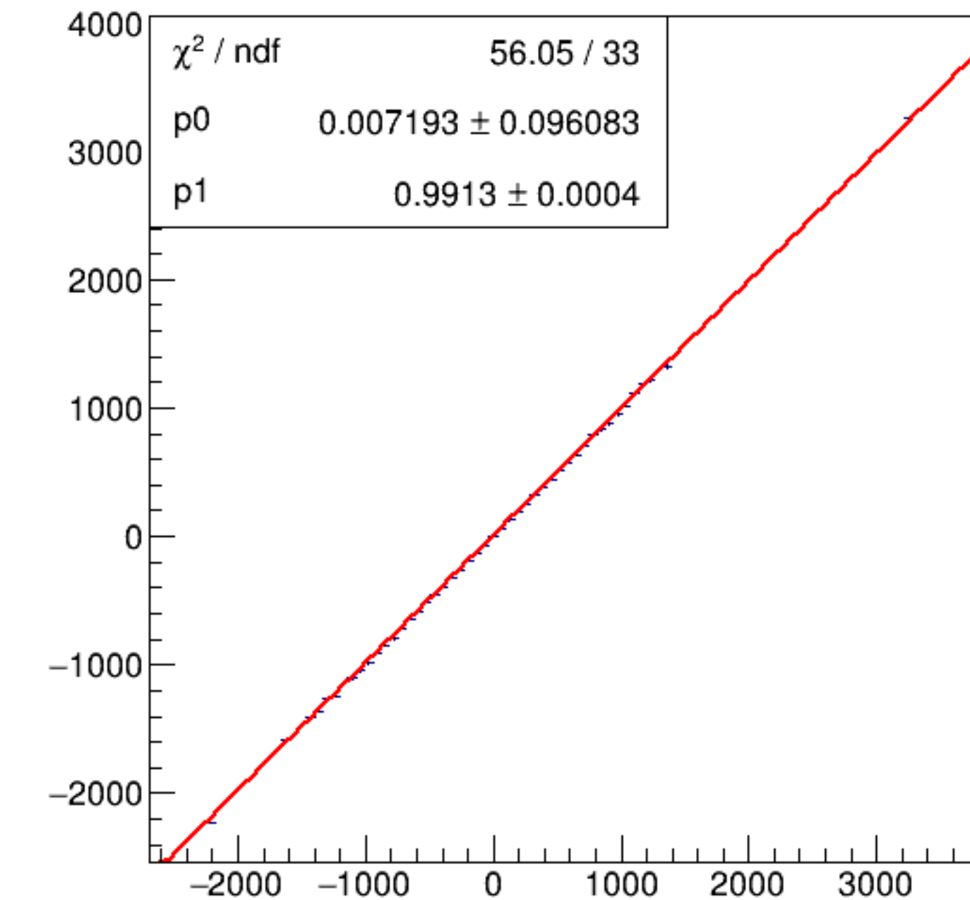
run6590_000_asym_bcm_an_us_vs_asym_bcm_an_ds3_mul.png
