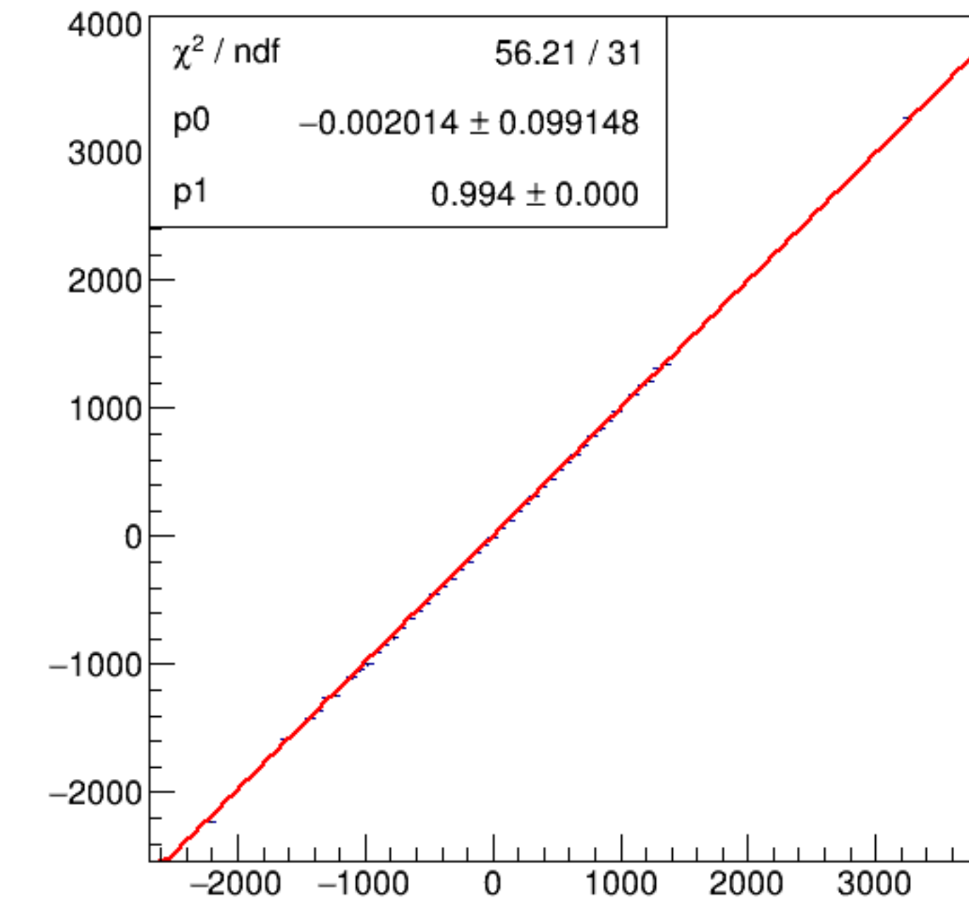
run6590_000_asym_bcm_an_us_vs_asym_bcm_an_ds_mul.png
