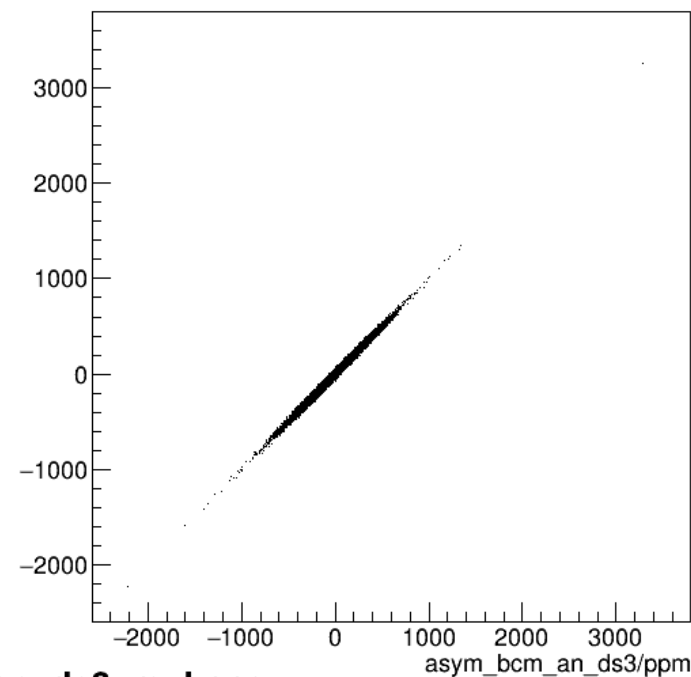
run6590_000_asym_bcm_an_us_vs_asym_bcm_an_ds3_mul.png
