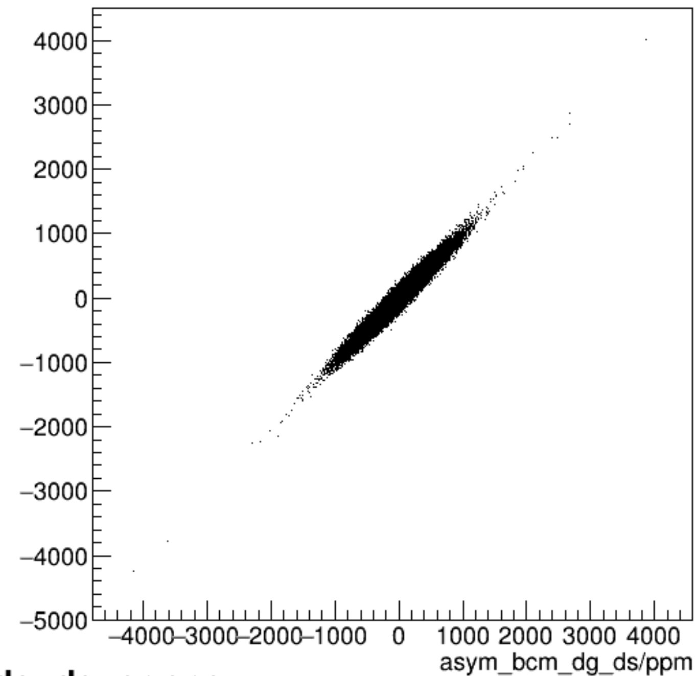
run6590_000_asym_bcm_dg_us_vs_asym_bcm_dg_ds_pr.png
