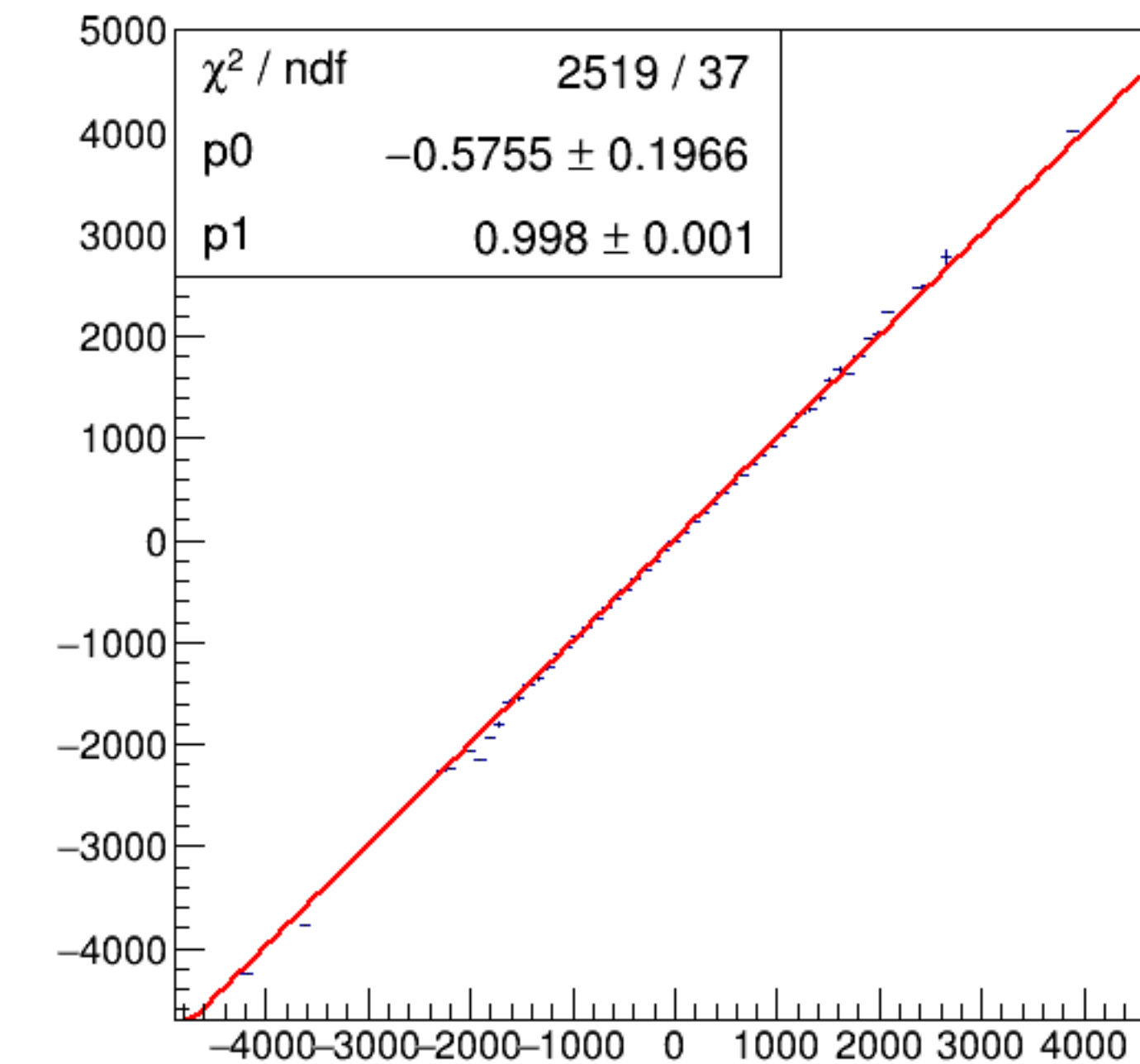
run6590_000_asym_bcm_dg_us_vs_asym_bcm_dg_ds_pr.png
