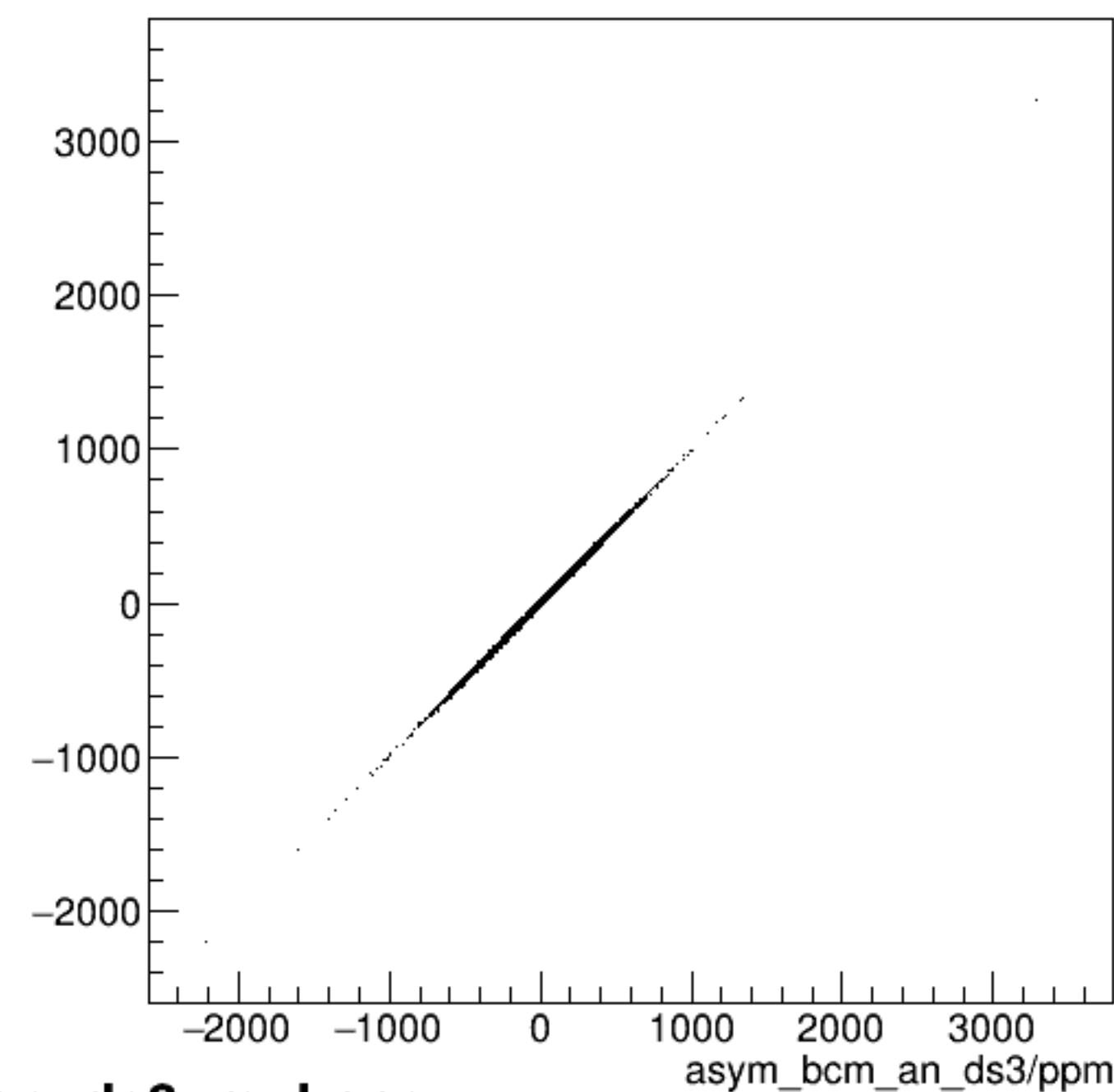
run6590_000_asym_bcm_an_ds_vs_asym_bcm_an_ds3_mul.png
