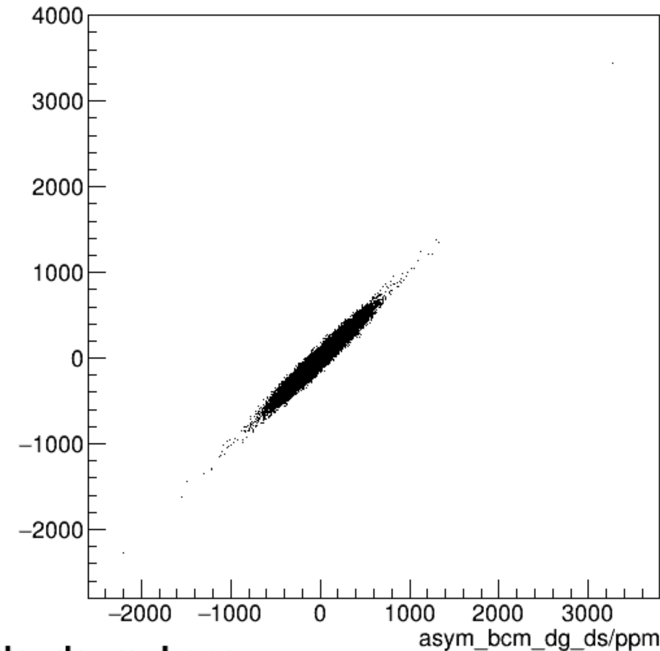
run6590_000_asym_bcm_dg_us_vs_asym_bcm_dg_ds_mul.png
