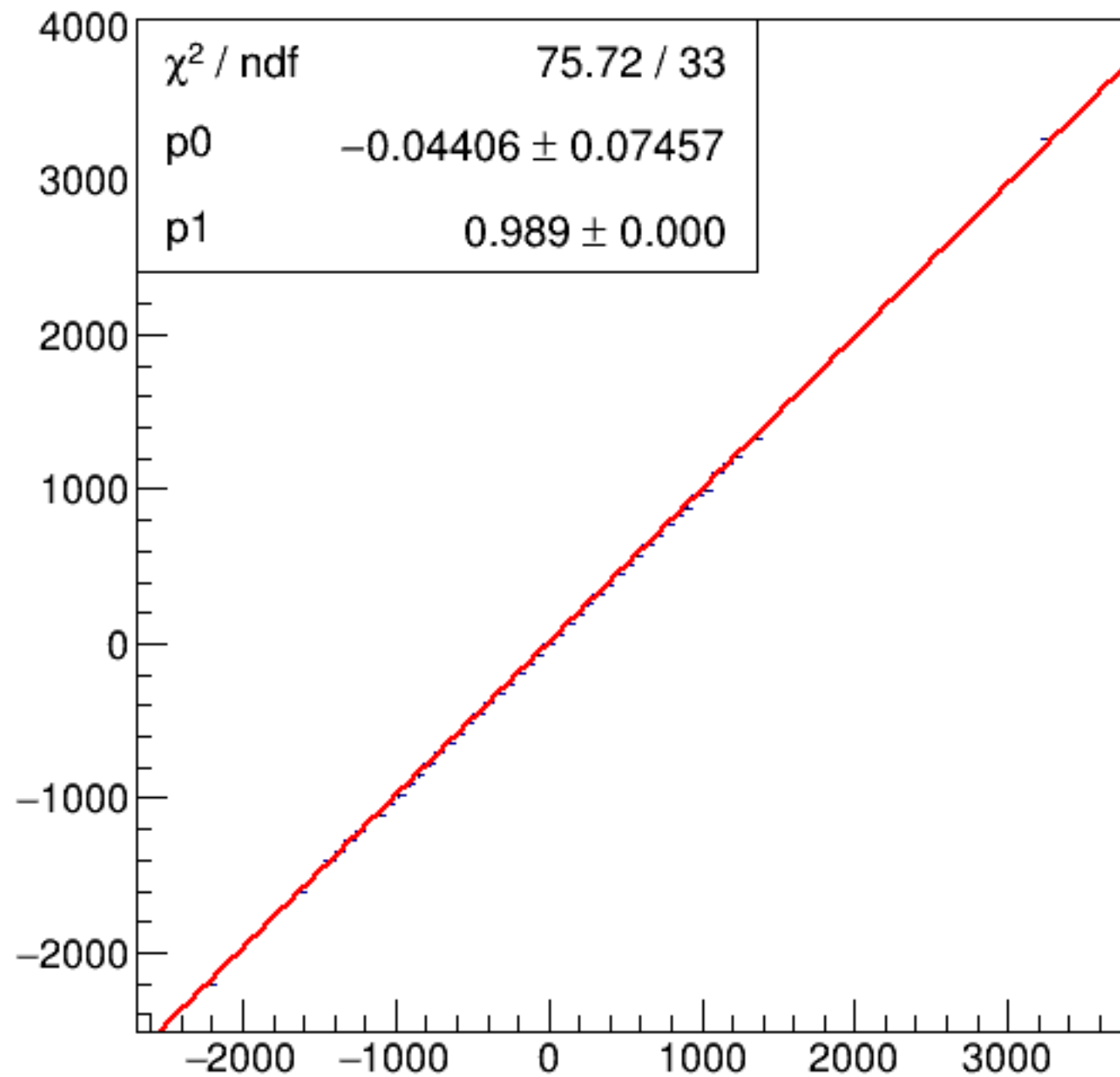
run6590_000_asym_bcm_an_ds_vs_asym_bcm_an_ds3_mul.png
