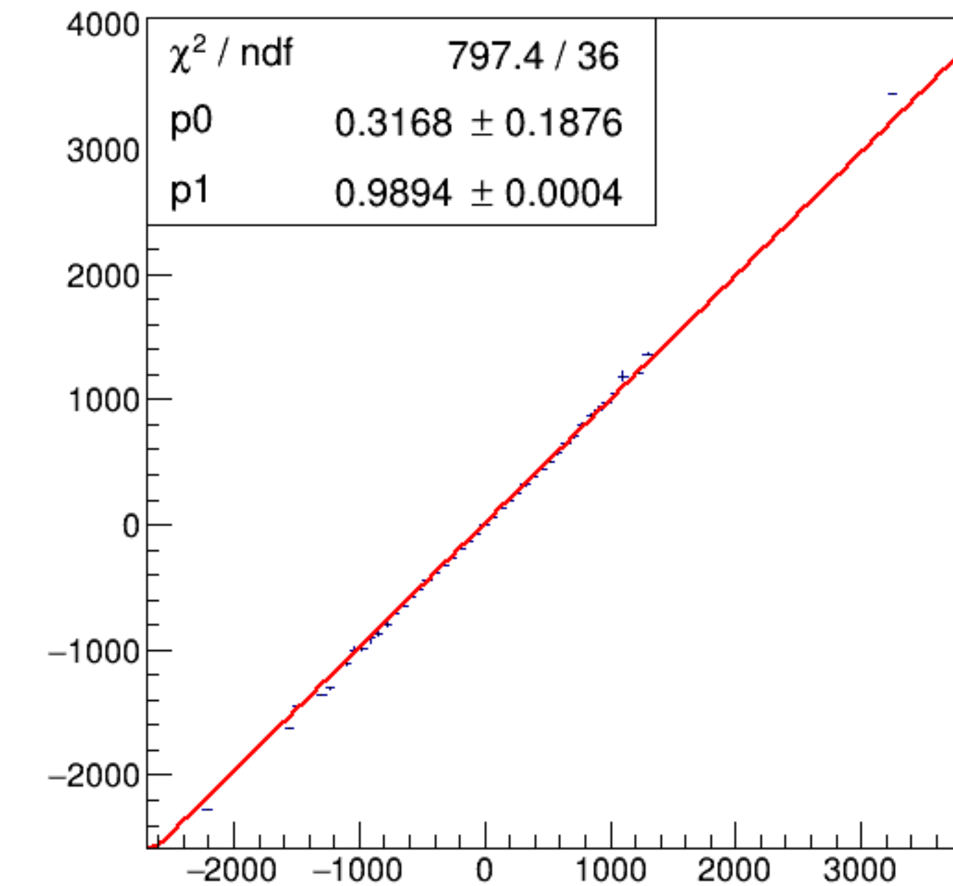
run6590_000_asym_bcm_dg_us_vs_asym_bcm_dg_ds_mul.png
