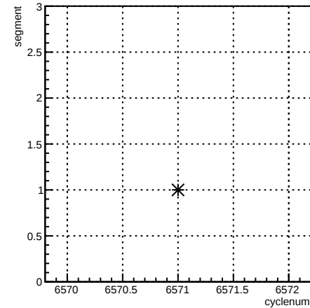
segment:cyclenum {run == 6591}
