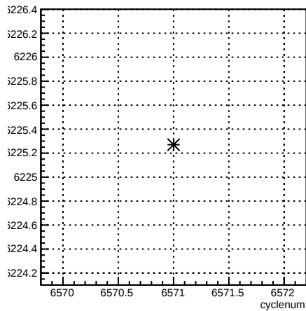
usl_coil3:cyclenum {run == 6591}
