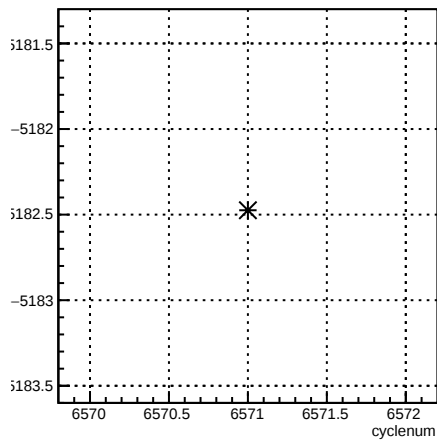
usr_coil3:cyclenum {run == 6591}
