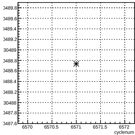
usl_coil6:cyclenum {run == 6591}
