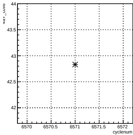
4aY_coil6:cyclenum {run == 6591}
