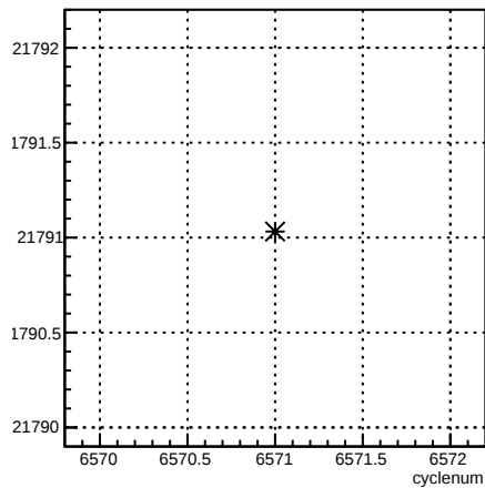
usl_coil7:cyclenum {run == 6591}
