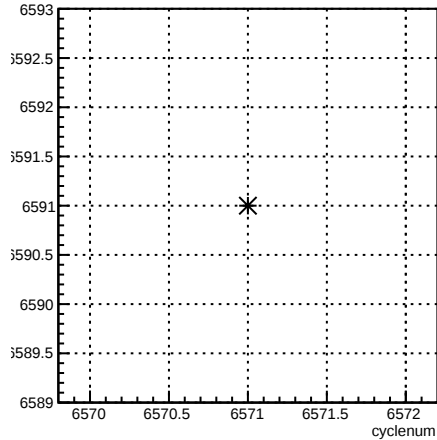
run:cyclenum {run == 6591}
