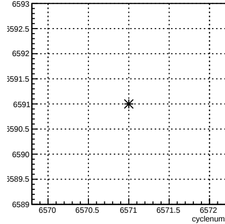
run:cyclenum {run == 6591}
