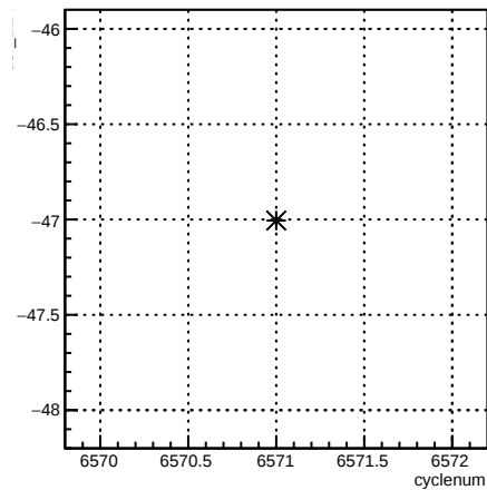
usr_12X:cyclenum {run == 6591}
