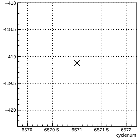
12X_coil7:cyclenum {run == 6591}
