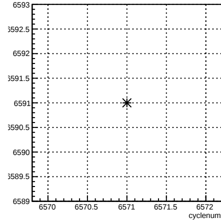
run:cyclenum {run == 6591}
