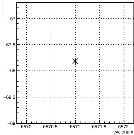
4eX_coil3:cyclenum {run == 6591}
