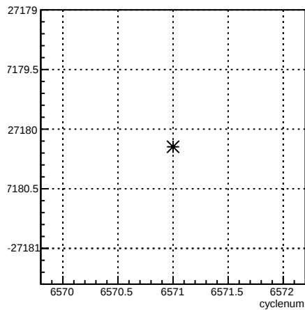
usr_coil1:cyclenum {run == 6591}
