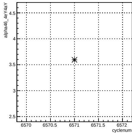
alpha46_4eY4aY:cyclenum {run == 6591}
