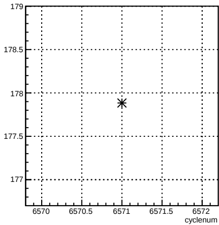
4aY_coil4:cyclenum {run == 6591}
