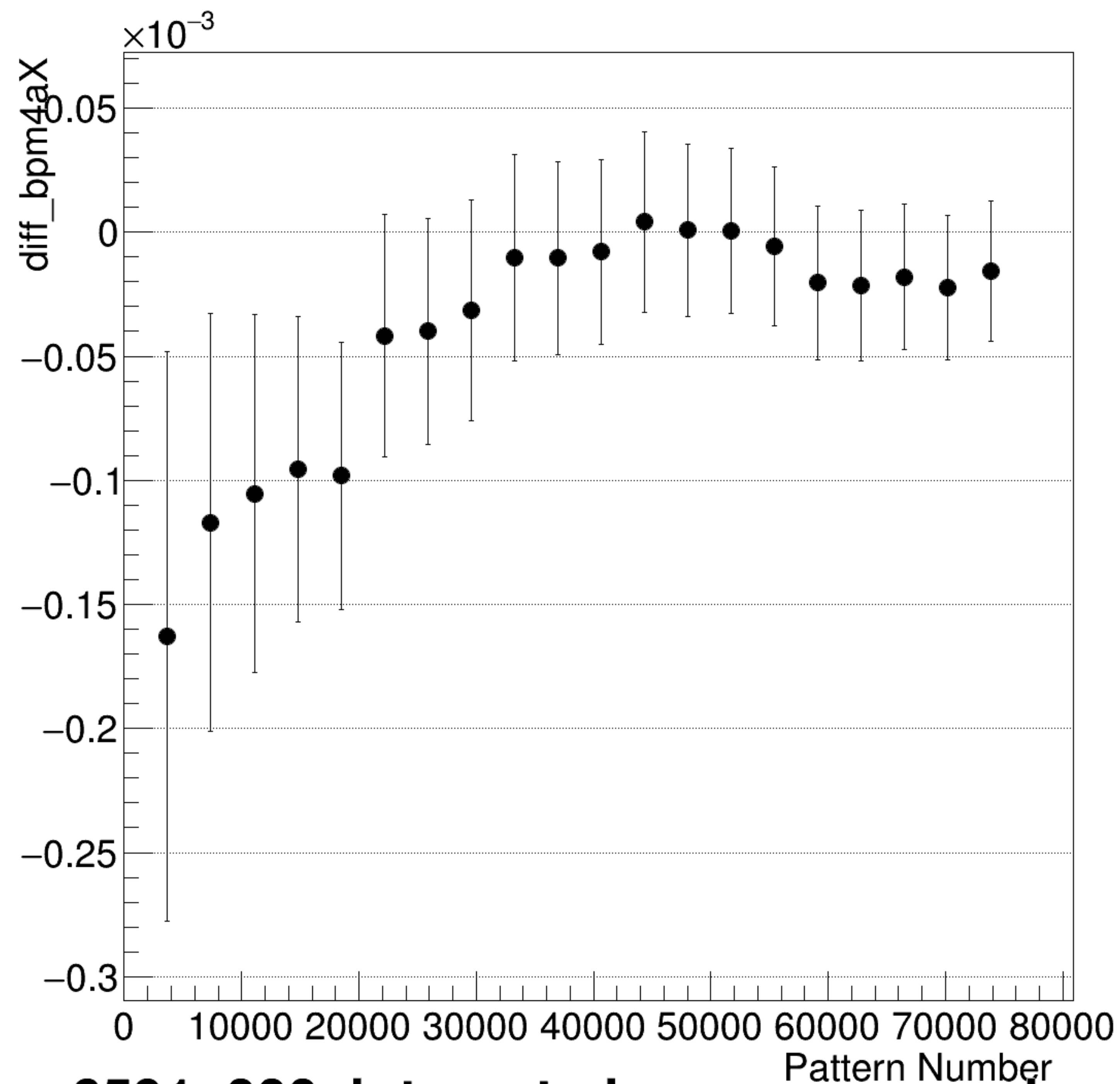
diff_bpm4aX Integrated Convergence
