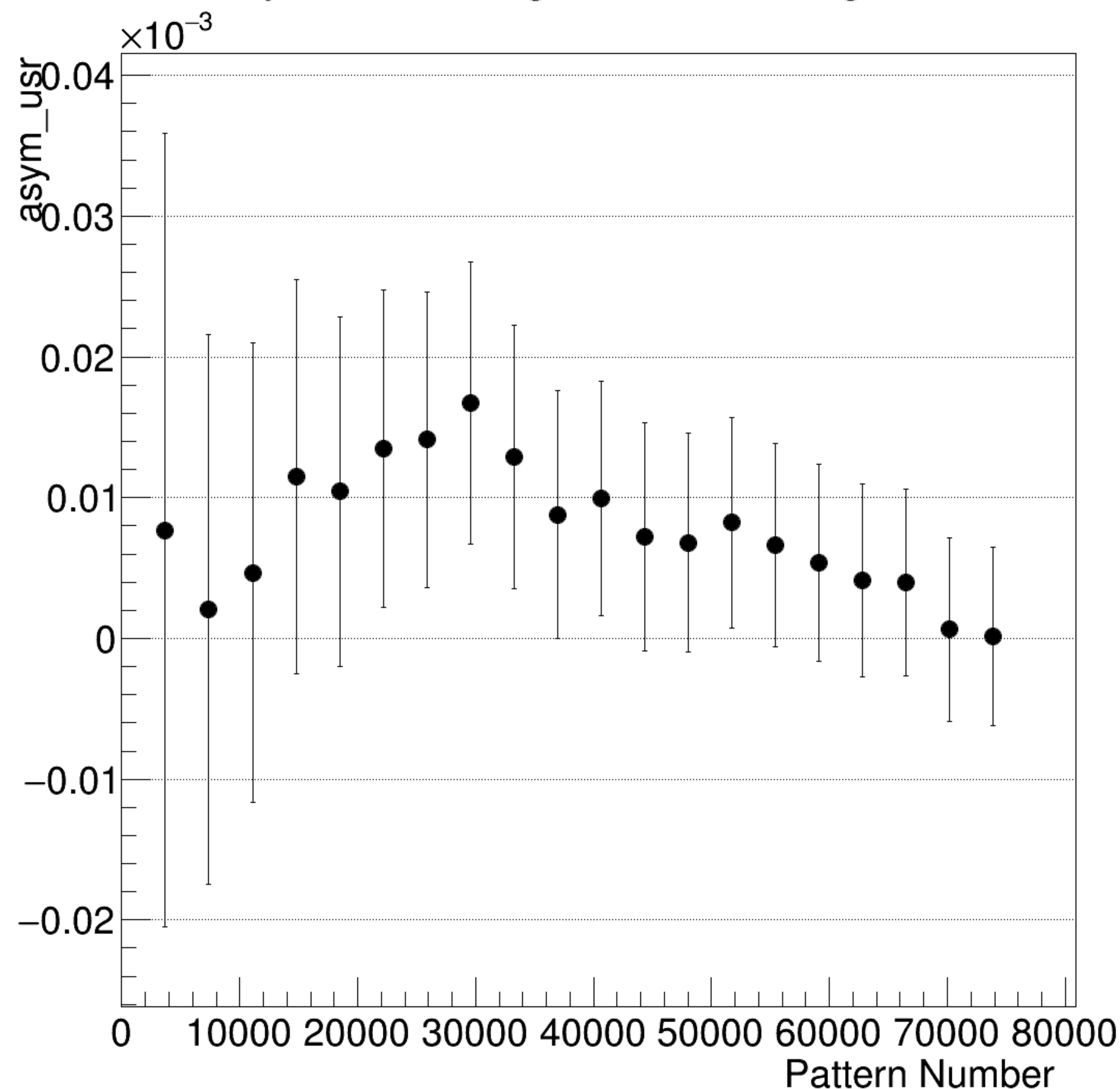
asym_usr Integrated Convergence
