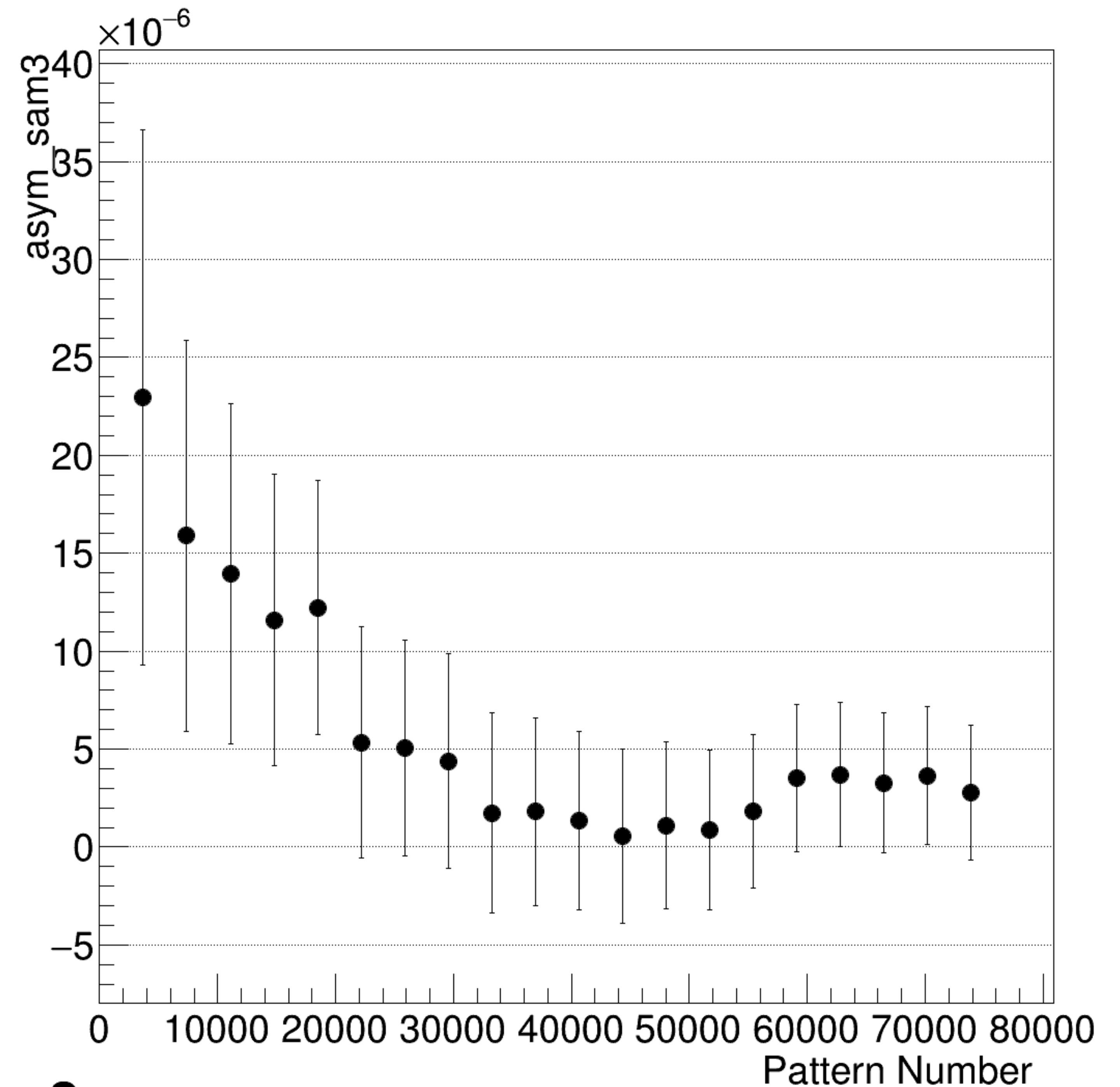
asym_sam3 Integrated Convergence
