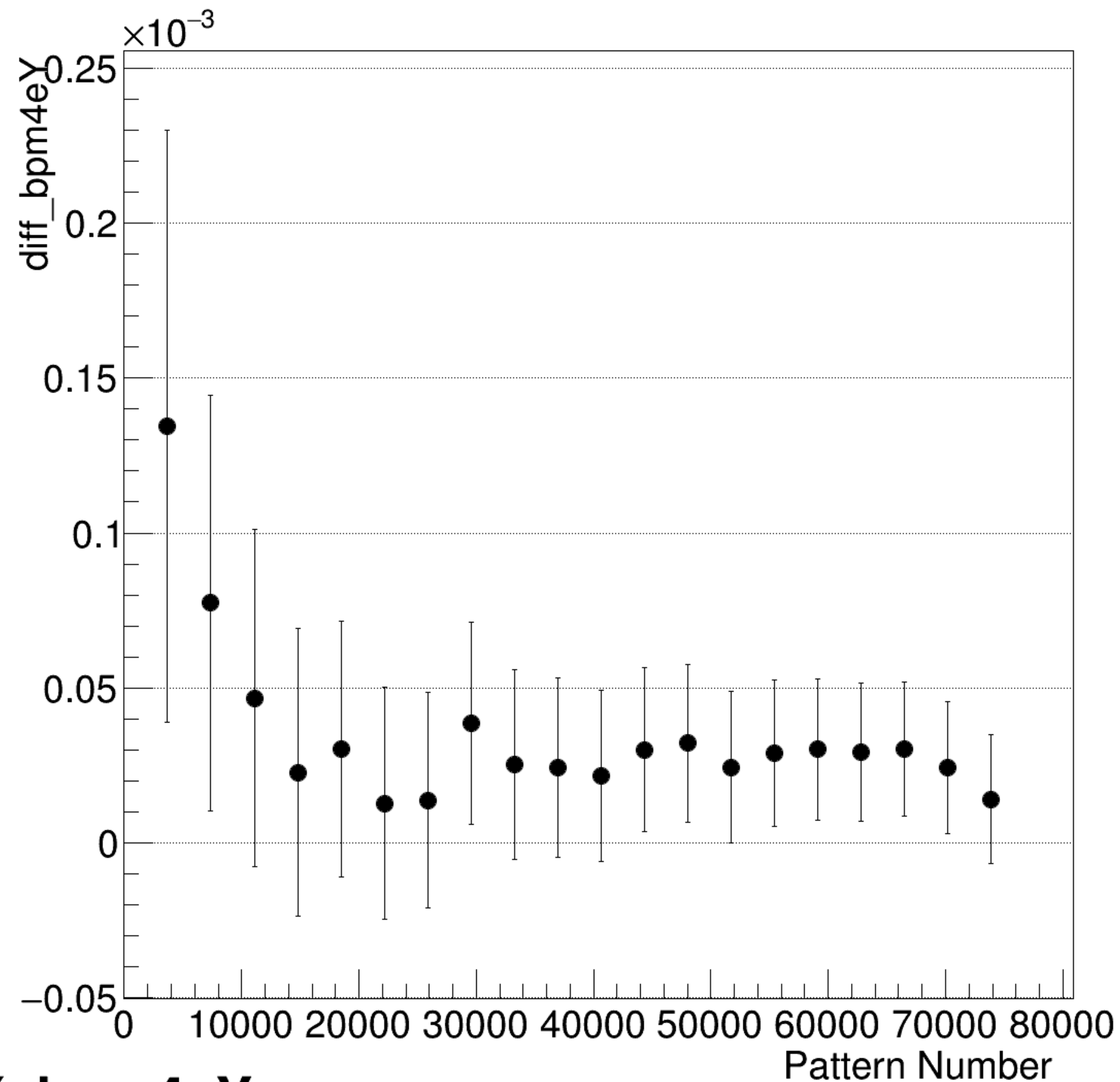
diff_bpm4eY Integrated Convergence
