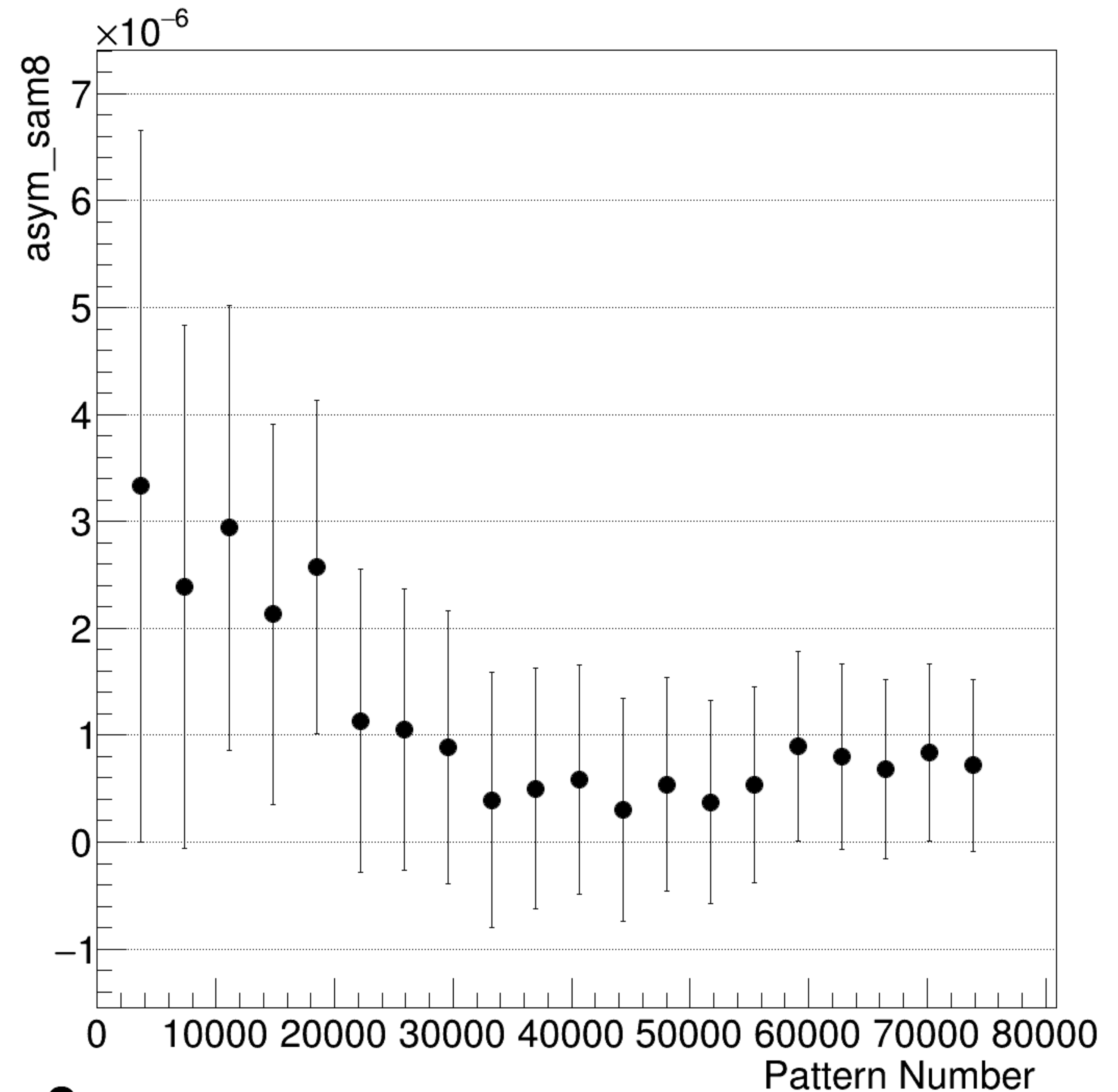
asym_sam8 Integrated Convergence
