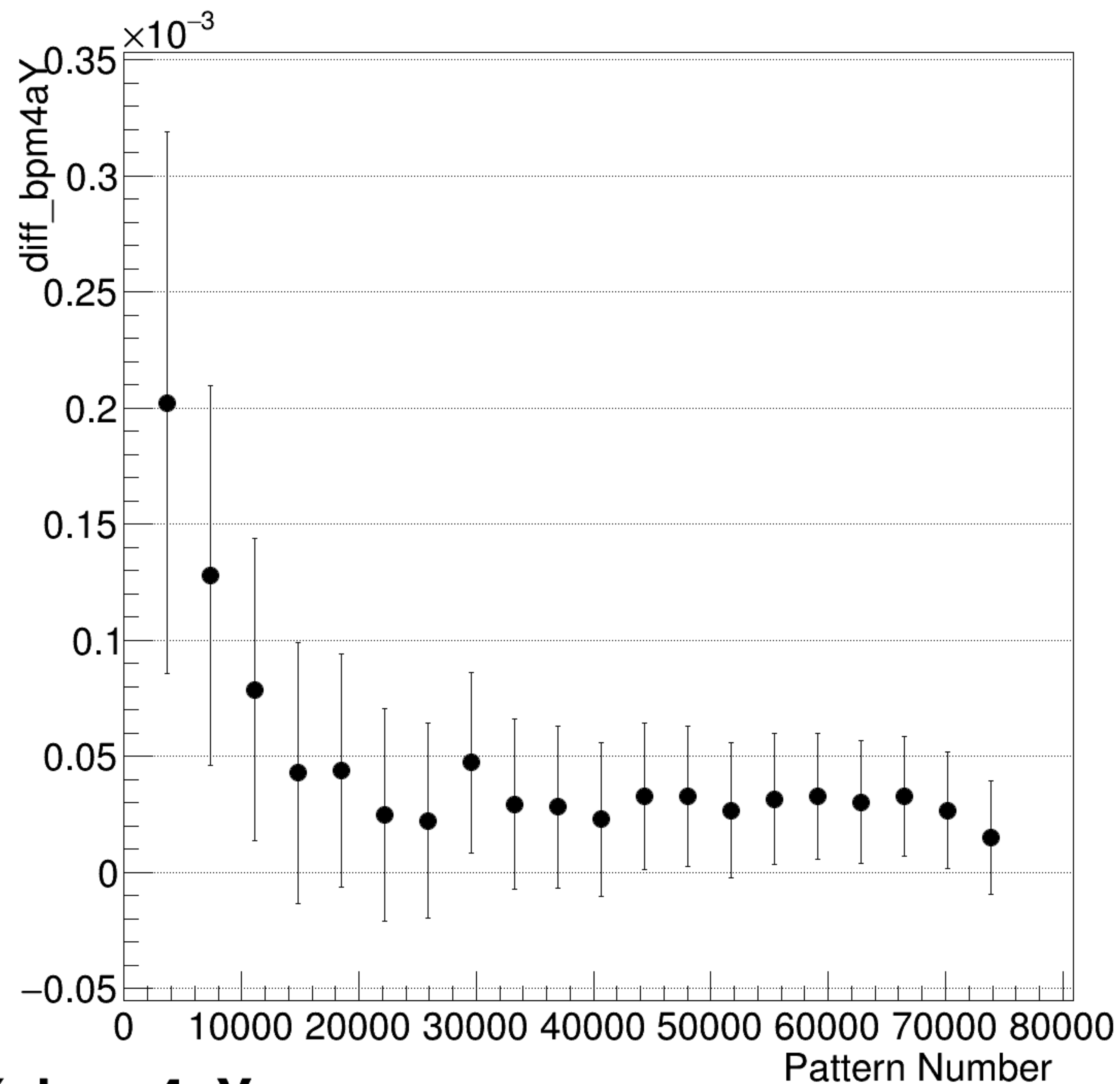
diff_bpm4aY Integrated Convergence
