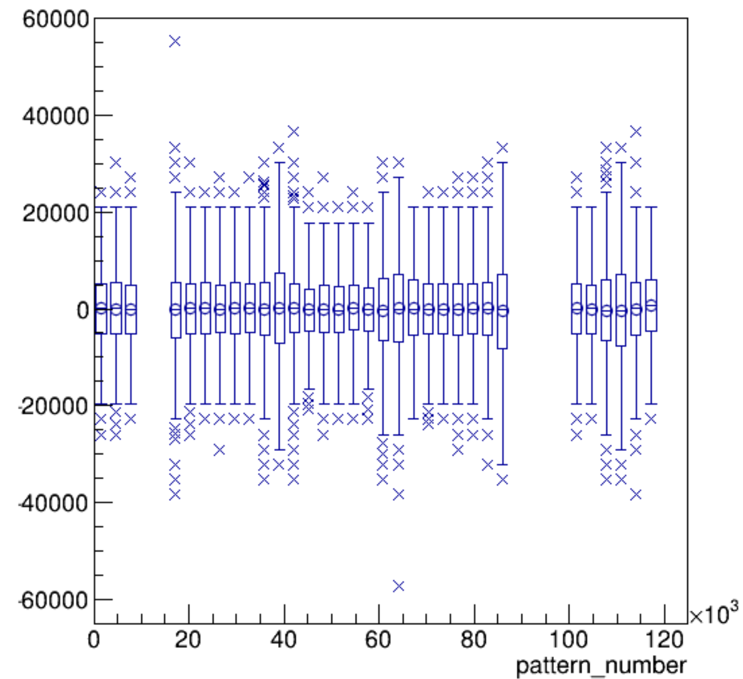
asym_atr2/ppm:pattern_number {ErrorFlag==0}
