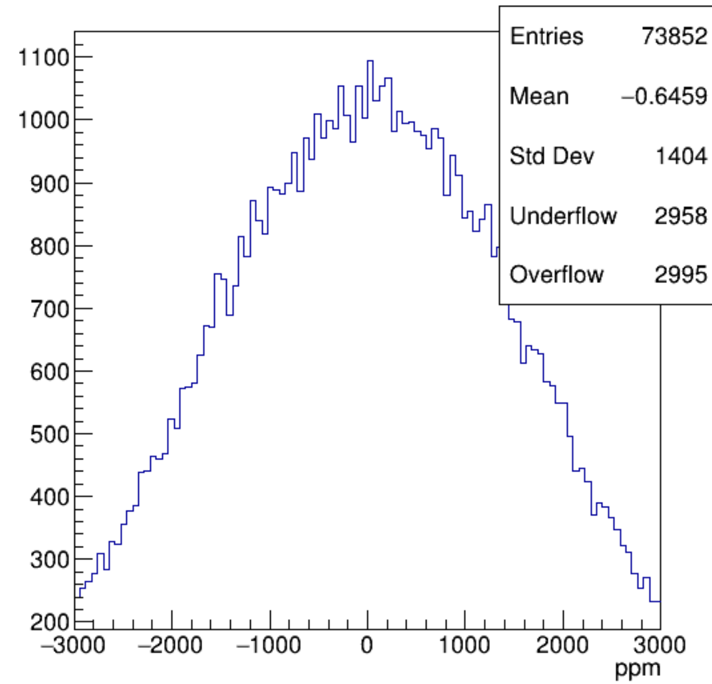
asym_usr
