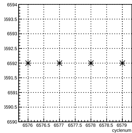
run:cyclenum {run == 6592}
