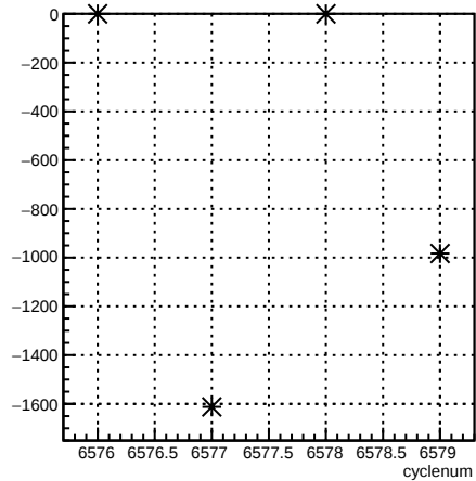
usl_coil6:cyclenum {run == 6592}
