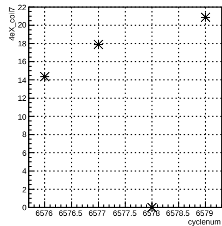
4eX_coil7:cyclenum {run == 6592}
