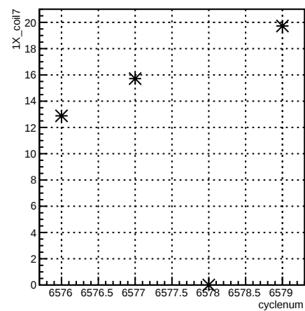
1X_coil7:cyclenum {run == 6592}
