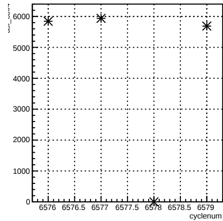
run:cyclenum {run == 6592}
