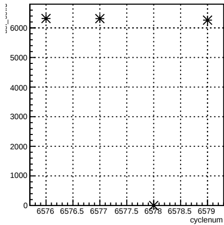
usl_coil7:cyclenum {run == 6592}
