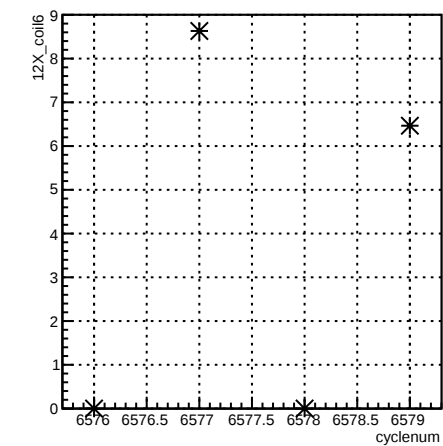
12X_coil6:cyclenum {run == 6592}
