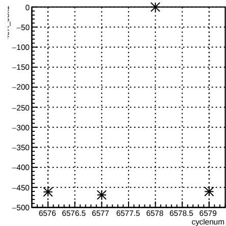
4eX_coil1:cyclenum {run == 6592}
