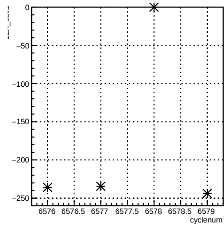
12X_coil1:cyclenum {run == 6592}
