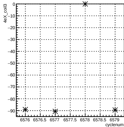
4eX_coil3:cyclenum {run == 6592}
