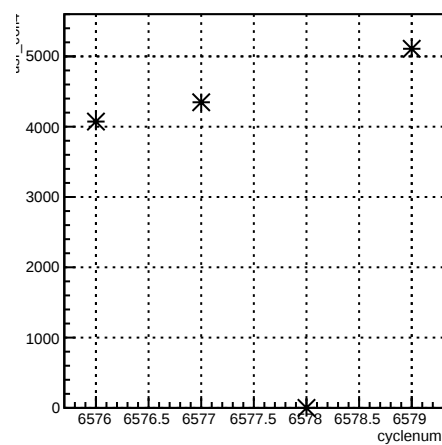
usr_coil4:cyclenum {run == 6592}
