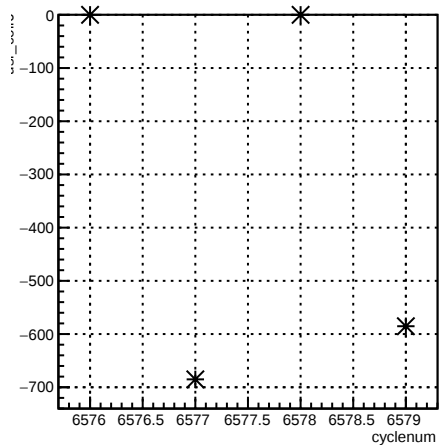
usr_coil6:cyclenum {run == 6592}
