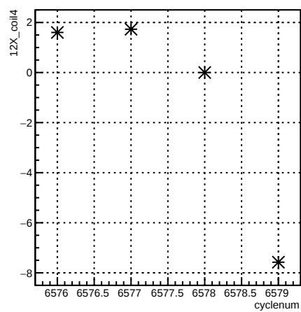
12X_coil4:cyclenum {run == 6592}
