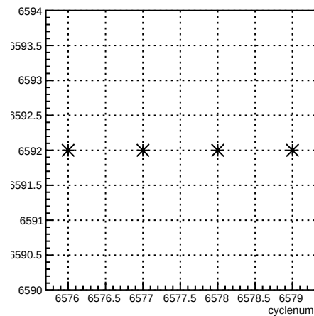
run:cyclenum {run == 6592}
