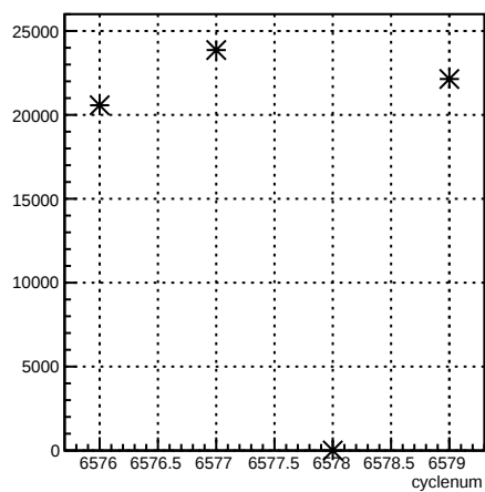
usl_coil7:cyclenum {run == 6592}
