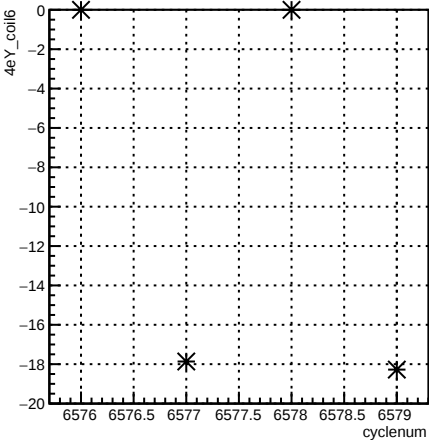
4eY_coil6:cyclenum {run == 6592}
