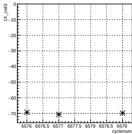
1X_coil3:cyclenum {run == 6592}
