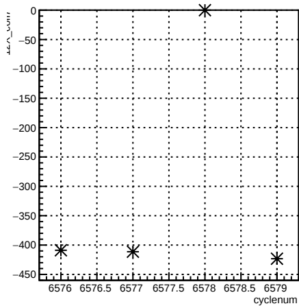
12X_coil7:cyclenum {run == 6592}
