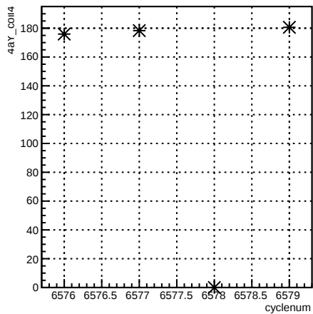
4eY_coil4:cyclenum {run == 6592}
