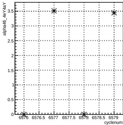
run:cyclenum {run == 6592}
