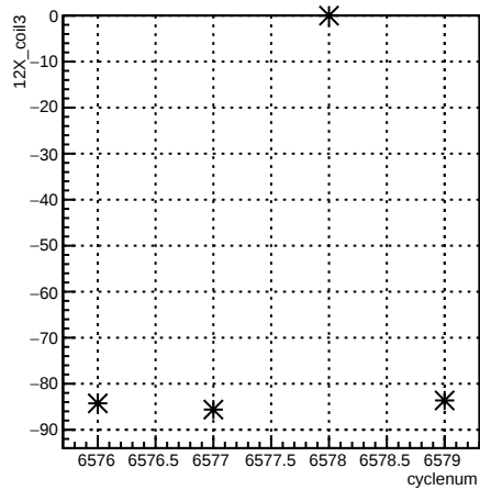
12X_coil3:cyclenum {run == 6592}
