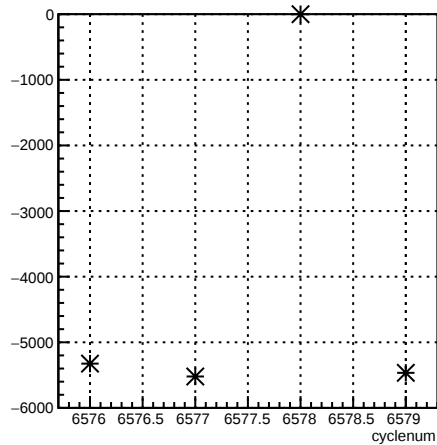
usr_coil3:cyclenum {run == 6592}
