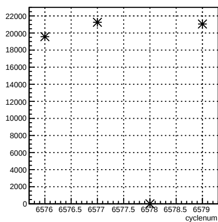
usr_coil7:cyclenum {run == 6592}
