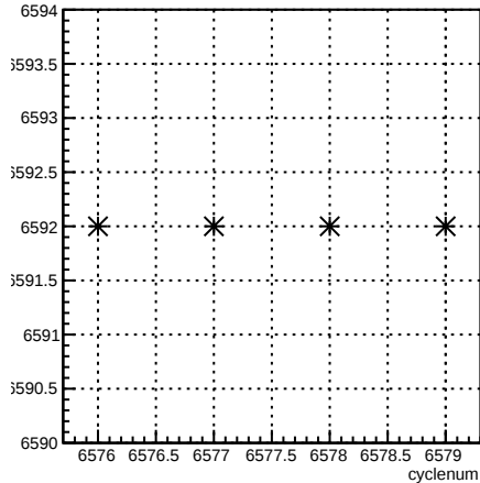
run:cyclenum {run == 6592}
