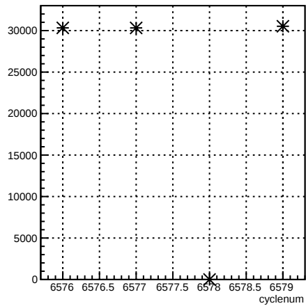
usl_coil6:cyclenum {run == 6592}
