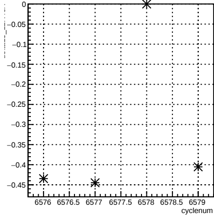
segment:cyclenum {run == 6592}
