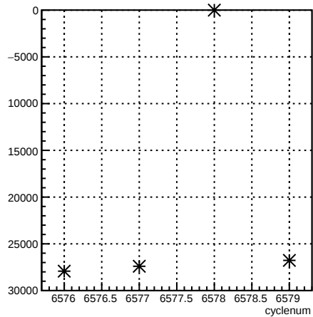
usr_coil1:cyclenum {run == 6592}
