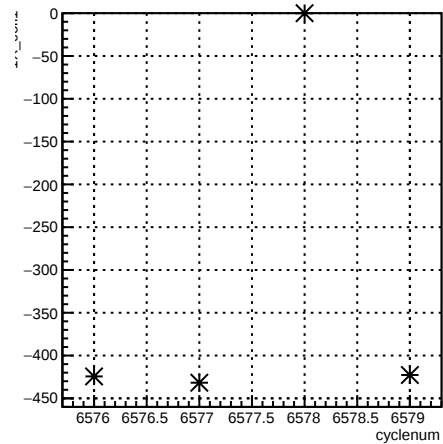
1X_coil1:cyclenum {run == 6592}
