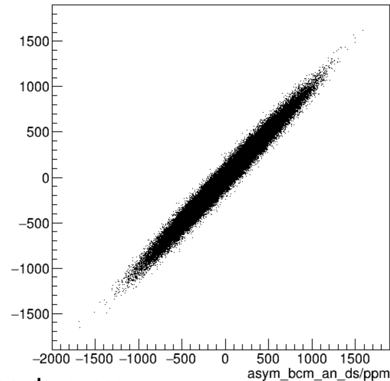
run6592_000_asym_bcm_dg_us_vs_asym_bcm_an_ds_pr.png
