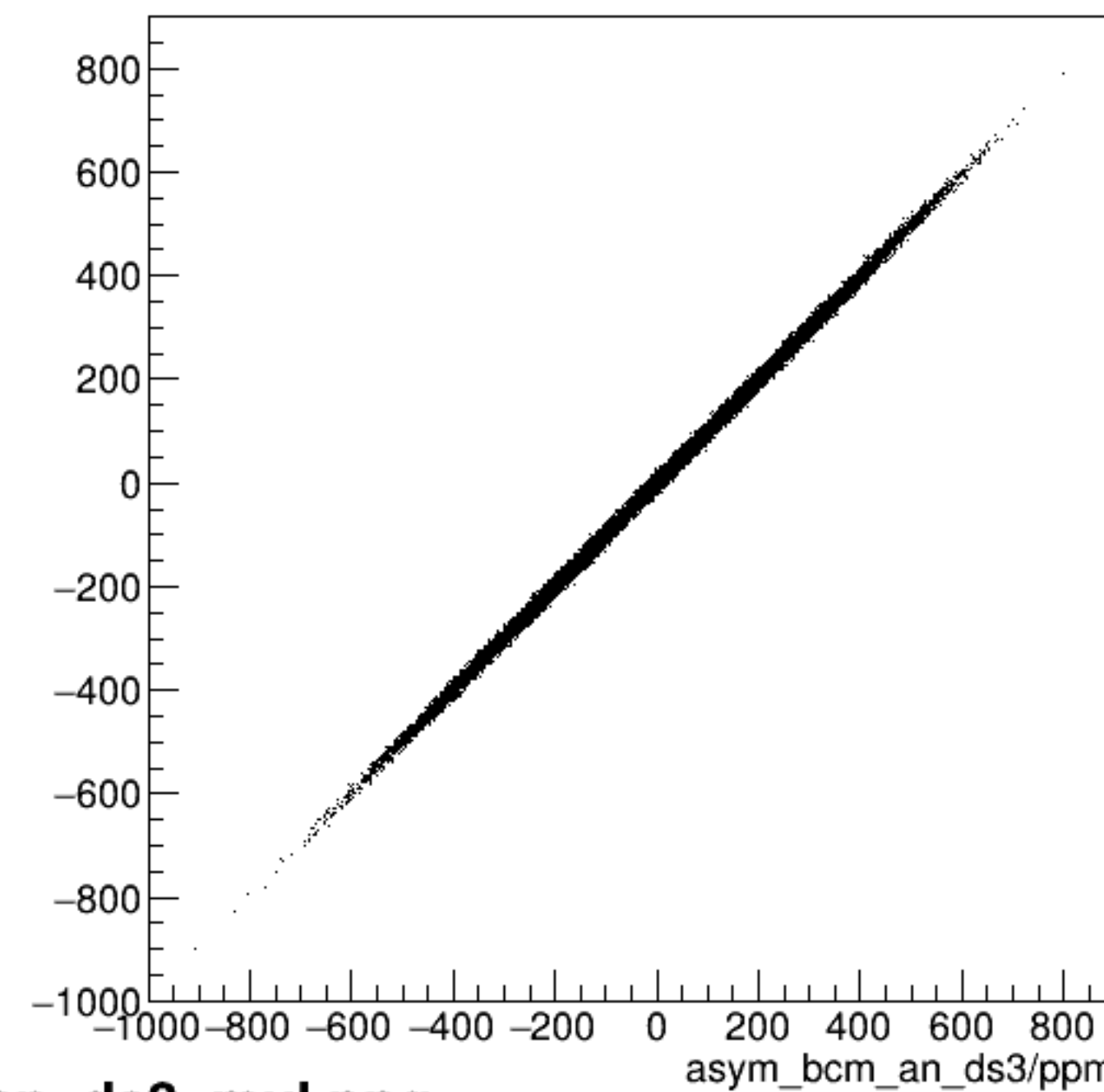
run6592_000_asym_bcm_an_ds_vs_asym_bcm_an_ds3_mul.png
