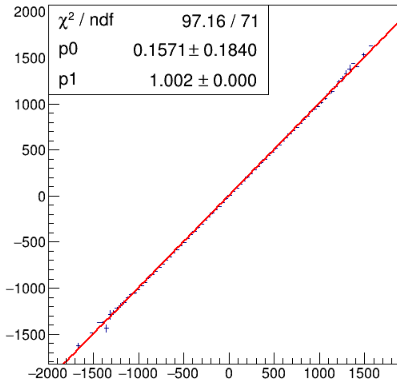
run6592_000_asym_bcm_dg_us_vs_asym_bcm_an_ds_pr.png
