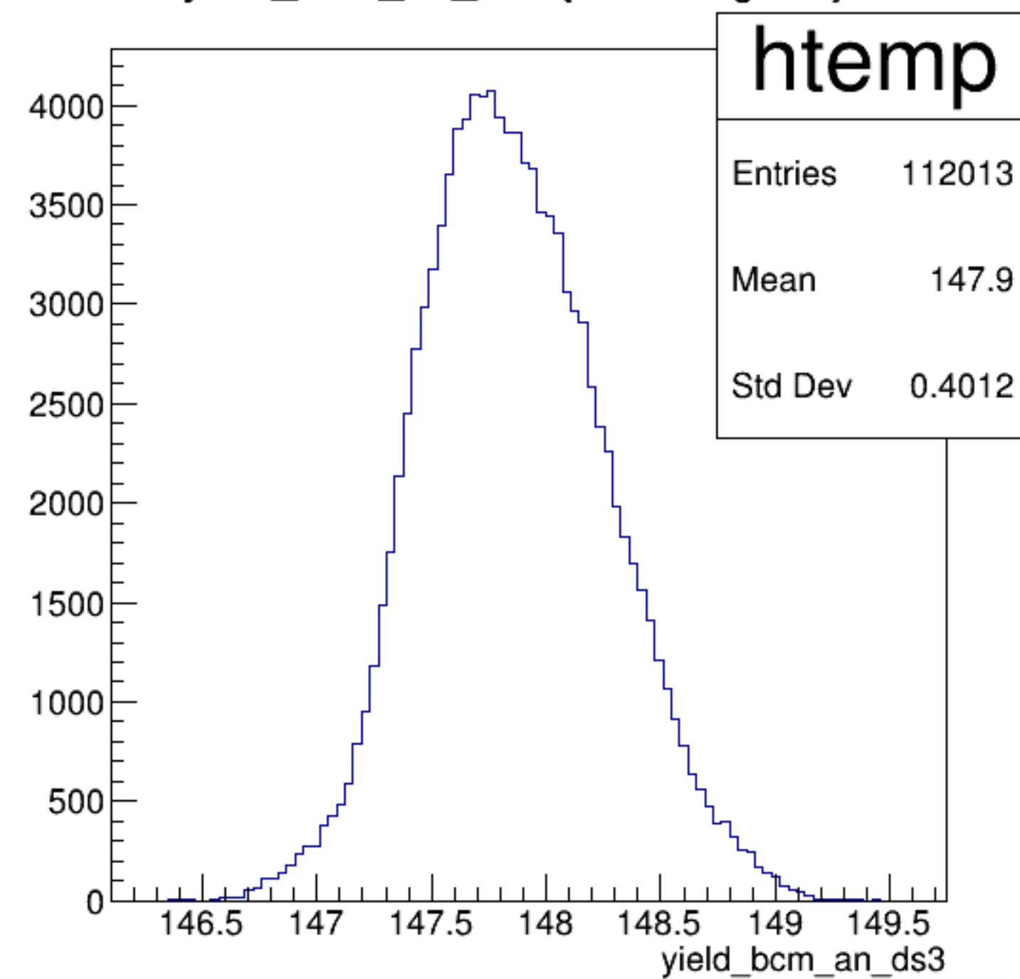
yield_bcm_an_ds3 {ErrorFlag==0}
