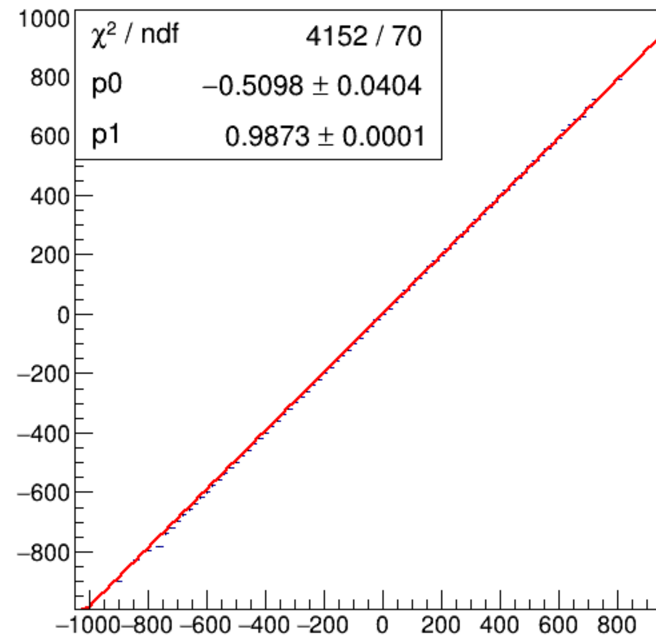
run6592_000_asym_bcm_an_ds_vs_asym_bcm_an_ds3_mul.png
