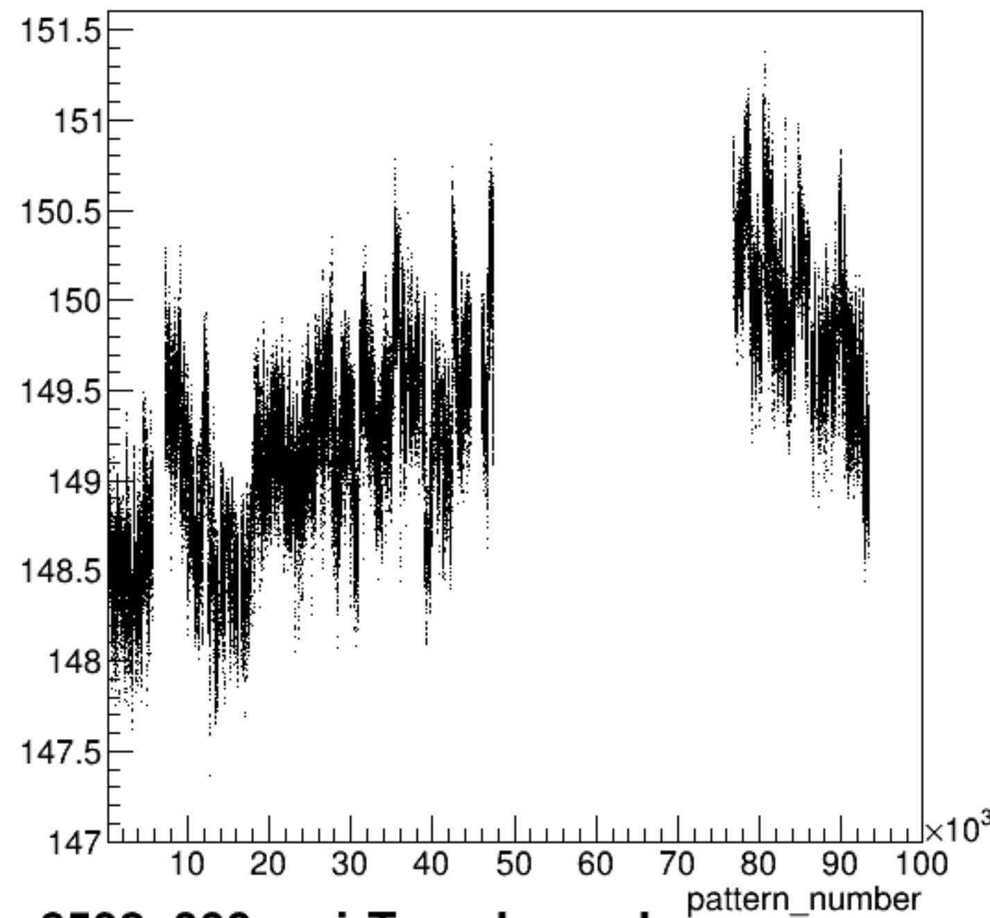
yield_bcm_dg_us:pattern_number {ErrorFlag==0}
