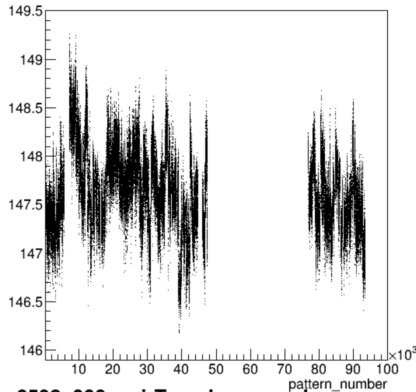
yield_bcm_an_ds:pattern_number {ErrorFlag==0}
