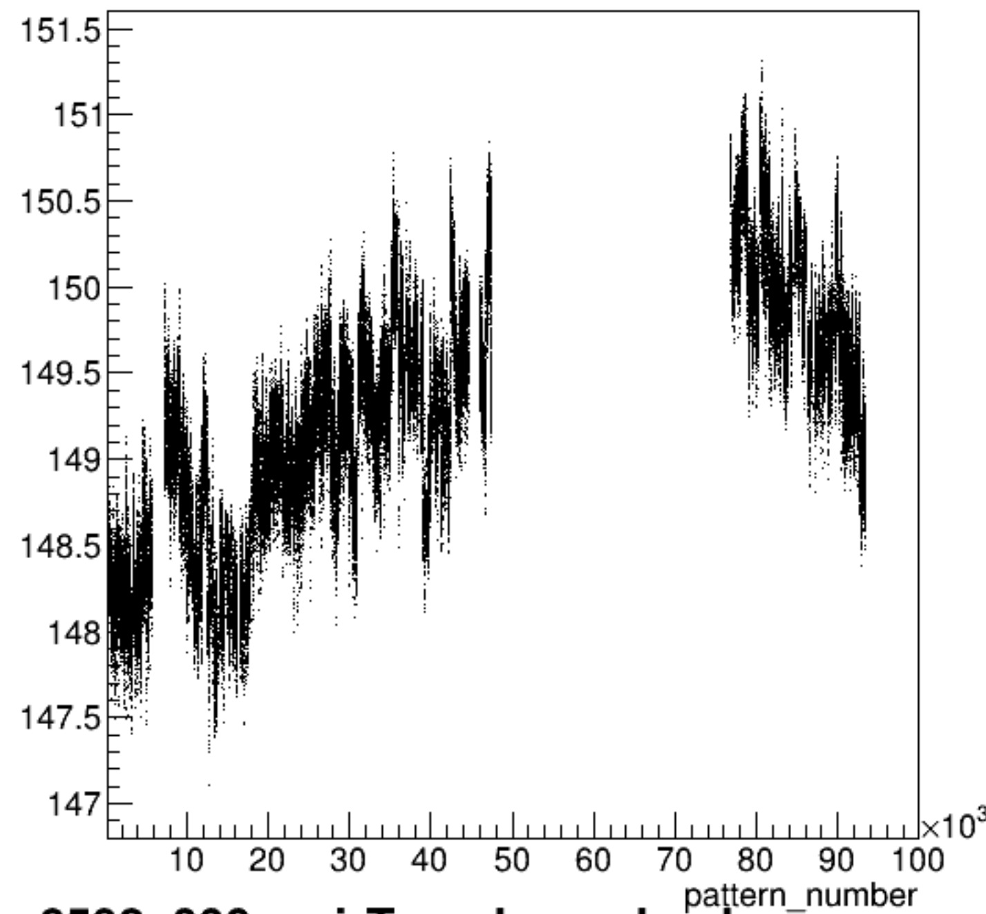
yield_bcm_dg_ds:pattern_number {ErrorFlag==0}
