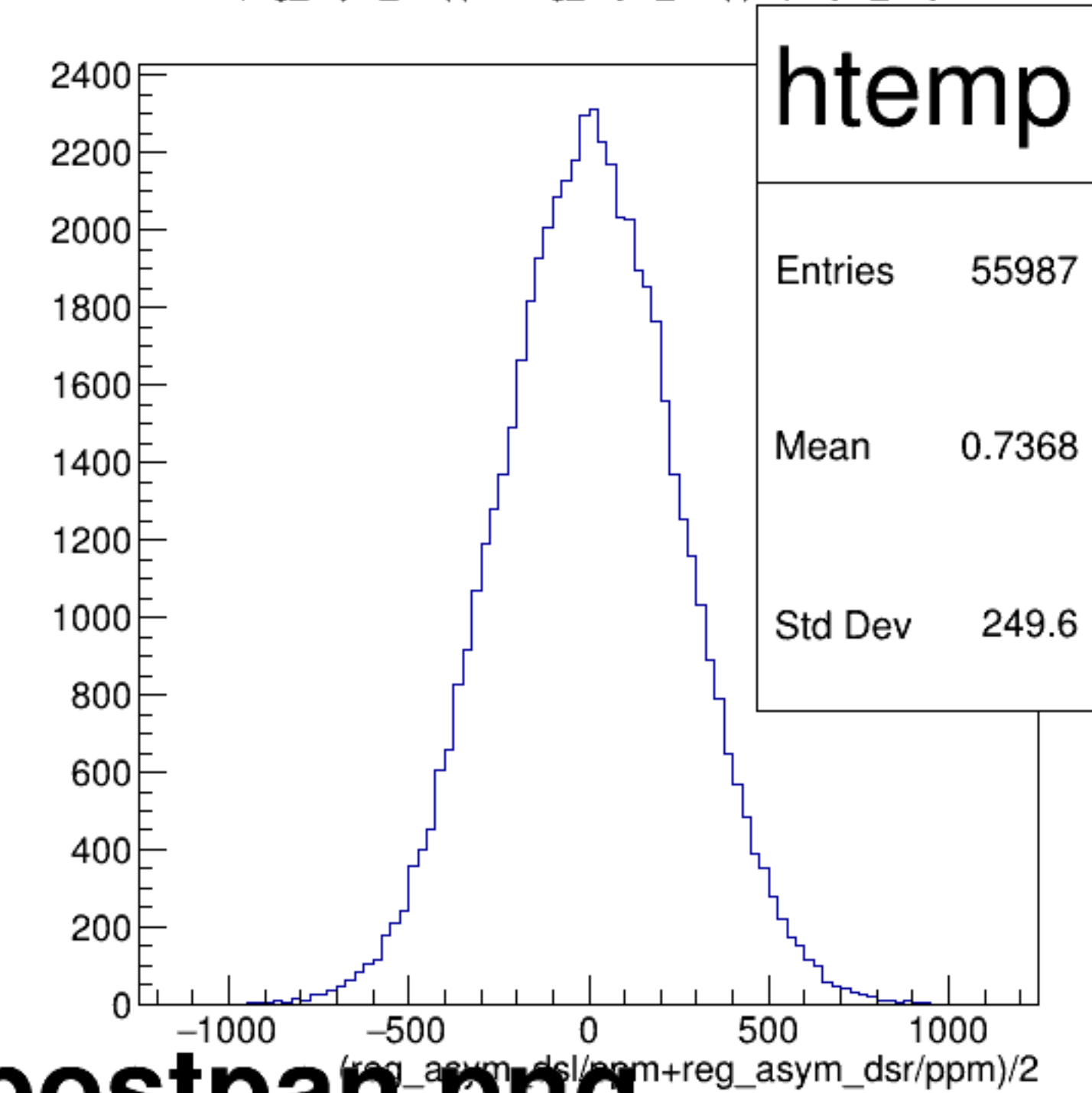
(reg_asym_dsl/ppm+reg_asym_dsr/ppm)/2 {ok_cut}
