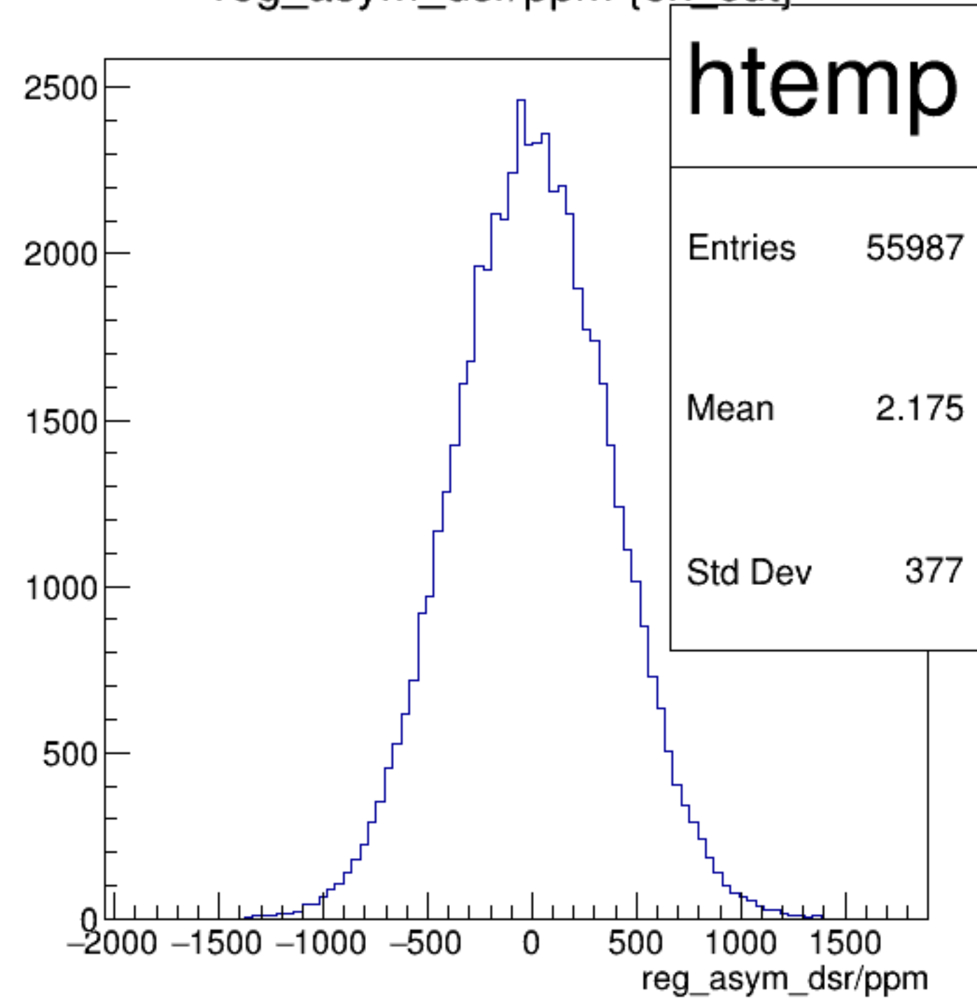
reg_asym_dsr/ppm {ok_cut}
