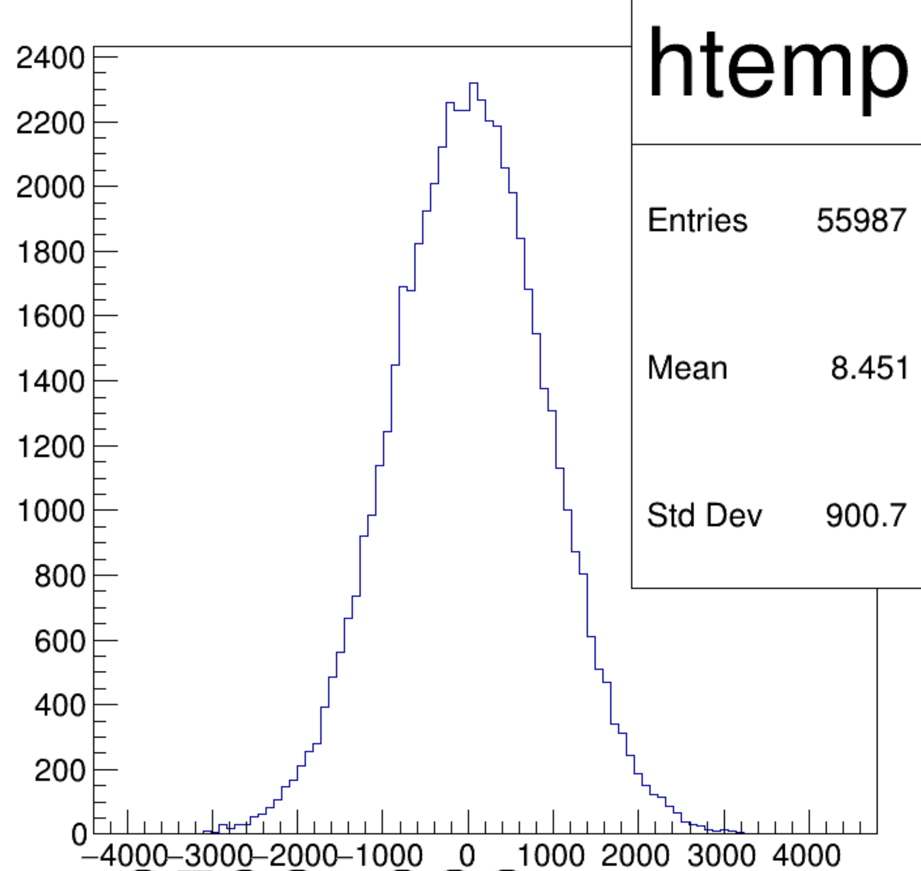
(asym_usl/ppm-asym_usr/ppm)/2 {ok_cut}
