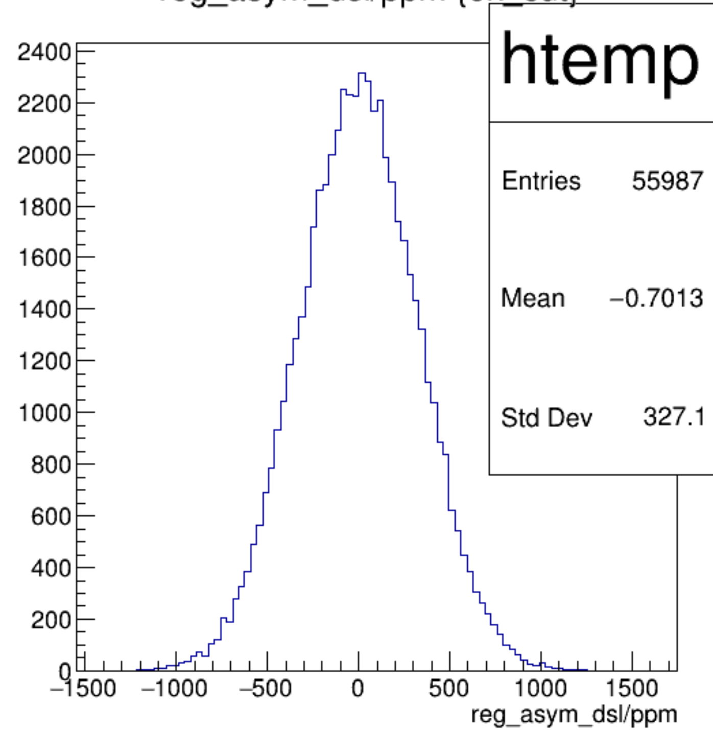
reg_asym_dsl/ppm {ok_cut}
