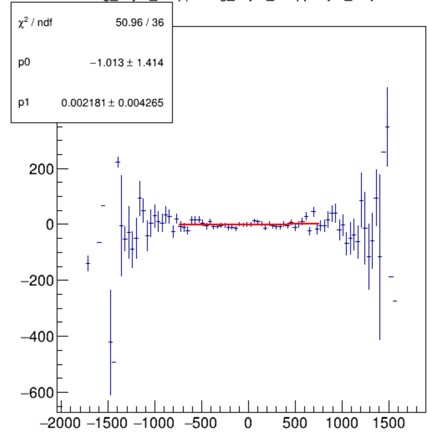
reg_asym_dsl/ppm:reg_asym_dsr/ppm {ok_cut}
