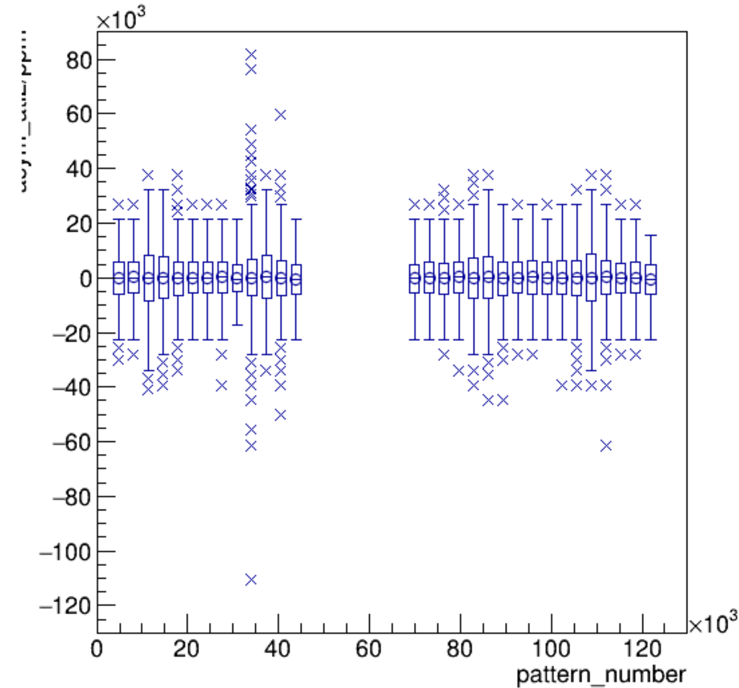
asym_atl2/ppm:pattern_number {ErrorFlag==0}
