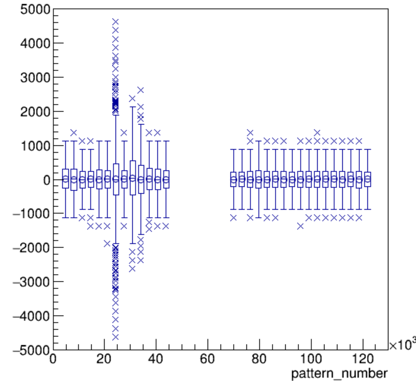
asym_bcm_an_us/ppm:pattern_number {ErrorFlag==0}
