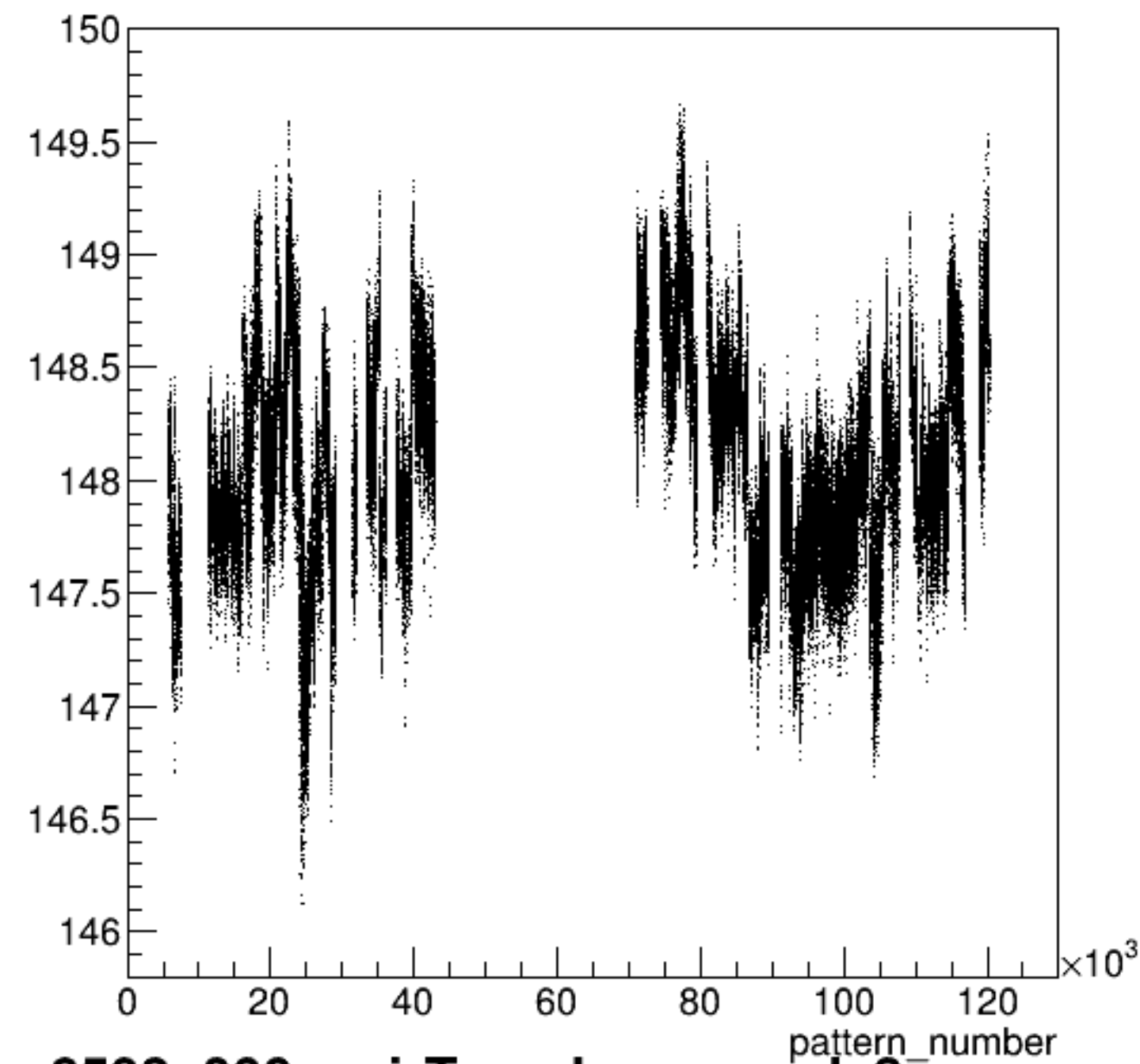
yield_bcm_an_ds3:pattern_number {ErrorFlag==0}
