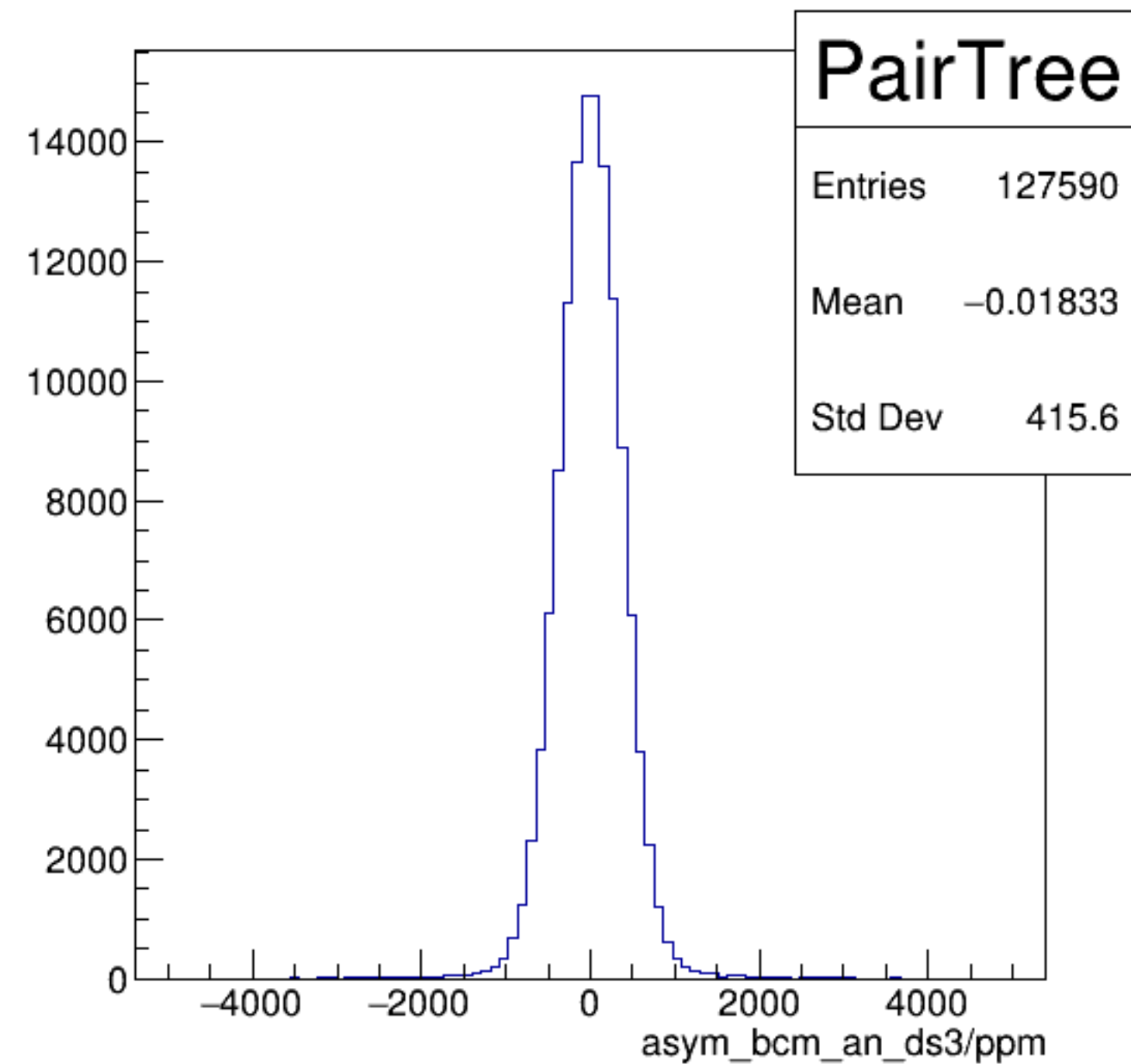
asym_bcm_an_ds3/ppm {ErrorFlag==0}
