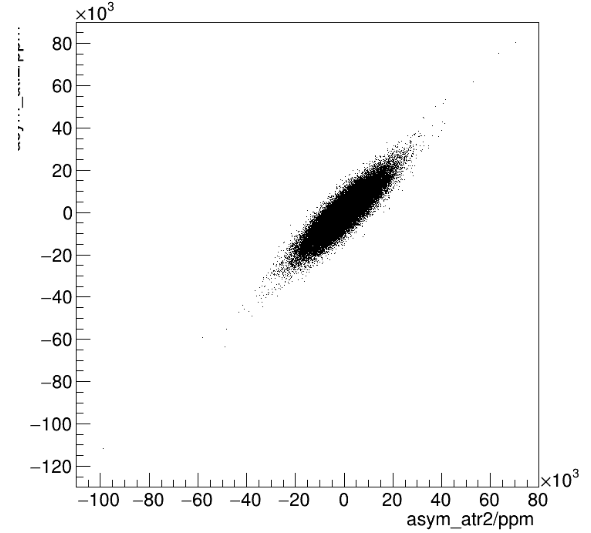
asym_atl2/ppm:asym_atr2/ppm {ok_cut}
