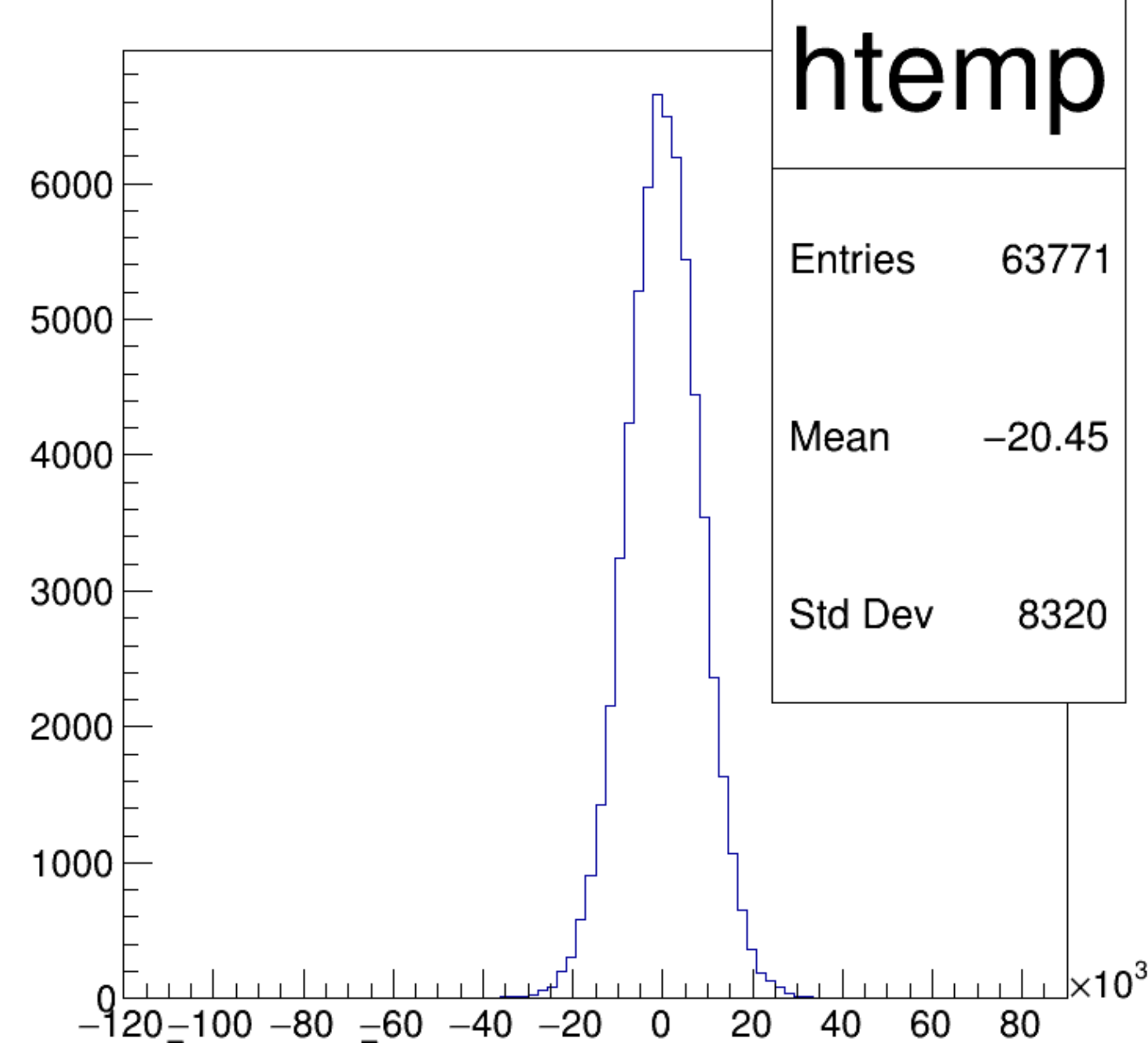
(asym_atl2/ppm+asym_atr2/ppm)/2 {ok_cut}
