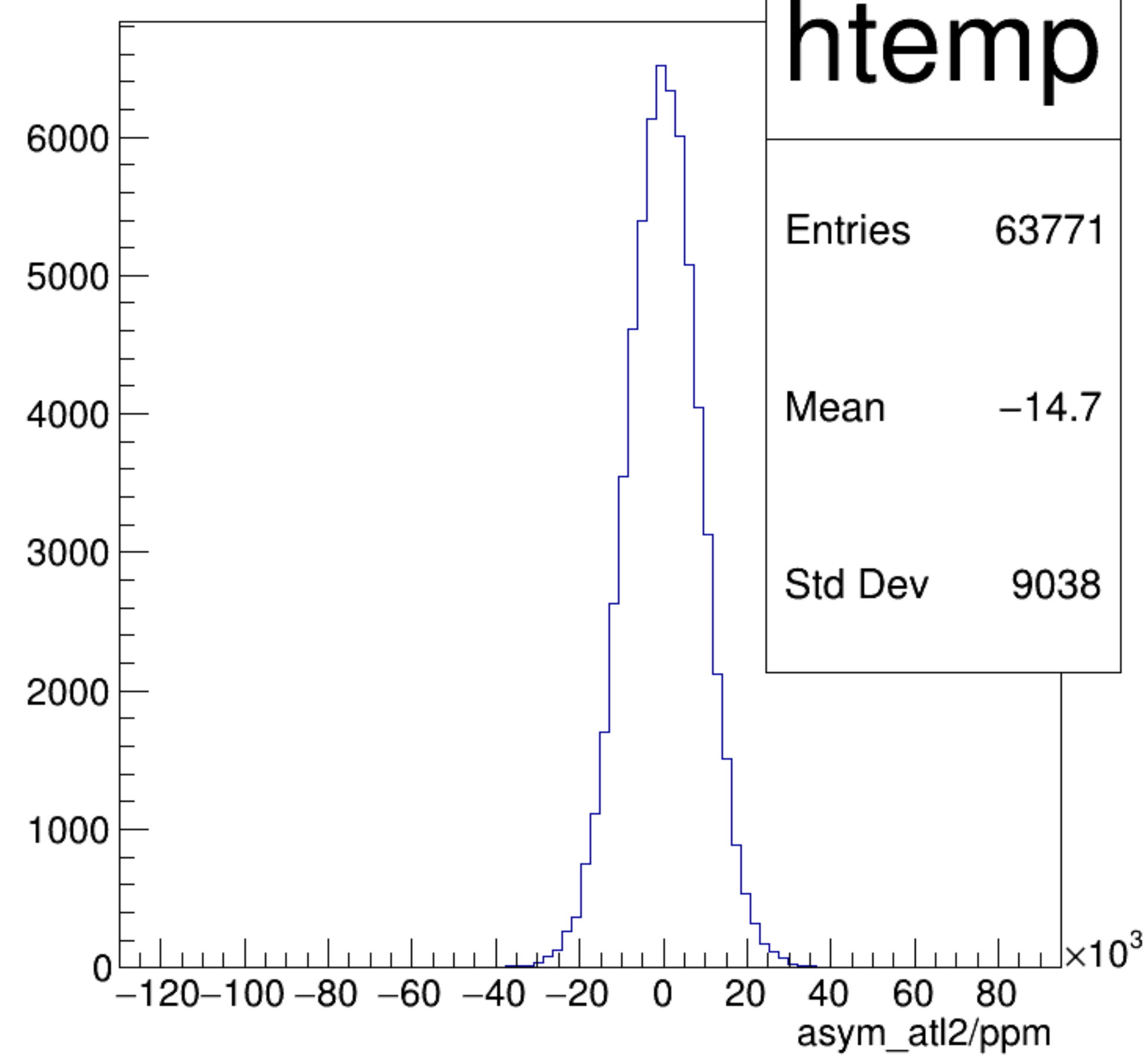
asym_atl2/ppm {ok_cut}
