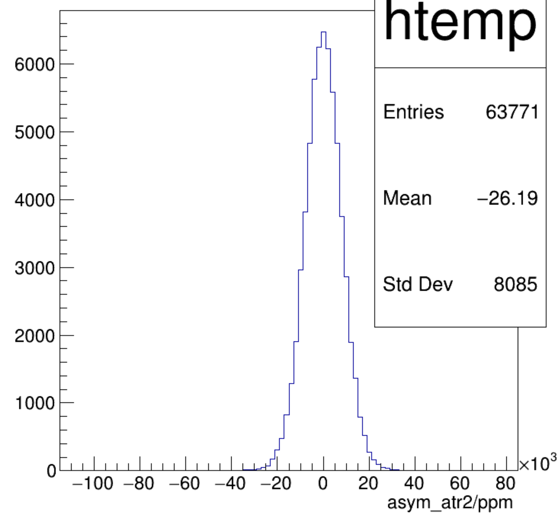
asym_atr2/ppm {ok_cut}
