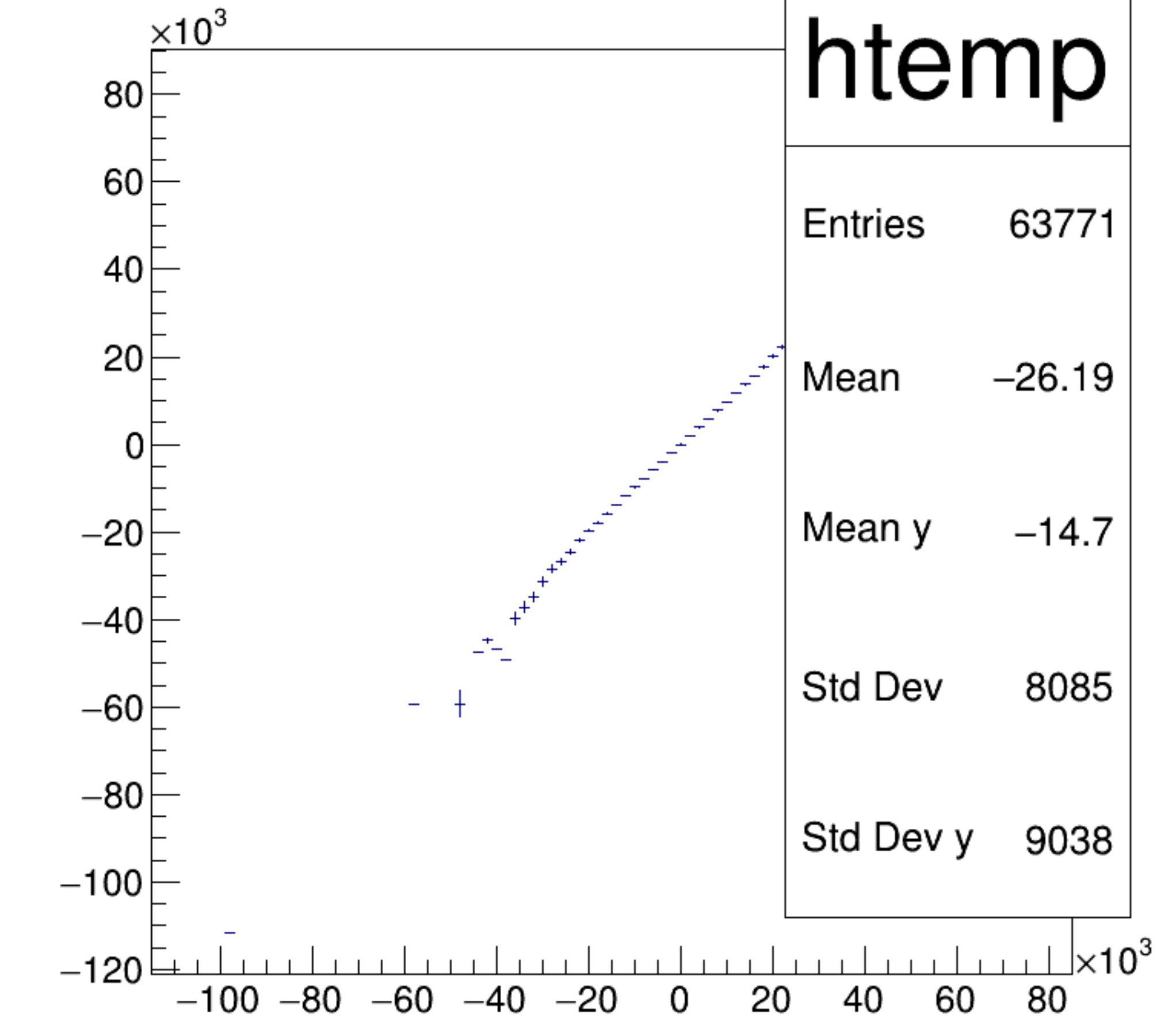
asym_atl2/ppm:asym_atr2/ppm {ok_cut}
