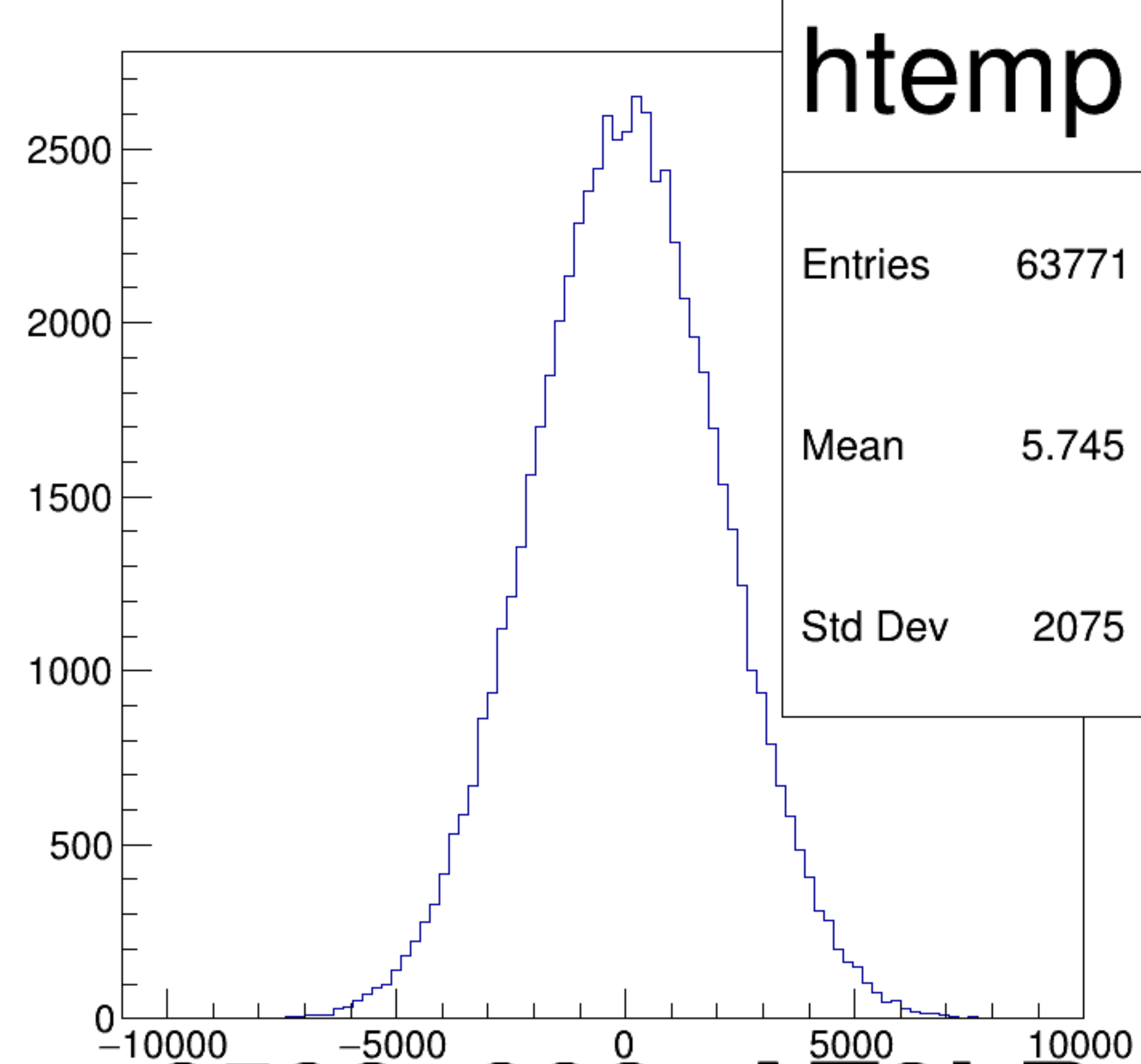
(asym_atl2/ppm-asym_atr2/ppm)/2 {ok_cut}
