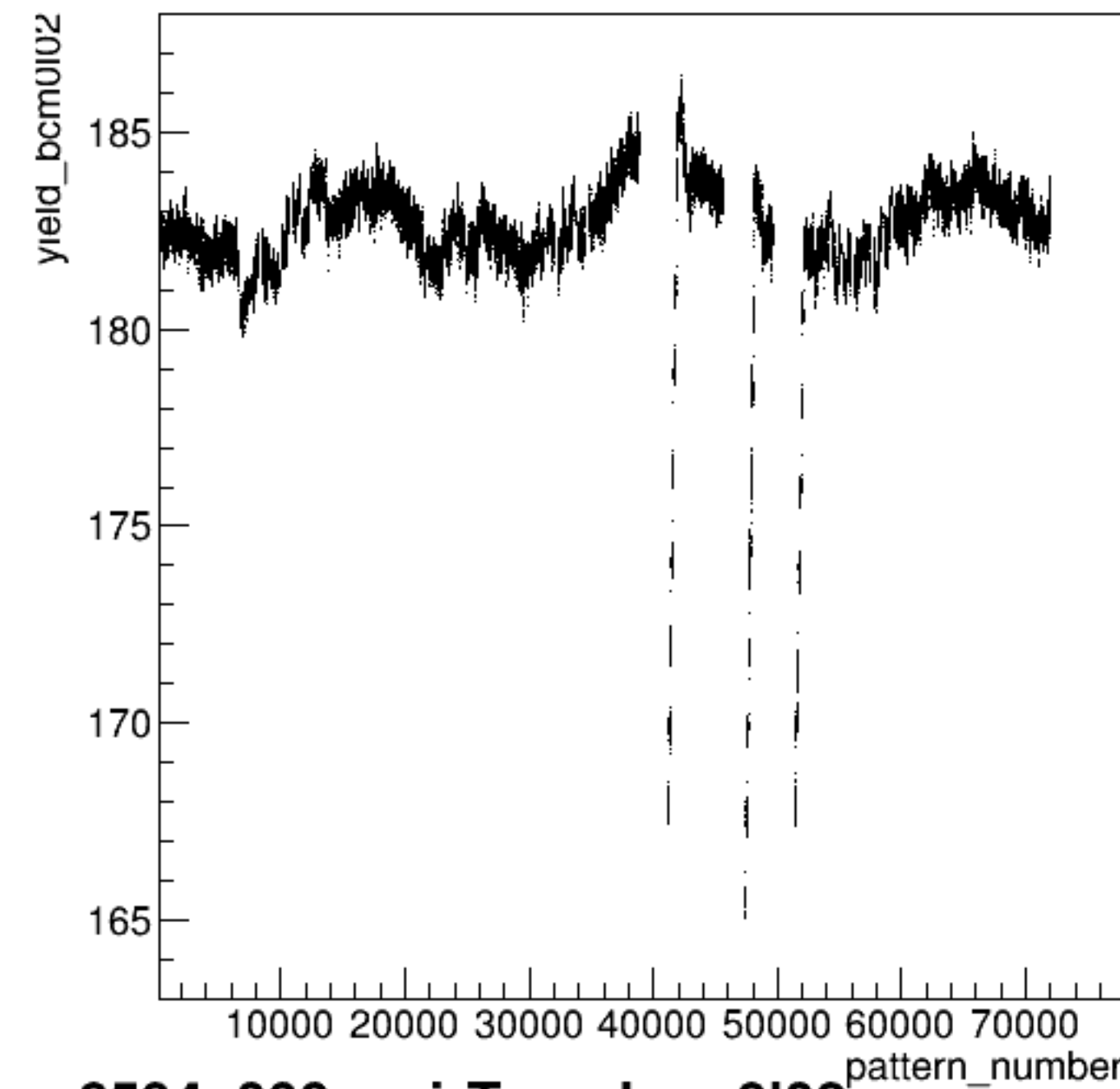
yield_bcm0l02:pattern_number {ErrorFlag==0}
