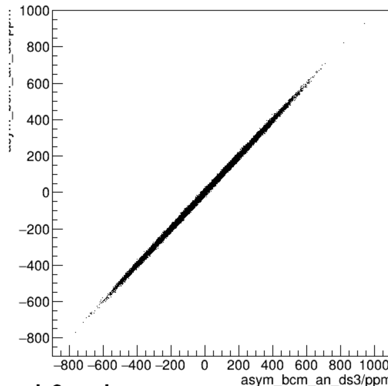
run6594_000_asym_bcm_an_ds_vs_asym_bcm_an_ds3_mul.png
