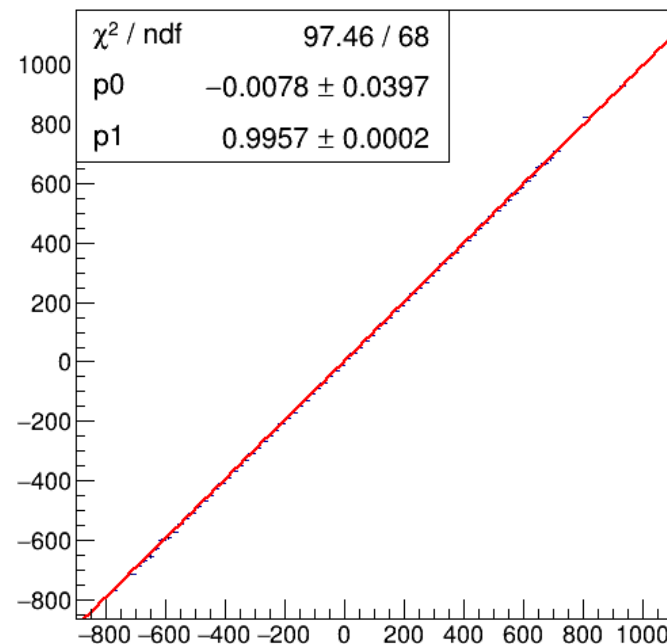
run6594_000_asym_bcm_an_ds_vs_asym_bcm_an_ds3_mul.png
