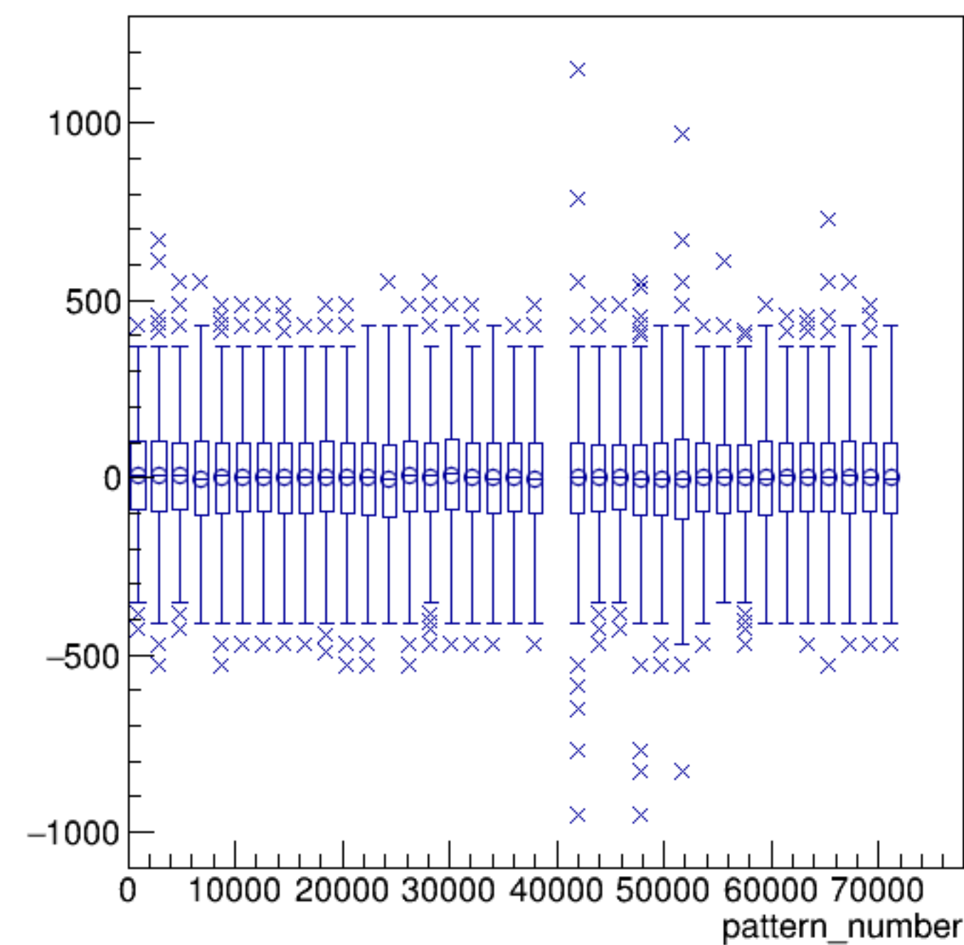
asym_bcm0l02/ppm:pattern_number {ErrorFlag==0}
