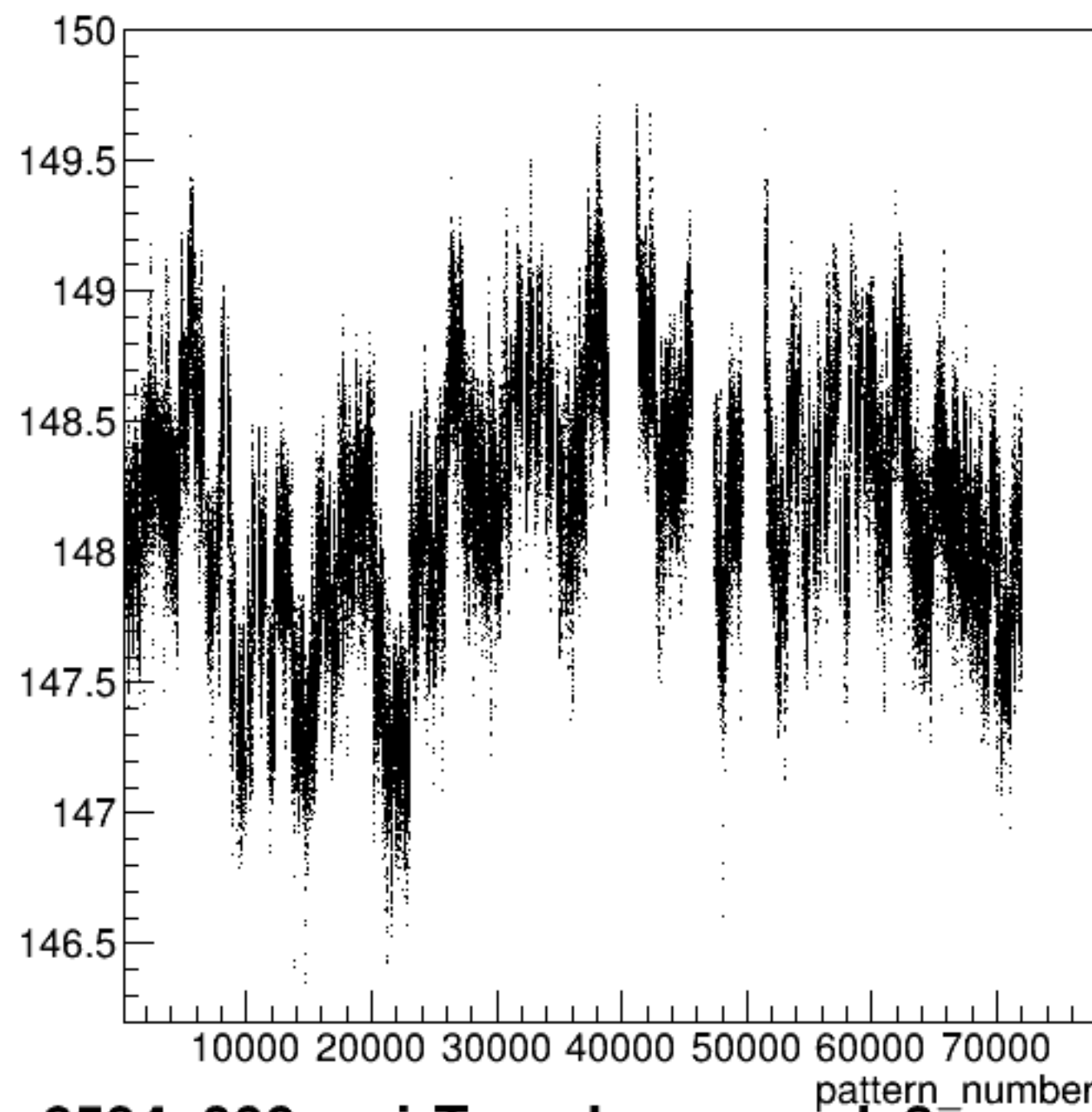
yield_bcm_an_ds3:pattern_number {ErrorFlag==0}
