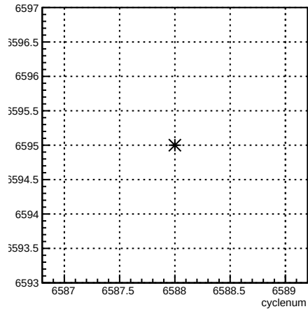
run:cyclenum {run == 6595}
