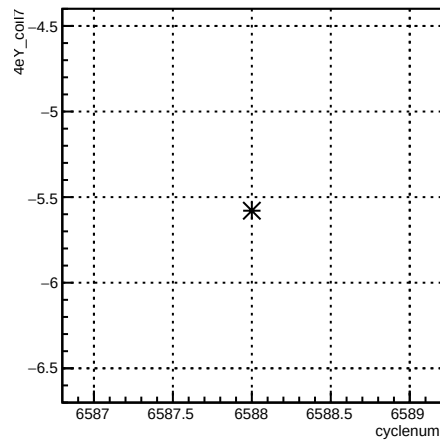
4eY_coil7:cyclenum {run == 6595}
