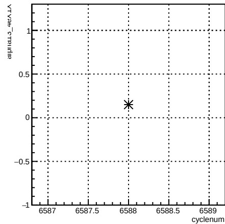
alpha13_4eX1X:cyclenum {run == 6595}
