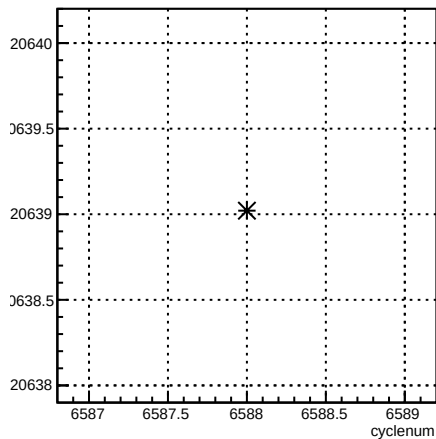
usr_coil7:cyclenum {run == 6595}
