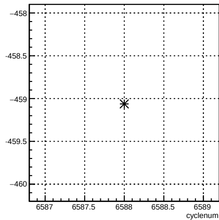
4eX_coil1:cyclenum {run == 6595}
