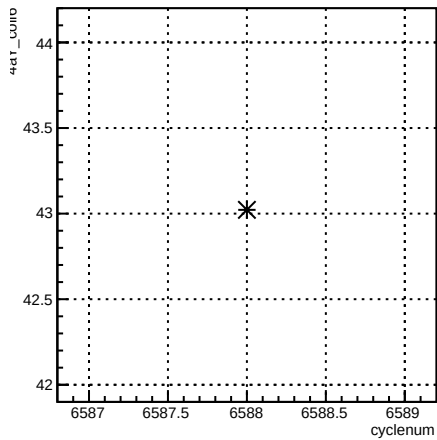
4eY_coil6:cyclenum {run == 6595}
