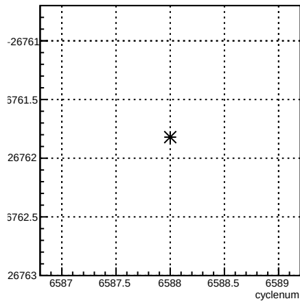
usr_coil6:cyclenum {run == 6595}
