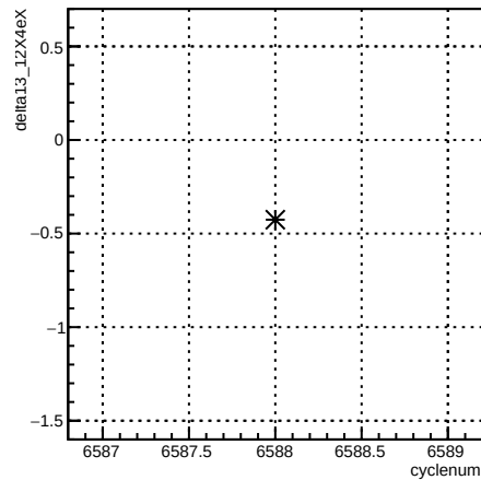
delta13_12X4eX:cyclenum {run == 6595}
