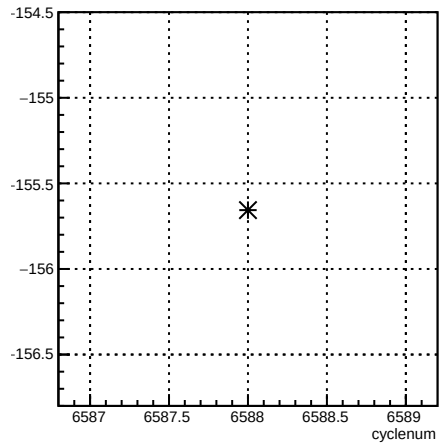
usr_1X:cyclenum {run == 6595}
