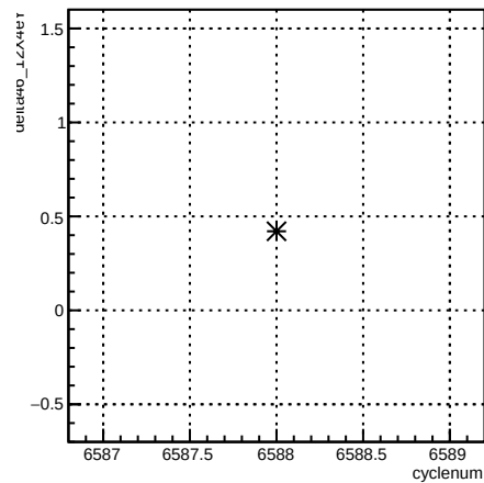
delta46_12X4eY:cyclenum {run == 6595}
