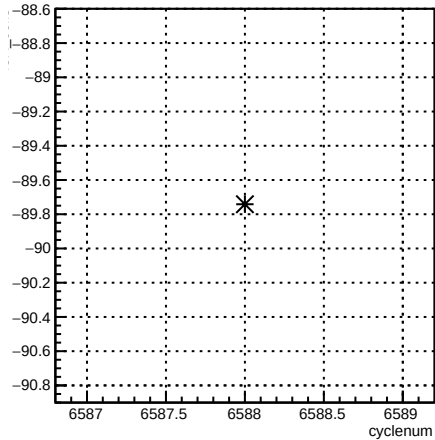
4eX_coil3:cyclenum {run == 6595}
