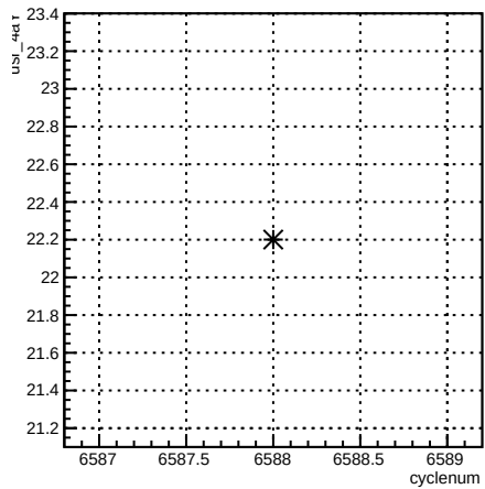
usr_4aY:cyclenum {run == 6595}
