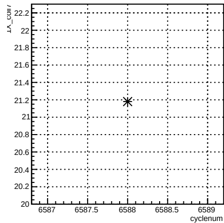
4eX_coil7:cyclenum {run == 6595}
