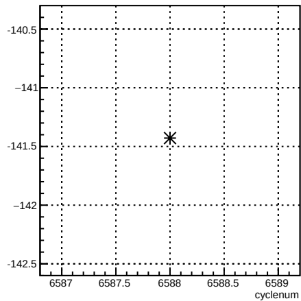
usl_4eY:cyclenum {run == 6595}
