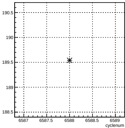
4eY_coil4:cyclenum {run == 6595}
