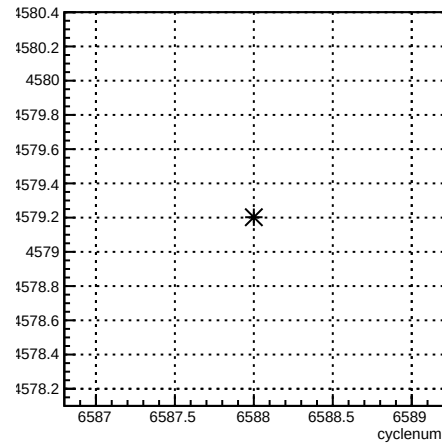
usr_coil4:cyclenum {run == 6595}
