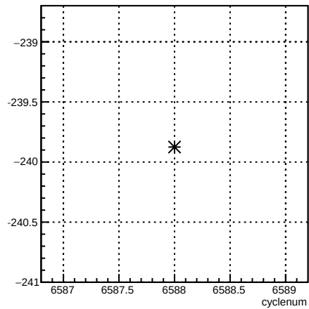
12X_coil6:cyclenum {run == 6595}
