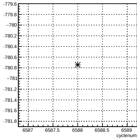
usr_coil6:cyclenum {run == 6595}
