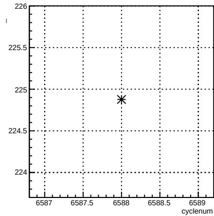
usr_4eX:cyclenum {run == 6595}
