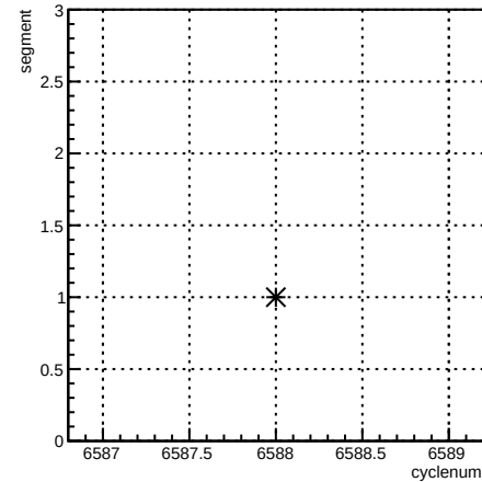
segment:cyclenum {run == 6595}
