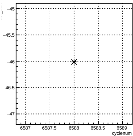
usr_12X:cyclenum {run == 6595}
