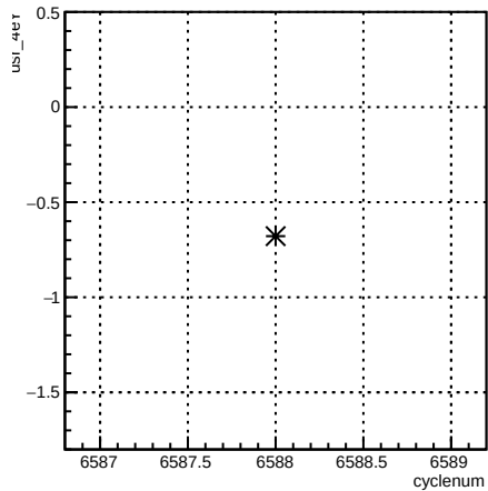
usr_4eY:cyclenum {run == 6595}
