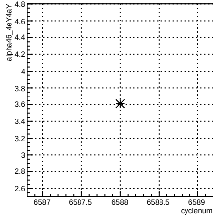
alpha46_4eY4aY:cyclenum {run == 6595}
