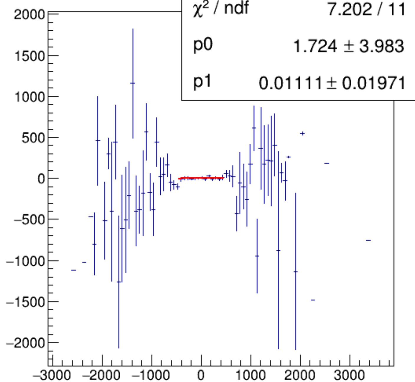
reg_asym_usl/ppm:AqUS/ppm {ok_cut}
