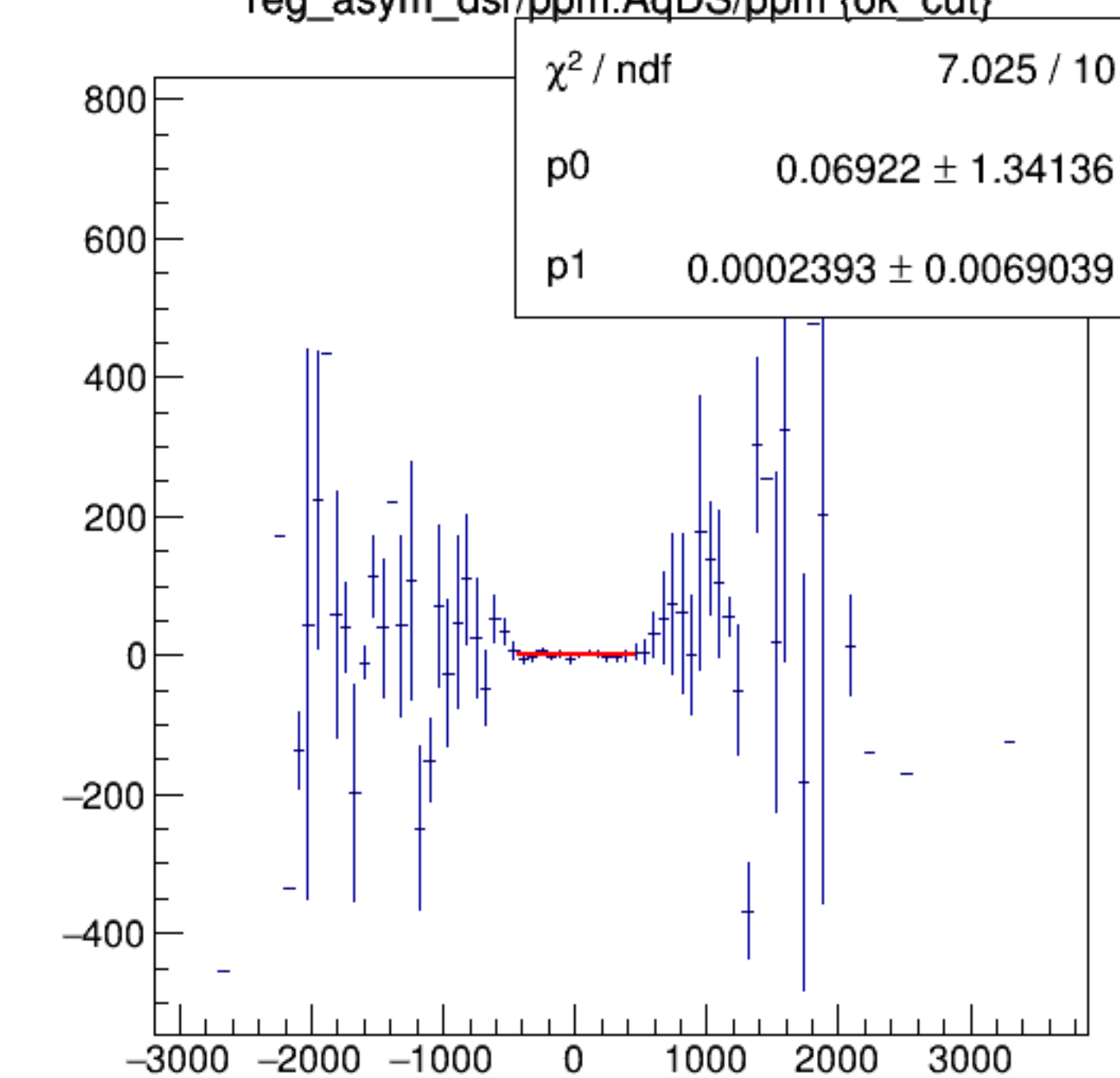
reg_asym_dsr/ppm:AqDS/ppm {ok_cut}
