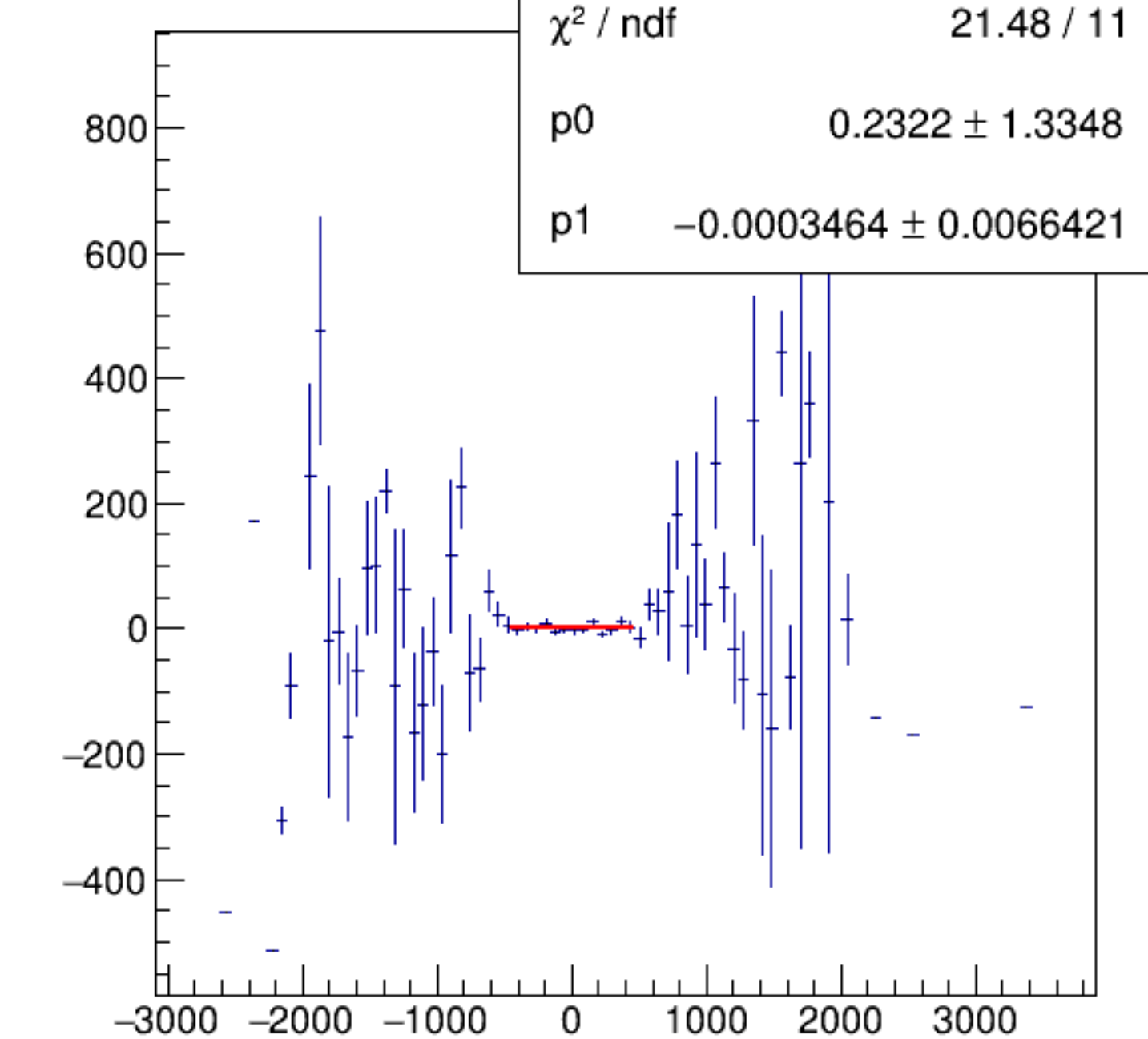
reg_asym_dsr/ppm:AqUS/ppm {ok_cut}
