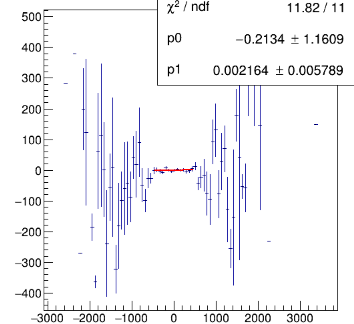
reg_asym_dsl/ppm:AqUS/ppm {ok_cut}
