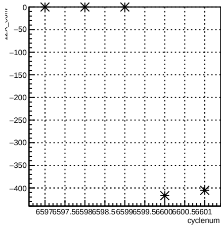
12X_coil7:cyclenum {run == 6597}
