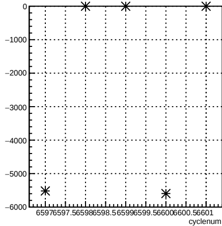
usr_coil3:cyclenum {run == 6597}
