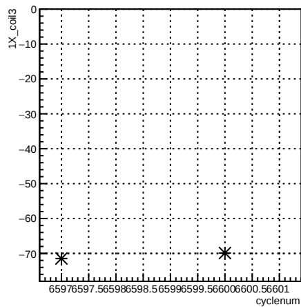
1X_coil3:cyclenum {run == 6597}
