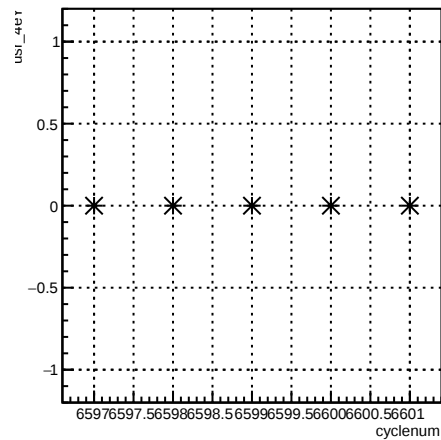
usr_4eY:cyclenum {run == 6597}
