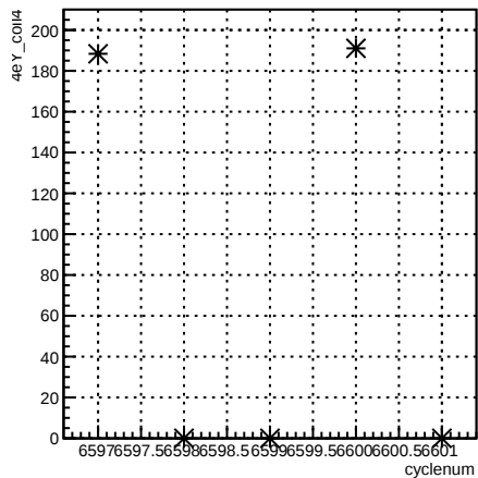
4eY_coil4:cyclenum {run == 6597}
