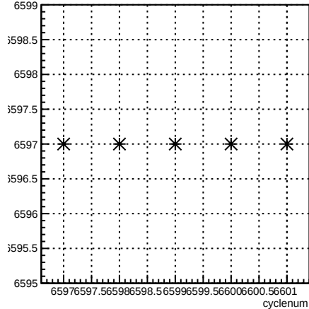
run:cyclenum {run == 6597}
