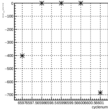
usr_coil6:cyclenum {run == 6597}
