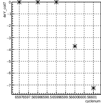
4eY_coil7:cyclenum {run == 6597}
