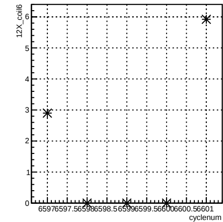
12X_coil6:cyclenum {run == 6597}
