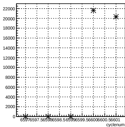
usr_coil7:cyclenum {run == 6597}
