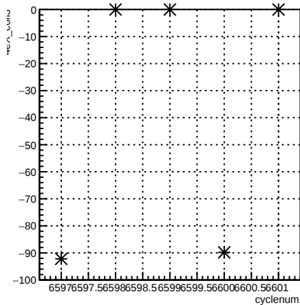
4eX_coil3:cyclenum {run == 6597}
