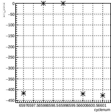
1X_coil1:cyclenum {run == 6597}
