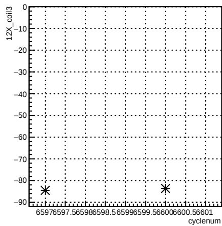
12X_coil3:cyclenum {run == 6597}
