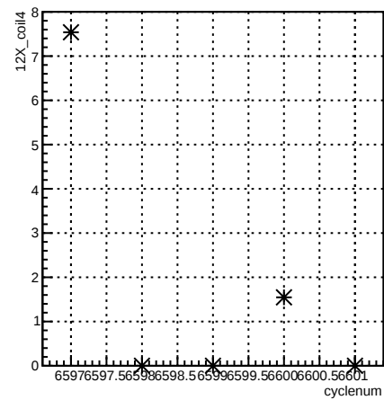
12X_coil4:cyclenum {run == 6597}
