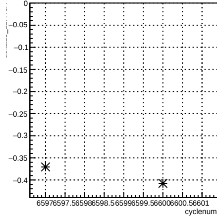
segment:cyclenum {run == 6597}
