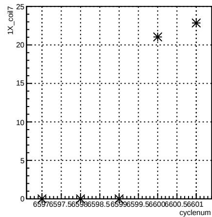
1X_coil7:cyclenum {run == 6597}
