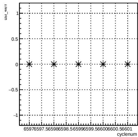
usl_4eY:cyclenum {run == 6597}
