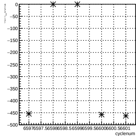
4eX_coil1:cyclenum {run == 6597}
