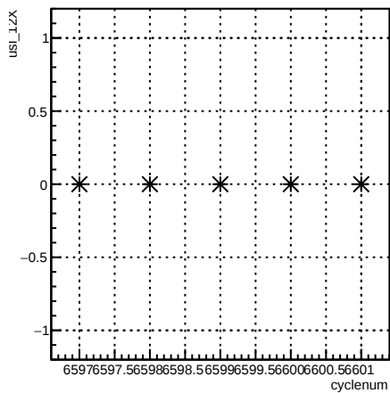
usl_12X:cyclenum {run == 6597}
