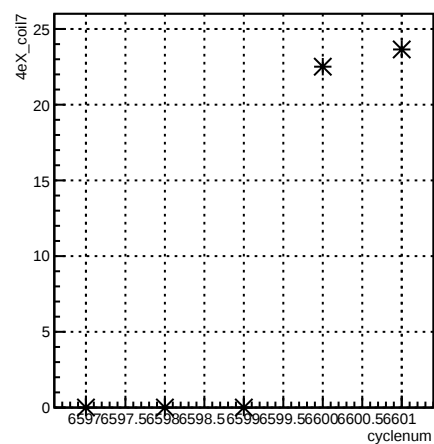
4eX_coil7:cyclenum {run == 6597}
