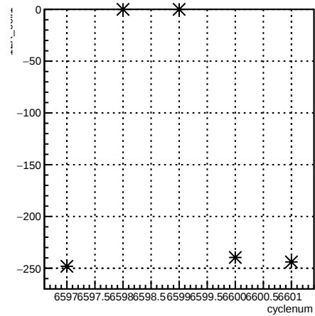
12X_coil1:cyclenum {run == 6597}
