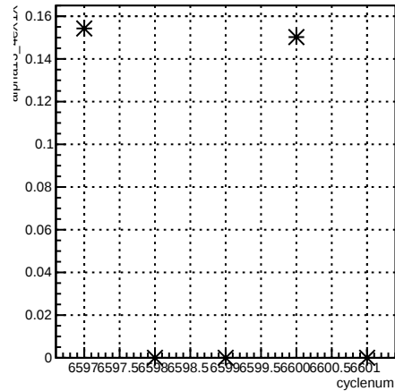
delta46_12X4eY:cyclenum {run == 6597}
