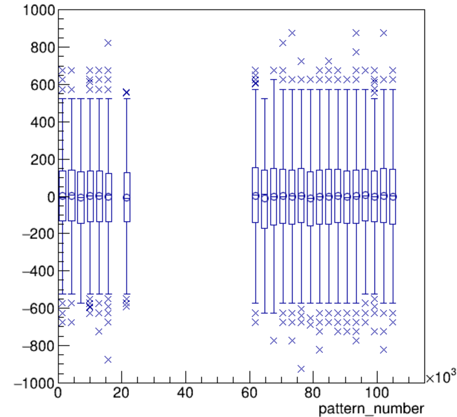
asym_bcm_dg_ds/ppm:pattern_number {ErrorFlag==0}
