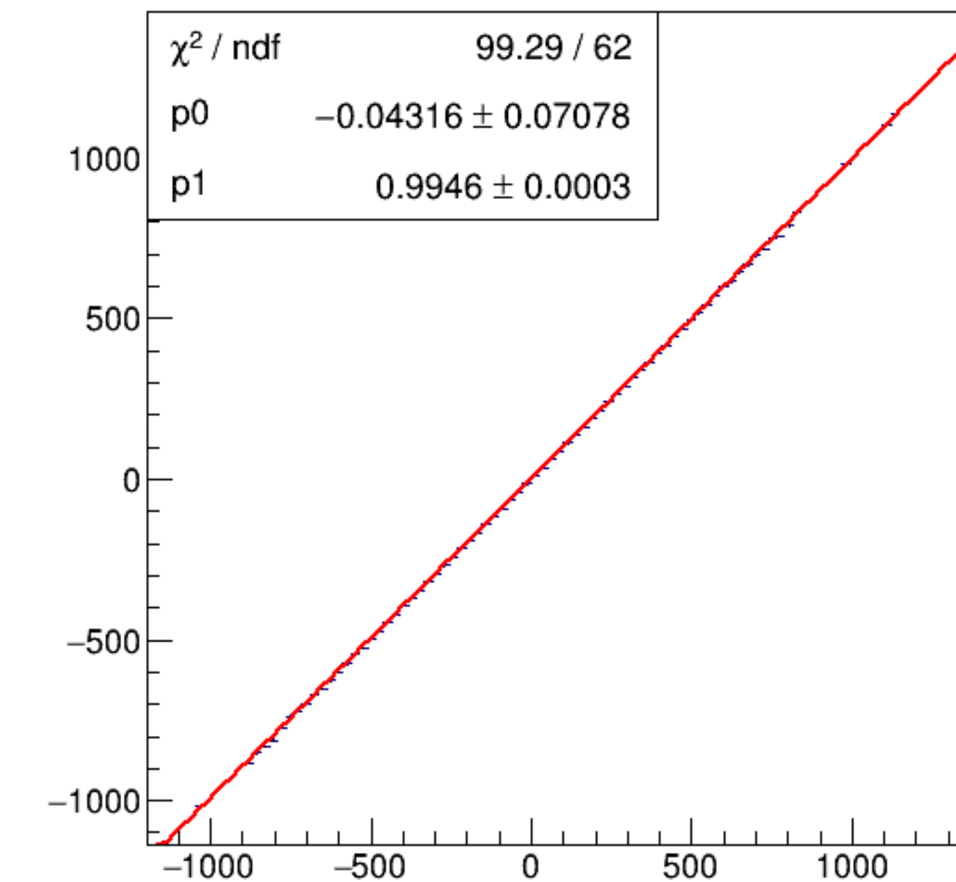
run6598_000_asym_bcm_an_ds_vs_asym_bcm_an_ds3_mul.png
