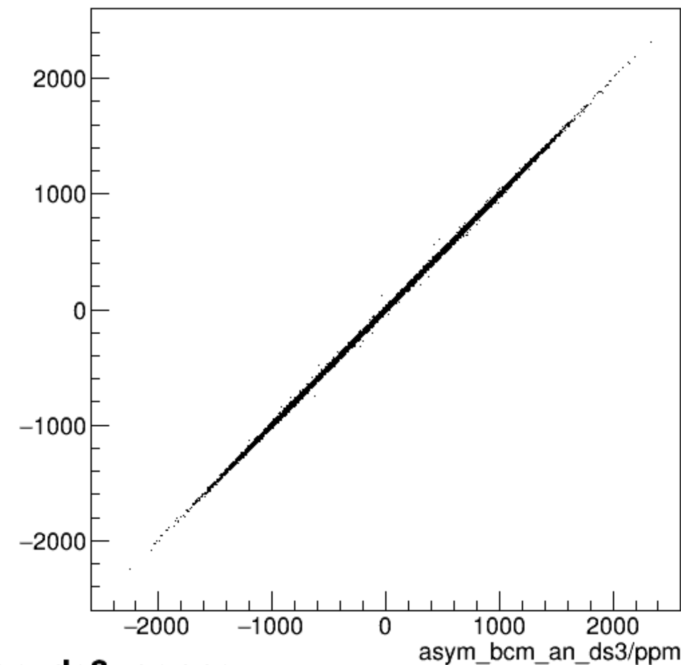
run6598_000_asym_bcm_an_ds_vs_asym_bcm_an_ds3_pr.png
