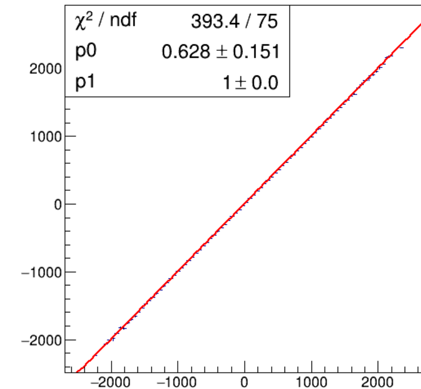
run6598_000_asym_bcm_an_us_vs_asym_bcm_an_ds3_pr.png
