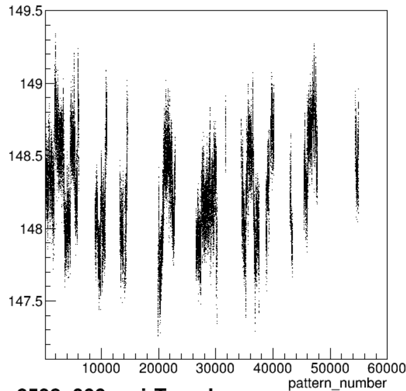
yield_bcm_an_us:pattern_number {ErrorFlag==0}
