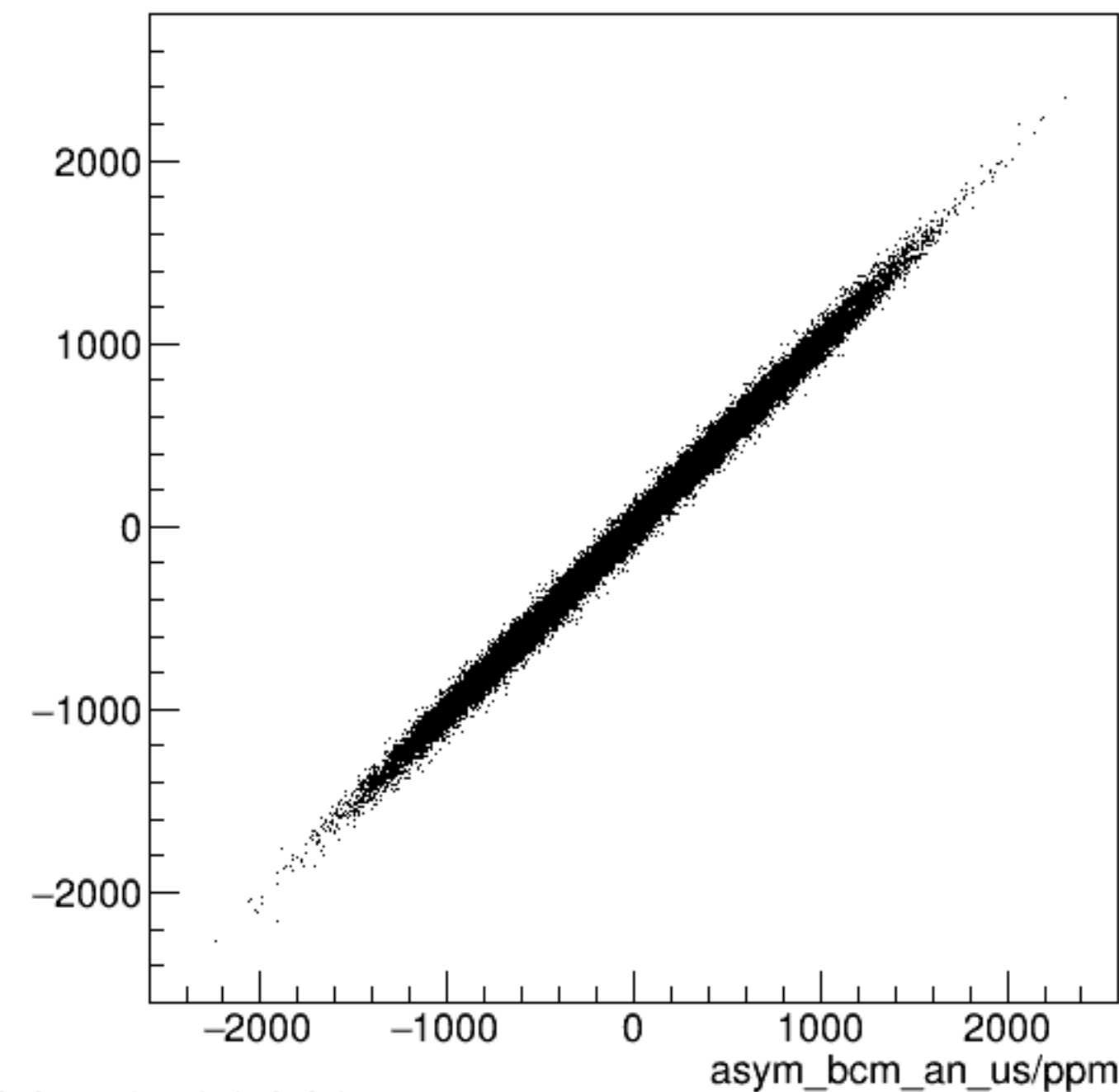
run6598_000_asym_bcm_dg_ds_vs_asym_bcm_an_us_pr.png
