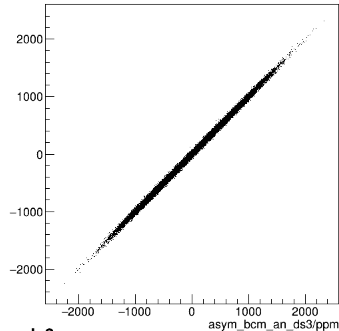
run6598_000_asym_bcm_an_us_vs_asym_bcm_an_ds3_pr.png
