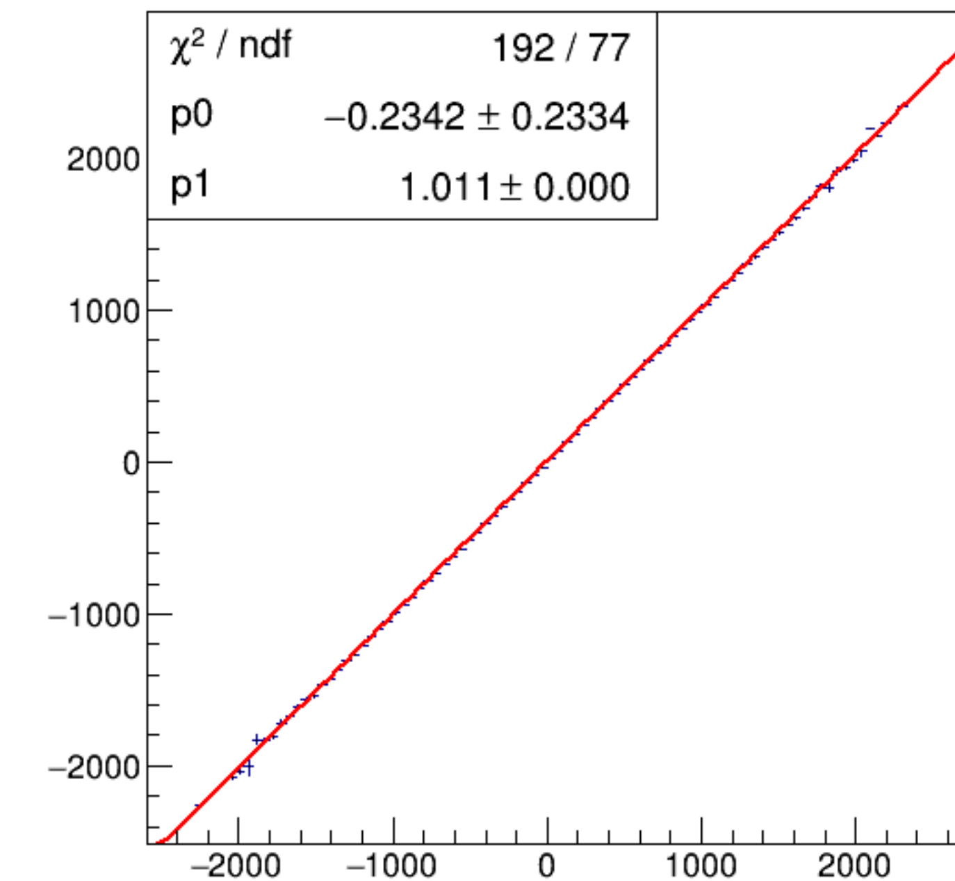
run6598_000_asym_bcm_dg_ds_vs_asym_bcm_an_us_pr.png
