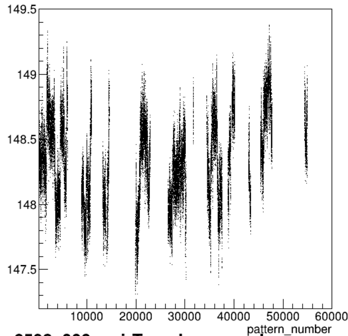
yield_bcm_an_ds:pattern_number {ErrorFlag==0}
