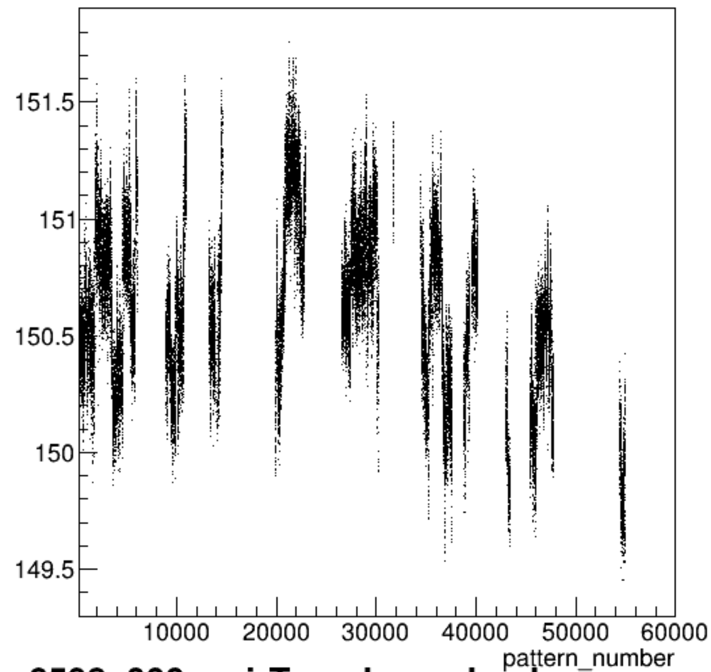
yield_bcm_dg_ds:pattern_number {ErrorFlag==0}
