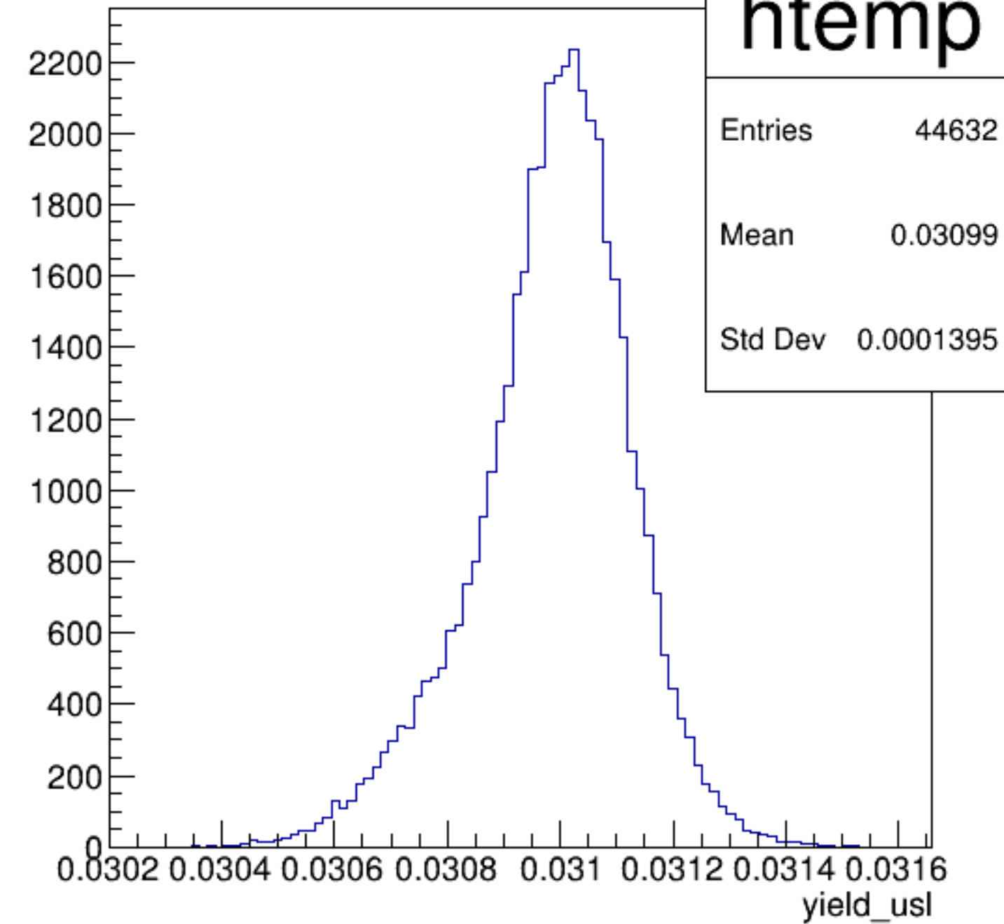
yield_usl {ErrorFlag==0}
