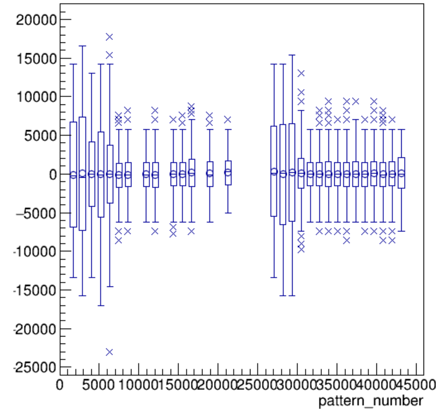
asym_usl/ppm:pattern_number {ErrorFlag==0}
