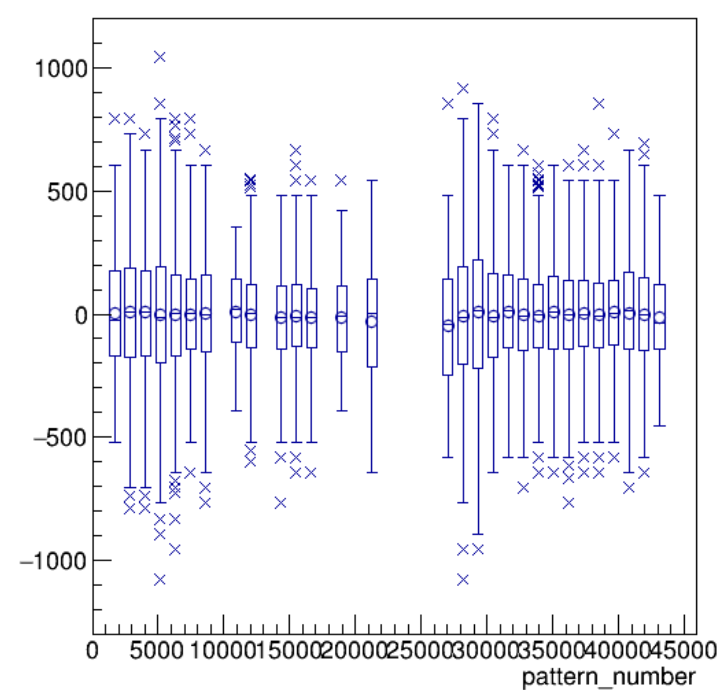
asym_sam8/ppm:pattern_number {ErrorFlag==0}
