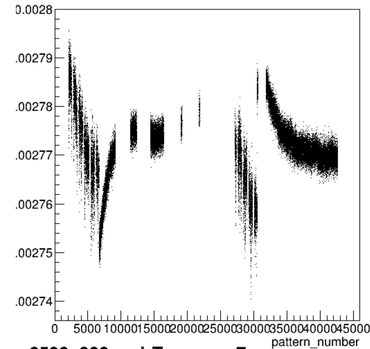
yield_sam7:pattern_number {ErrorFlag==0}
