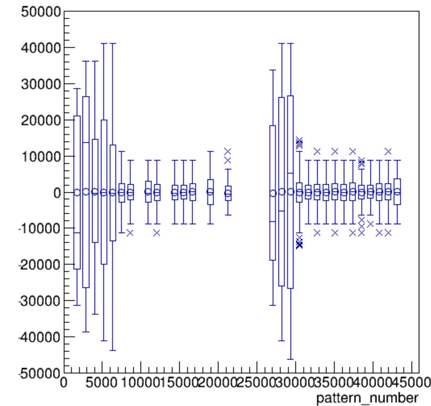
asym_sam4/ppm:pattern_number {ErrorFlag==0}
