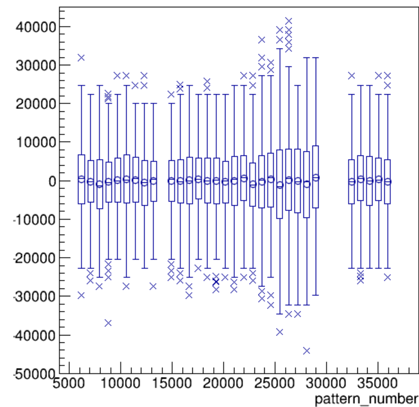
asym_atl2/ppm:pattern_number {ErrorFlag==0}
