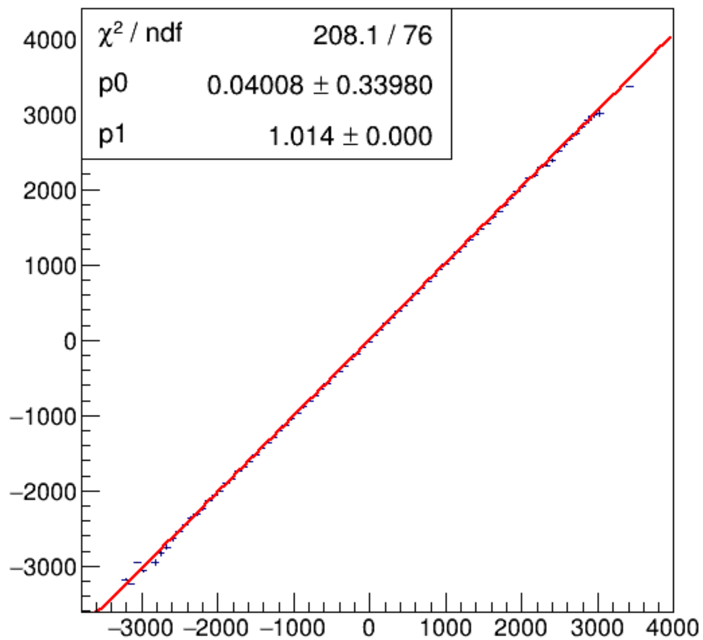
run6600_000_asym_bcm_dg_us_vs_asym_bcm_dg_ds_pr.png
