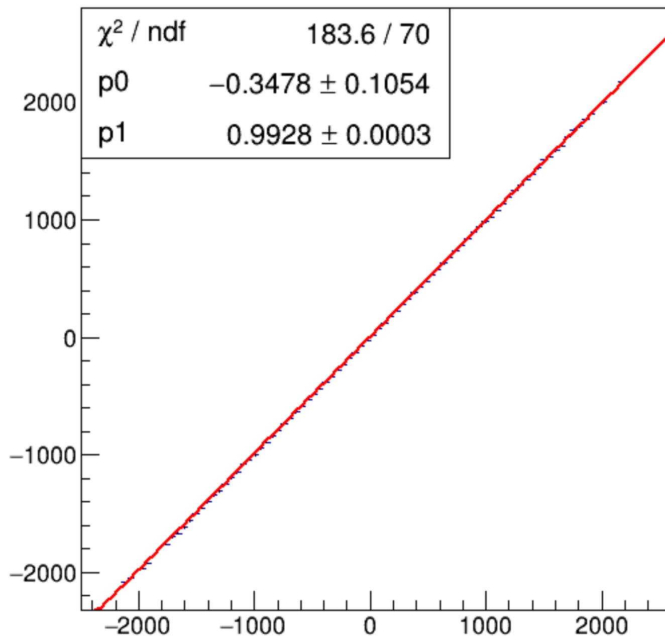
run6600_000_asym_bcm_an_ds_vs_asym_bcm_an_ds3_mul.png
