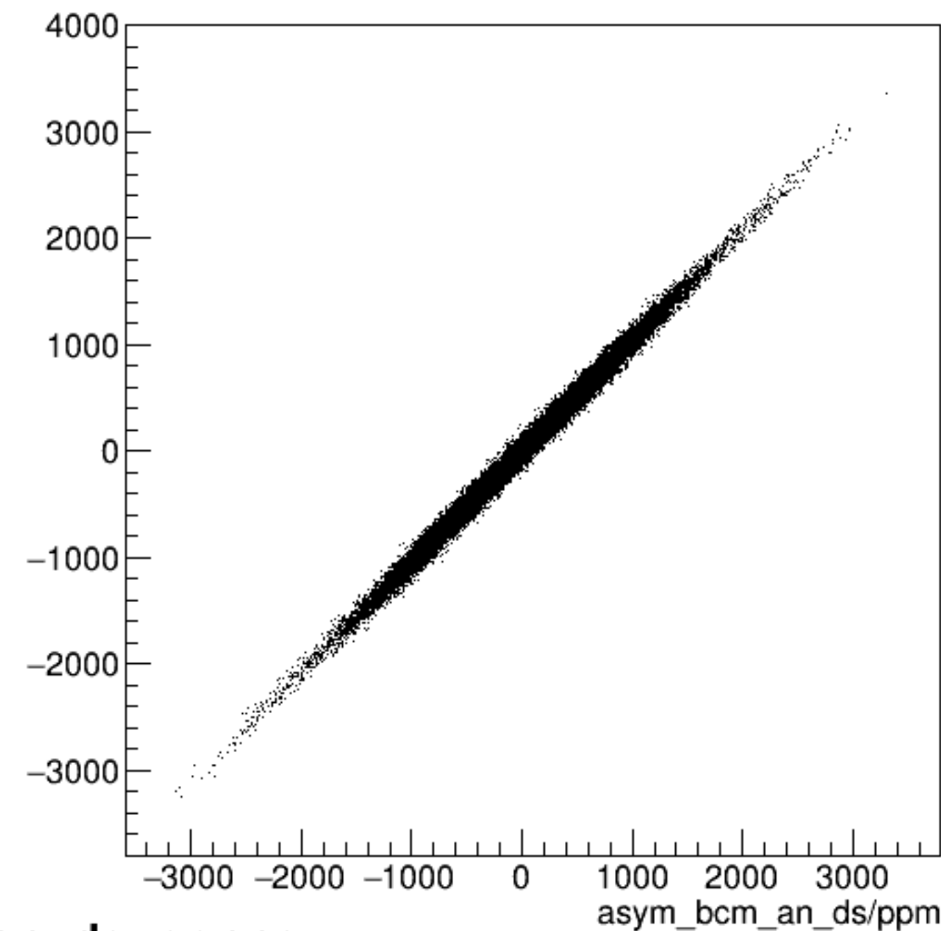
run6600_000_asym_bcm_dg_us_vs_asym_bcm_an_ds_pr.png
