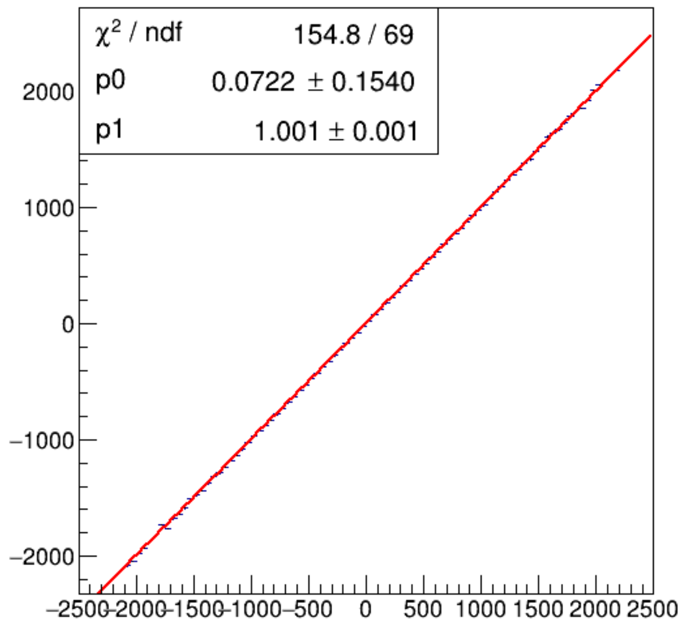
run6600_000_asym_bcm_an_us_vs_asym_bcm_an_ds_mul.png
