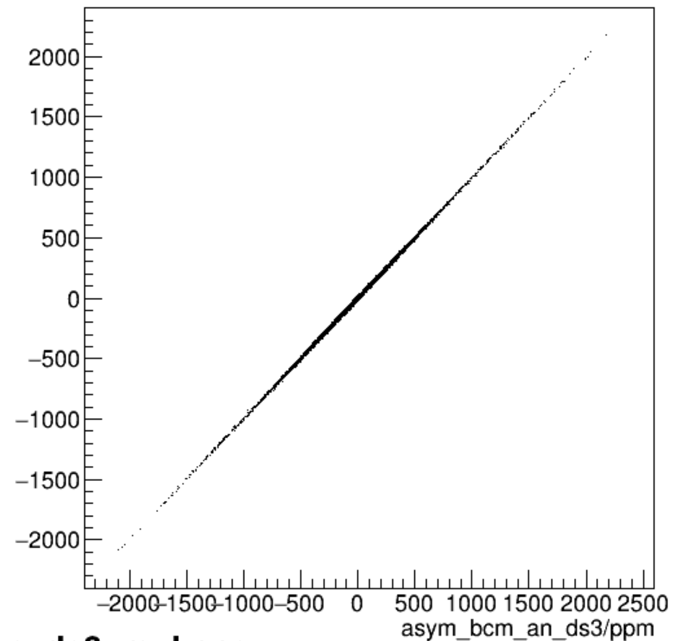
run6600_000_asym_bcm_an_ds_vs_asym_bcm_an_ds3_mul.png
