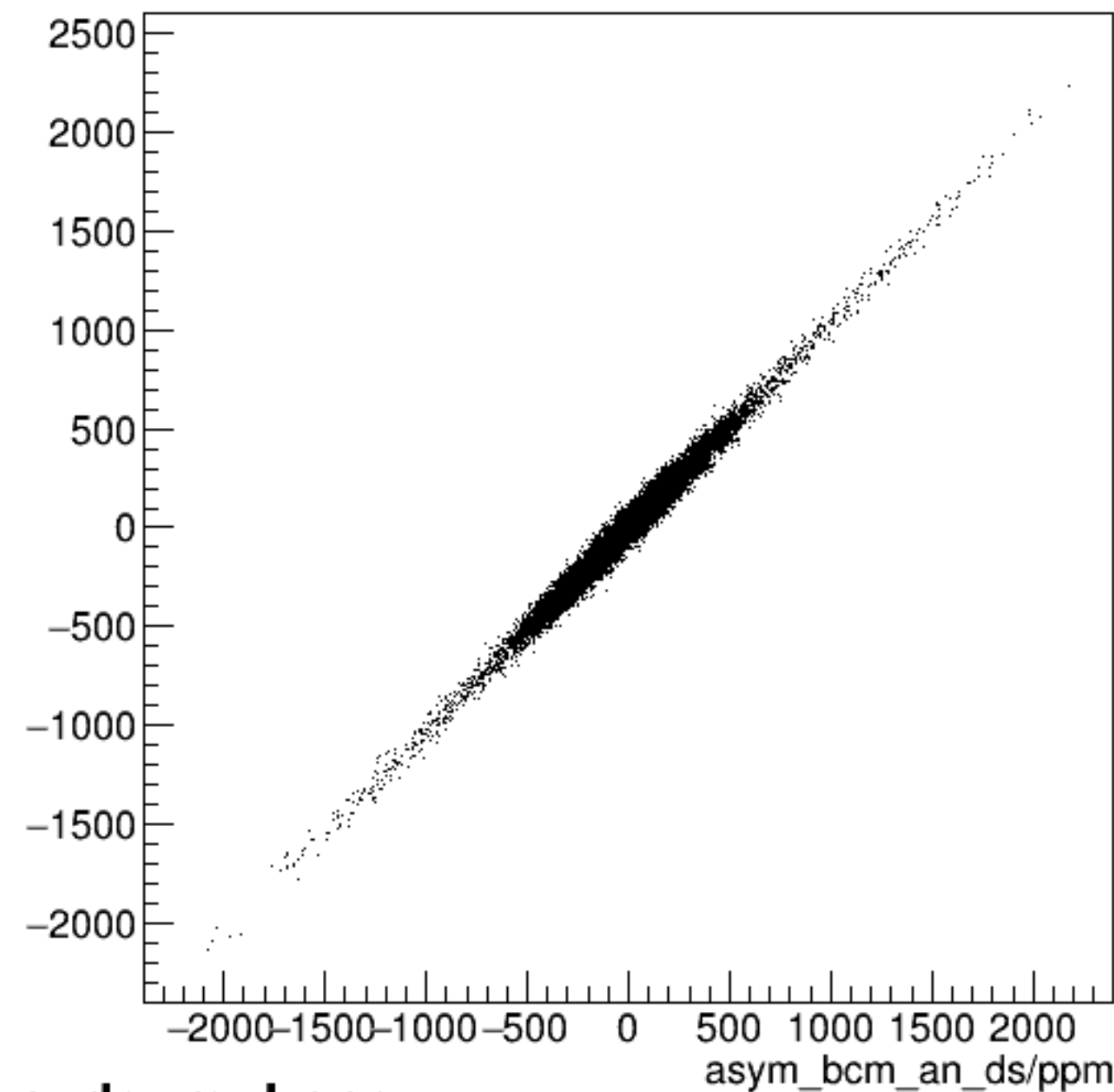
run6600_000_asym_bcm_dg_us_vs_asym_bcm_an_ds_mul.png
