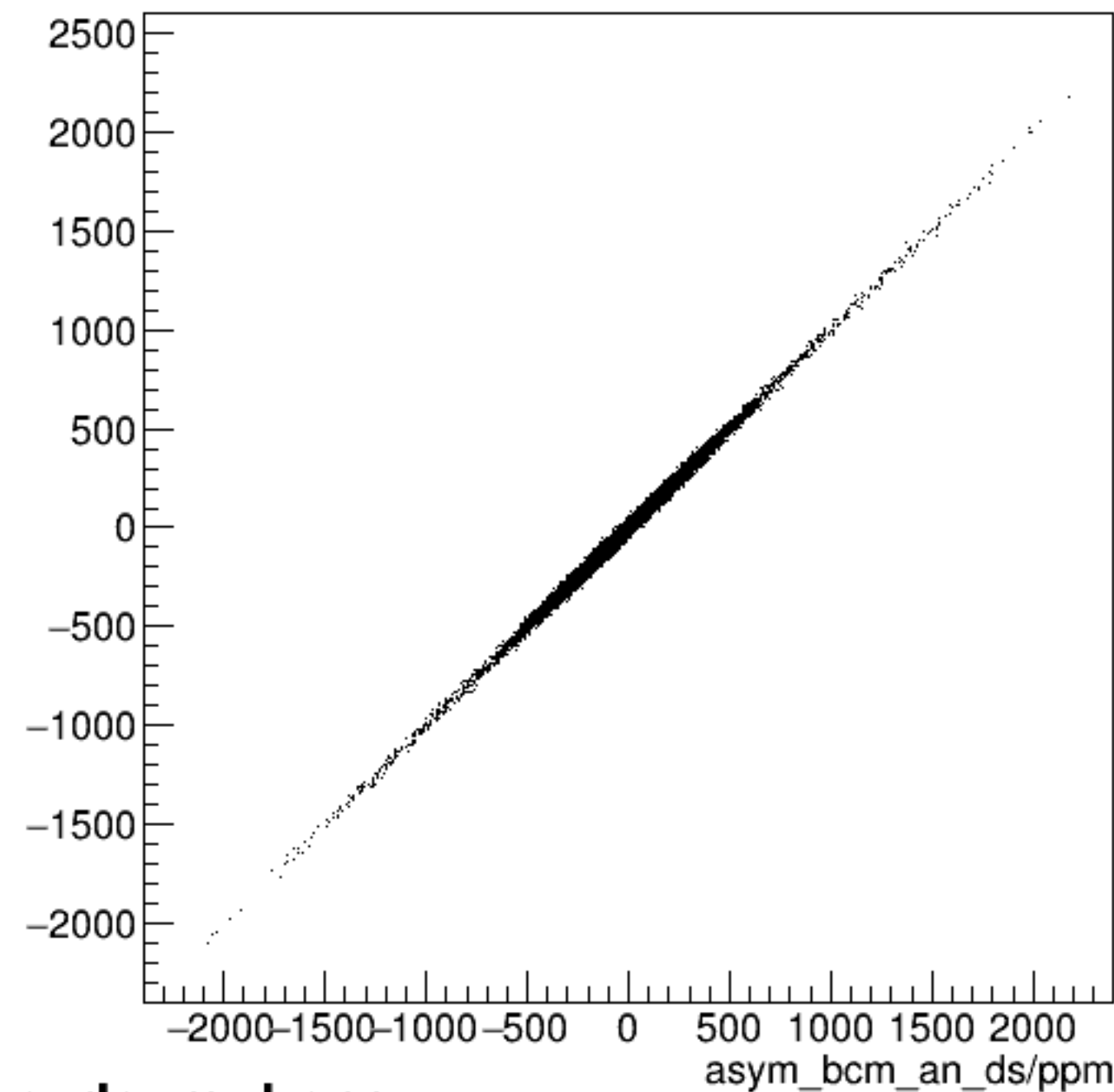
run6600_000_asym_bcm_an_us_vs_asym_bcm_an_ds_mul.png
