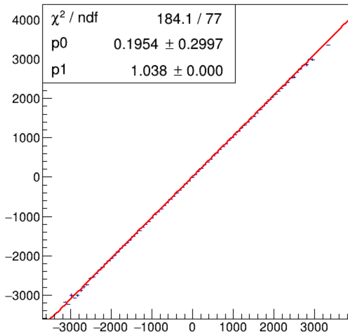
run6600_000_asym_bcm_dg_us_vs_asym_bcm_an_ds_pr.png
