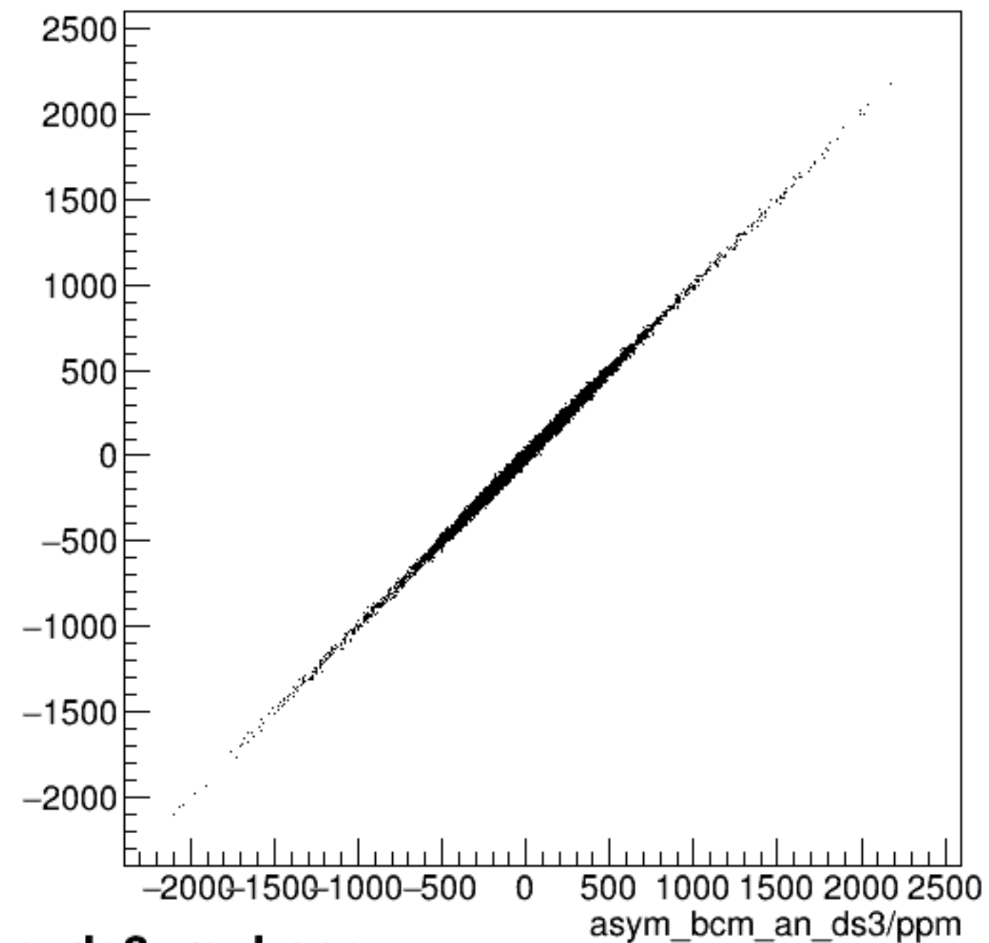
run6600_000_asym_bcm_an_us_vs_asym_bcm_an_ds3_mul.png
