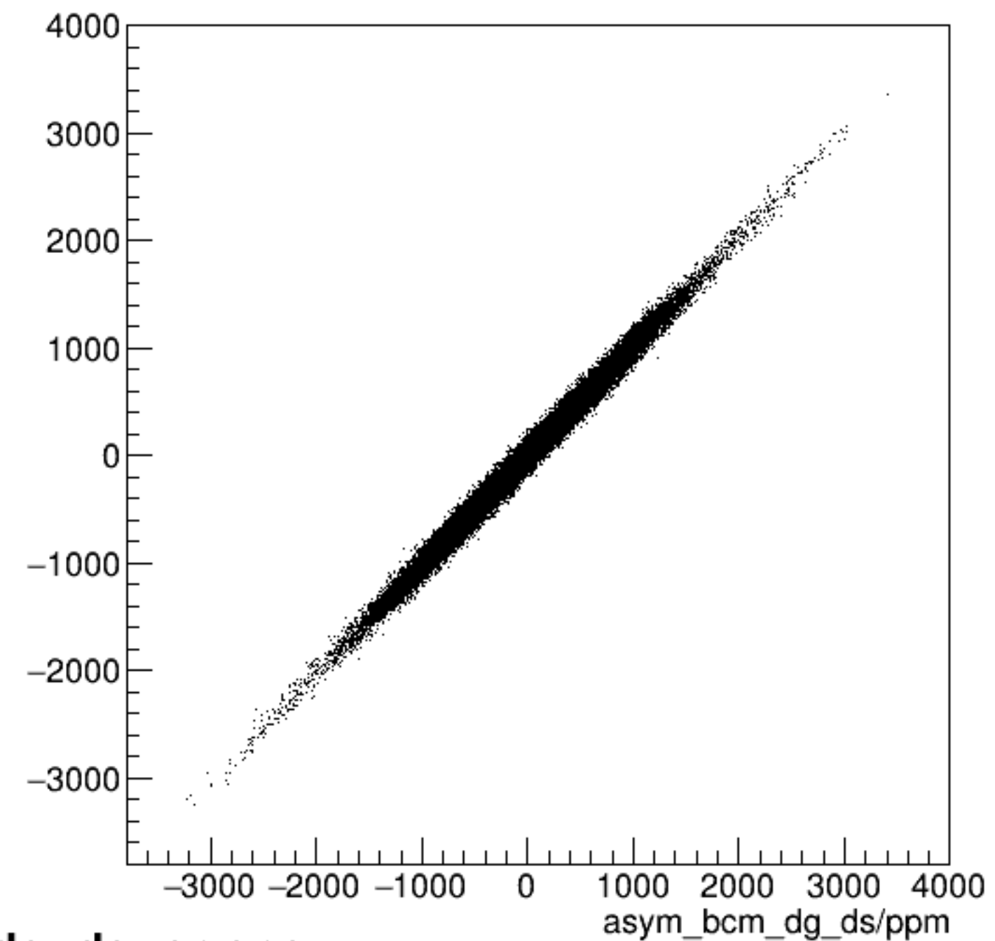
run6600_000_asym_bcm_dg_us_vs_asym_bcm_dg_ds_pr.png
