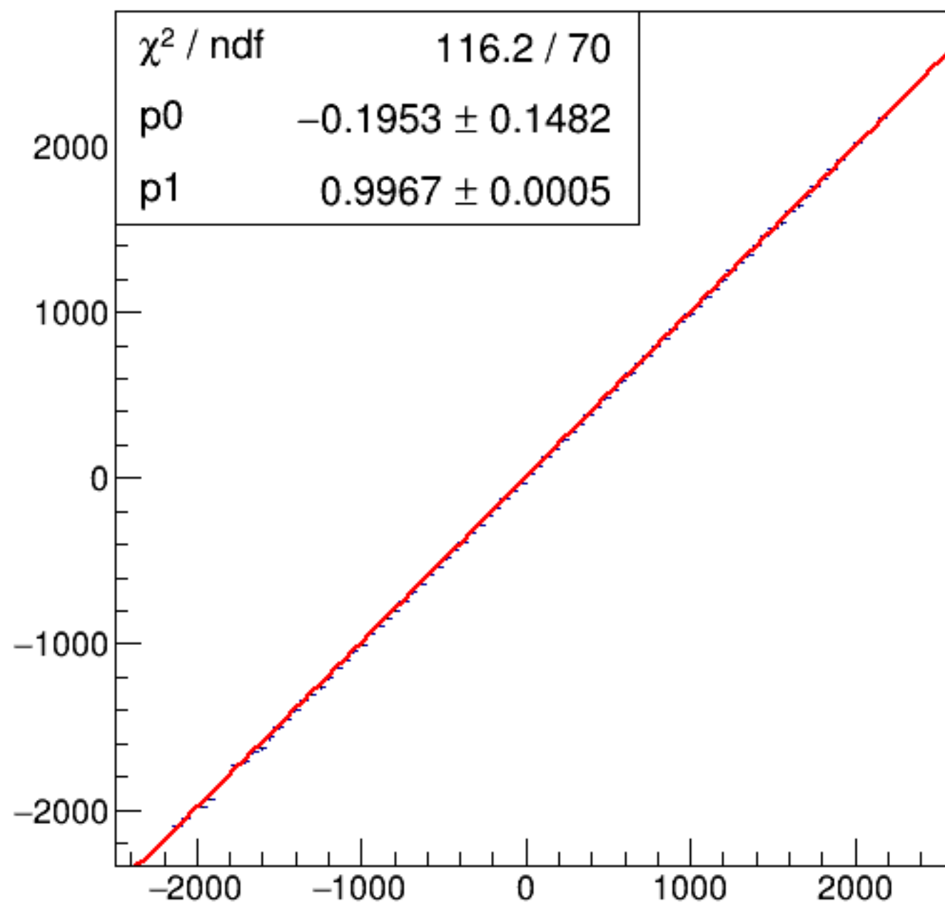
run6600_000_asym_bcm_an_us_vs_asym_bcm_an_ds3_mul.png
