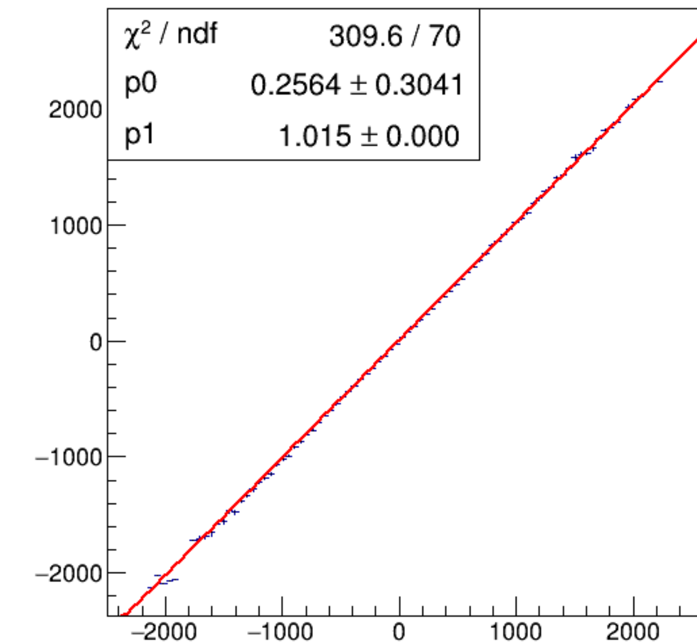
run6600_000_asym_bcm_dg_us_vs_asym_bcm_dg_ds_mul.png
