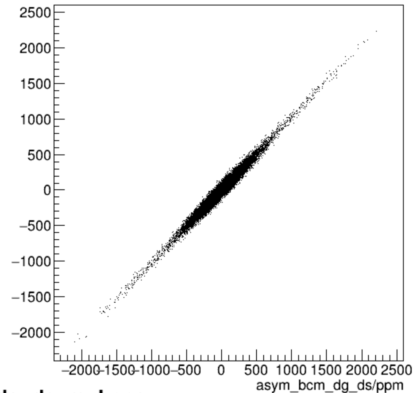
run6600_000_asym_bcm_dg_us_vs_asym_bcm_dg_ds_mul.png
