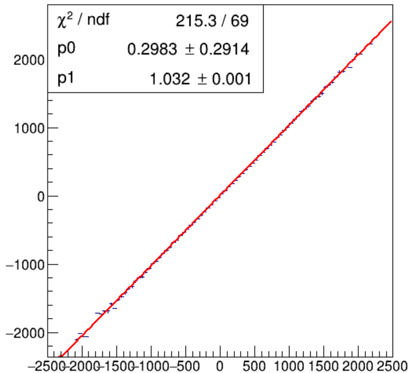
run6600_000_asym_bcm_dg_us_vs_asym_bcm_an_ds_mul.png
