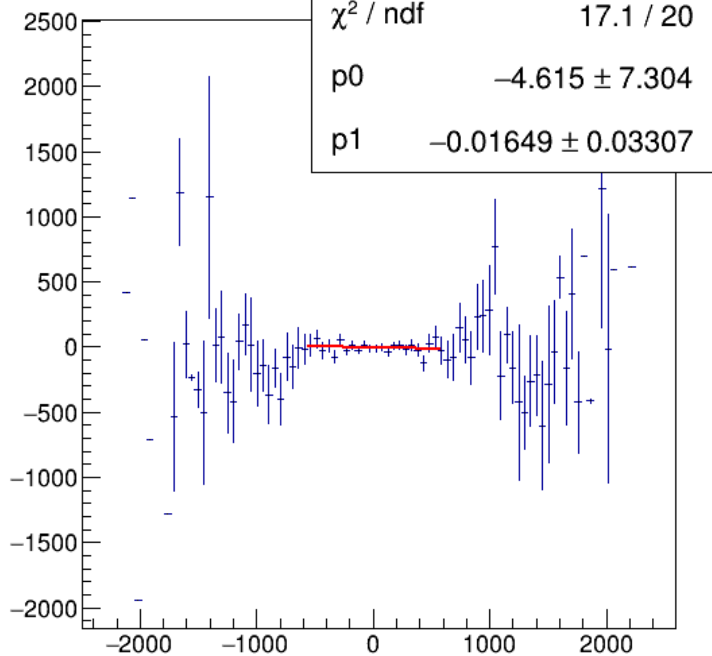
reg_asym_usl/ppm:AqDS/ppm {ok_cut}
