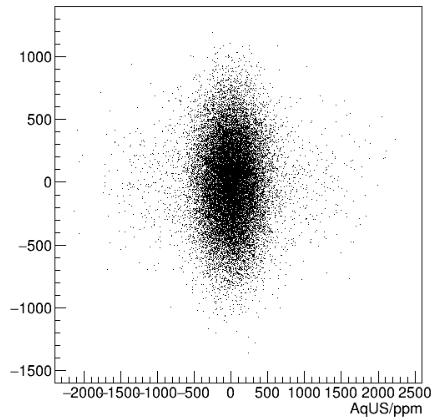
reg_asym_dsl/ppm:AqUS/ppm {ok_cut}
