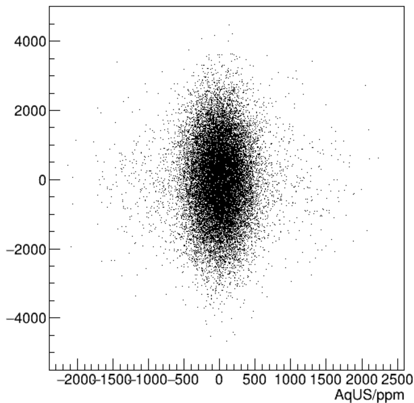
reg_asym_usl/ppm:AqUS/ppm {ok_cut}
