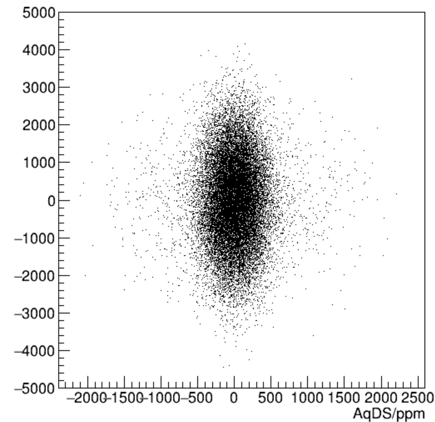
reg_asym_usr/ppm:AqDS/ppm {ok_cut}
