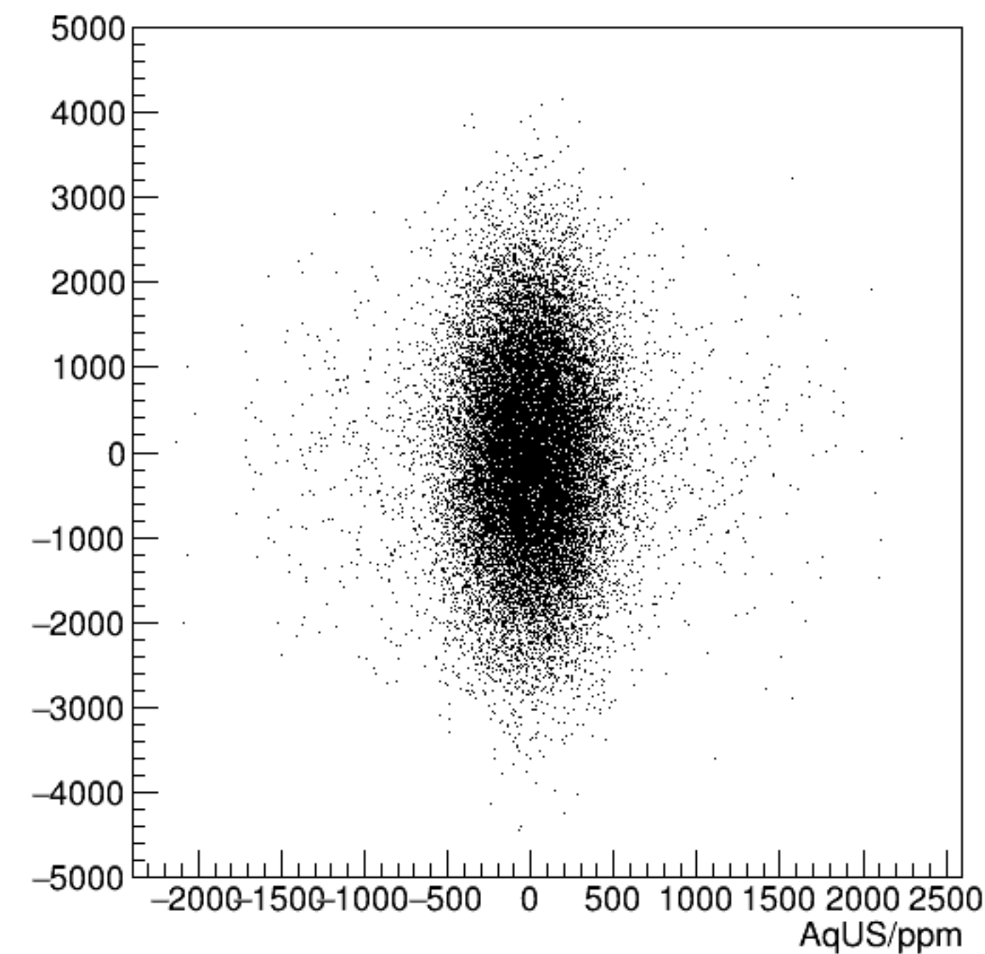
reg_asym_usr/ppm:AqUS/ppm {ok_cut}
