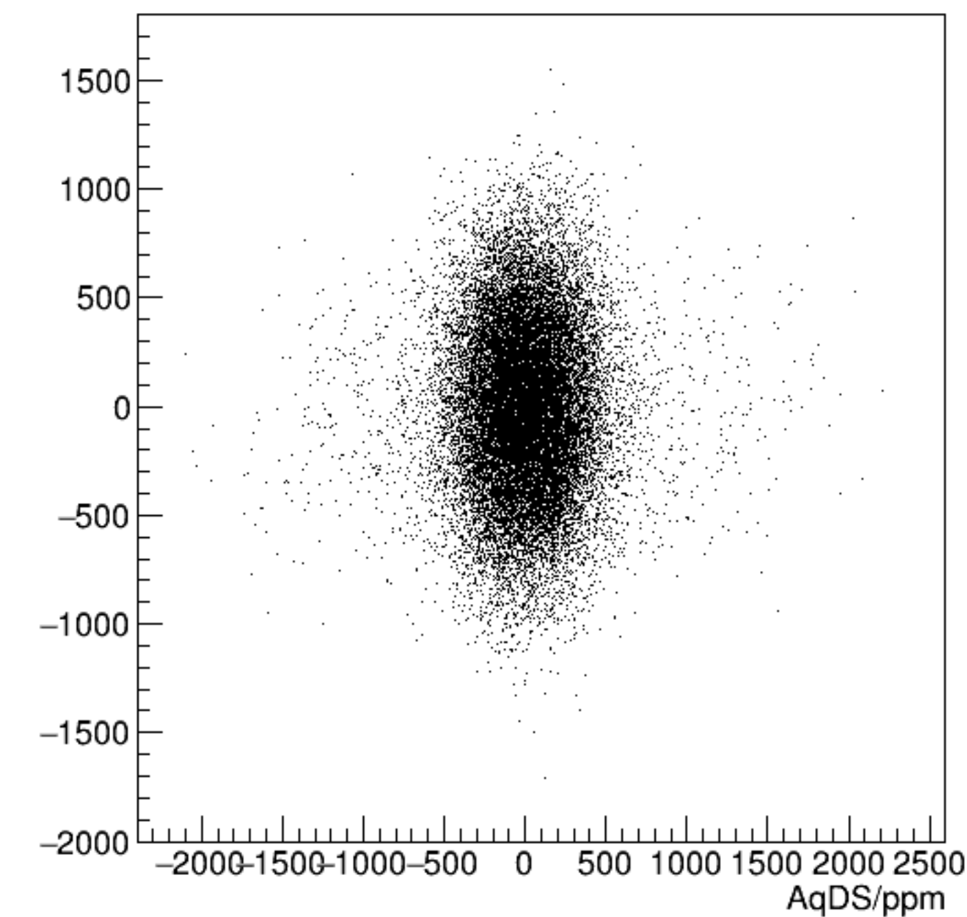
reg_asym_dsr/ppm:AqDS/ppm {ok_cut}
