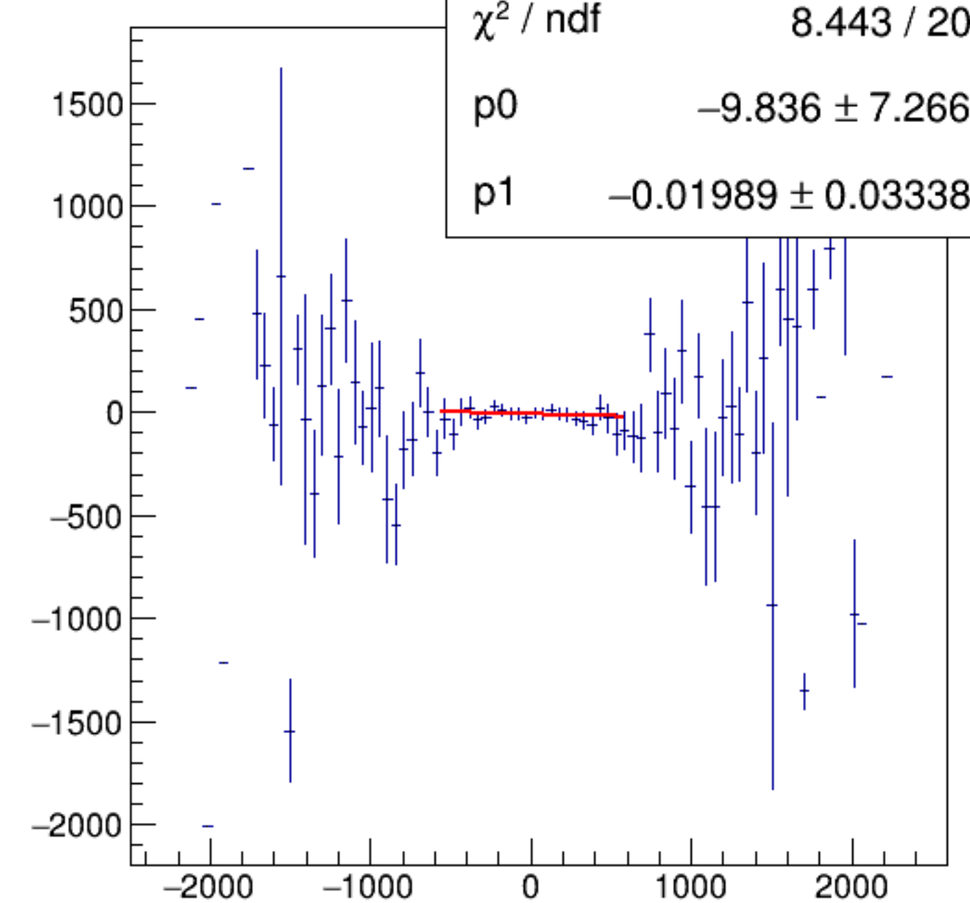
reg_asym_usr/ppm:AqDS/ppm {ok_cut}
