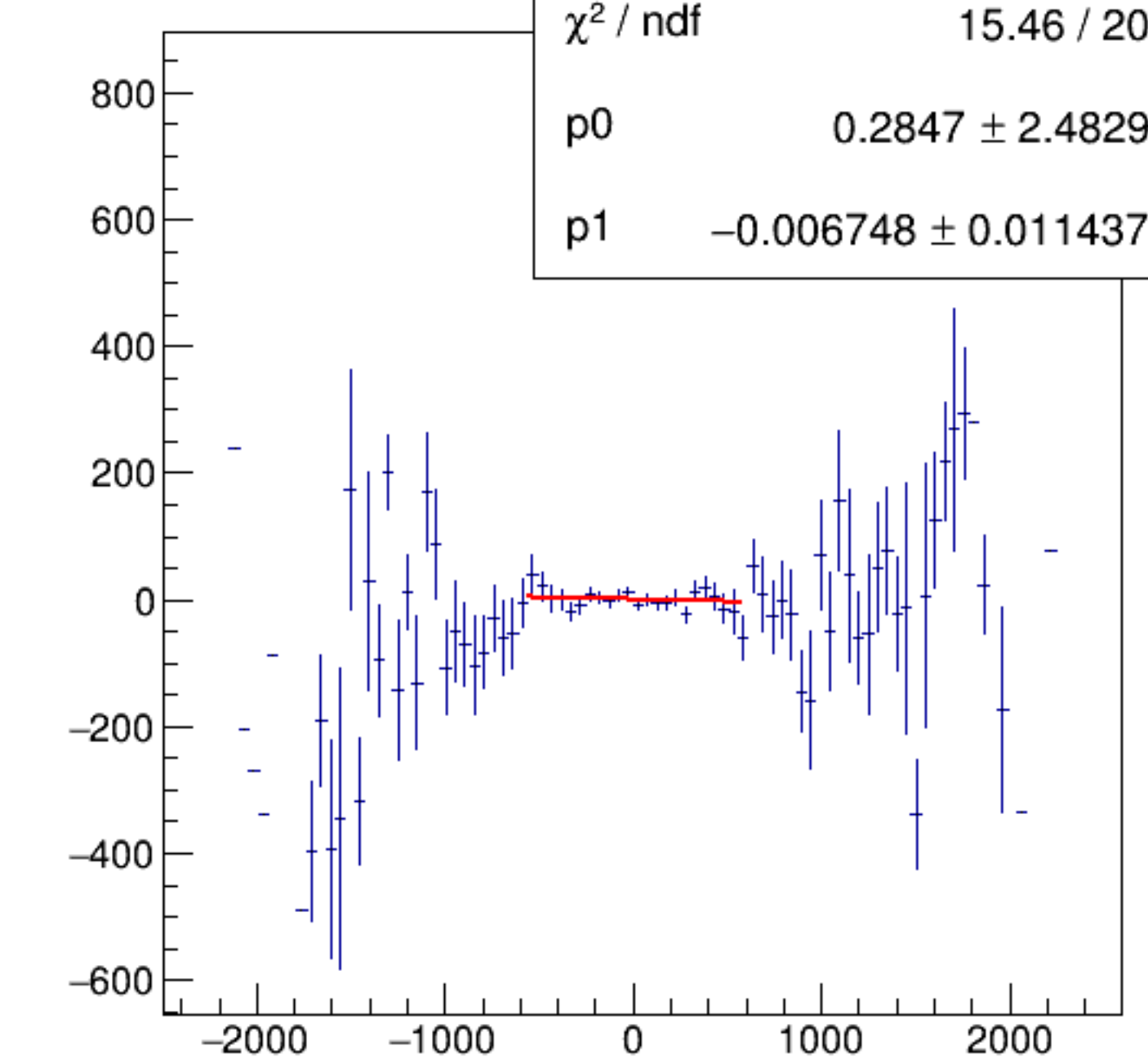
reg_asym_dsr/ppm:AqDS/ppm {ok_cut}
