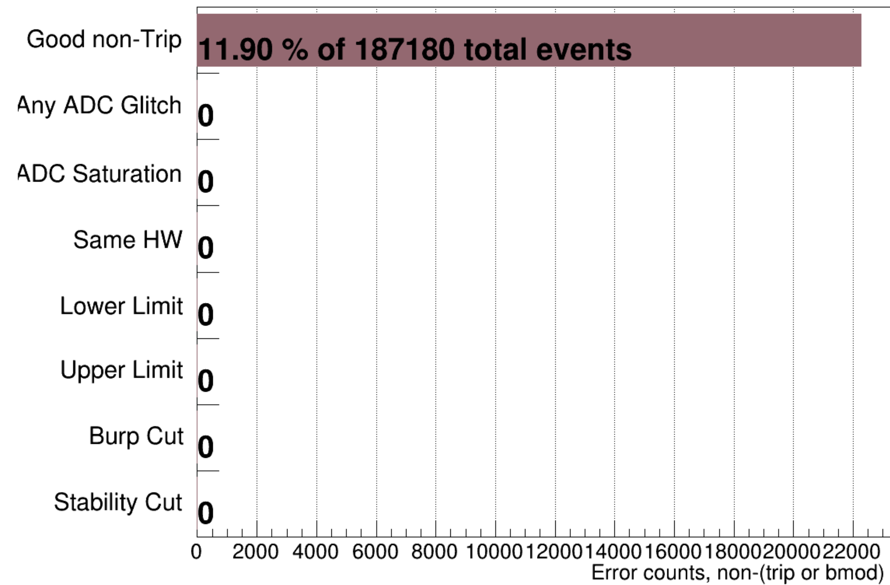
usl's Device Error Counter && Not (Trip || BMOD)
