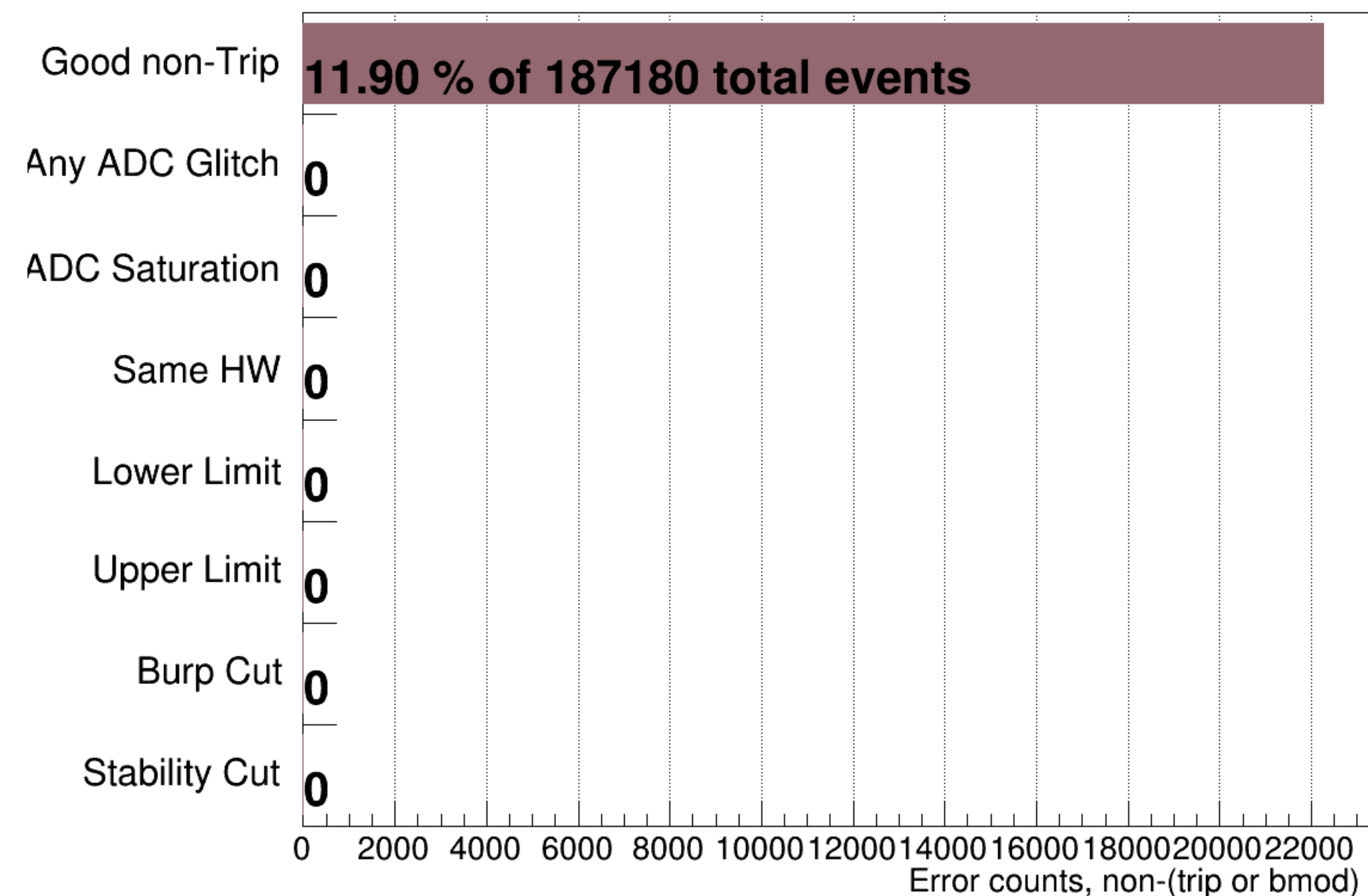
sam7's Device Error Counter && Not (Trip || BMOD)
