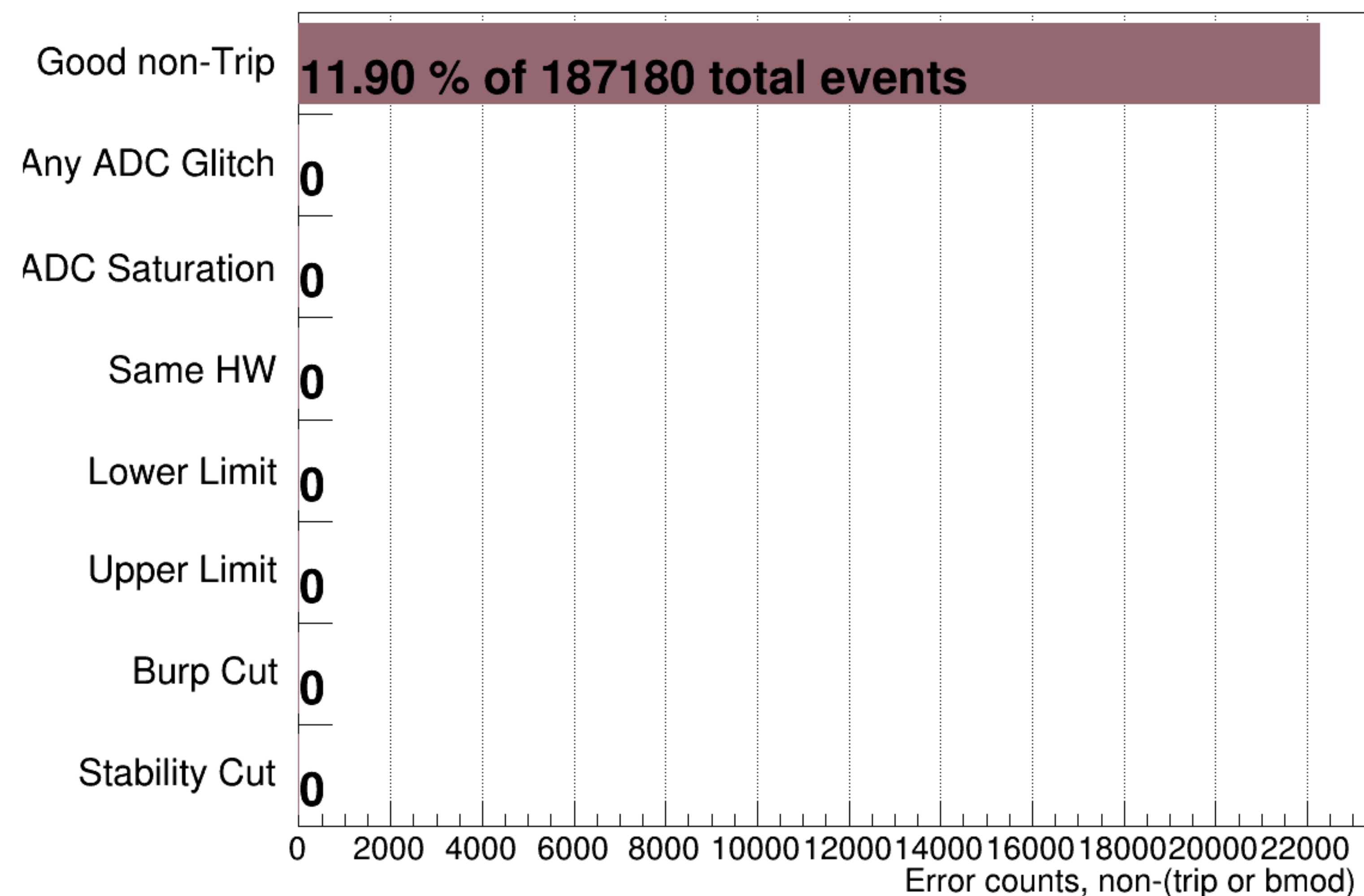
bcm_an_ds's Device Error Counter &amp; Not (Trip || BMOD)
