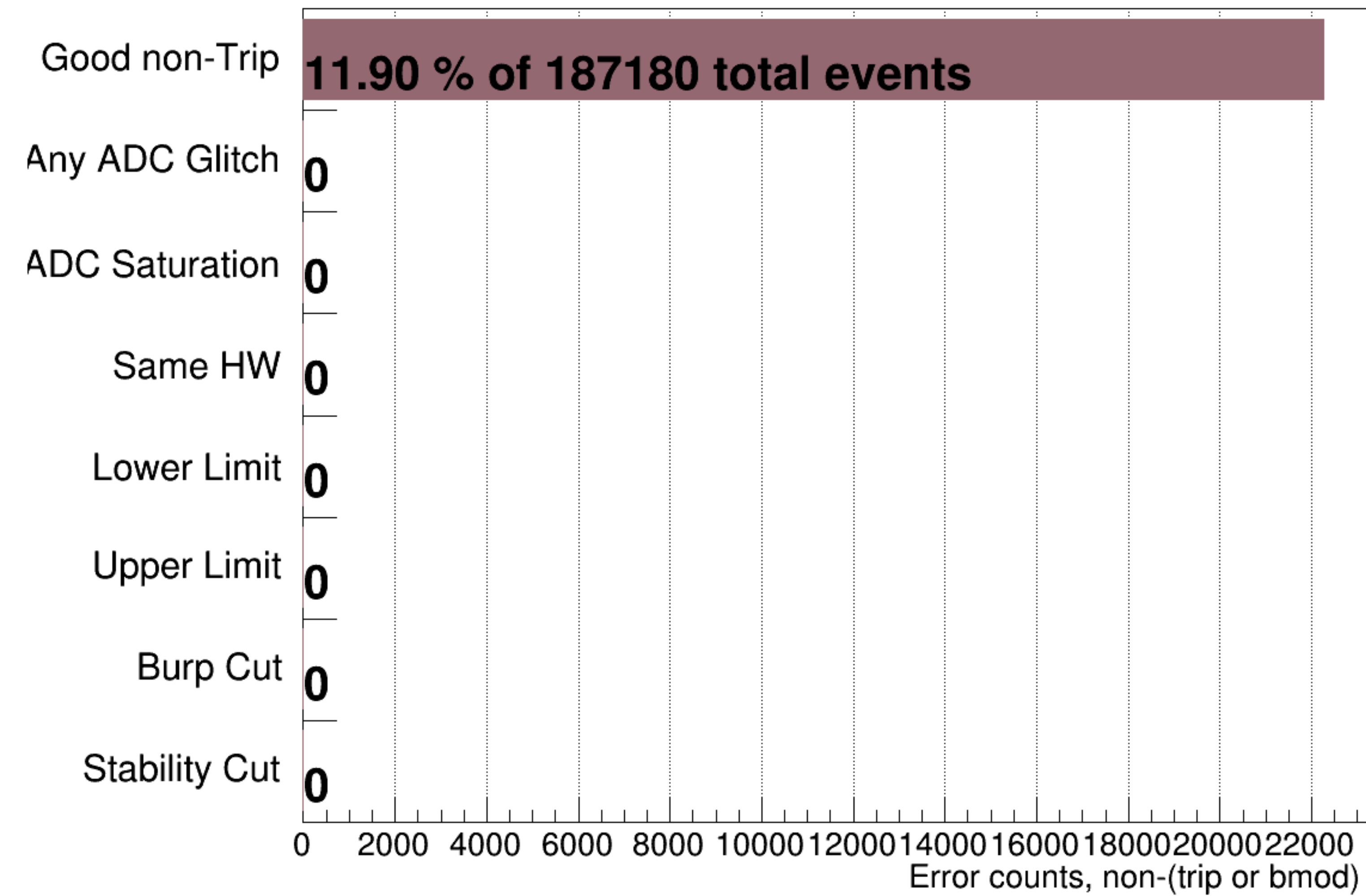
atr1's Device Error Counter &amp; Not (Trip || BMOD)
