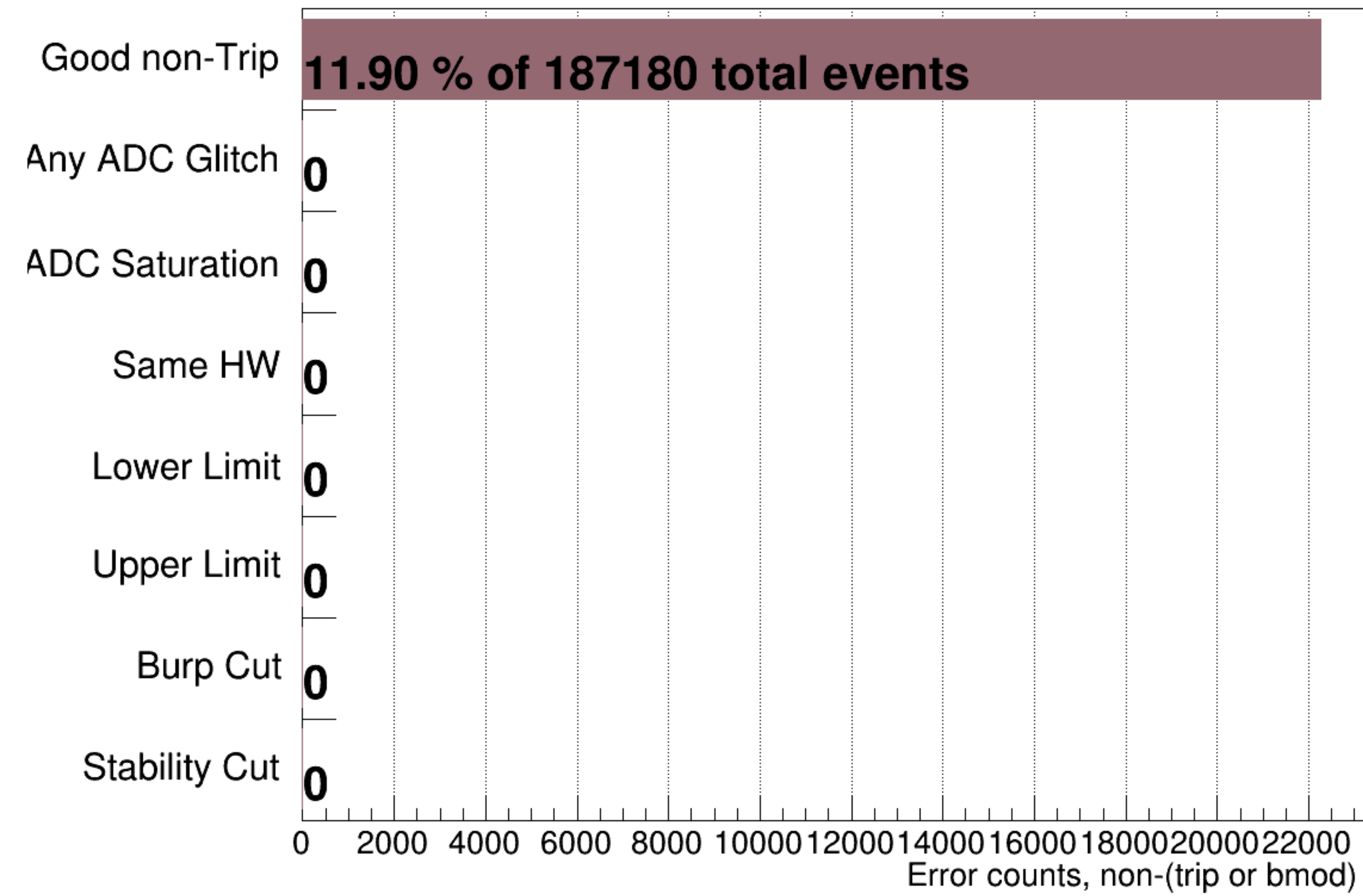
atl1's Device Error Counter &amp; Not (Trip || BMOD)
