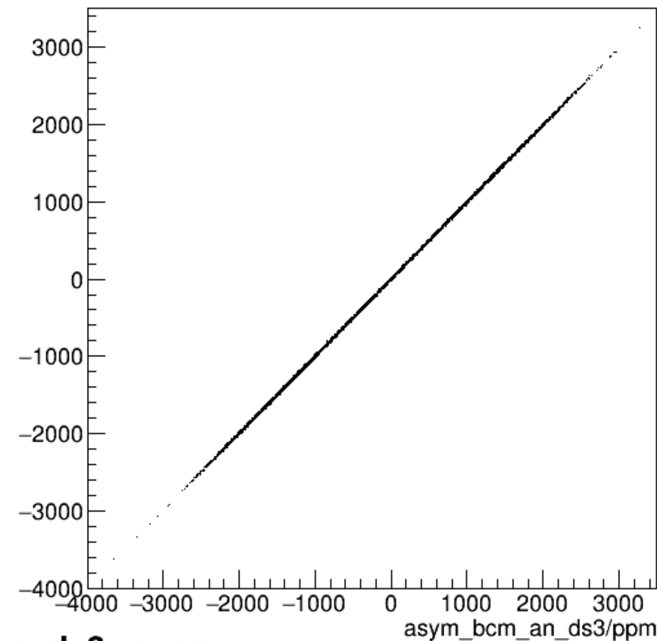
run6608_000_asym_bcm_an_ds_vs_asym_bcm_an_ds3_pr.png
