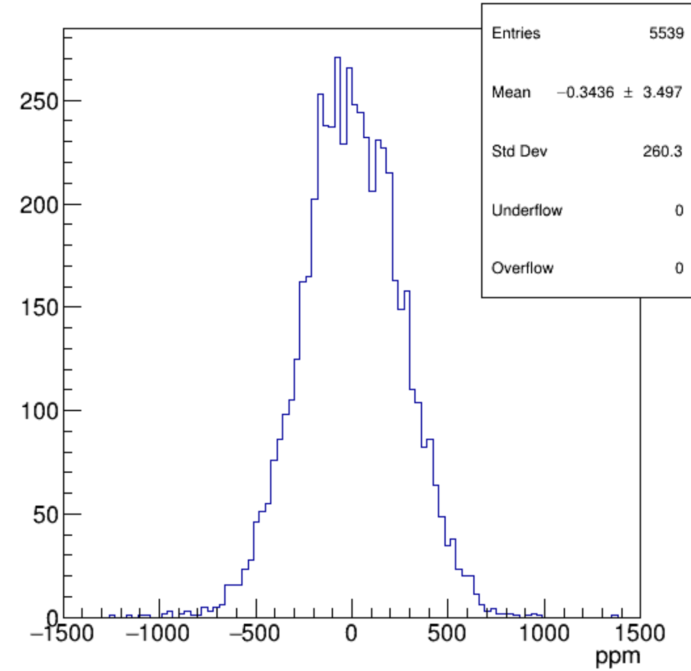
asym_bcm_an_ds
