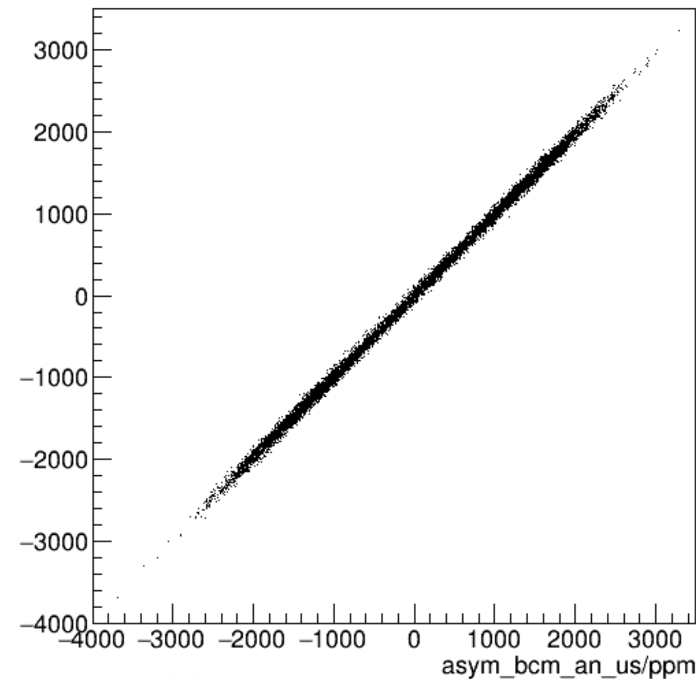
run6608_000_asym_bcm_dg_ds_vs_asym_bcm_an_us_pr.png
