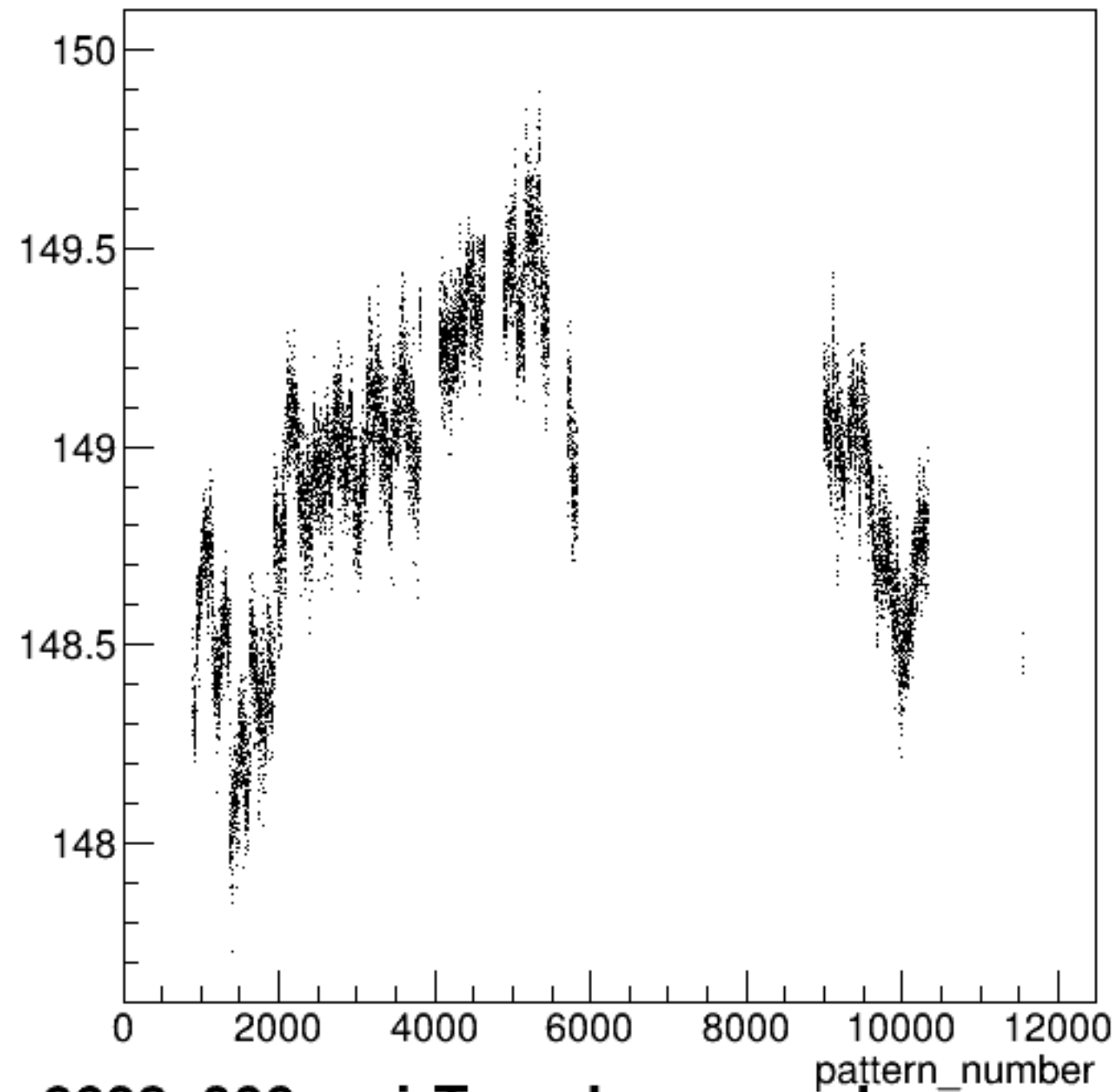
yield_bcm_an_ds:pattern_number {ErrorFlag==0}
