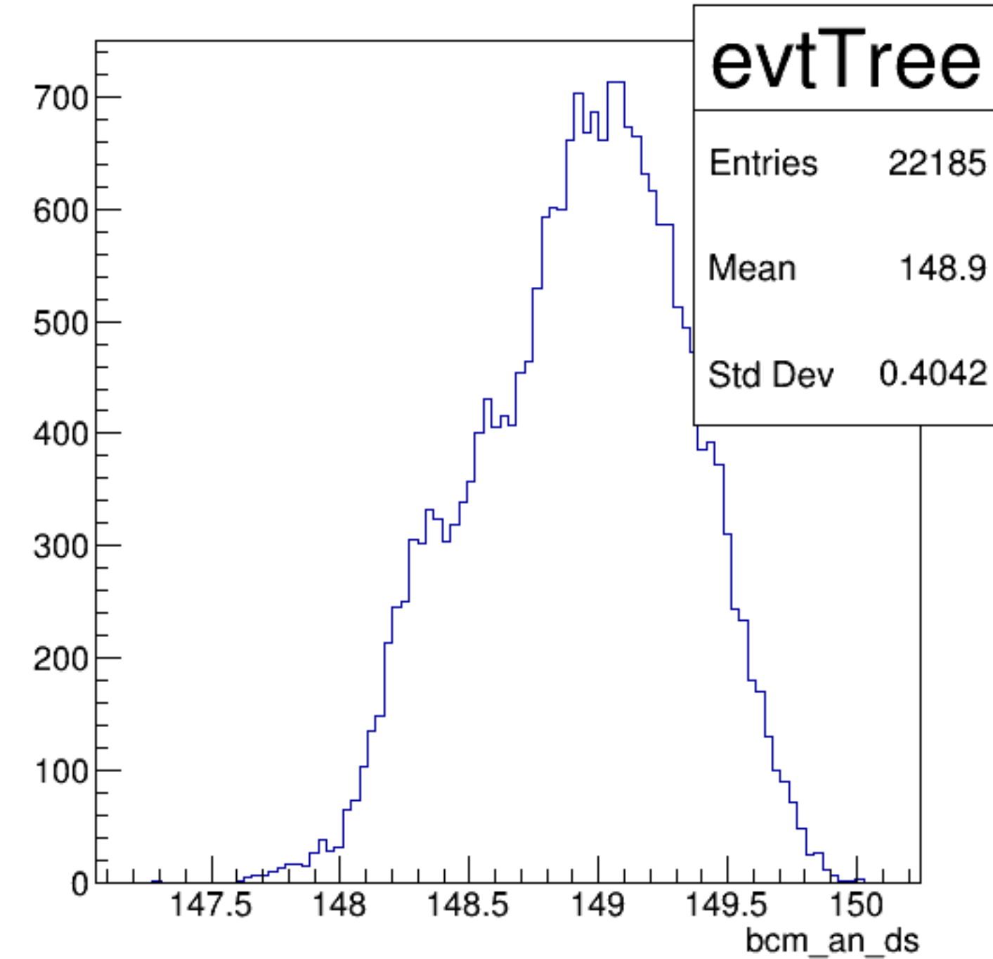
bcm_an_ds {ErrorFlag==0}
