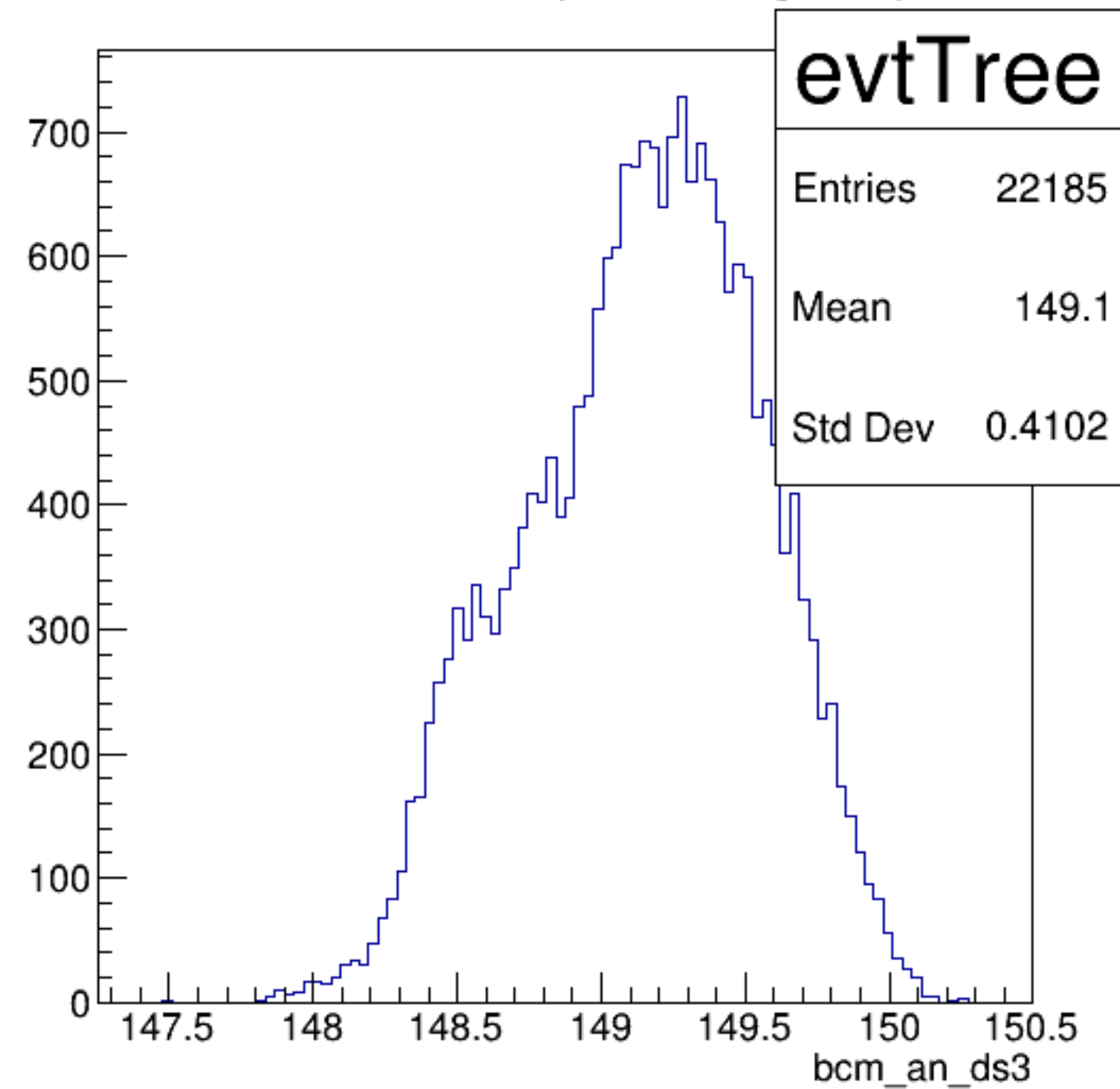
bcm_an_ds3 {ErrorFlag==0}
