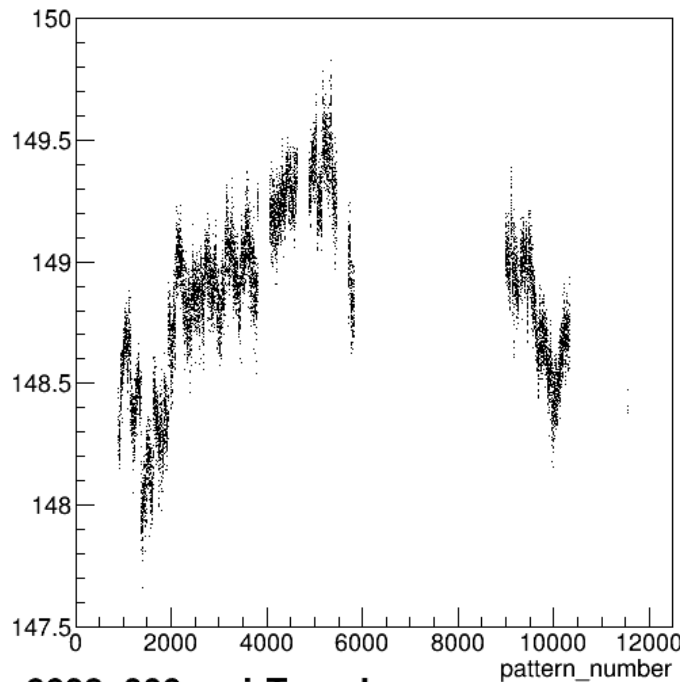
yield_bcm_an_us:pattern_number {ErrorFlag==0}
