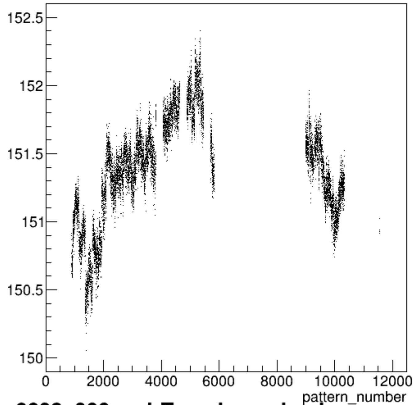
yield_bcm_dg_ds:pattern_number {ErrorFlag==0}
