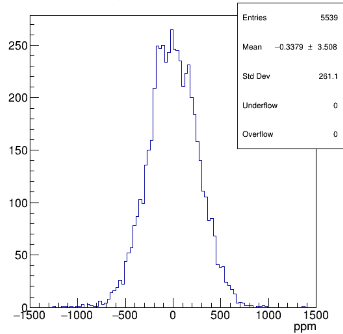
asym_bcm_an_ds3
