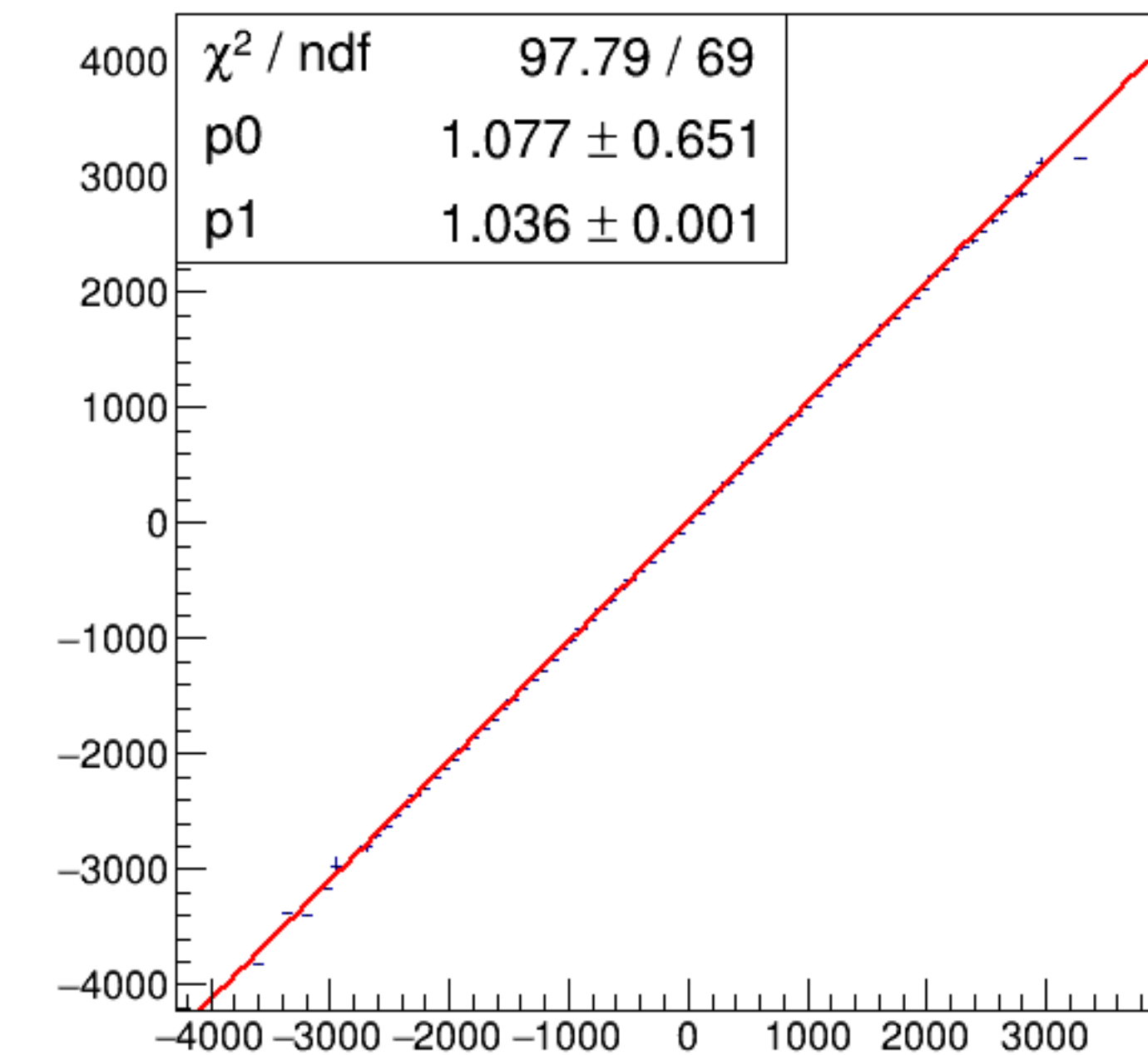
run6608_000_asym_bcm_dg_us_vs_asym_bcm_an_ds_pr.png
