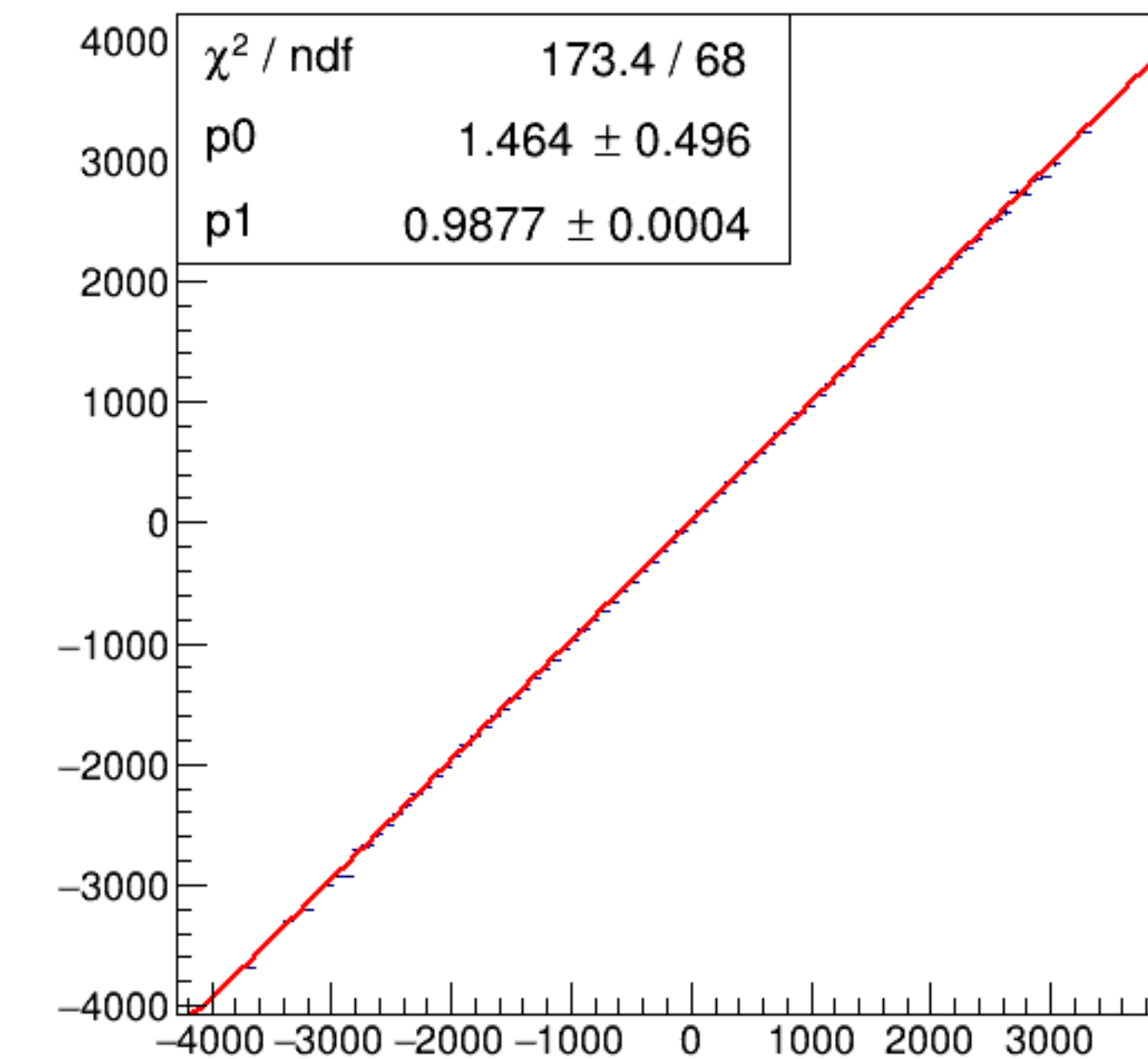
run6608_000_asym_bcm_dg_ds_vs_asym_bcm_an_us_pr.png
