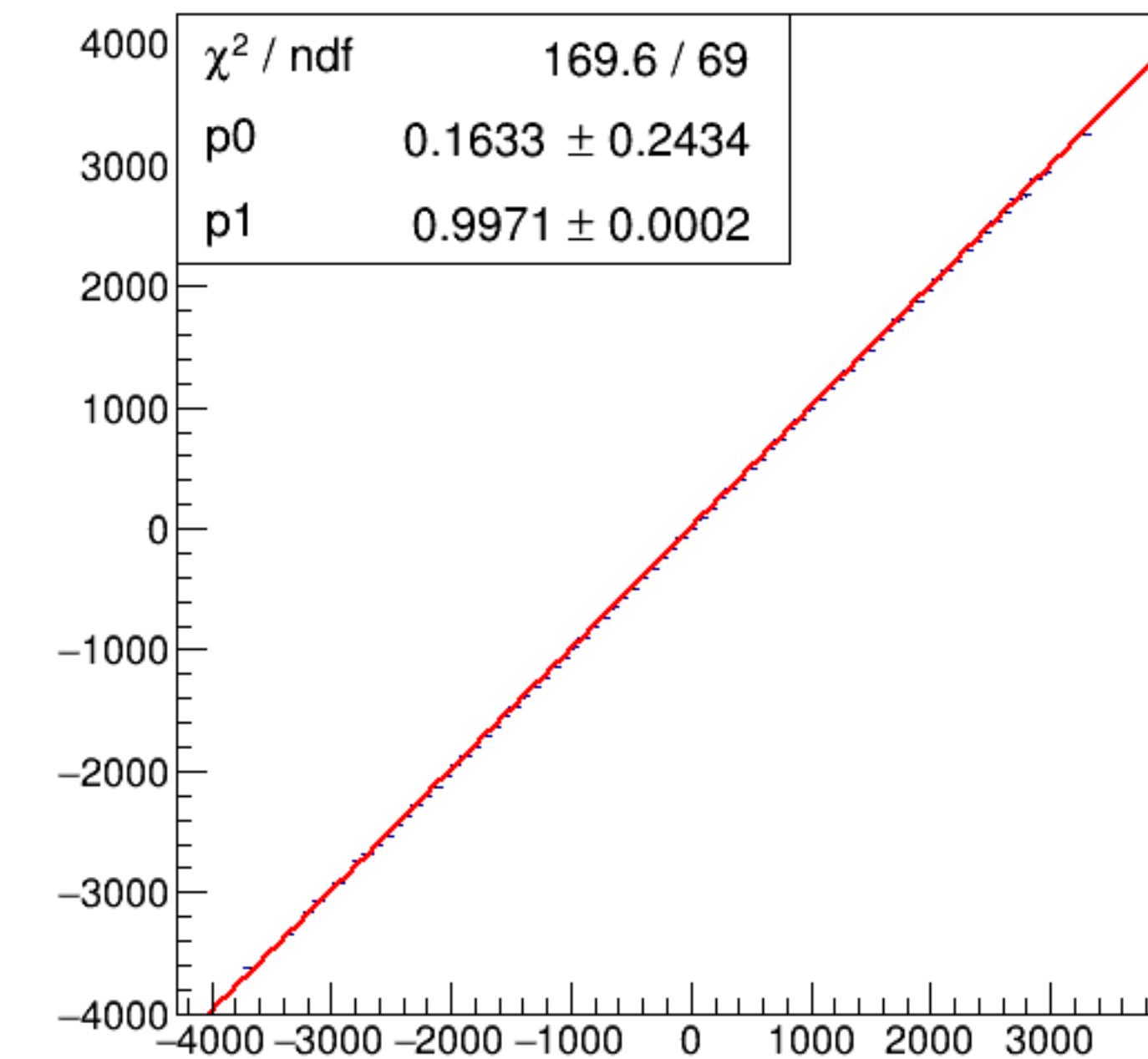
run6608_000_asym_bcm_an_ds_vs_asym_bcm_an_ds3_pr.png
