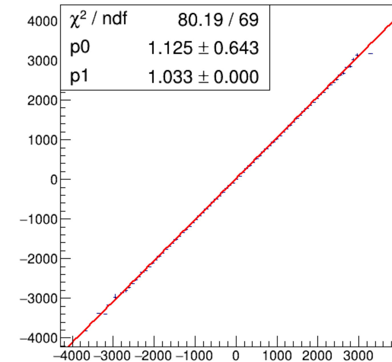
run6608_000_asym_bcm_dg_us_vs_asym_bcm_an_ds3_pr.png
