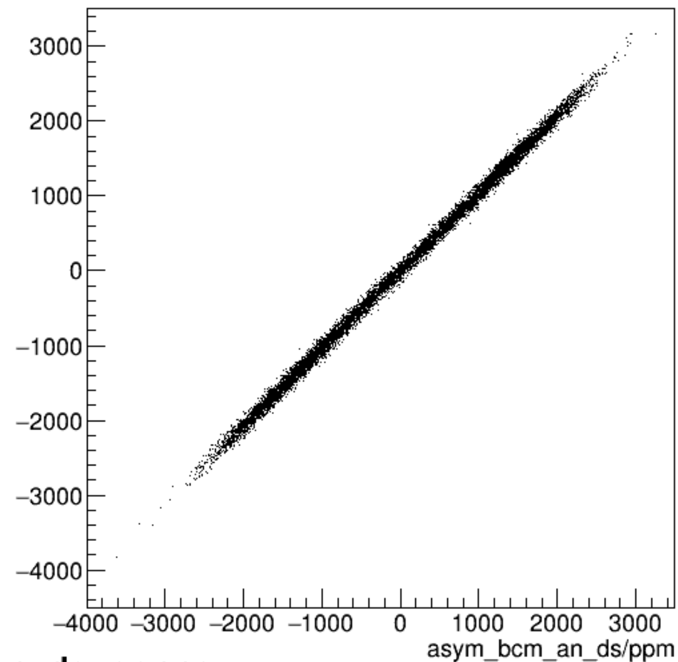
run6608_000_asym_bcm_dg_us_vs_asym_bcm_an_ds_pr.png
