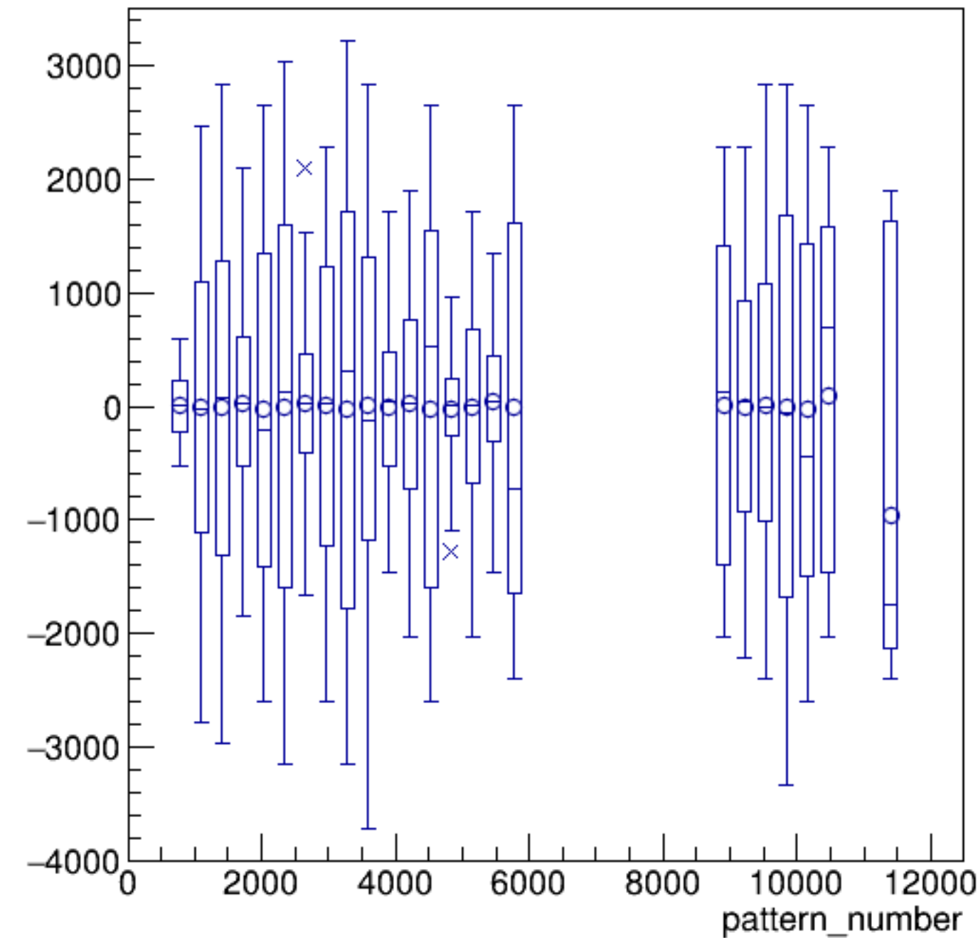
asym_bcm_an_ds/ppm:pattern_number {ErrorFlag==0}
