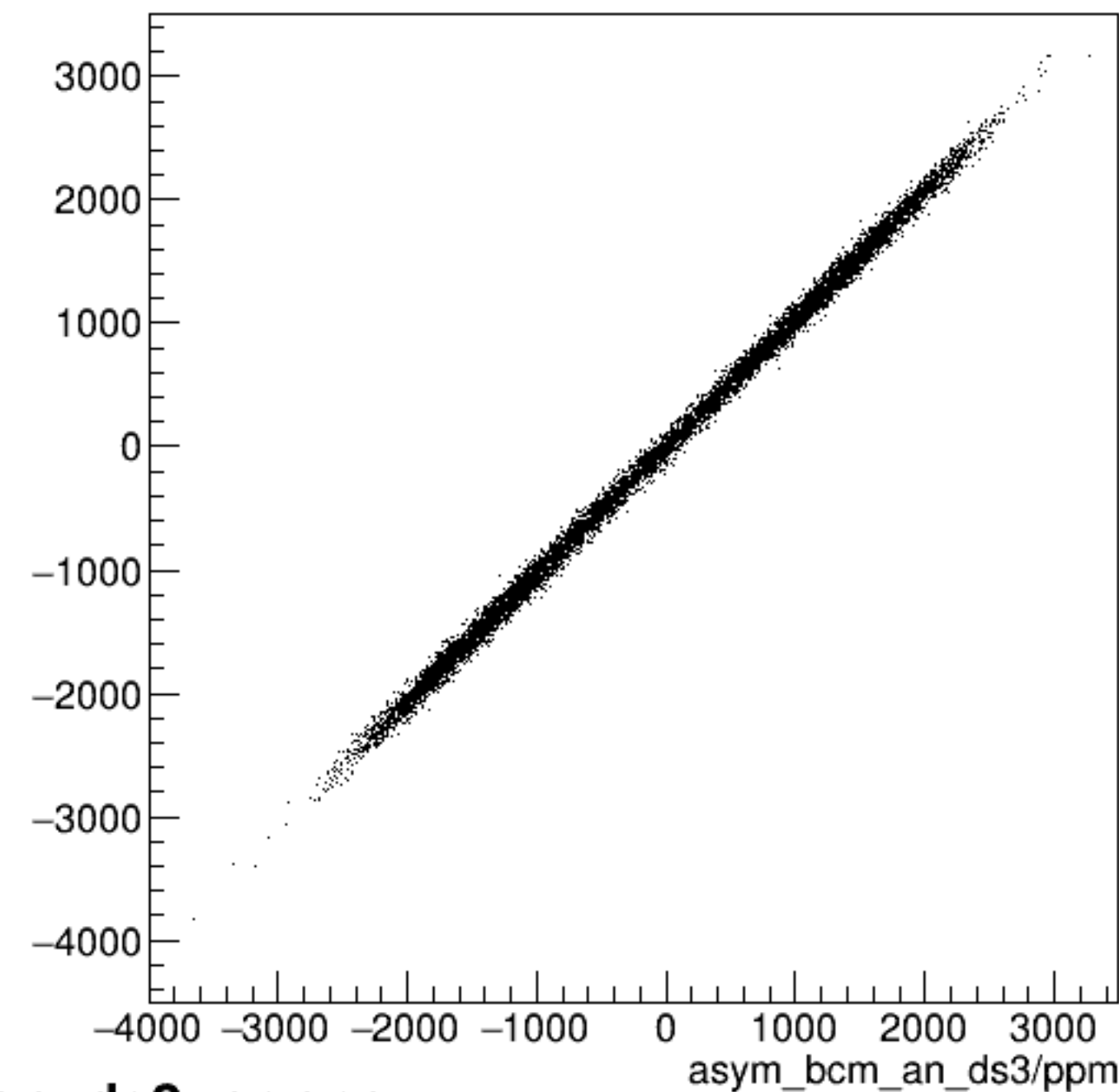
run6608_000_asym_bcm_dg_us_vs_asym_bcm_an_ds3_pr.png
