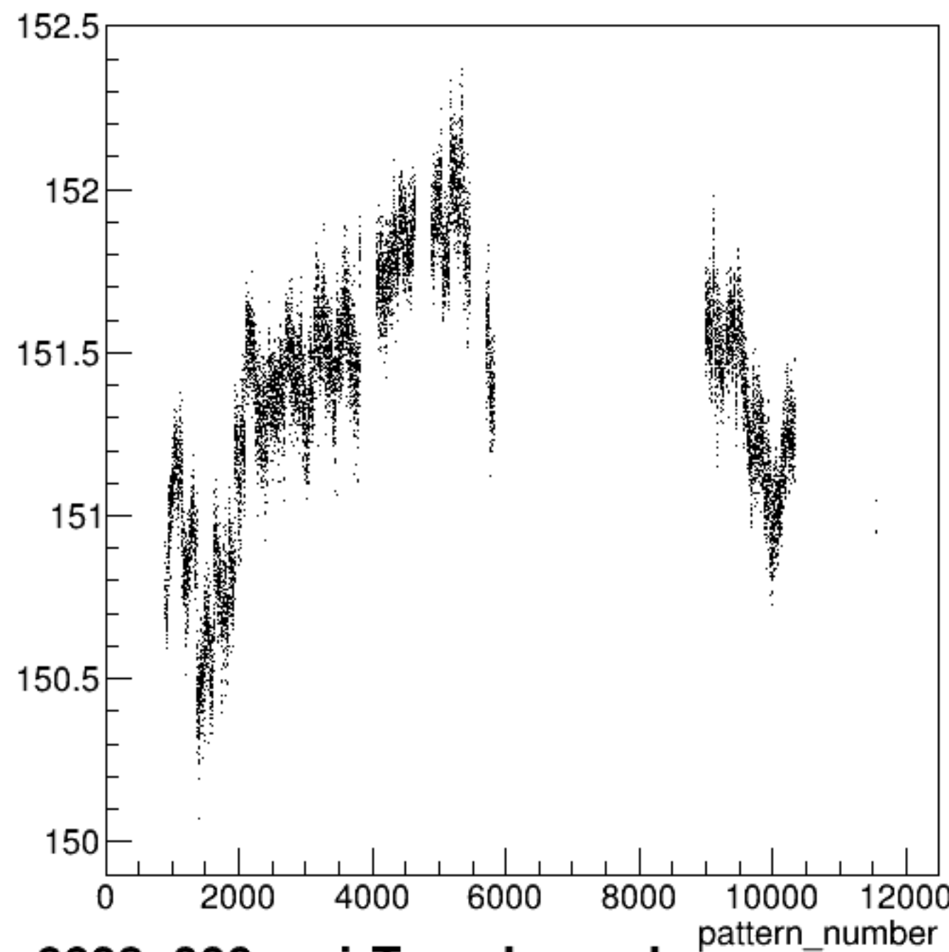
yield_bcm_dg_us:pattern_number {ErrorFlag==0}
