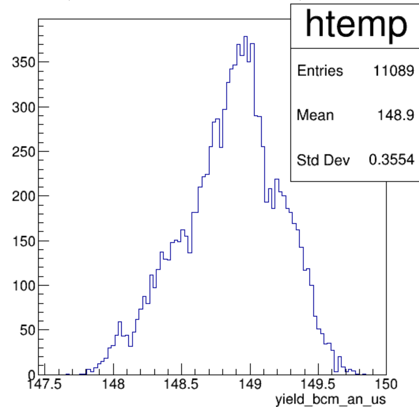
yield_bcm_an_us {ErrorFlag==0}
