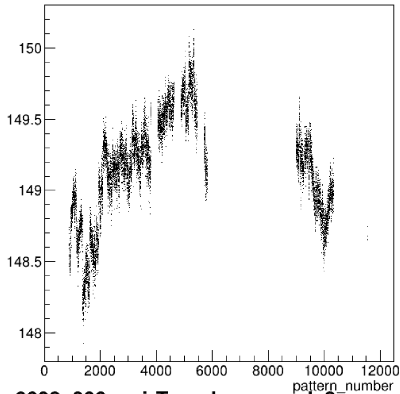
yield_bcm_an_ds3:pattern_number {ErrorFlag==0}
