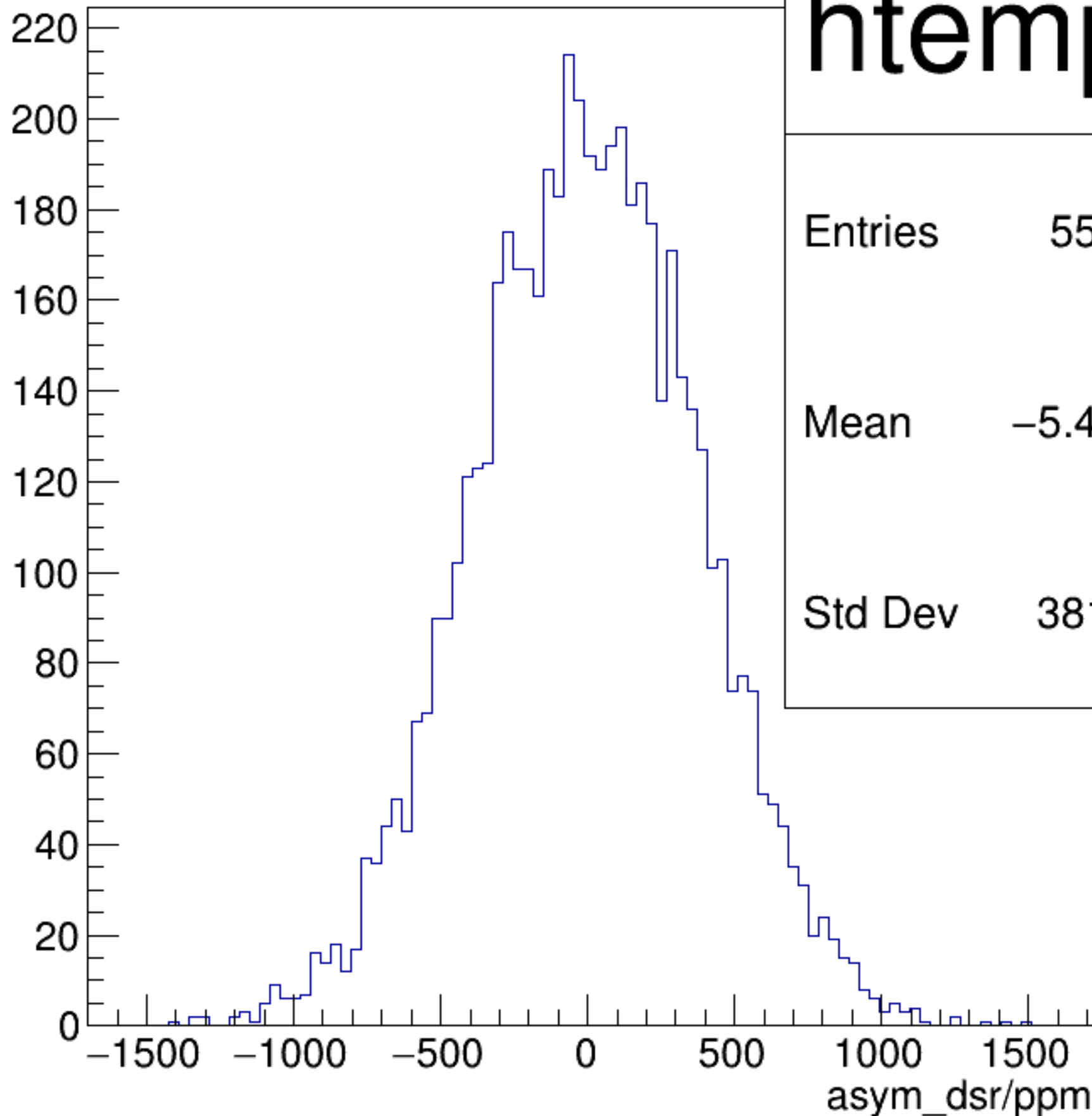
asym_dsr/ppm {ok_cut}
