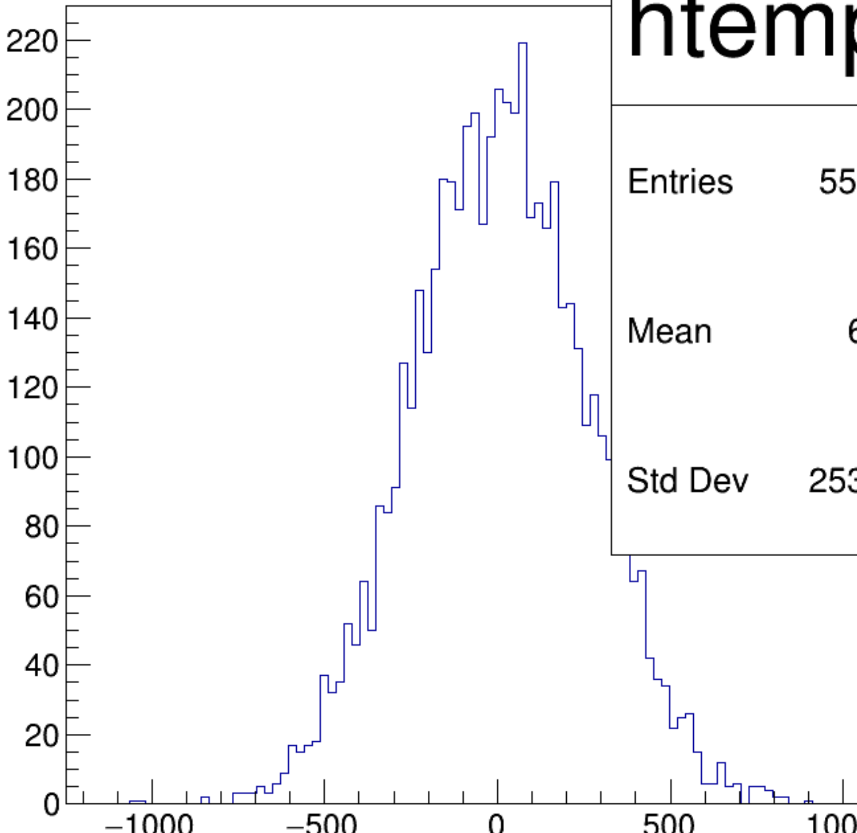
(asym_dsl/ppm-asym_dsr/ppm)/2 {ok_cut}
