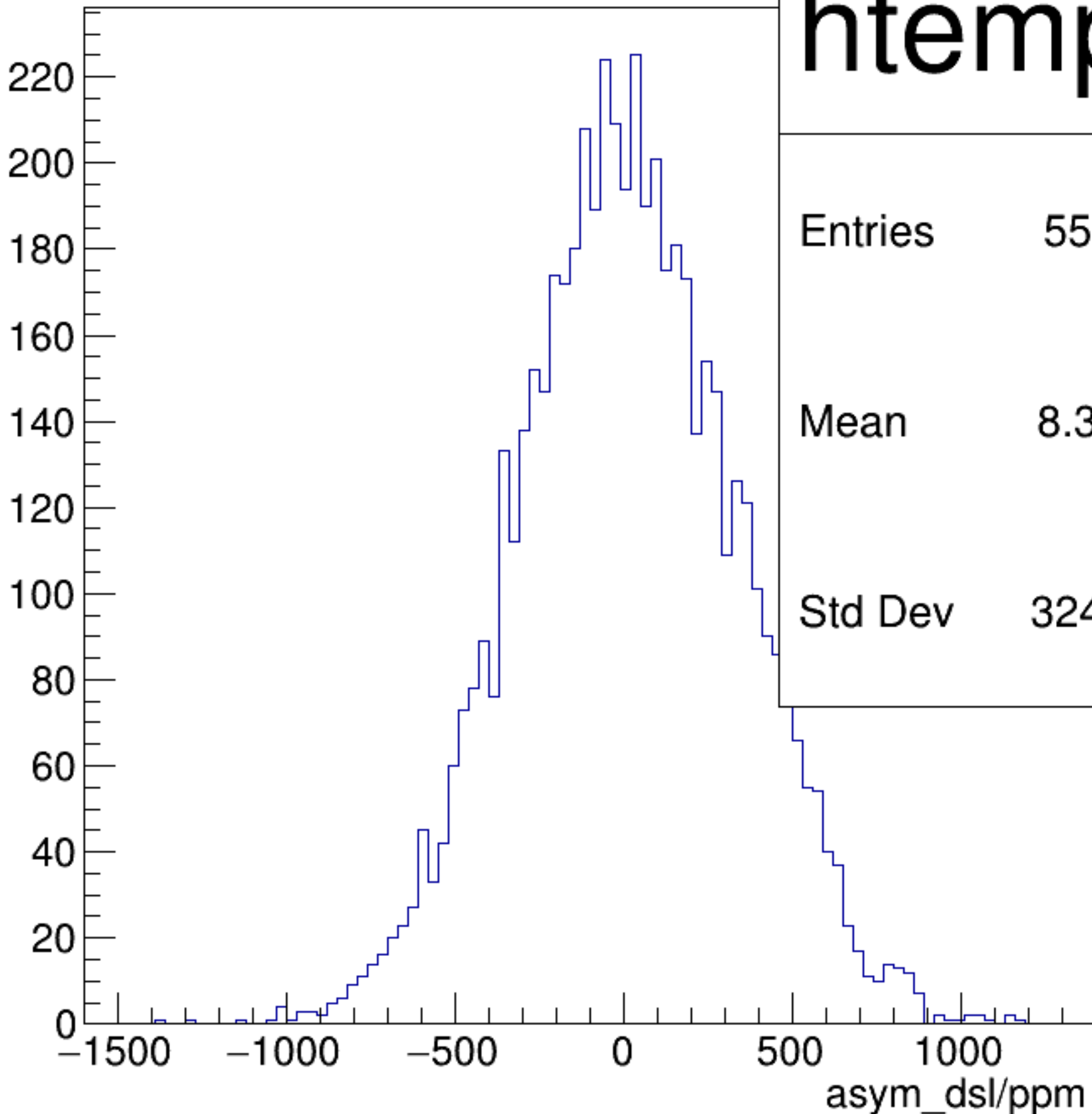
asym_dsl/ppm {ok_cut}
