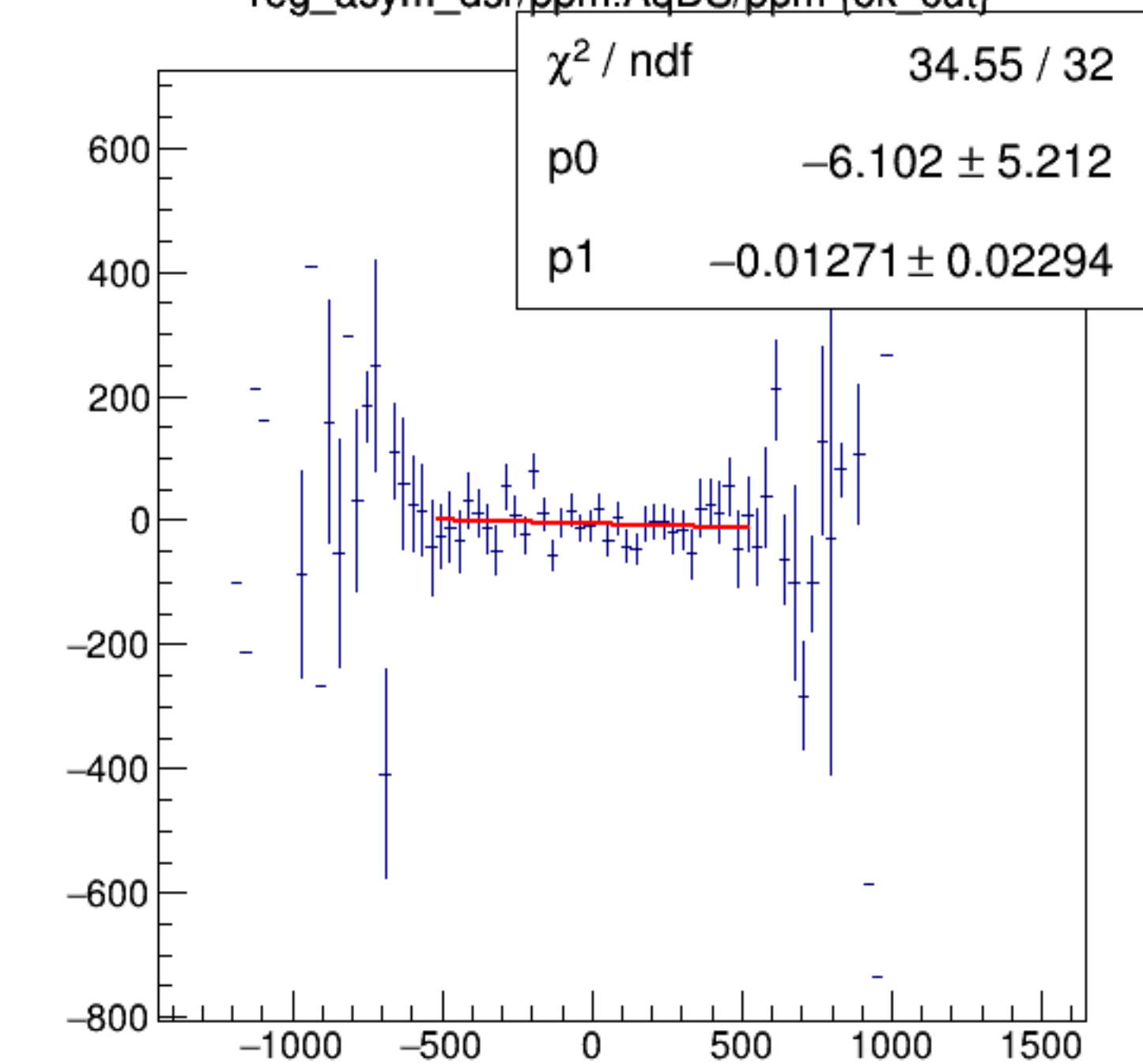
reg_asym_dsr/ppm:AqDS/ppm {ok_cut}
