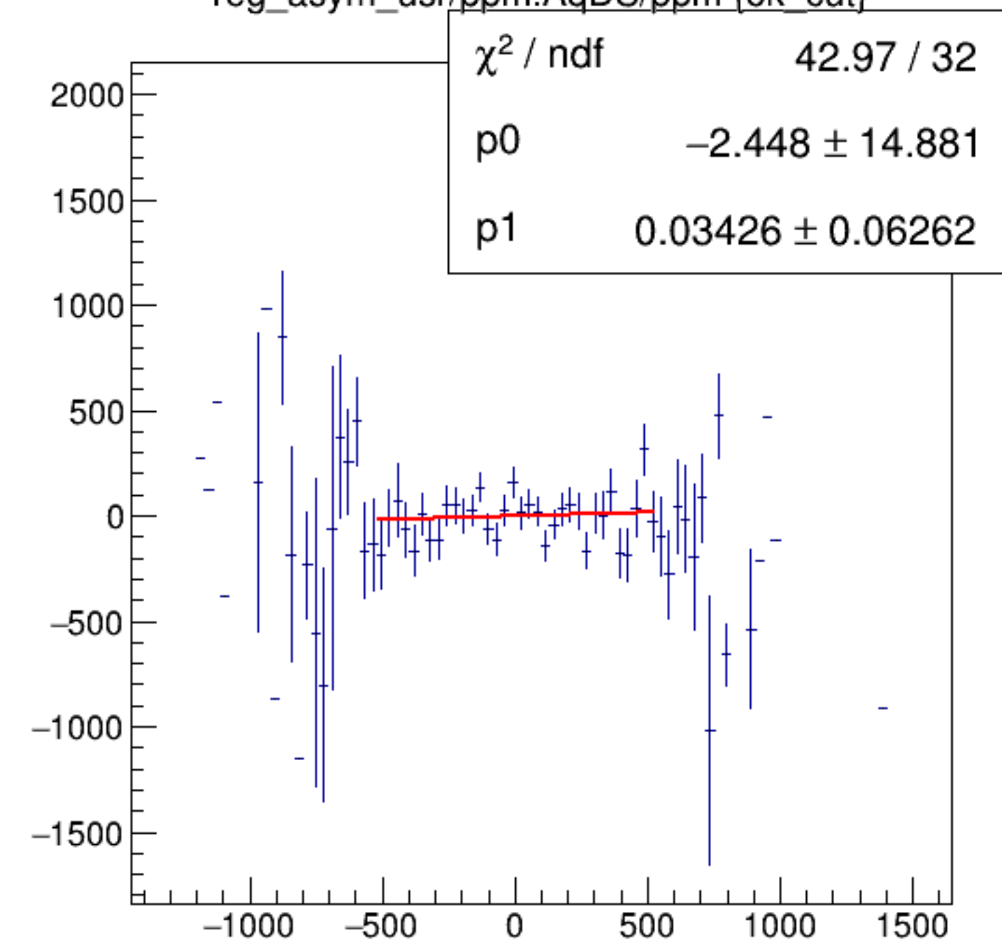
reg_asym_usr/ppm:AqDS/ppm {ok_cut}
