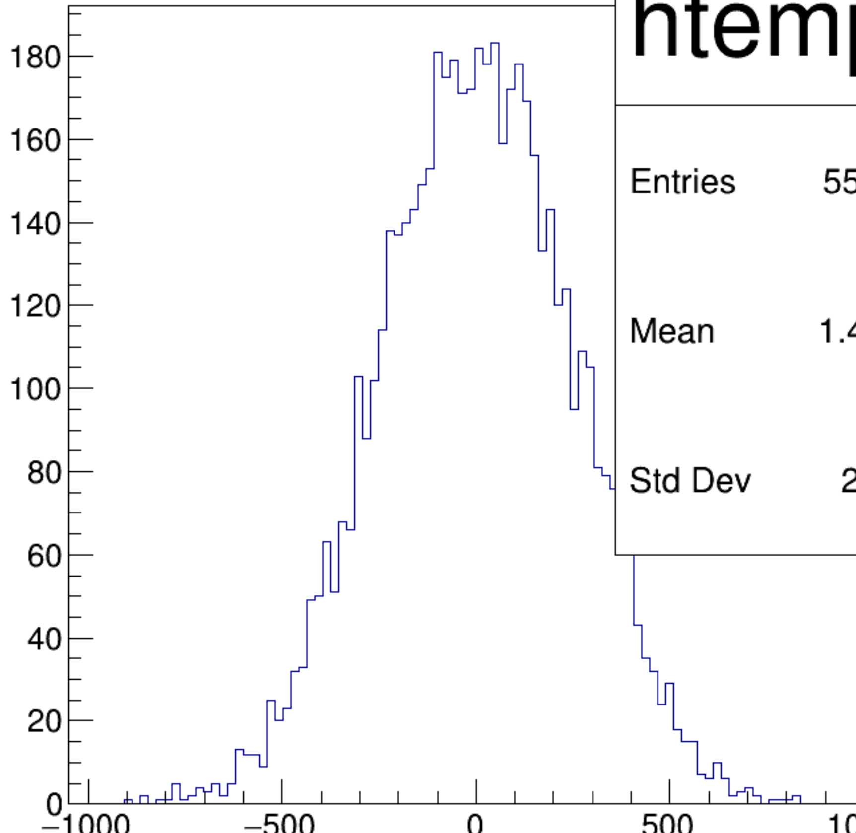
(asym_dsl/ppm+asym_dsr/ppm)/2 {ok_cut}
