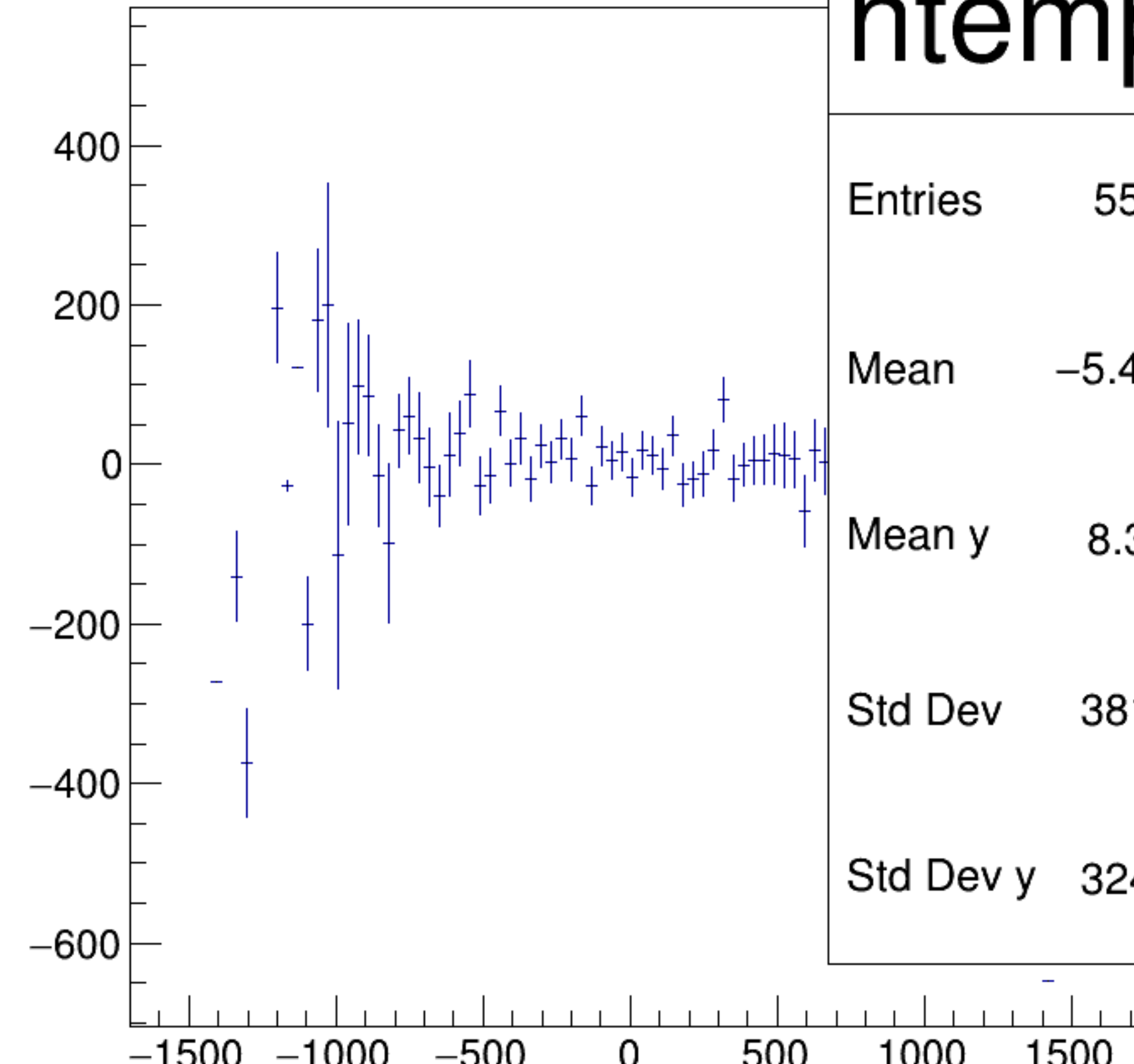
asym_dsl/ppm:asym_dsr/ppm {ok_cut}
