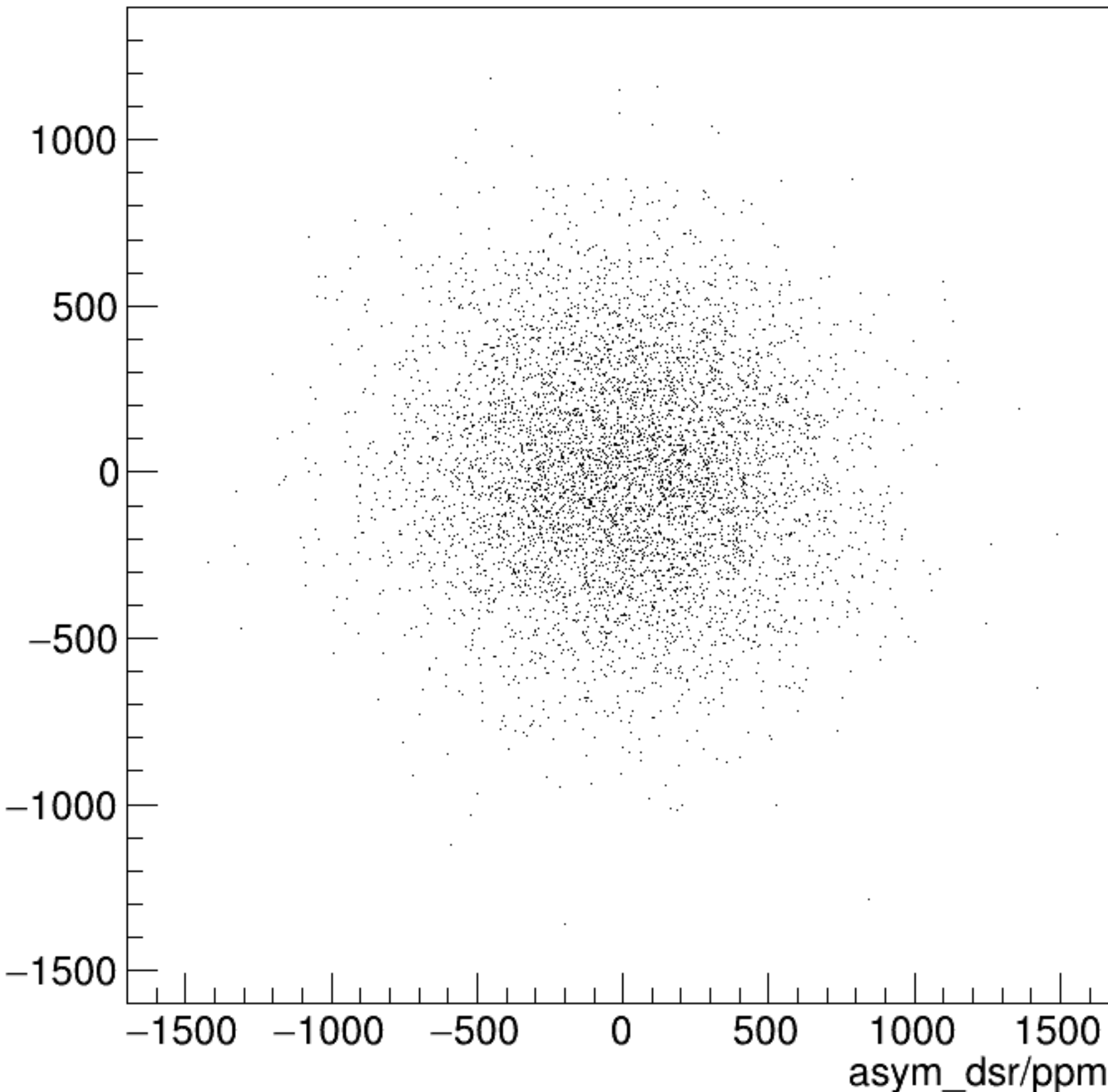
asym_dsl/ppm:asym_dsr/ppm {ok_cut}
