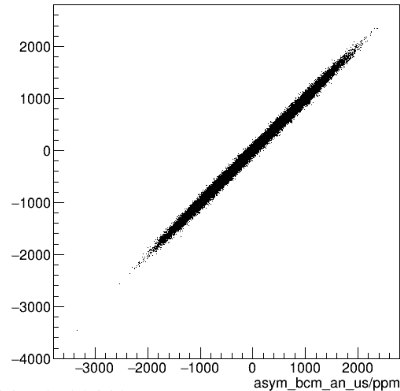
run6627_000_asym_bcm_dg_ds_vs_asym_bcm_an_us_pr.png
