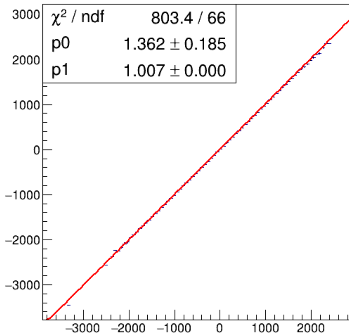
run6627_000_asym_bcm_dg_ds_vs_asym_bcm_an_us_pr.png
