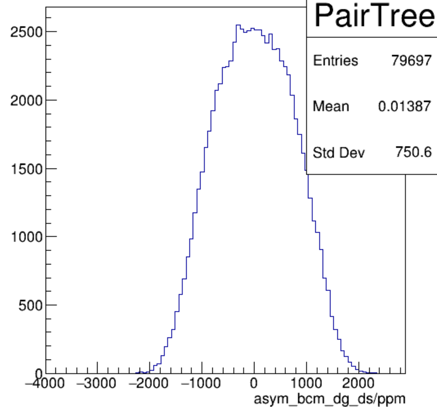
asym_bcm_dg_ds/ppm {ErrorFlag==0}
