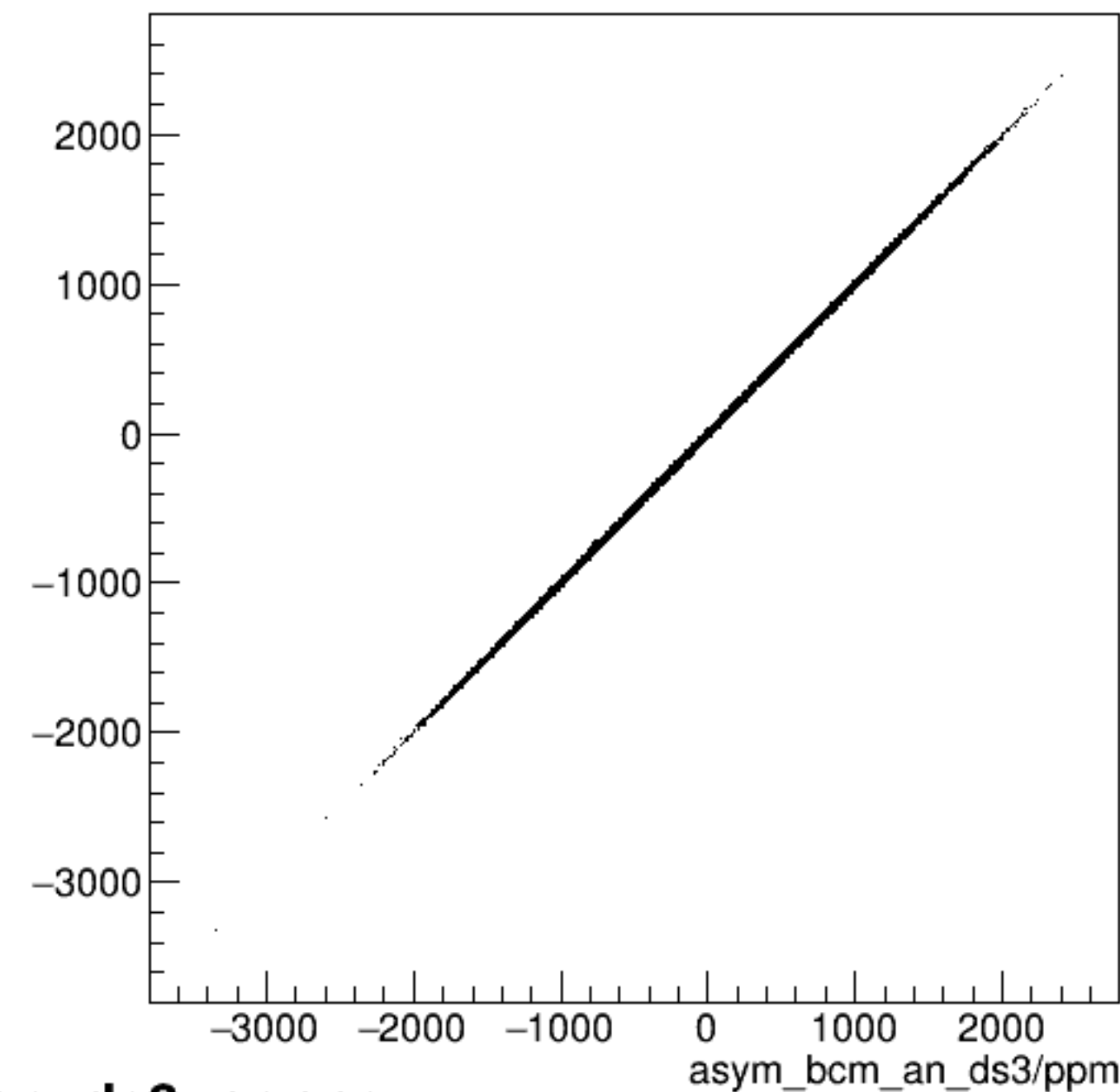
run6627_000_asym_bcm_an_ds_vs_asym_bcm_an_ds3_pr.png
