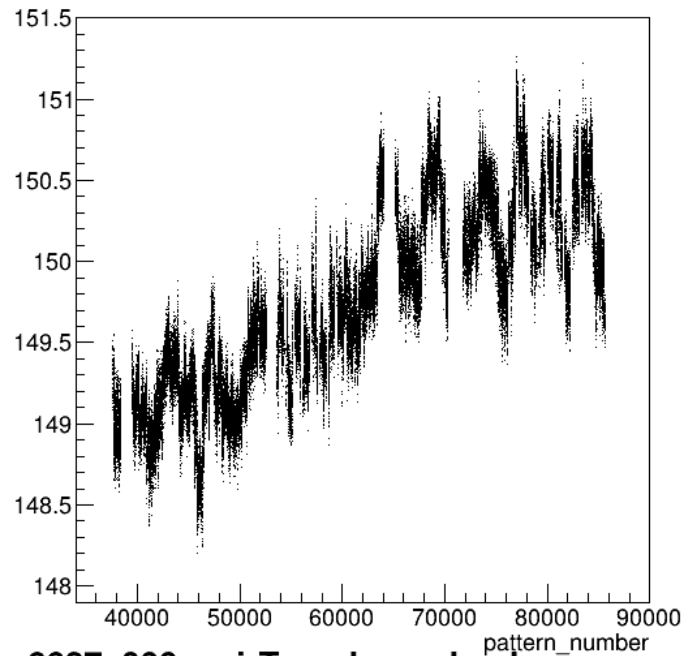
yield_bcm_dg_ds:pattern_number {ErrorFlag==0}
