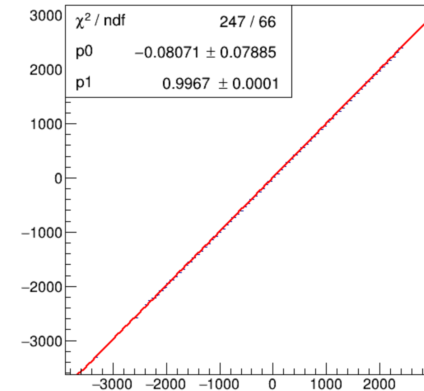
run6627_000_asym_bcm_an_ds_vs_asym_bcm_an_ds3_pr.png
