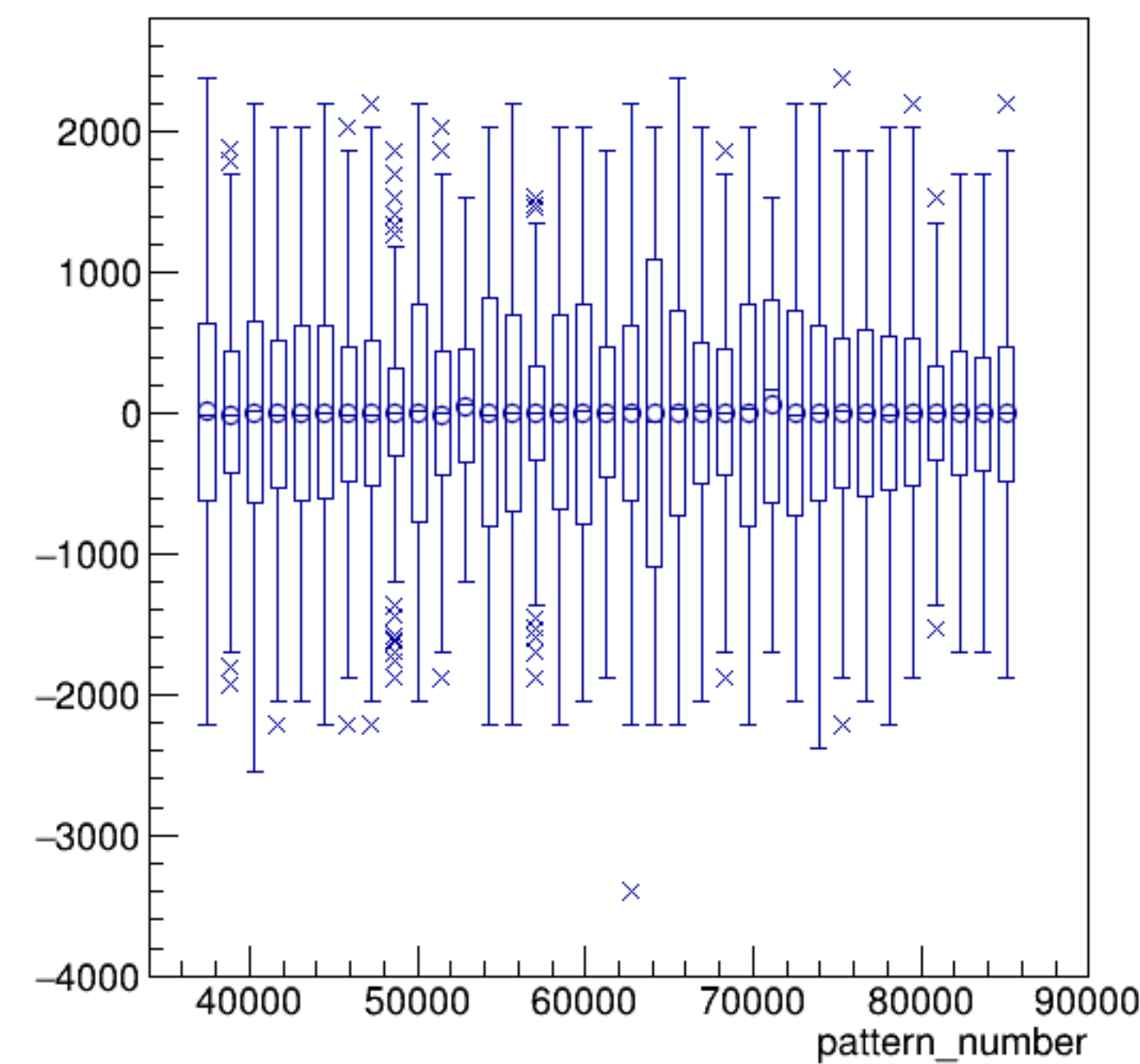
asym_bcm_dg_ds/ppm:pattern_number {ErrorFlag==0}
