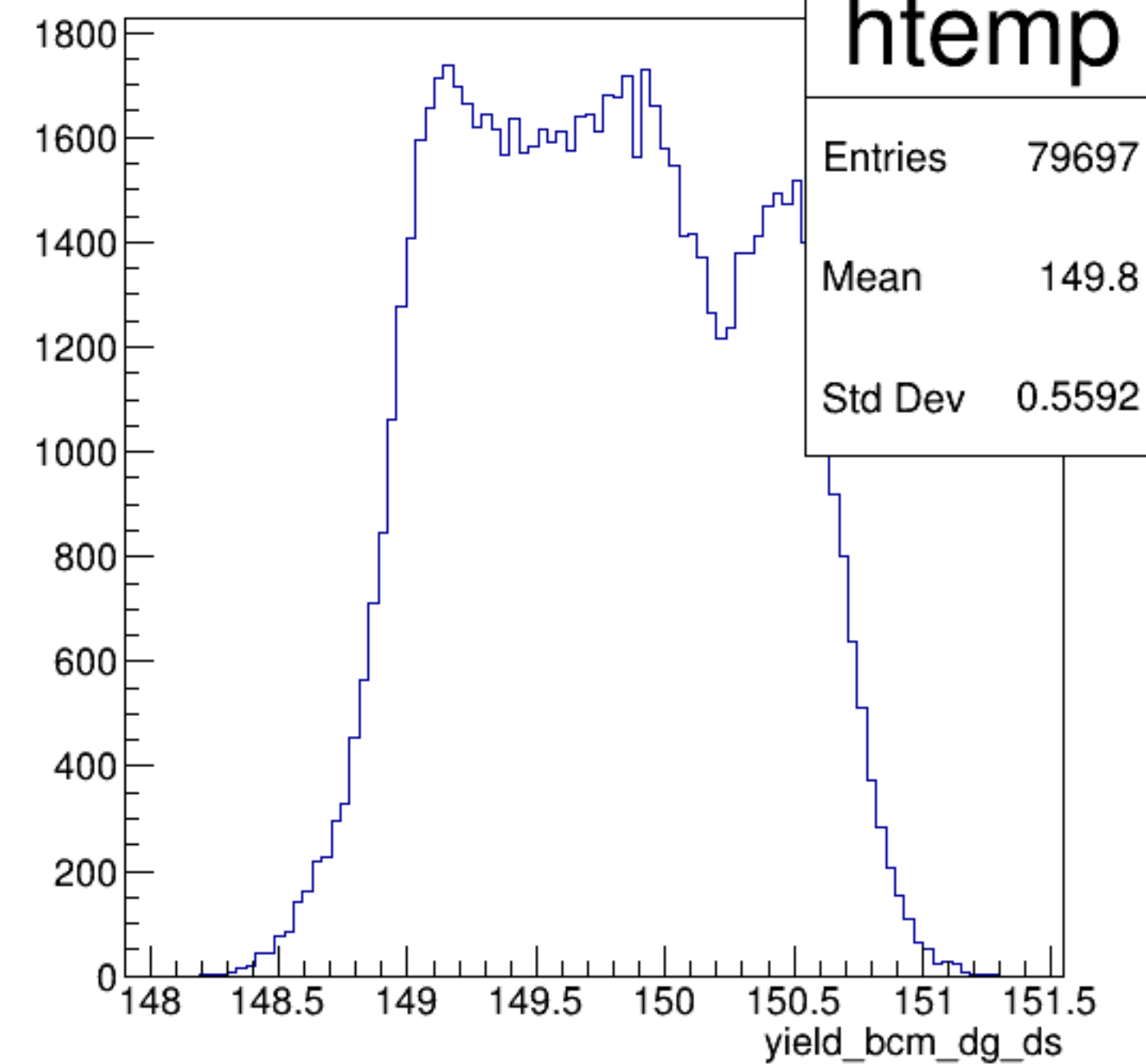
yield_bcm_dg_ds {ErrorFlag==0}
