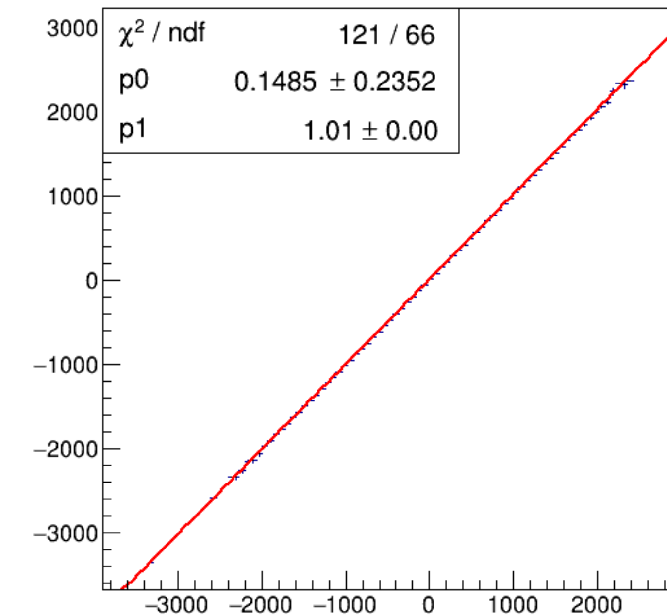
run6627_000_asym_bcm_dg_us_vs_asym_bcm_an_ds3_pr.png
