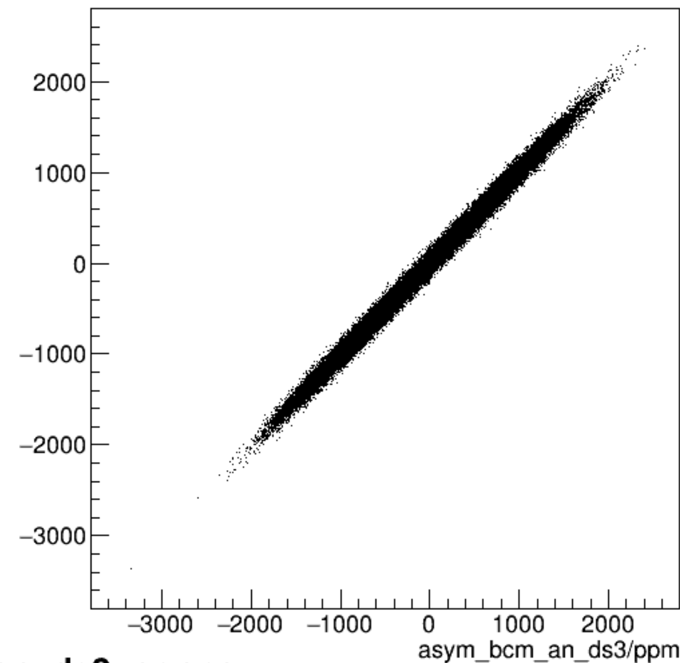
run6627_000_asym_bcm_dg_us_vs_asym_bcm_an_ds3_pr.png
