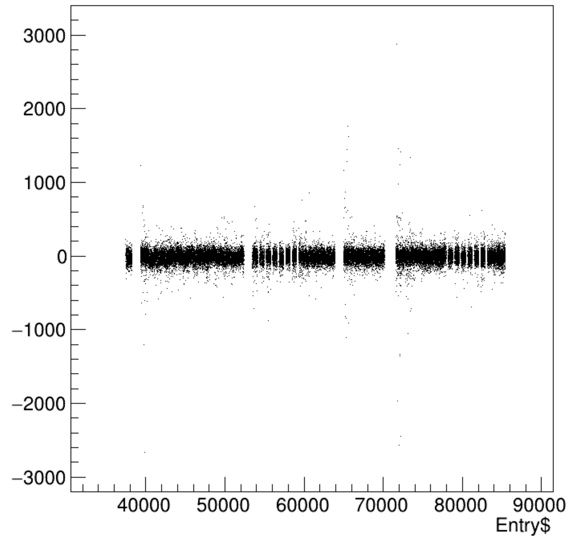
asym_bpm2i02WS/ppm:Entry$ {ErrorFlag==0}
