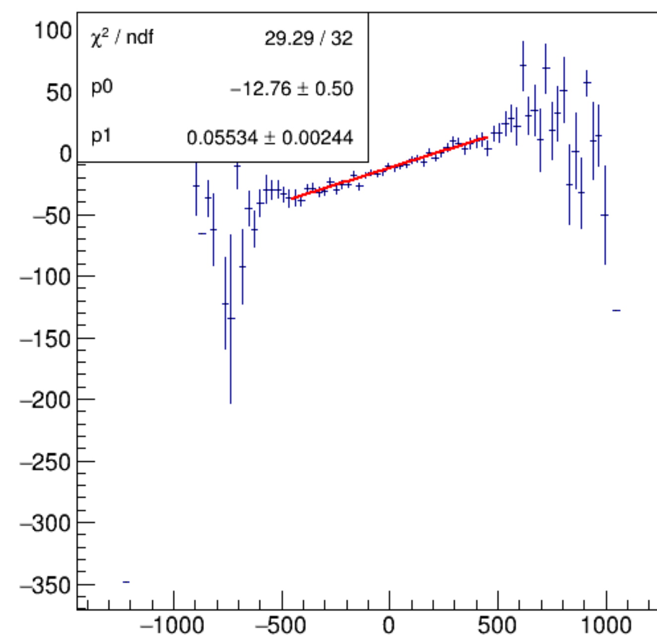
asym_bpm1i02WS/ppm:Aq/ppm {ErrorFlag==0}
