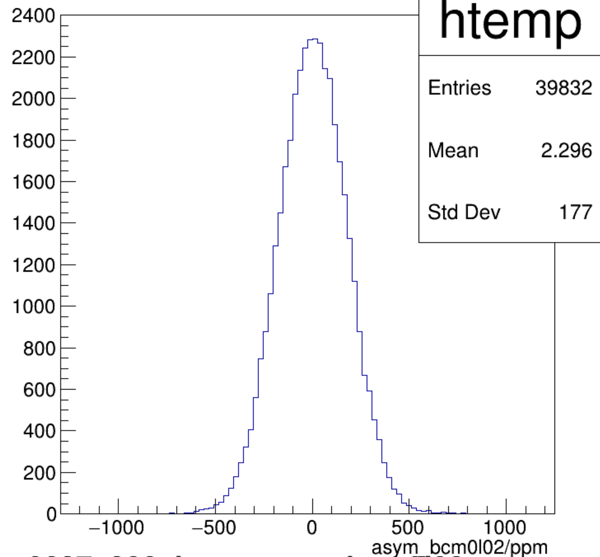
asym_bcm0l02/ppm {ErrorFlag==0}
