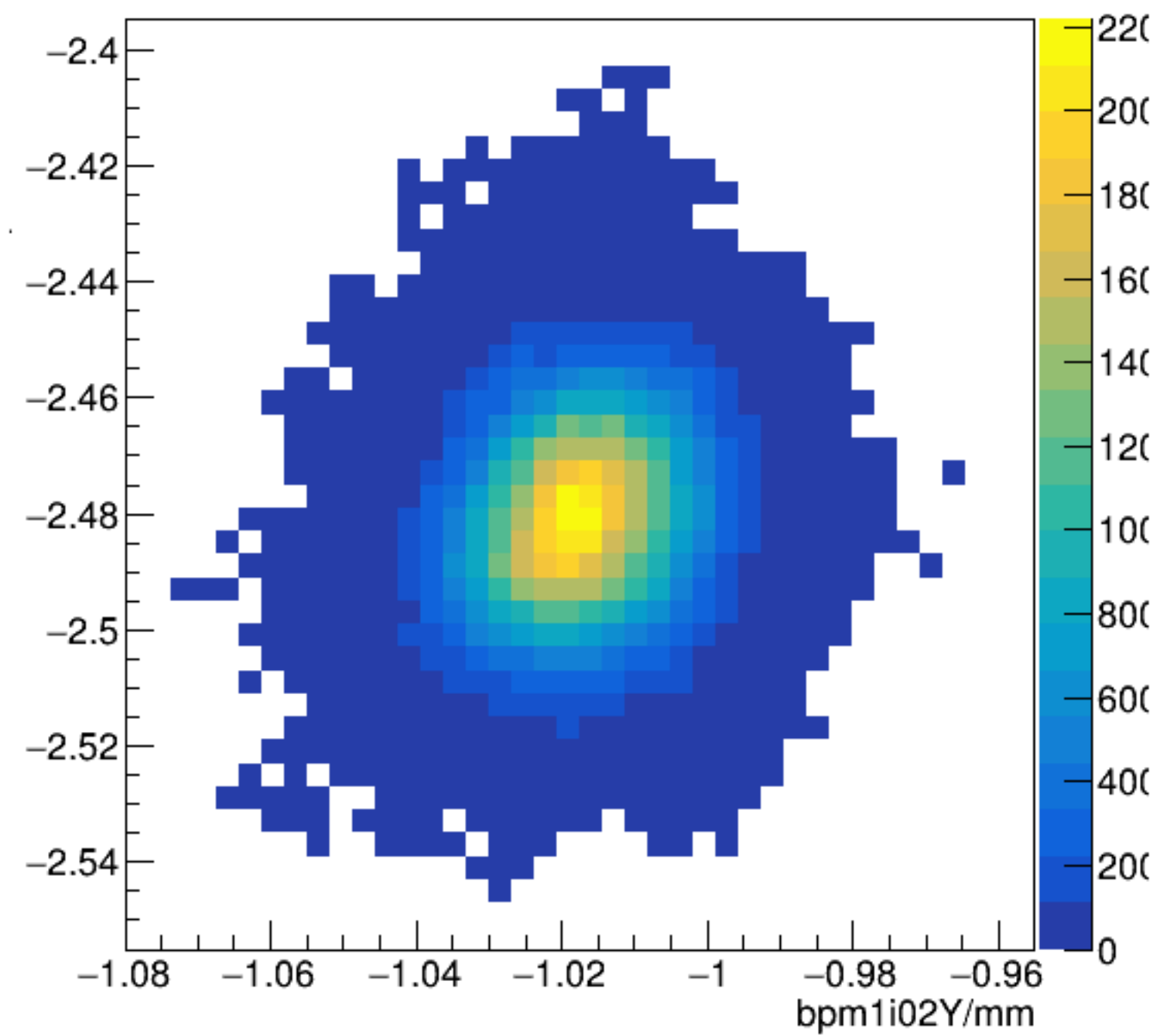
bpm1i02X/mm:bpm1i02Y/mm {ErrorFlag==0}
