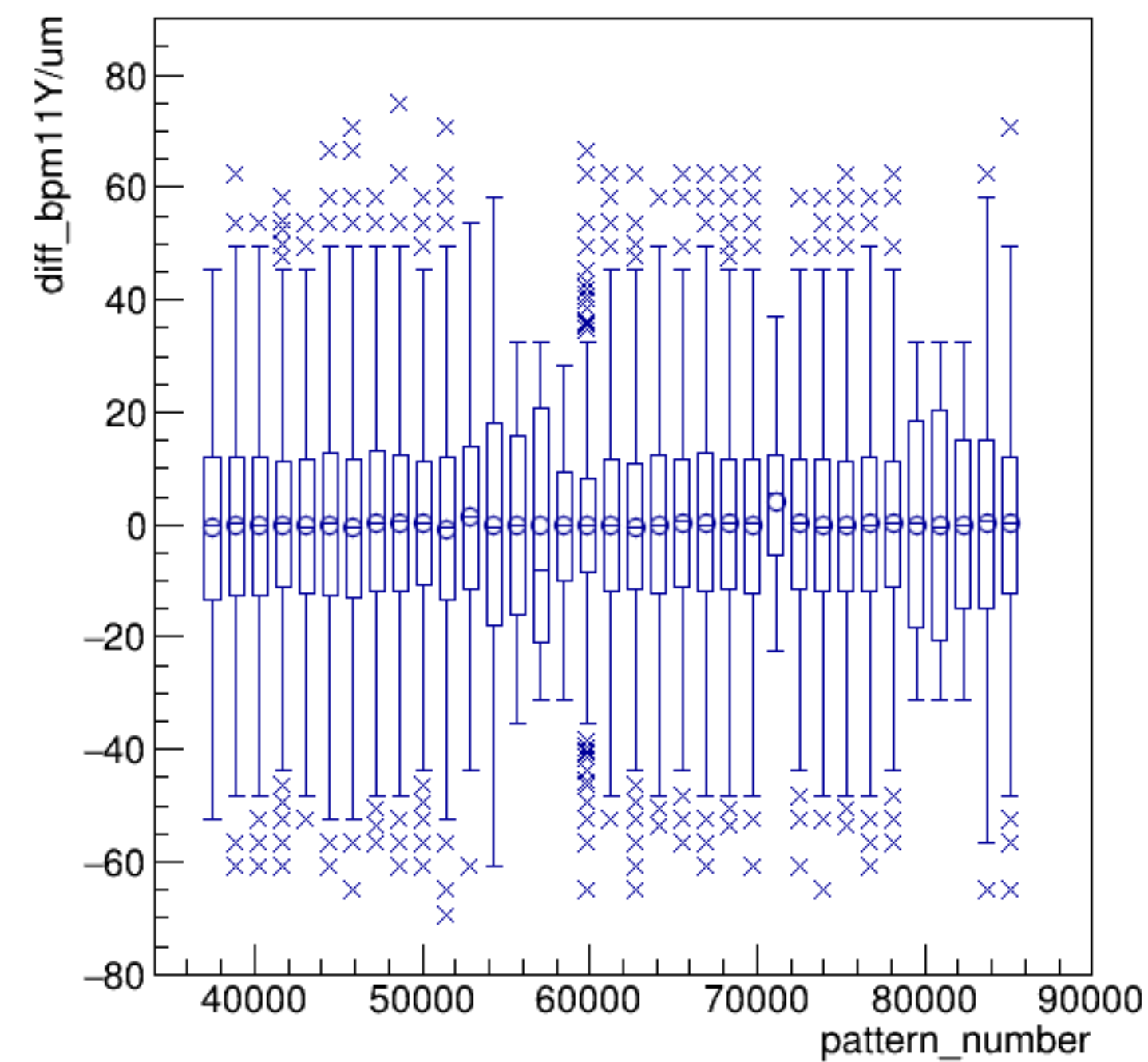
diff_bpm11Y/um:pattern_number {ErrorFlag==0}
