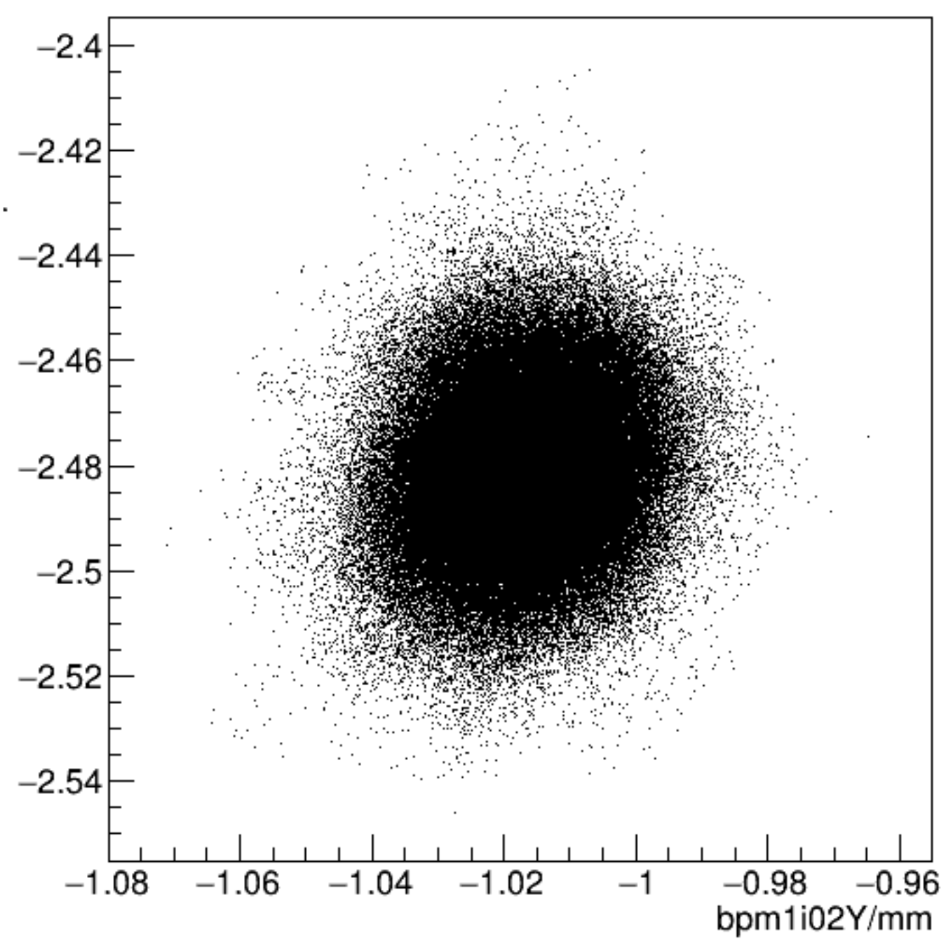
bpm1i02X/mm:bpm1i02Y/mm {ErrorFlag==0}
