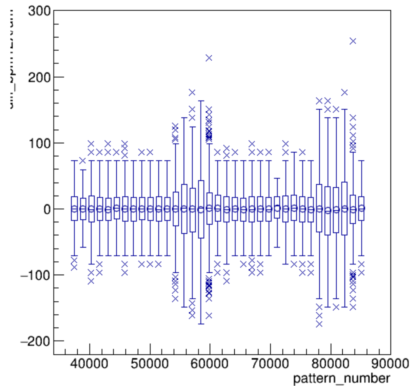
diff_bpm12X/um:pattern_number {ErrorFlag==0}
