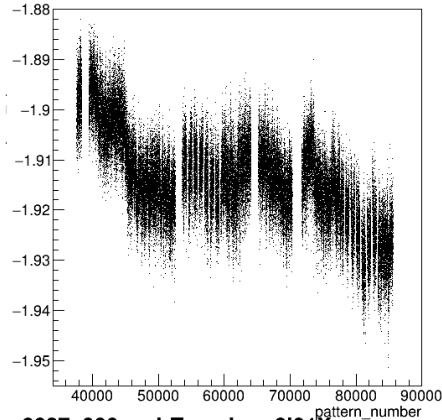
yield_bpm0l01X/mm:pattern_number {ErrorFlag==0}
