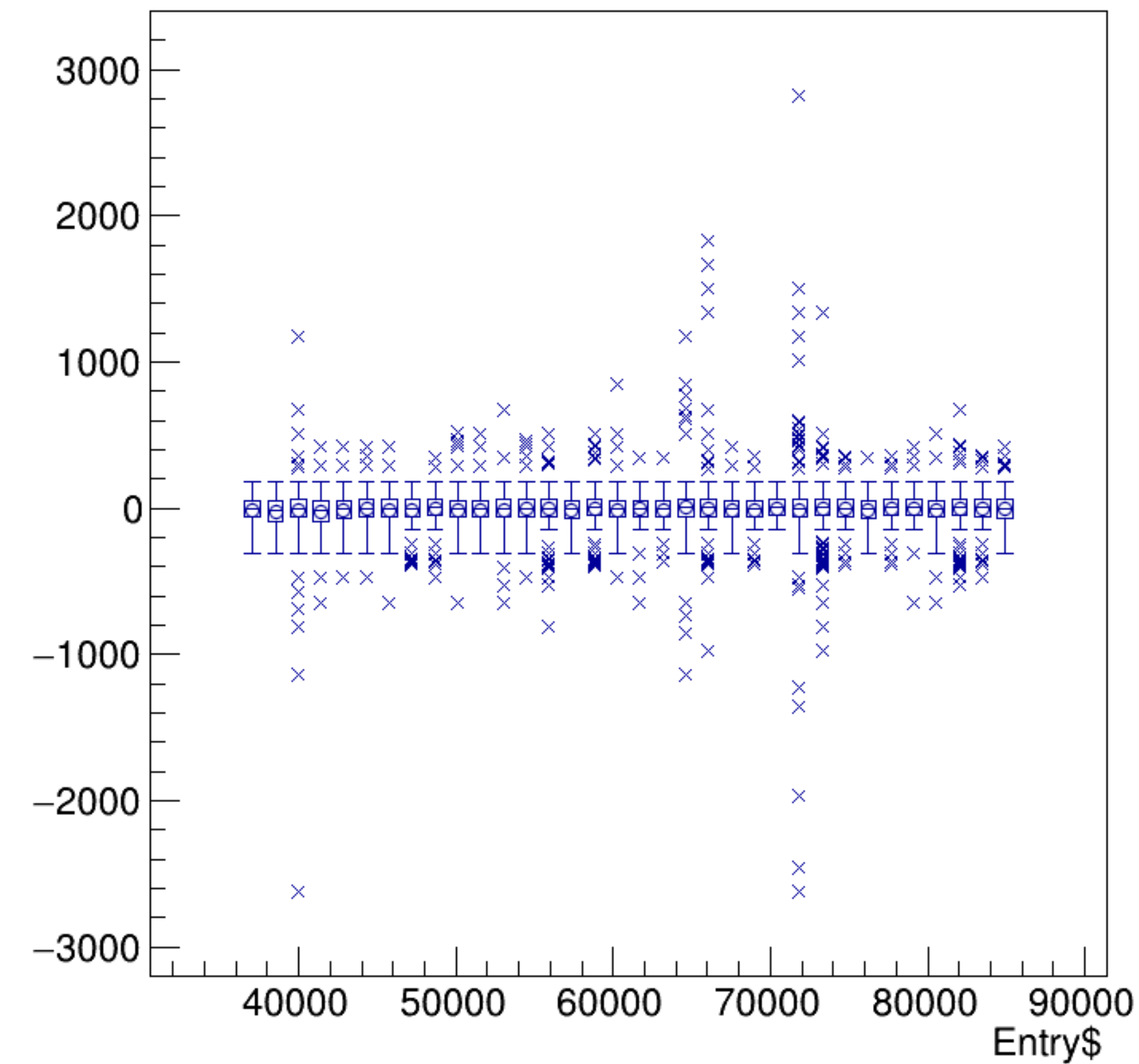
asym_bpm2i02WS/ppm:Entry$ {ErrorFlag==0}
