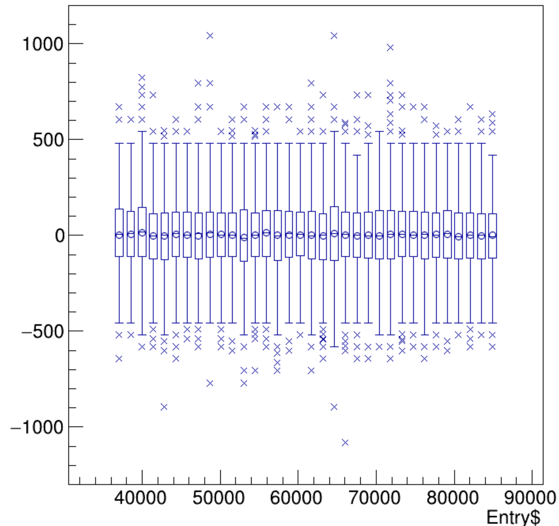
asym_bcm0l02/ppm:Entry$ {ErrorFlag==0}
