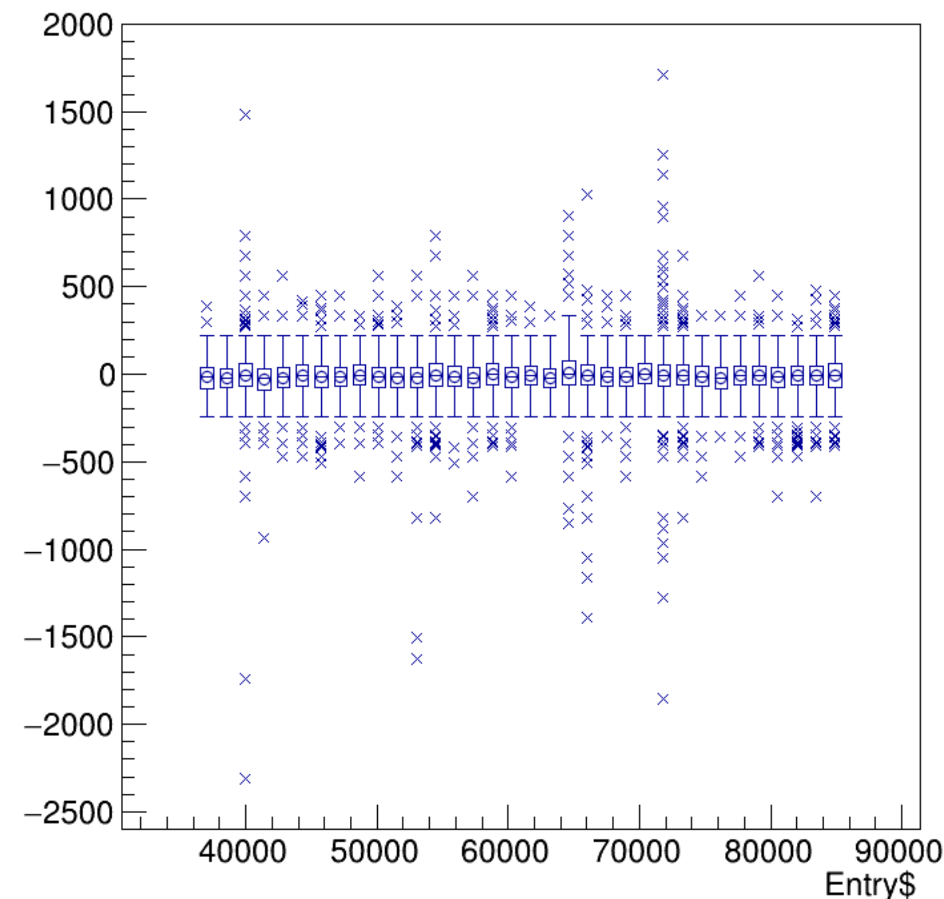
asym_bpm1i02WS/ppm:Entry$ {ErrorFlag==0}
