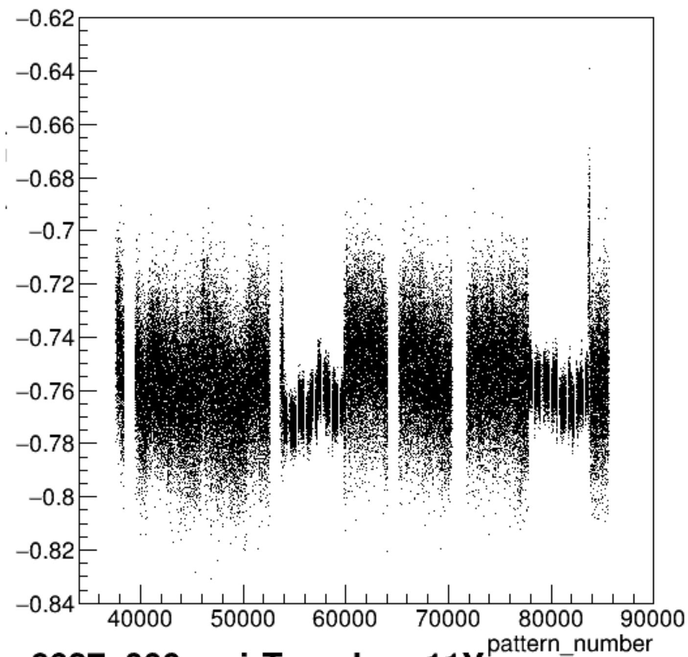
yield_bpm11Y/mm:pattern_number {ErrorFlag==0}
