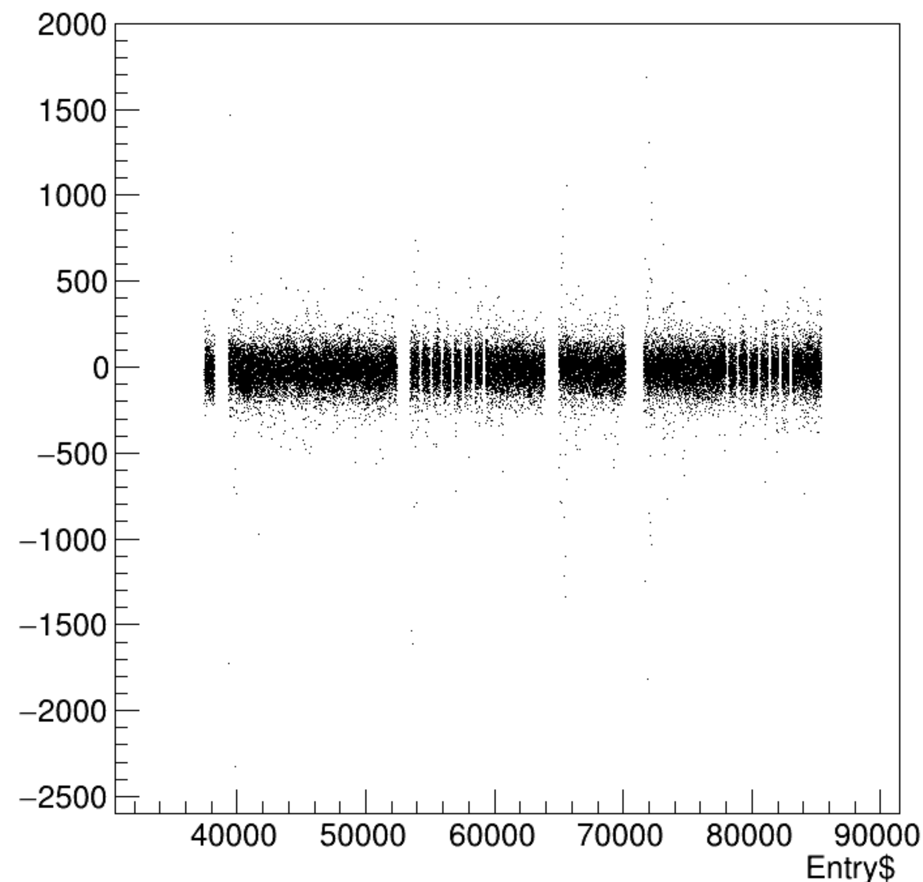
asym_bpm1i02WS/ppm:Entry$ {ErrorFlag==0}
