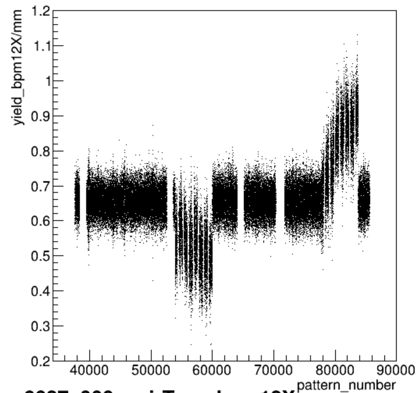
yield_bpm12X/mm:pattern_number {ErrorFlag==0}
